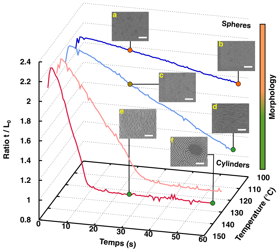
Figure 2.4.: Main image: Kinetics of film thickness of PS- b -PDMS 42 kg/mol with DOS under thermal annealing for temperatures between 110–140 °C by in-situ ellipsometry. Top-view SEM images of PS- b -PDMS after 30 s (a,c,e) and 60 s (b,d,f) of thermal annealing in the range 110–140 °C. Scale bar corresponds to 200 nm.
