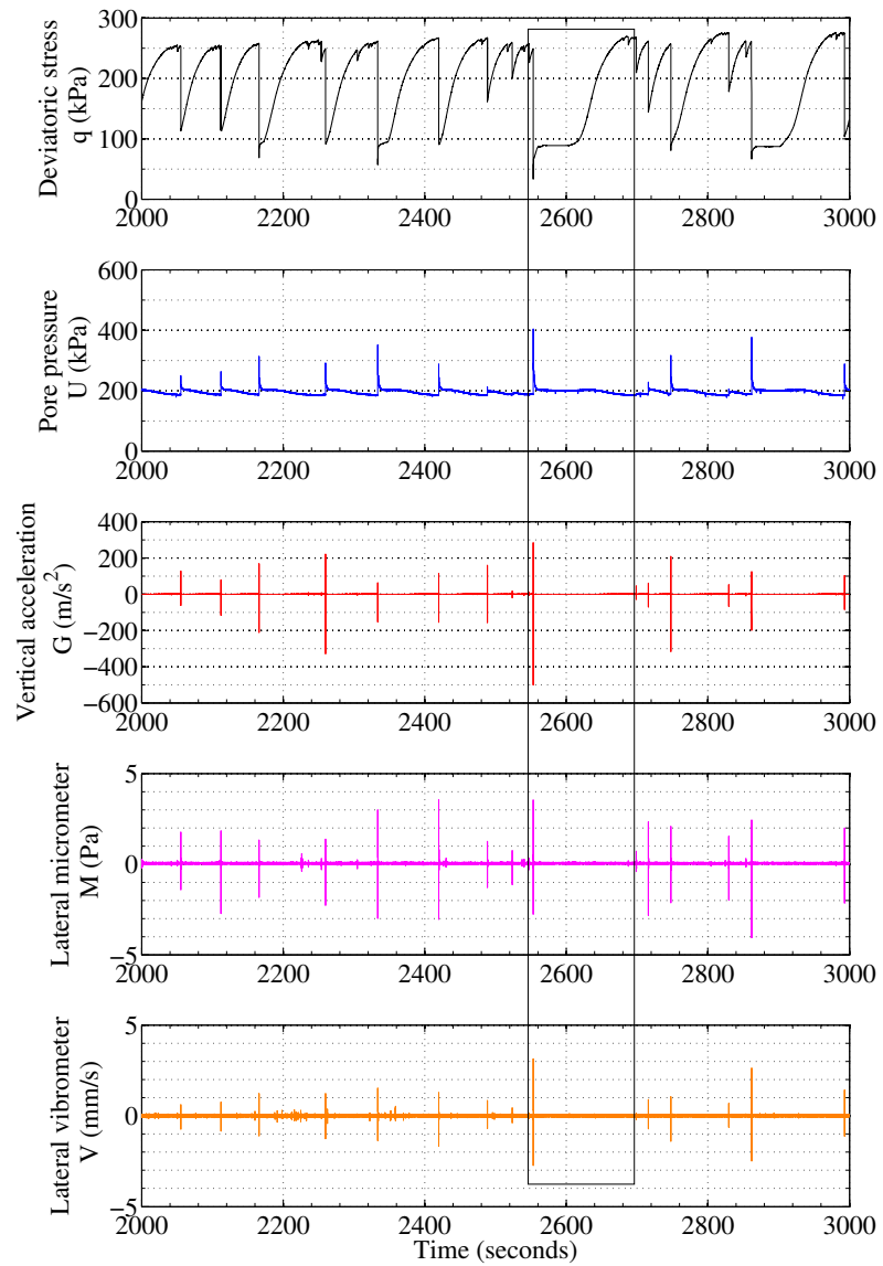
Figure 6.3: Mechanical and acoustical measurements within 1000 seconds of test N120-CIDNC series.
