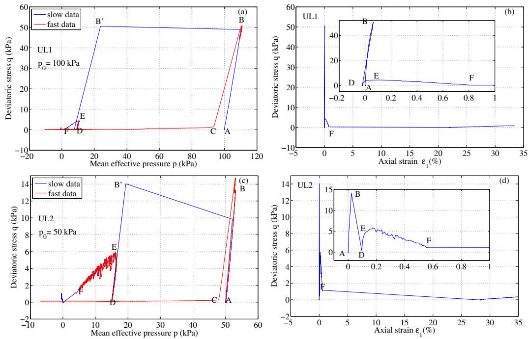
Figure 5.5: Global behaviour in static liquefaction of test UL 01 (a,b) and UL 02 (c,d).
