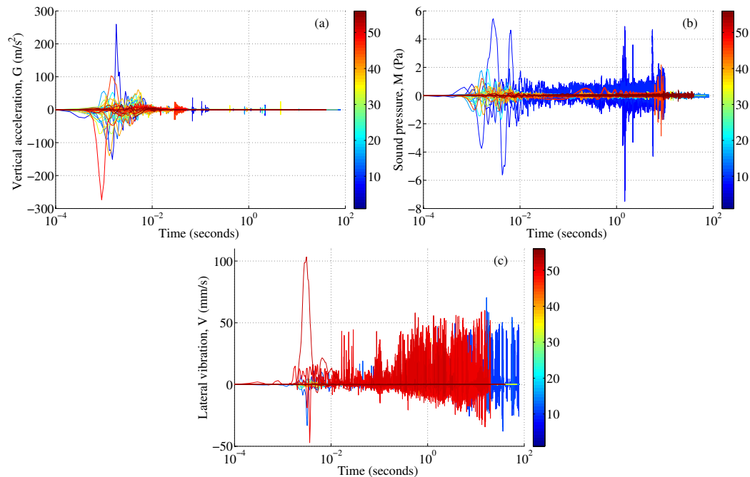
Figure 6.6: Detailed temporal evolution of G, M, V measurements of Collapse series.
