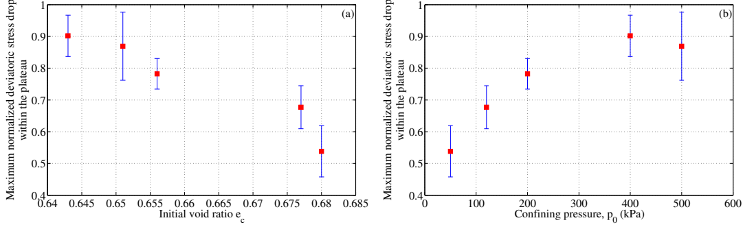
Figure 4.11: Effect of void ratio and confining pressure on the global behaviour of stick-slip.
