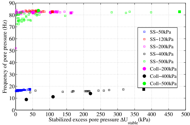
Figure 4.13: Effect of stabilised excess pore pressure \Delta U_{stable} on the frequency of pore pressure.
