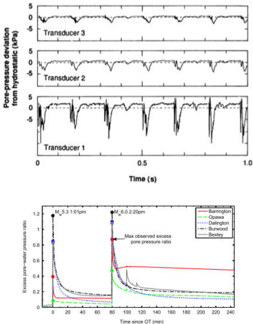
Figure 2.7: Time evolution of pore pressure from (a) laboratory test by Iverson (55), (b) realistic measurement of Christchurch earthquake (9).
