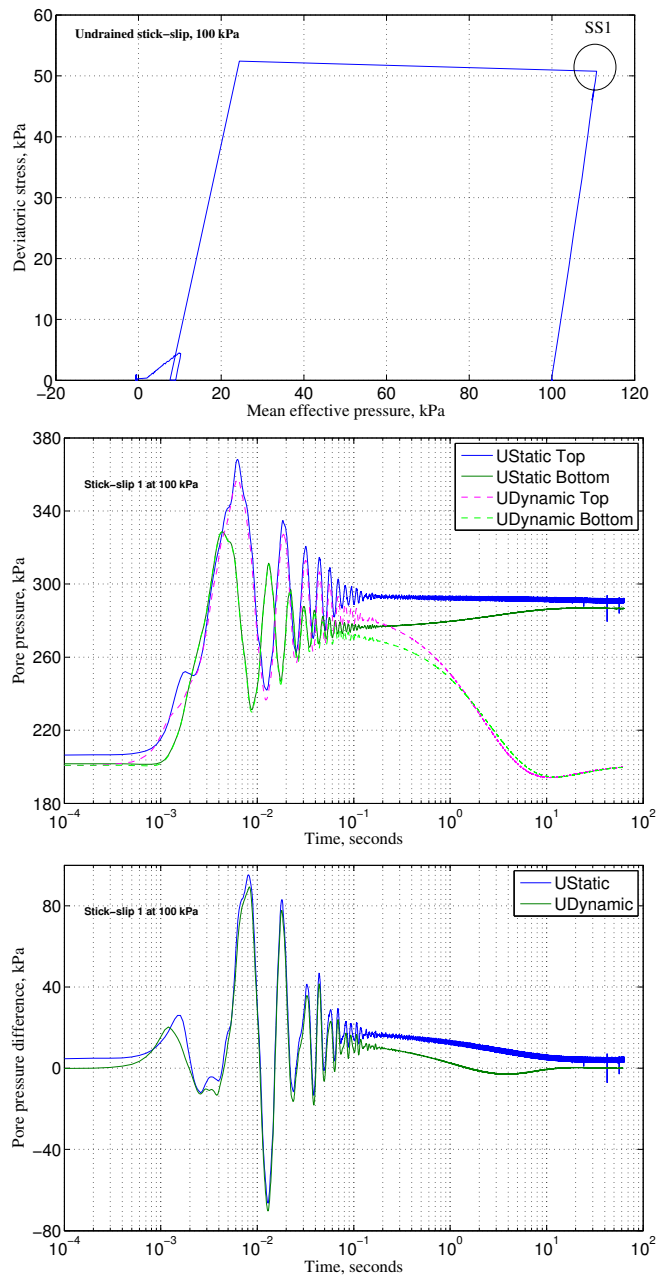
Fig. 12 (a) Effective stress path for undrained compression at 100 kPa of confining pressure, (b) temporal evolution of top and bottom dynamic and static pore pressures, (c) pore pressure difference between top and bottom of the first undrained stick-slip at 100 kPa on 0.7 mm CVP beads.
