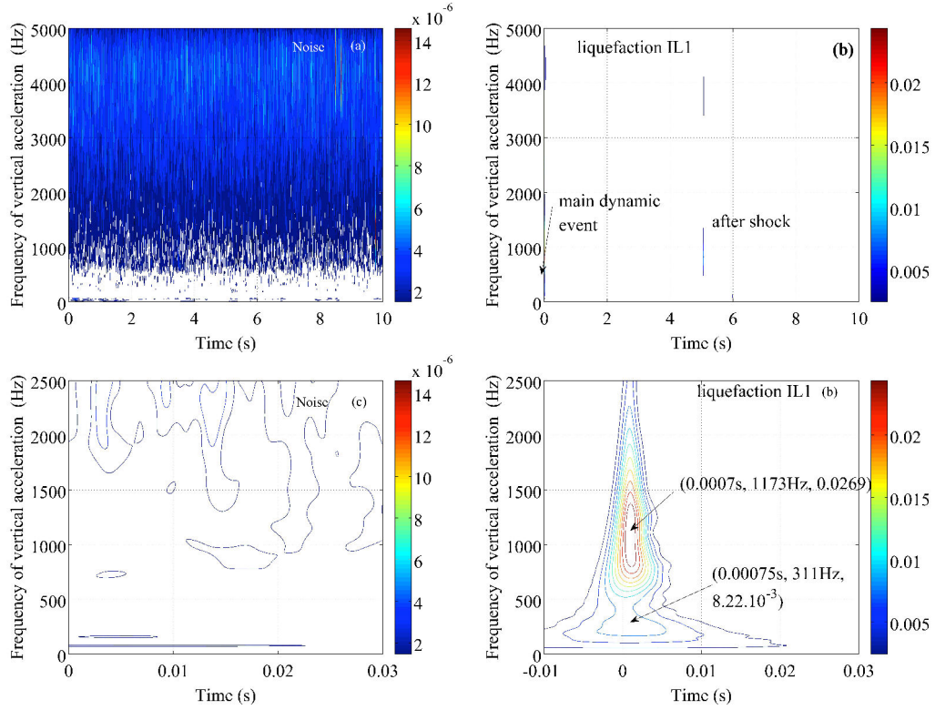
Figure 6.17: CCWT spectrum of vertical top cap acceleration G for noise signal (left) and isotropic liquefaction (right).
