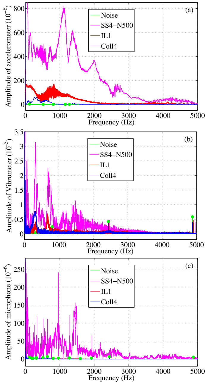
Figure 6.27: FFT spectra of collapse Coll 04 , liquefaction IL 01 , stick-slip SS 04 -test N500.
