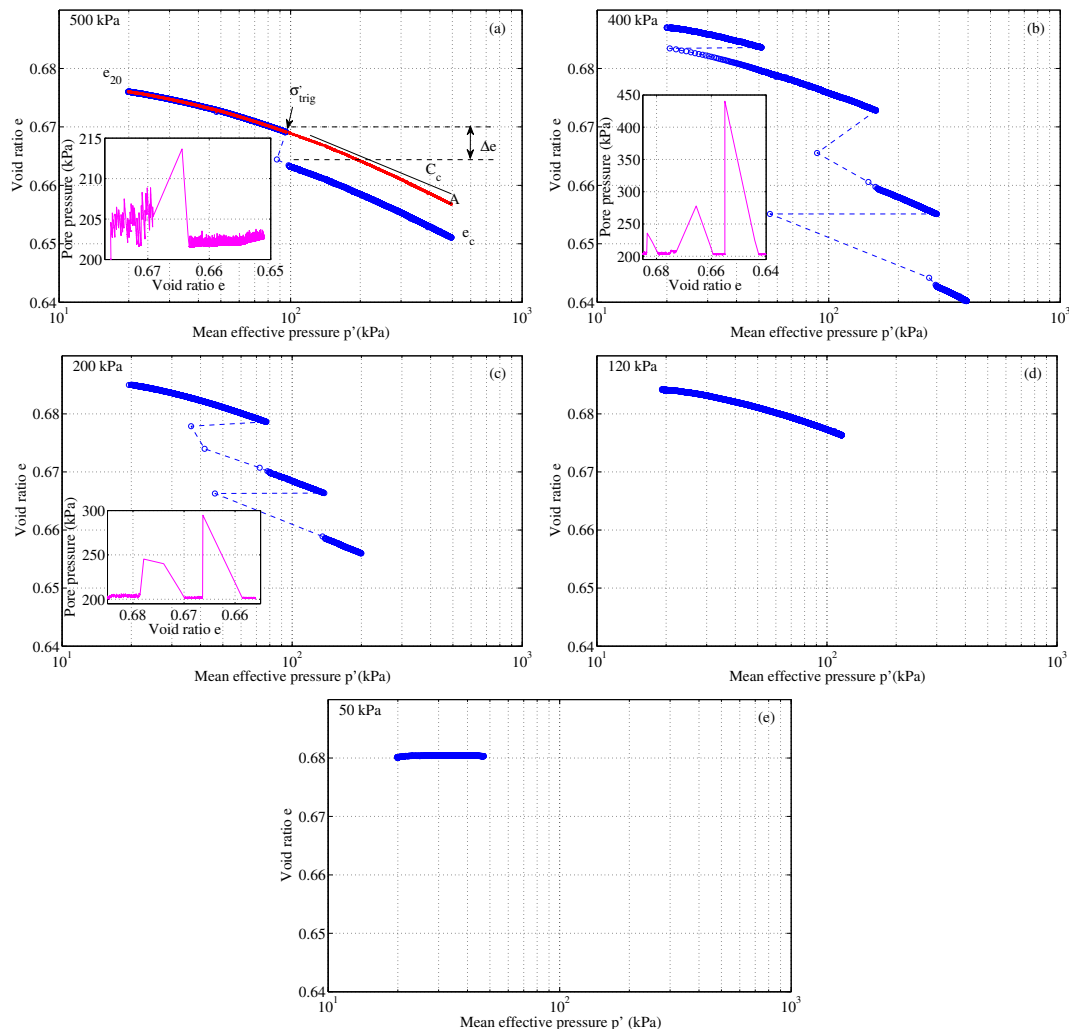
Figure 4.3: Global behaviour in isotropic consolidation phase to reach different effective confining pressure p'_0 from 50 up to 500 kPa.
