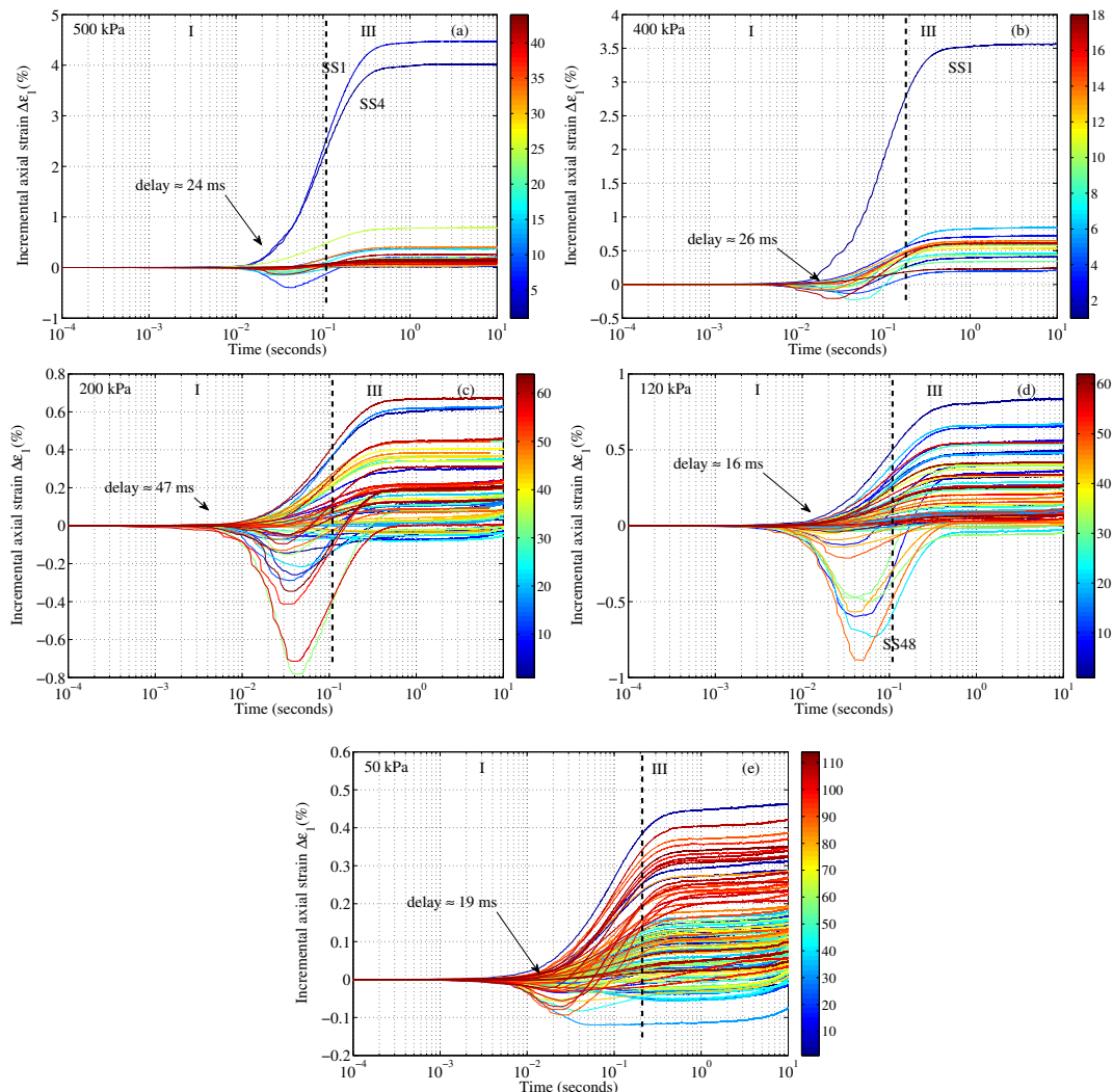
Figure 4.8: Time evolution of incremental axial strain \Delta\varepsilon_1 during stick-slip events at (a) 500 kPa of confining pressure, (b) 400 kPa, (c) 200 kPa, (d) 120 kPa and (e) 50 kPa.
