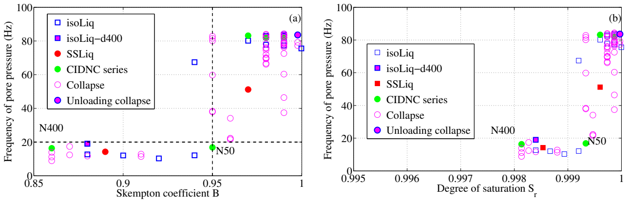
Figure 5.20: Impact of saturation of granular medium on the vibration frequency of pore pressure for all collapses and liquefaction events.
