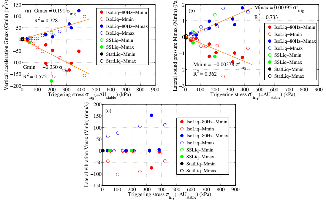
Figure 6.20: Relation of amplitude of vertical acceleration G , lateral sound pressure M , lateral vibration V and effective triggering stress \sigma'_{trig} (= \Delta U_{stable}) during liquefaction events.
