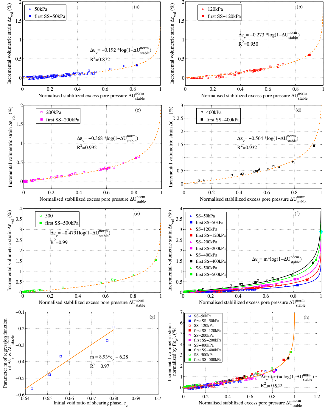
Figure 4.25: Normalised stabilised excess pore pressure \Delta U_{stable}^{norm} and incremental volumetric strain \Delta \varepsilon_{vol} incorporating with the effect void ratio e_c at the beginning of shearing.
