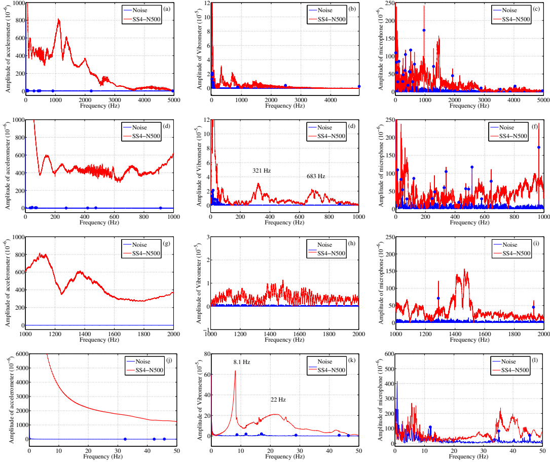
Figure D.2: Frequency analysis by FFT of vertical top cap acceleration G (left), lateral vibration V (middle), lateral sound pressure M (right) of stick-slip event SS_{04} of test N500 .
