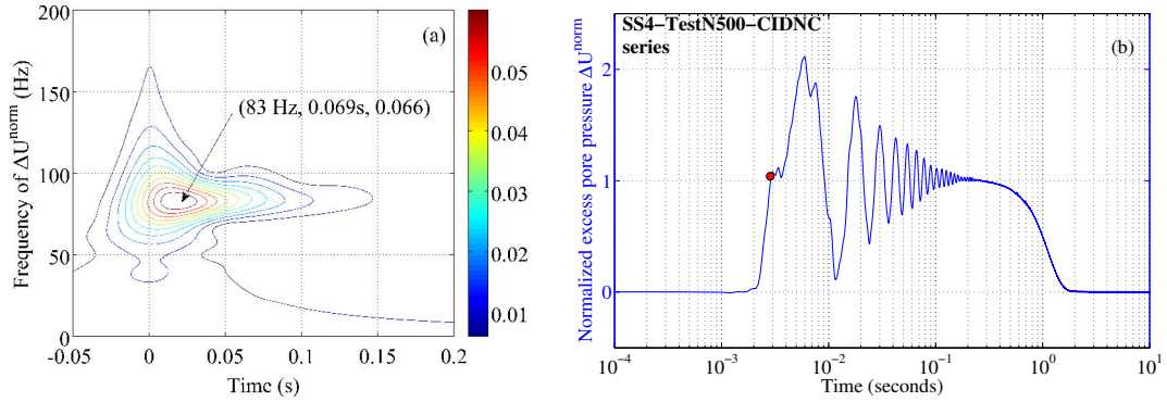
Figure D.7: CCWT spectrum of normalised excess pore pressure \Delta U^{norm} of stick-slip SS 04 of test N500.
