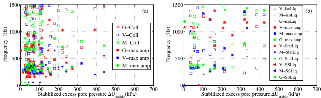
Figure 6.29: Characteristic frequencies of collapse and liquefaction identified by CCWT.
