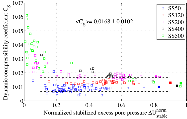
Figure 4.32: Compressibility of individual test in both isotropic and triaxial compression and relation between C_s and \Delta U_{stable}^{norm} .
