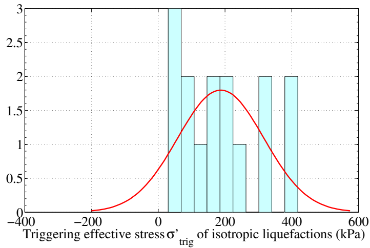
Figure C.1: Distribution of the triggering stress \sigma'_{trig} of liquefaction events
