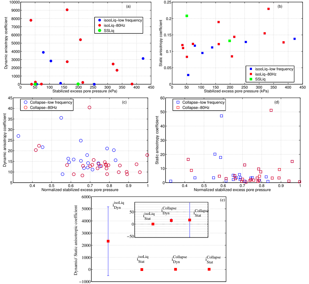
Figure 5.38: Dynamic and static anisotropy coefficients during liquefactions and collapses.
