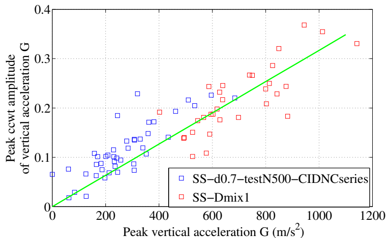
Figure 6.36: CCWT amplitude of vertical top cap acceleration between monodisperse material and binary mixture.
