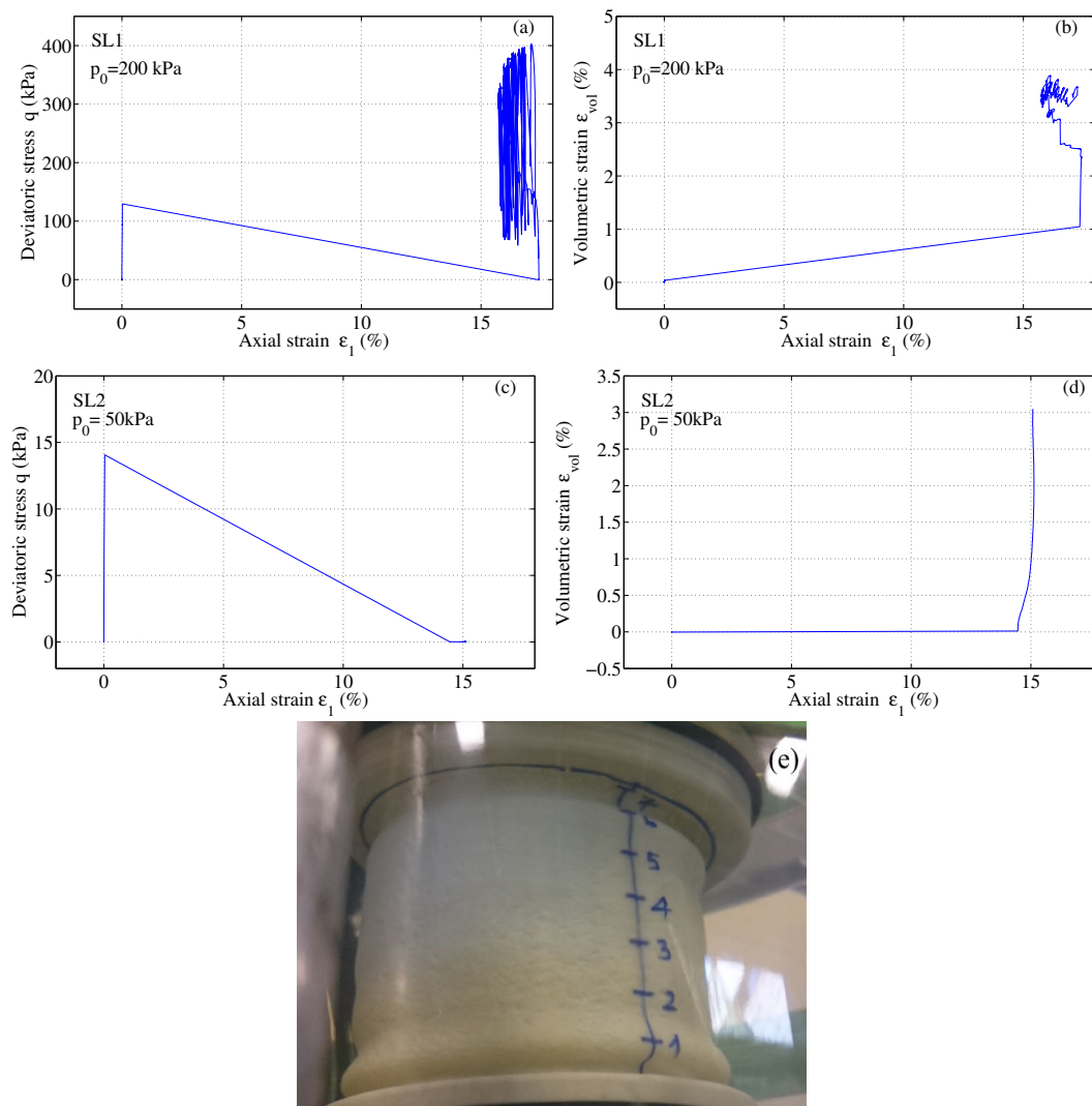
Figure 5.3: Global behaviour in stick-slip liquefaction: Stress-strain behaviour and volumetric strain behaviour of test SL_{01} at confining pressure p_0 = 200 kPa (a,b), test SL_{02} at p_0 = 50 kPa (c,d), illustration of the failure deformation after stick-slip liquefaction SL_{01} (e).
