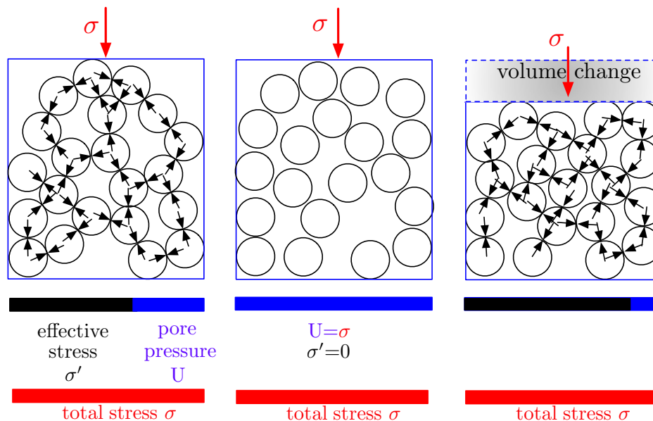
Figure 2.11: Schematic diagram of the stress composition of saturated medium including two phases, solid and liquid.
