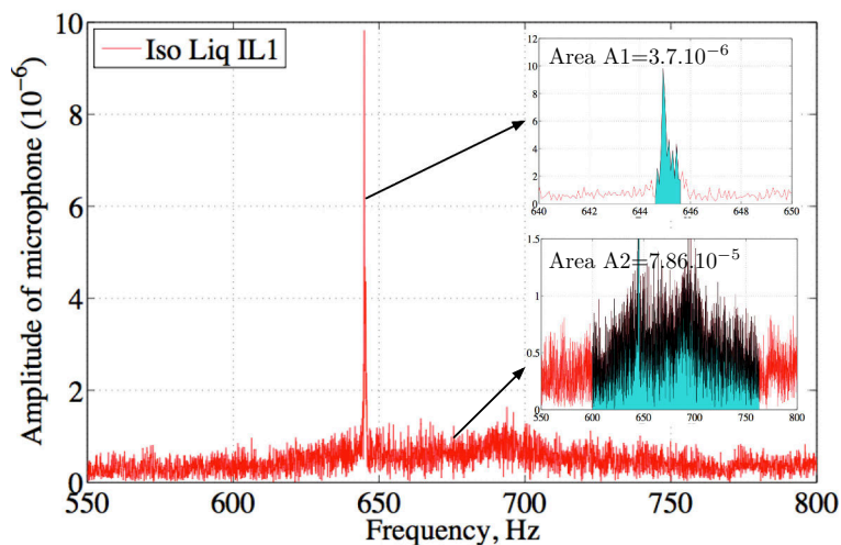
Figure 6.16: Approximate estimation of CCWT spectrum of microphone M for spike frequency and round frequency during isotropic liquefaction IL_{01} .
