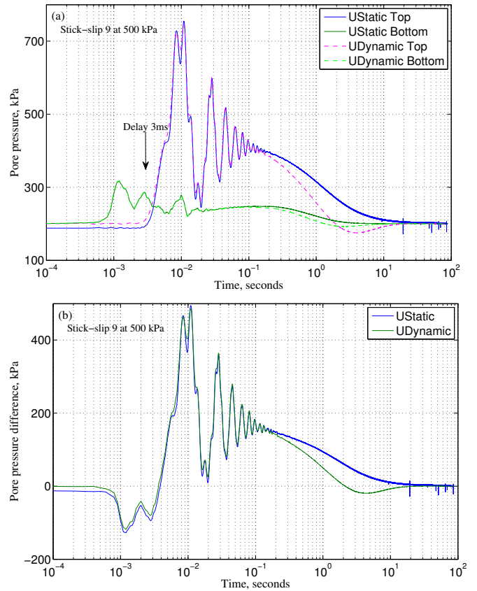
Fig. 6 (a) Temporal evolution of top and bottom dynamic and static pore pressures, (b) pore pressure difference between top and bottom of stick-slip SS9 at 500 kPa of confining pressure on 0.7 mm CVP beads.
