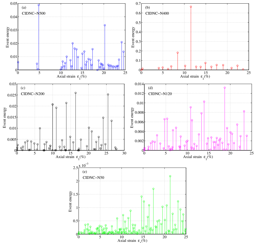
Figure 6.32: Energy release in each stick-slip event estimated for CIDNC series.
