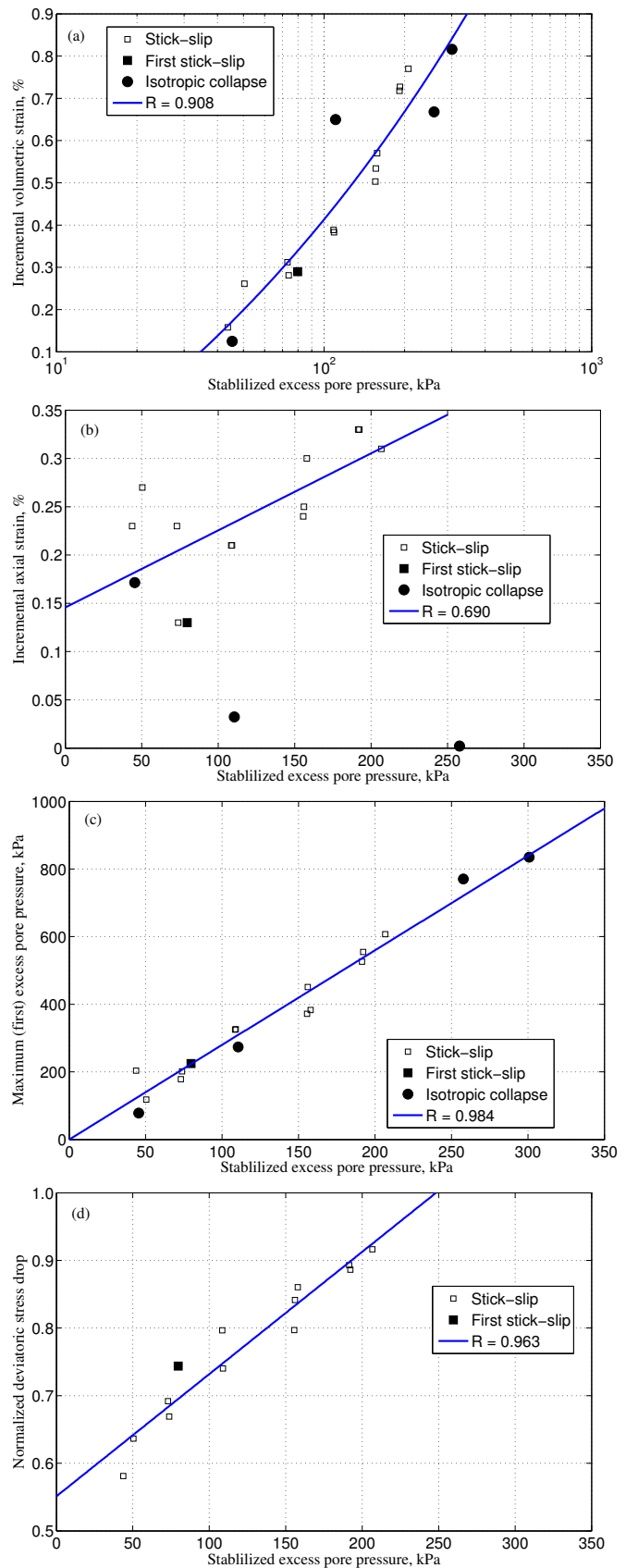
Fig. 9 Effects of dynamic stabilized excess pore pressure on (a) incremental volumetric strain \Delta \epsilon_v , (b) incremental axial strain \Delta \epsilon_a , (c) dynamic excess pore pressure peak \Delta U_{top}^{peak} and (d) normalised deviatoric stress \Delta q^{norm} .
