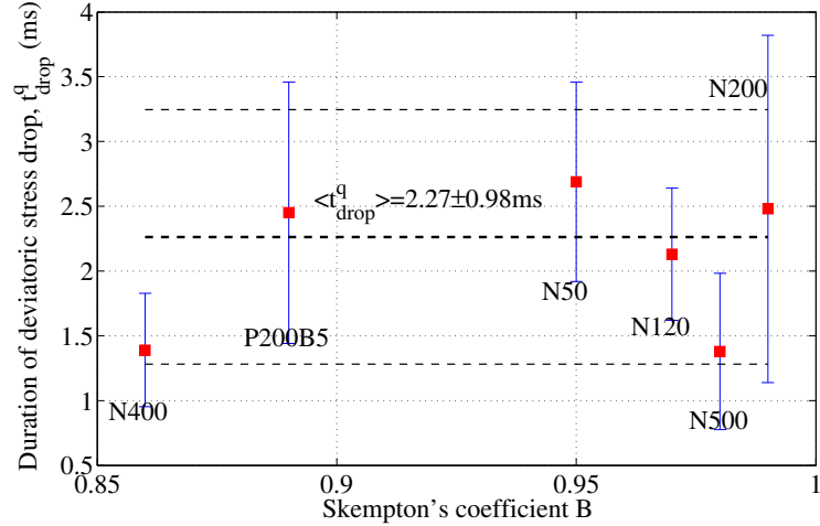
Figure 4.20: Duration of deviatoric stress drop t_{drop}^q in relevance with Skempton's coefficient B.
