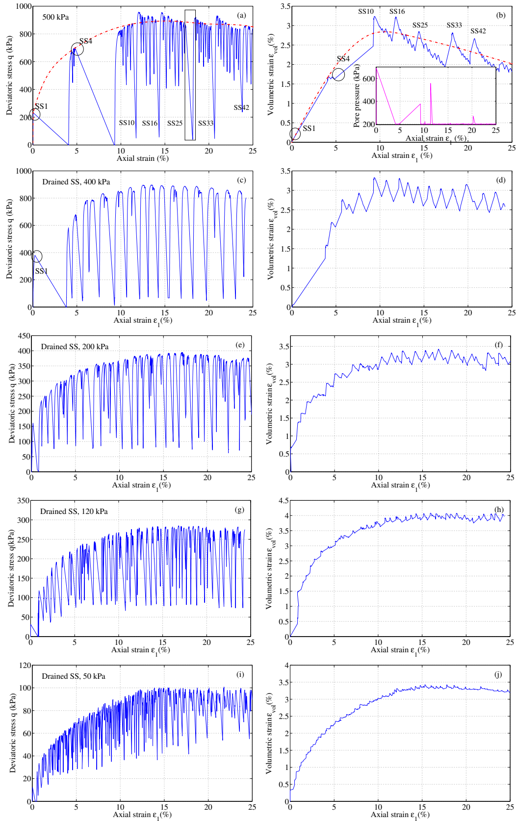
Figure 4.4: Global drained compression stick-slip behaviour in drained shearing phase at different confining pressure p'_0 .
