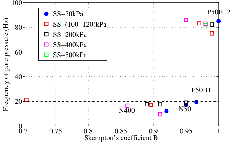
Figure 4.14: Variation of frequency of pore pressure in relevance to Skempton's coefficient B.
