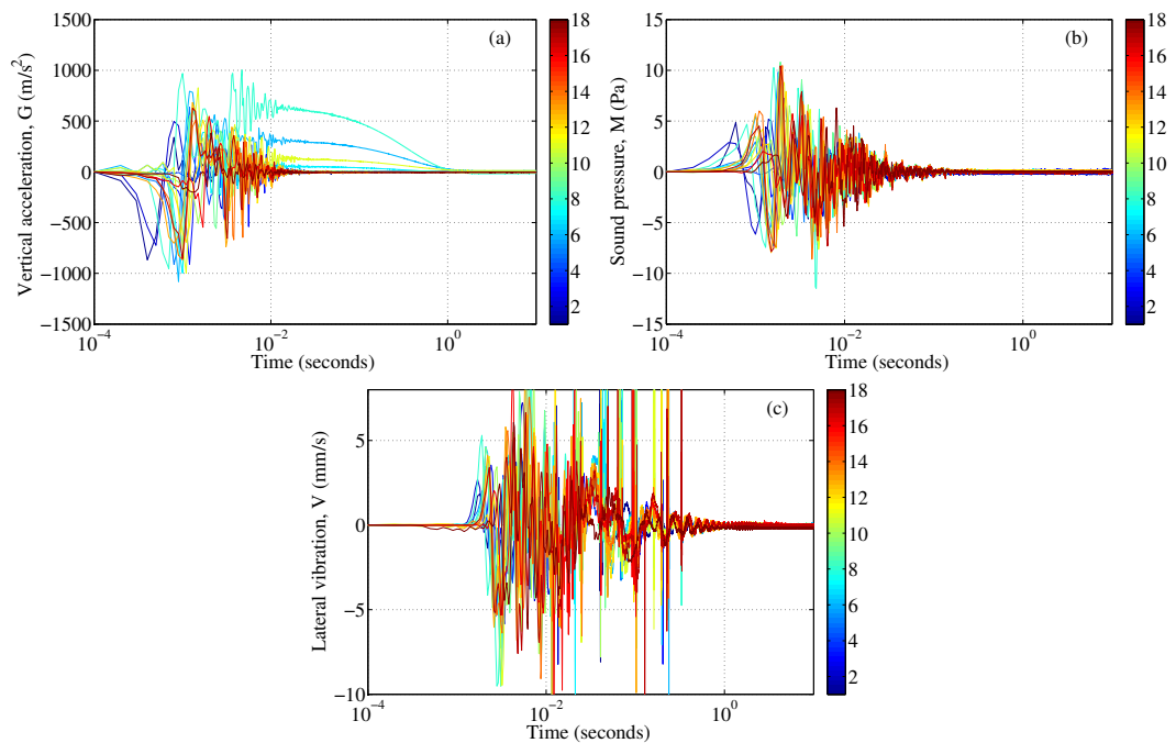
Figure 6.8: Detailed temporal evolution of G , M , V measurements of stick-slips at confining pressure of 400 kPa.
