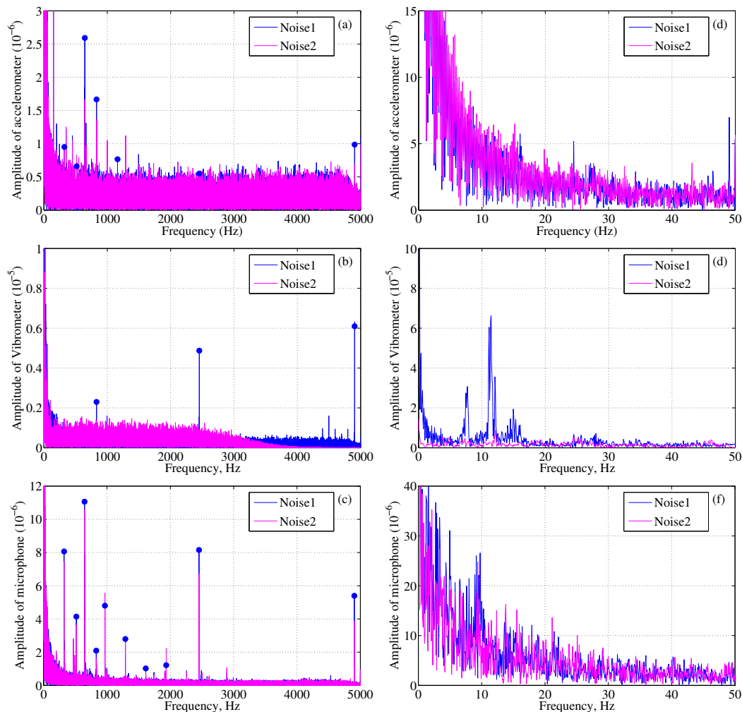
Figure D.1: Frequency analysis by FFT of two portions of noise from vertical top cap acceleration G , lateral vibration V , lateral sound pressure M within test IL_{01} .
