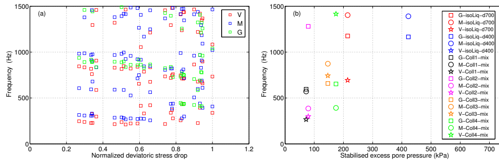
Figure 6.35: Characteristic frequency of stick-slip event for a binary mixture of 0.7mm and 0.4 mm at p_0 = 500 kPa.
