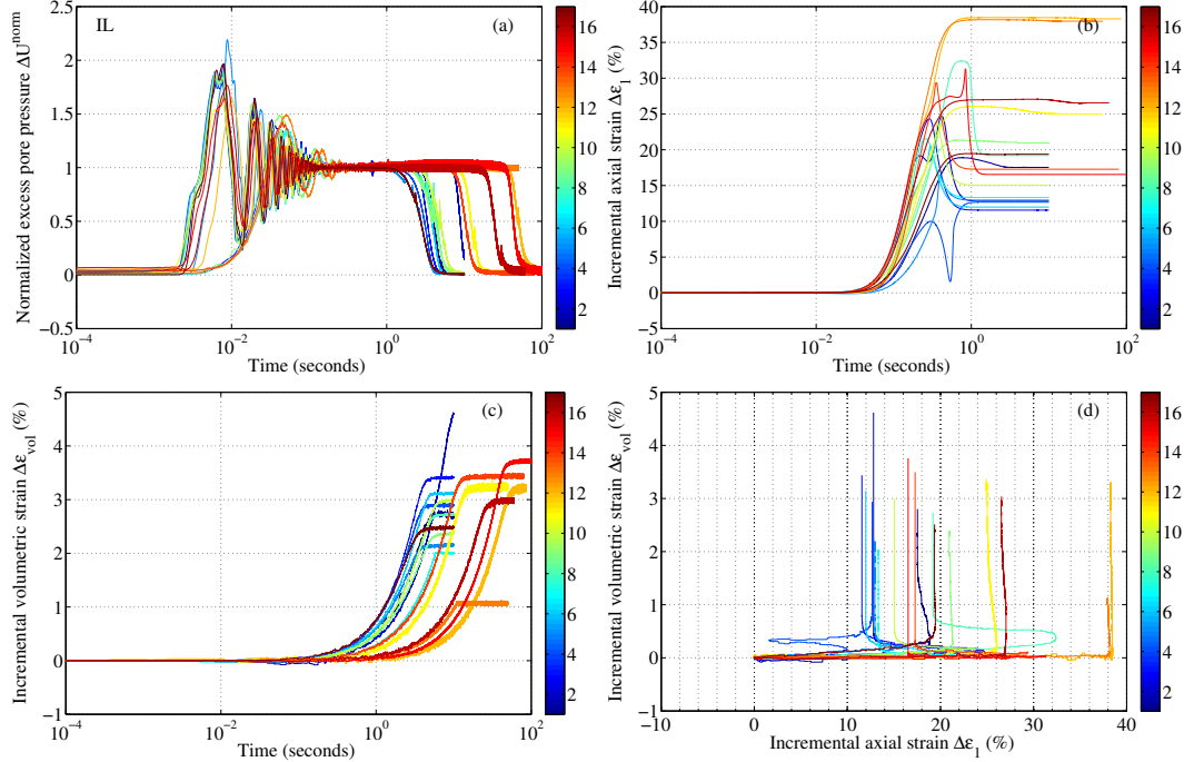
Figure 5.8: Detailed behaviour in isotropic liquefaction series.
