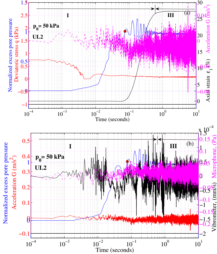
Figure 5.12: Detailed behaviour in static liquefaction event UL 02 at initial confining pressure of 50 kPa.
