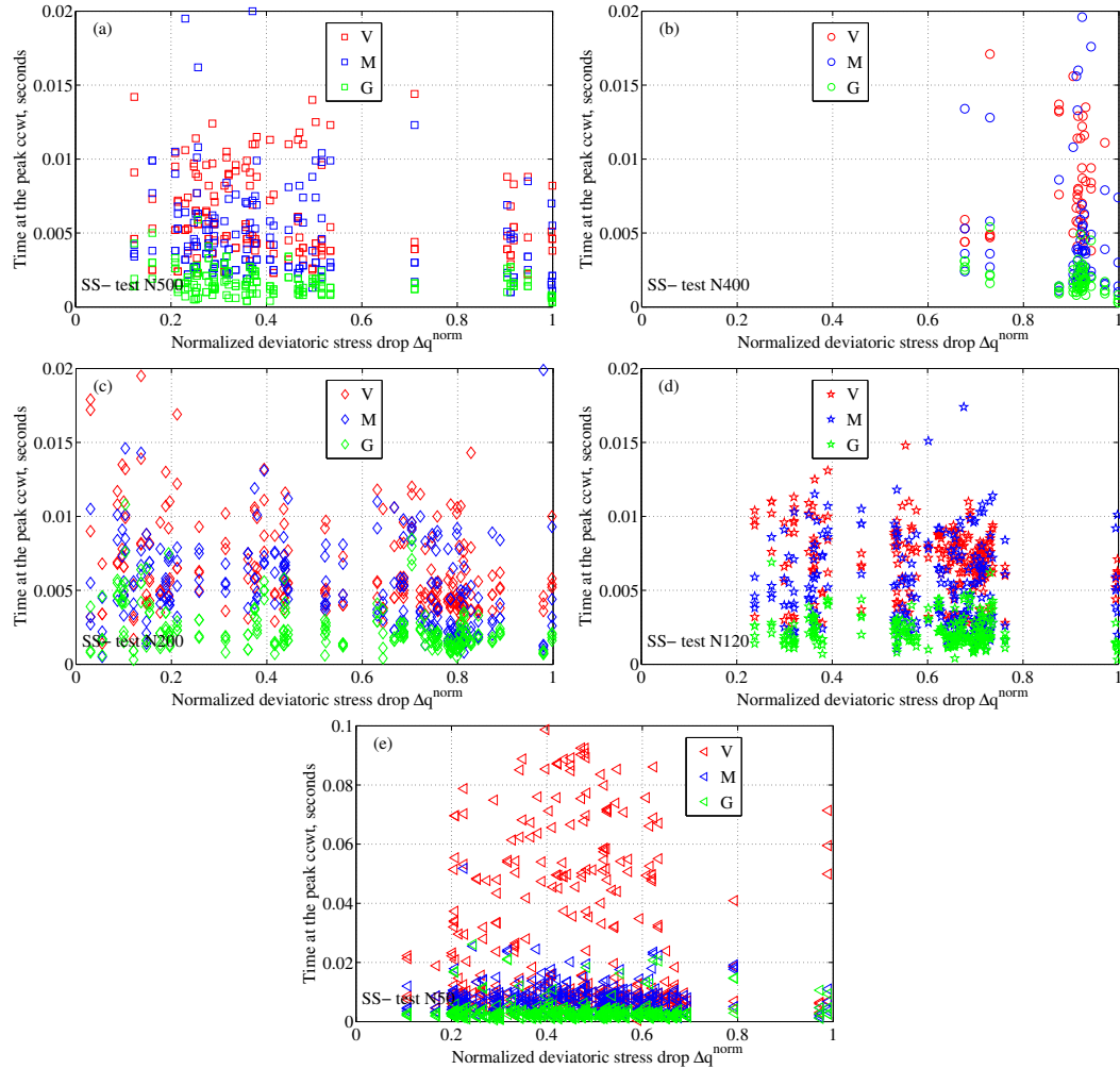
Figure 6.30: Time at the peak of CCWT amplitude of stick-slip events at different confining pressures(CIDNC series).
