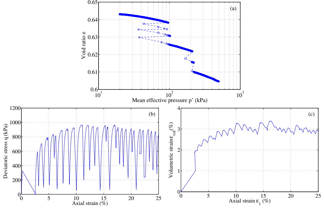
Figure 6.1: Global behaviour in (a) isotropic compression and drained shearing (b,c) of a binary mixture.
