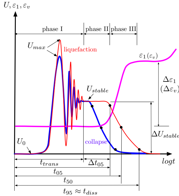
Figure 5.1: Schematic diagram of measurements within the study.
