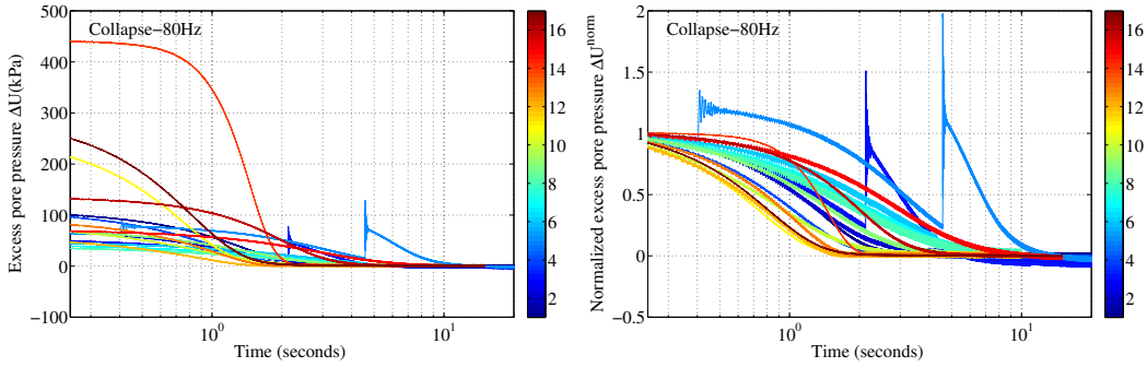
Figure 5.33: Evolution of excess pore pressure \Delta U in time within dissipation phase III.
