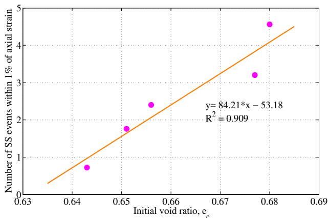
Figure 4.12: Effect of void ratio e_c and confining pressure p'_0 on the global behaviour of stick-slip.
