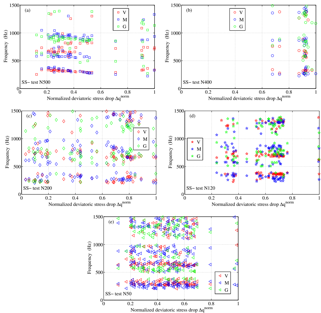
Figure 6.28: Characteristic frequencies of stick-slip event at different confining pressures identified by CCWT.
