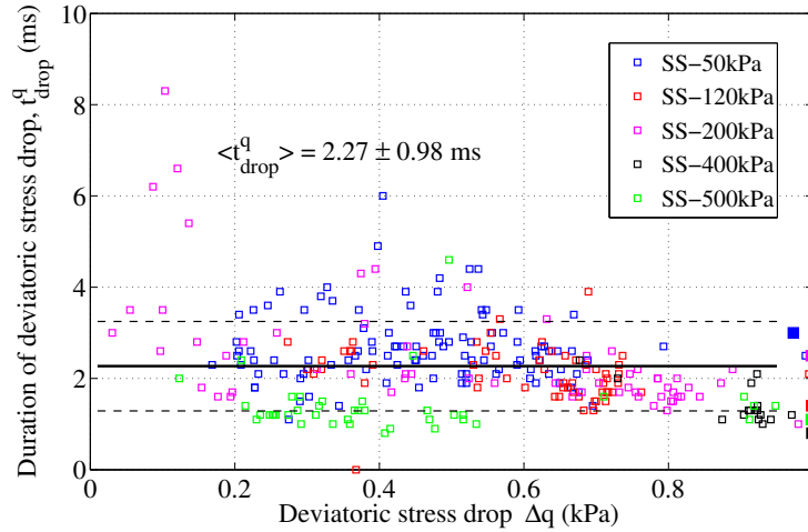
Figure 4.19: Duration of deviatoric stress drop t_{drop}^q in relevance with normalised deviatoric stress drop \Delta q^{norm} .
