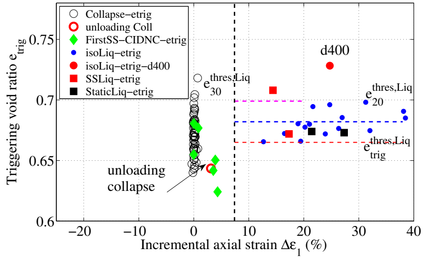
Figure 5.19: Location of triggering void ratio e_{trig} of studied liquefaction, collapse and large first stick-slip events in relation to incremental axial strain \Delta\varepsilon_1 .
