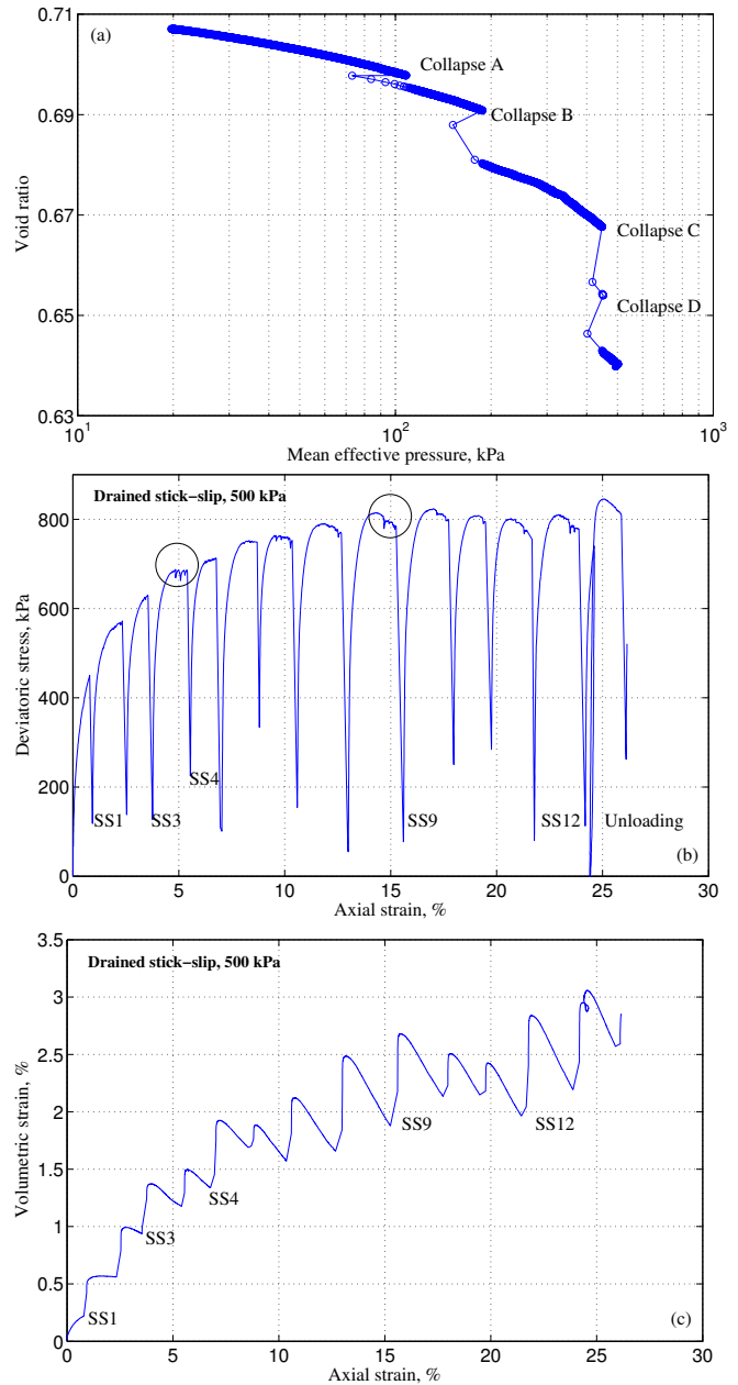
Fig. 3 (a) Isotropic instabilities from 20 to 500 kPa and (b) drained compression stick-slips with (c) coupled volumetric behaviour at 500 kPa of confining pressure on SLG 6-8 glass beads of 0.7 mm of diameter.
