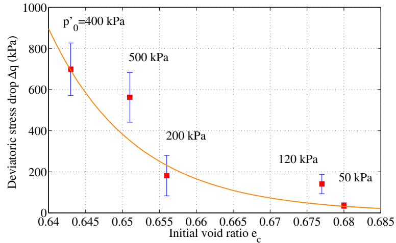
Figure 4.10: Effect of void ratio e_c at the beginning of shearing phase on the magnitude of deviatoric stress drop \Delta q .
