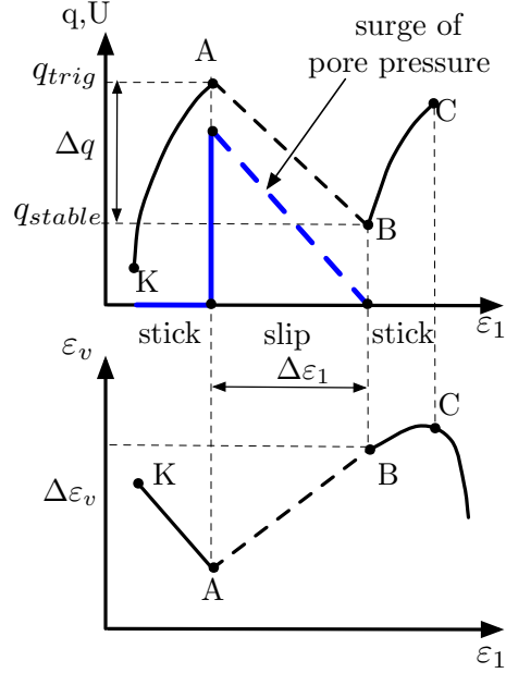
Figure 4.2: Definition of triaxial compression stick-slip event in schematic diagram.
