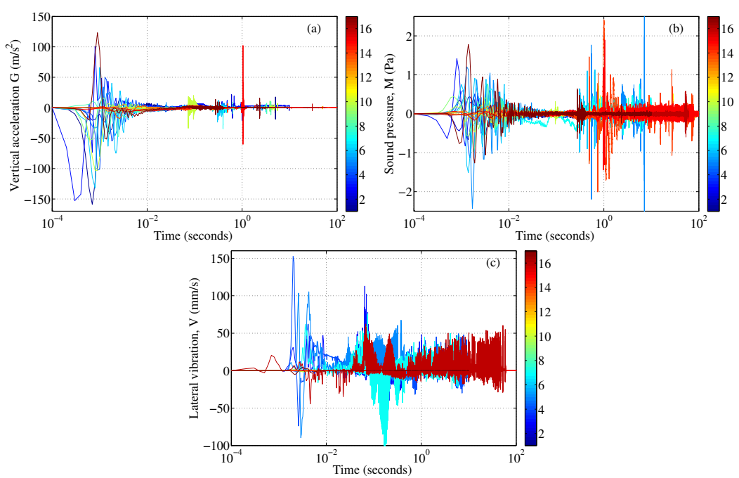
Figure 6.5: Detailed temporal evolution of G, M, V measurements of isotropic liquefaction series.
