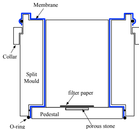
Figure 3.4: Accessories for sample fabrication
