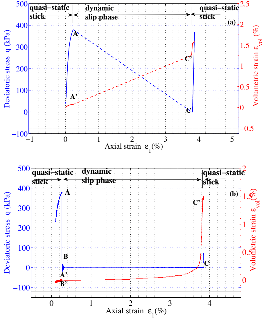
Figure 4.18: Typical stick-slip behaviour in drained triaxial compression at 400 kPa with stress-strain and volumetric strain behaviours acquiring of (a) 0.2 Hz and (b) 10 kHz.
