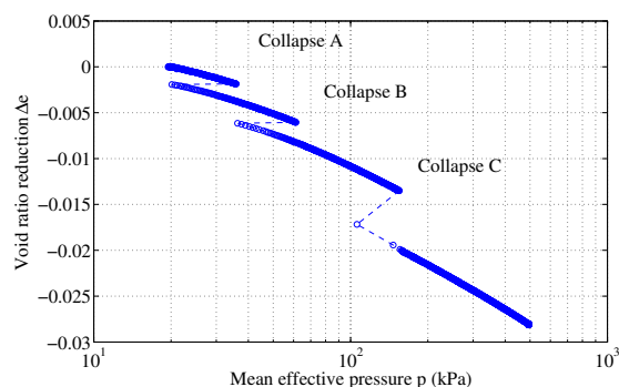
Figure 5.23: Compressibility behaviour during isotropic consolidation of slender sample H/D = 2 .
