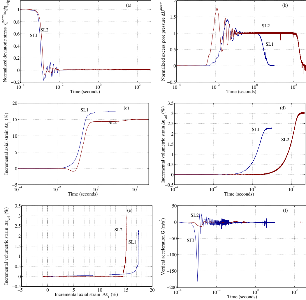
Figure 5.10: Detailed behaviour in drained stick-slip liquefaction events: (a) temporal evolution of normalised deviatoric stress q^{norm} , (b) normalised excess pore pressure \Delta U^{norm} , (c) incremental axial strain \Delta \varepsilon_1 , (d) incremental volumetric strain \Delta \varepsilon_{vol} and (e) evolution of \Delta \varepsilon_{vol} in accordance with \Delta \varepsilon_1 (e), (f) time history of vertical top cap acceleration.
