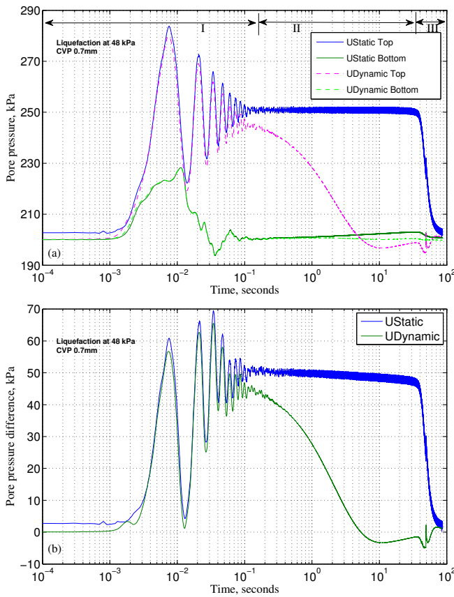
Fig. 11 (a) Temporal evolution of top and bottom dynamic and static pore pressures, (b) pore pressure difference between top and bottom of isotropic liquefaction at 48 kPa of confining pressure on 0.7 mm CVP beads.
