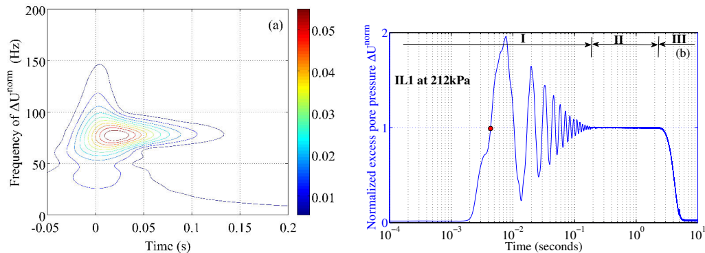
Figure 6.18: CCWT spectrum of normalised excess pore pressure \Delta U^{norm} during isotropic liquefaction IL_{01} .
