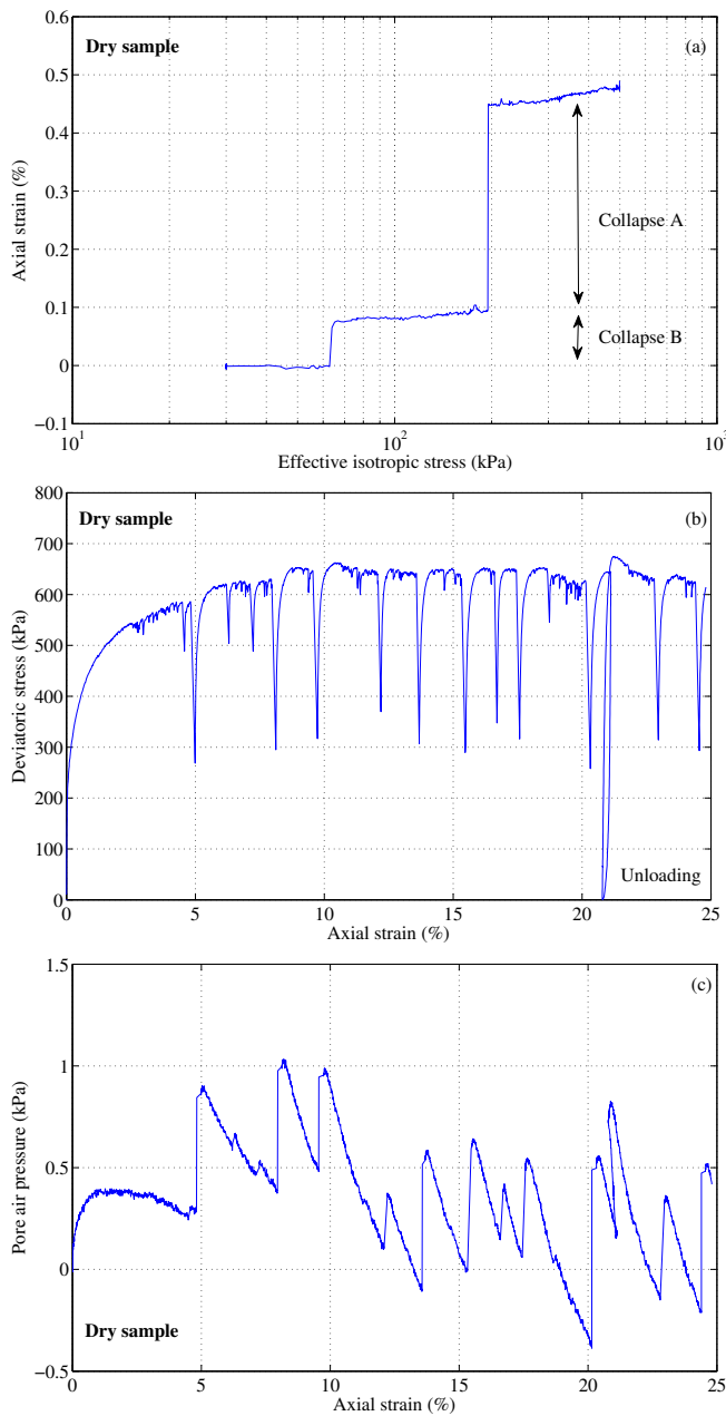
Fig. 13 (a) Isotropic consolidation with collapses at 62 and 197 kPa, (b) drained compression stick-slip behaviour with (c) pore air pressure at 500 kPa of confining pressure on dry medium dense specimen created by dry deposition method.
