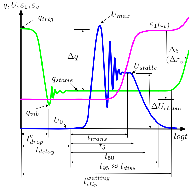
Figure 4.1: Schematic diagram of measurements of typical isotropic collapse and triaxial compression stick-slip.
