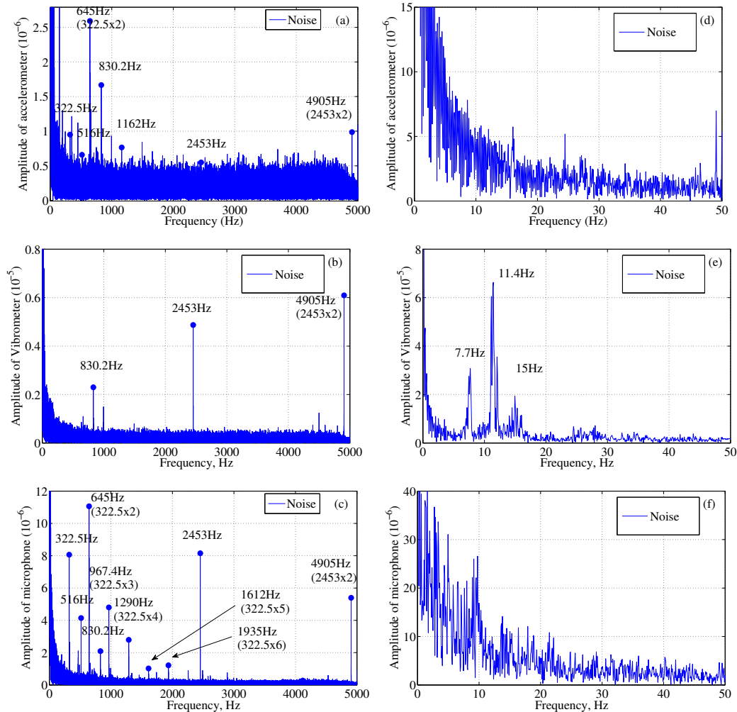
Figure 6.12: Frequency analysis by FFT of acceleration G (a,d), lateral vibration V (b,e), lateral sound pressure M (c,f) of the noise of 10 s prior to isotropic liquefaction event IL_{01} .
