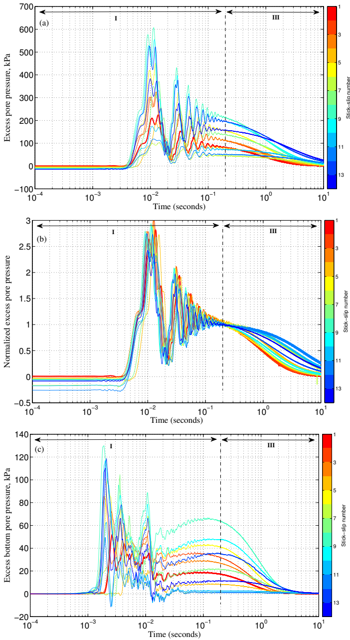
Fig. 7 Temporal evolution of (a) natural, (b) normalised static top and (c) natural bottom excess pore pressures of drained compression stick-slips at 500 kPa of confining pressure on 0.7 mm CVP beads. The stick-slip number is on the right colorbar.
