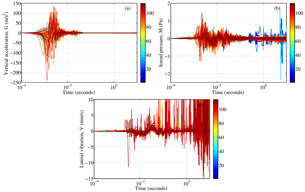
Figure 6.11: Detailed temporal evolution of G, M, V measurements of stick-slips at confining pressure of 50 kPa.
