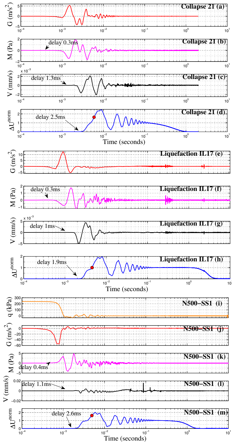
Figure 6.4: Detailed temporal evolution of vertical acceleration ( G ), lateral sound pressure ( M ), lateral vibration ( V ) and normalised excess pore pressure ( \Delta U^{norm} ) during an isotropic collapse Coll_{21} at triggering stress of 255.3 kPa (a to d), isotropic liquefaction IL_{17} at 383.9 kPa (e to h) and one large SS_{01} of test N500 at confining pressure of 500 kPa (i to m).
