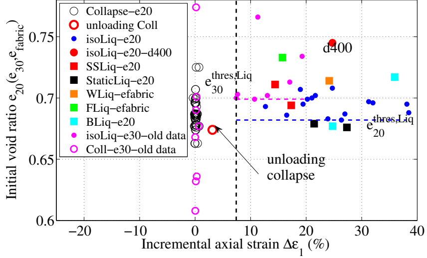
Figure 5.18: Location of initial void ratio e_{20} , e_{30} of studied liquefaction, collapse and large first stick-slip events in relation to incremental axial strain \Delta\varepsilon_1 .
