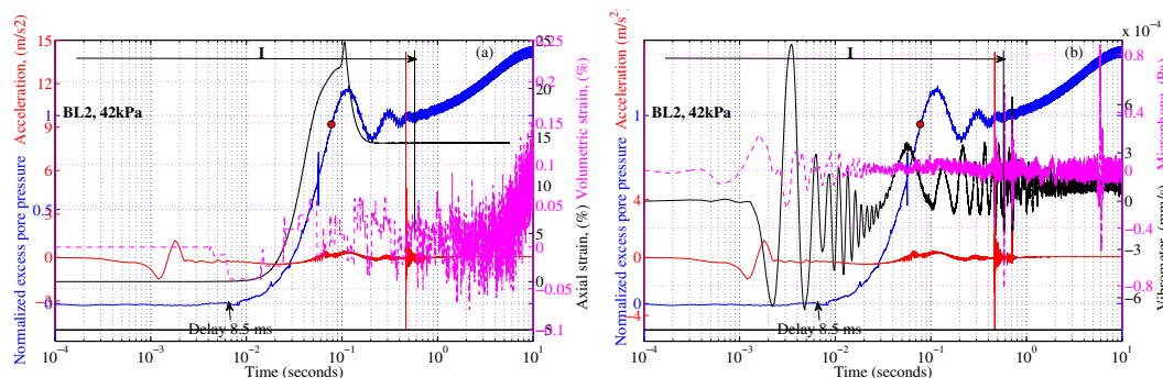
Figure 5.14: Detailed behaviour in liquefaction event BL 02 at effective confining pressure of 42 kPa during application of back pressure.
