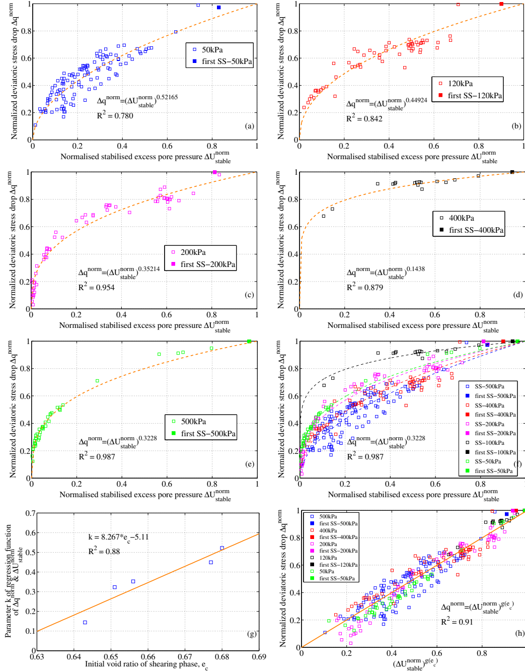
Figure 4.27: Relation of normalised stabilised excess pore pressure \Delta U_{stable}^{norm} and normalised deviatoric stress drop \Delta q^{norm} incorporated with the effect of void ratio e_c .
