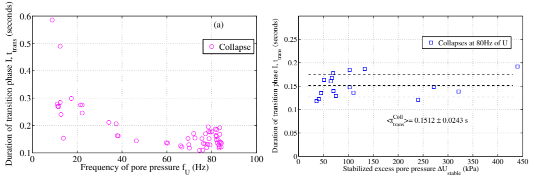
Figure 5.31: Time characteristics of phase I during collapse events.
