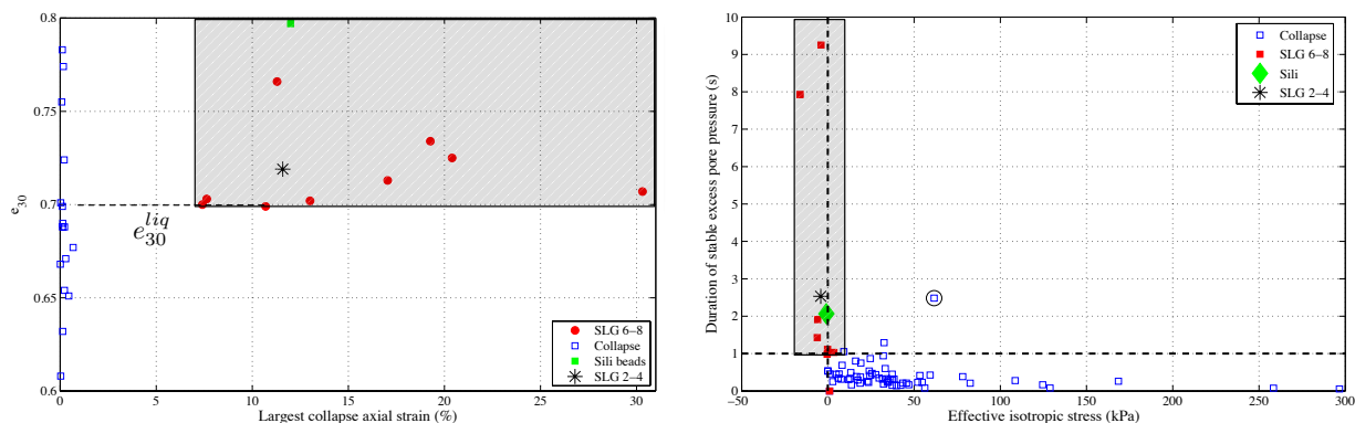
Figure 2.13: Conditions for isotropic liquefaction (left) Void ratio threshold, (right) Duration of stabilised excess pore pressure (31).
