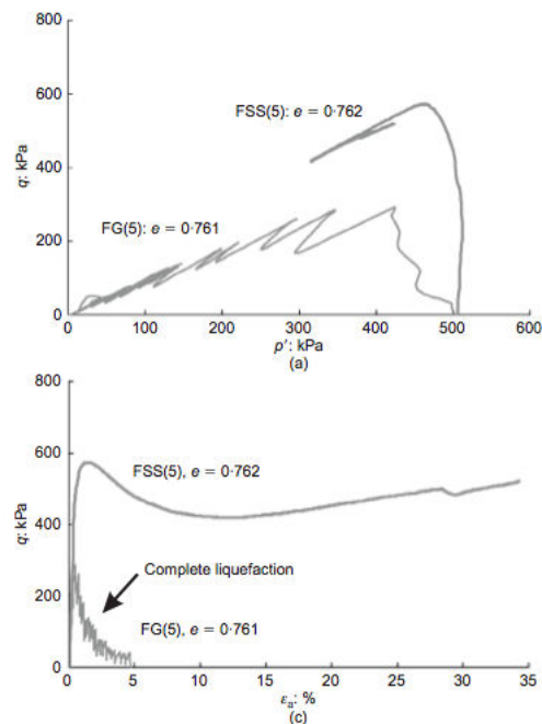
Figure 2.9: Undrained triaxial shear behaviour of Fujian sand modified by addition of 1.7 mm beads (126).
