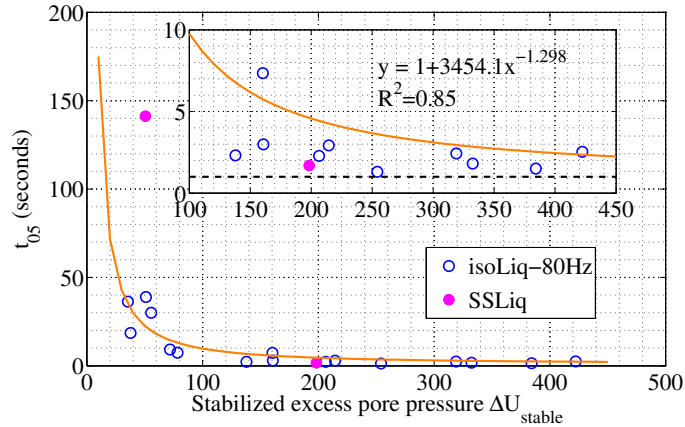
Figure 5.29: Evolution of the stabilised phase according to \Delta U_{stable} during isotropic liquefaction events.
