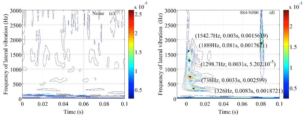
Figure D.4: CCWT spectrum of lateral vibration V for noise signal (left) and stick-slip SS 04 of test N500 (right).
