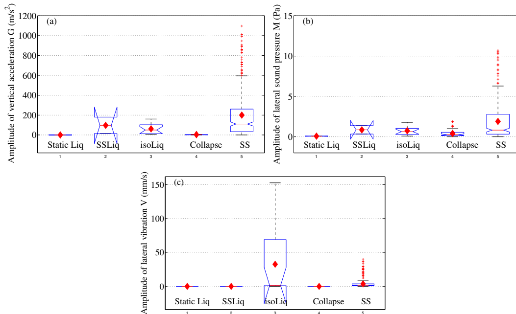
Figure 6.23: Amplitude of G, M, V in various kinds of instability events.
