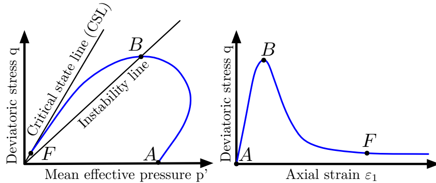
Figure 5.4: Static liquefaction of soil in the literature.
