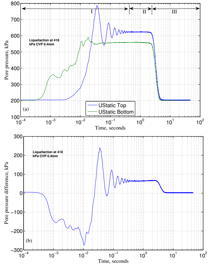
Fig. 10 (a) Temporal evolution of top and bottom static pore pressures, (b) pore pressure difference between top and bottom of isotropic liquefaction at 418 kPa of confining pressure on 0.4 mm CVP beads.
