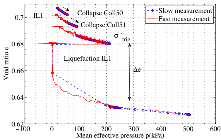
Figure C.2: Compressibility of isotropic liquefaction IL_{01} .
