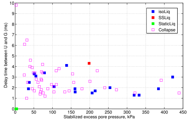
Figure 5.40: Time delay between acceleration G and excess pore pressure U of all kinds of liquefaction and collapse.
