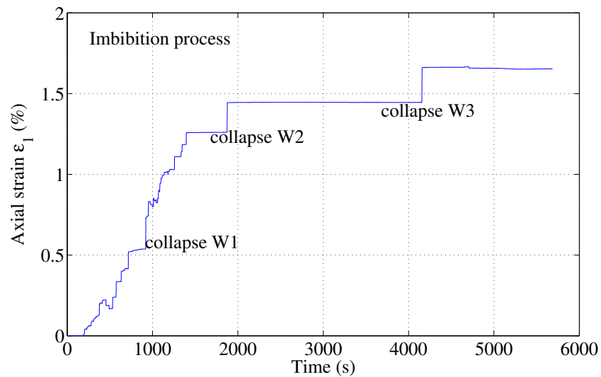
Figure A.1: Temporal evolution of axial strain during imbibition process.
