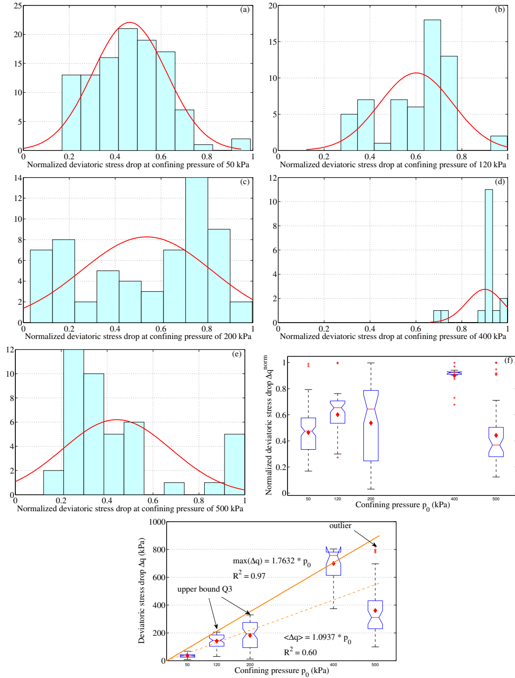
Figure B.1: Statistical estimation of the normalised deviatoric stress drop \Delta q^{norm} and \Delta q of major stick-slip events in accordance with effective confining pressure p'_0 .
