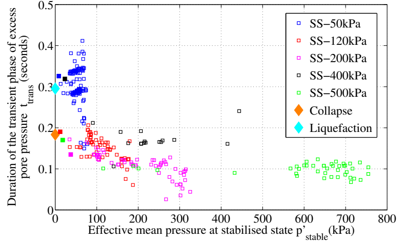
Figure 4.22: Relation between duration of the first transient phase of U , t_{trans} , and stabilised effective mean pressure p'_{stable} .
