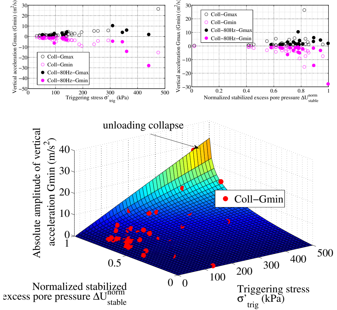
Figure 6.22: Relation of amplitude of G as a function of triggering stress \sigma_{trig} and normalised stabilised excess pore pressure \Delta U_{stable}^{norm} during collapse events.
