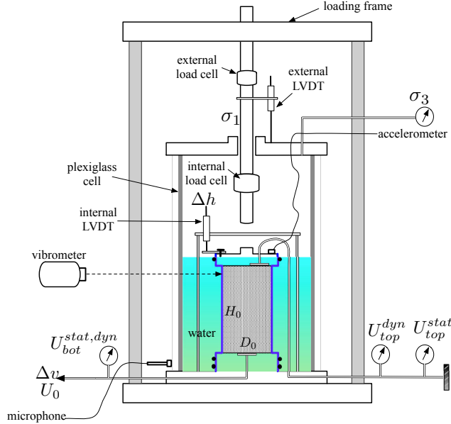
Figure 3.3: Scheme of the triaxial test apparatus
