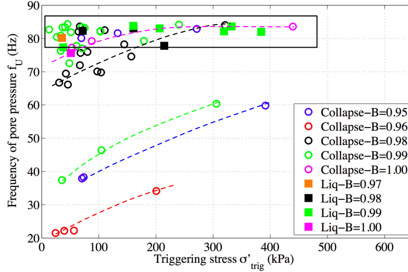
Figure 5.21: Impact of triggering stress \sigma'_{trig} of granular medium on the vibration frequency of pore pressure for all collapses and isotropic liquefaction events.
