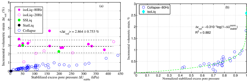
Figure 5.36: Incremental volumetric strain and stabilised excess pore pressure of liquefaction and collapse.
