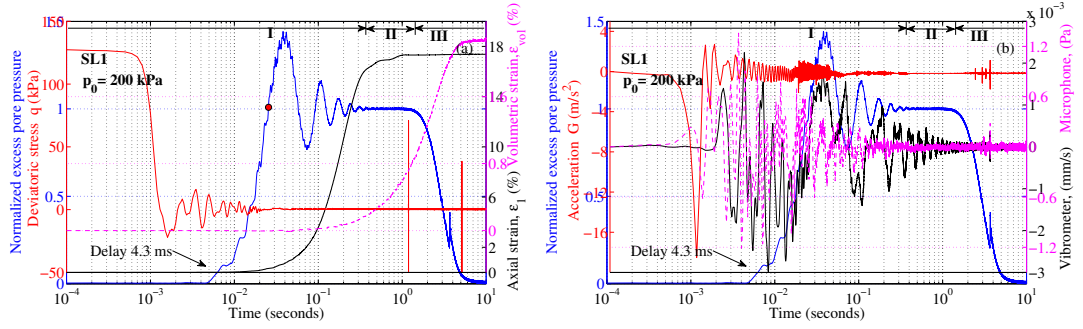
Figure 5.9: Detailed behaviour in drained stick-slip liquefaction event SL_{01} at confining pressure of 200 kPa.
