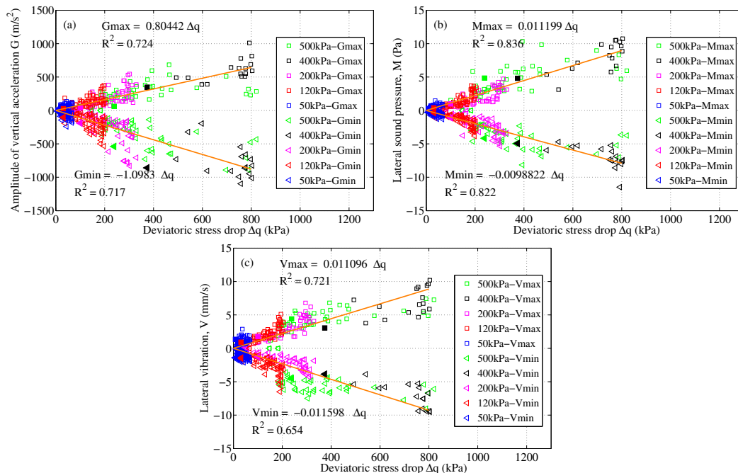
Figure 6.19: Relation of amplitude of vertical acceleration G , lateral sound pressure M , lateral vibration V and deviatoric stress drop \Delta q during stick-slip events.
