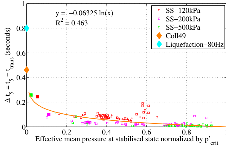
Figure 4.24: Duration between phase I and phase III of pore pressure, \Delta t_{05} , in relevance with \frac{p'_{stable}}{p'_{crit}} .
