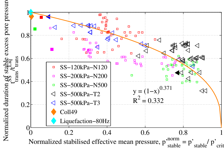
Figure 4.23: Relation between normalised duration of the first transient phase of U , t_{trans}^{norm} , and the normalised stabilised effective mean pressure p_{stable}^{norm} .
