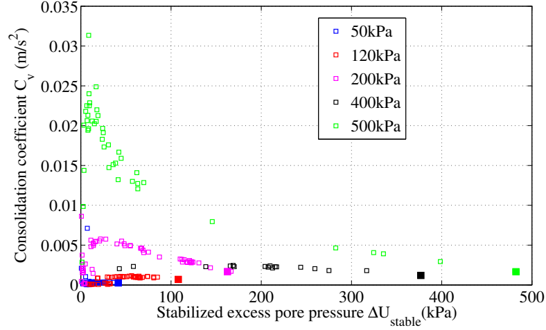
Figure 4.16: Consolidation coefficient C_v in relation to \Delta U_{stable}^{norm} .
