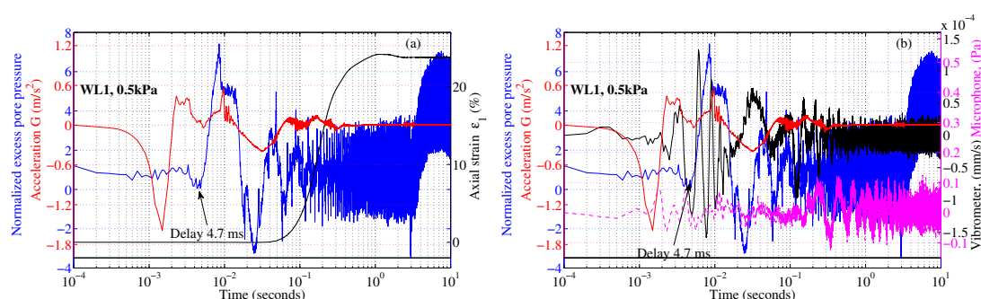
Figure 5.16: Detailed behaviour in liquefaction event during imbibition at effective triggering stress of 0.5 kPa.
