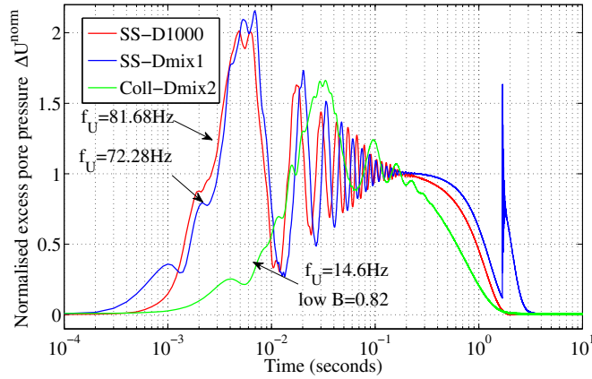
Figure 5.26: Temporal behaviour of pore pressure during instabilities within different assembly of various grain size.
