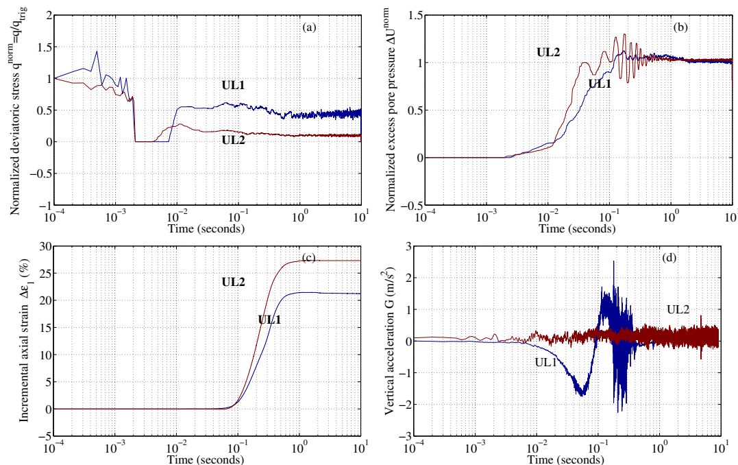
Figure 5.13: Detailed behaviour in static liquefaction events.
