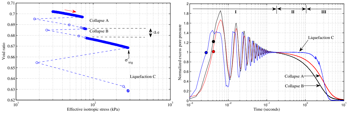
Figure 2.12: (left) Spontaneous instabilities under drained isotropic compression, (right) Time evolution of normalised pore pressure during isotropic collapse and isotropic liquefaction (31).
