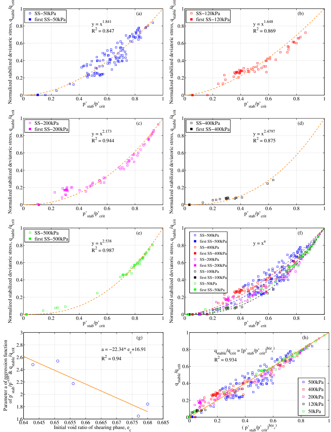
Figure 4.34: Boundary surface at different confining pressures p'_0 incorporated with the effect of void ratio e_c .
