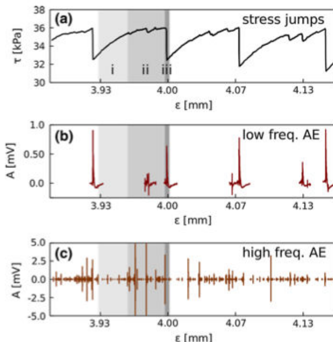
Figure 2.14: Stick-slip and acoustic measurements in direct shear stick-slip experiment of 4 mm beads under 60 kPa of confining pressure (81).
