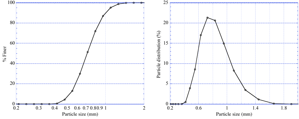
Figure 3.2: Gradation curve and grain size distribution of CVP glass beads
