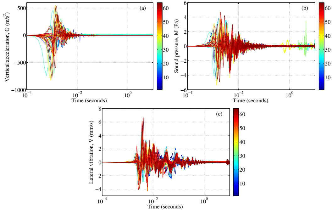
Figure 6.9: Detailed temporal evolution of G, M, V measurements of stick-slips at confining pressure of 200 kPa.
