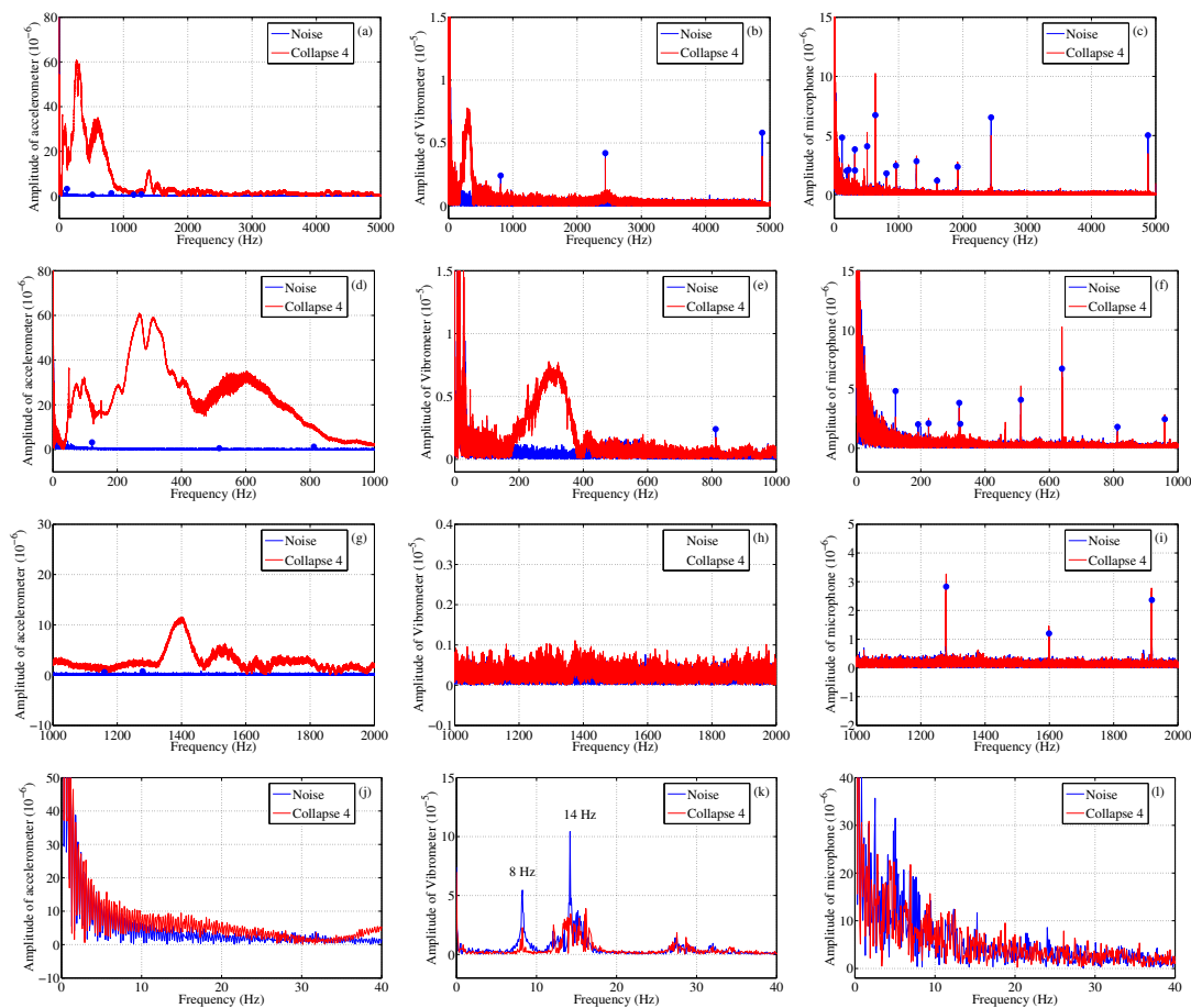
Figure D.8: Frequency analysis by FFT of vertical top cap acceleration G (left), lateral vibration V (middle), lateral sound pressure M (right) of collapse event \text{Coll}_{04} .
