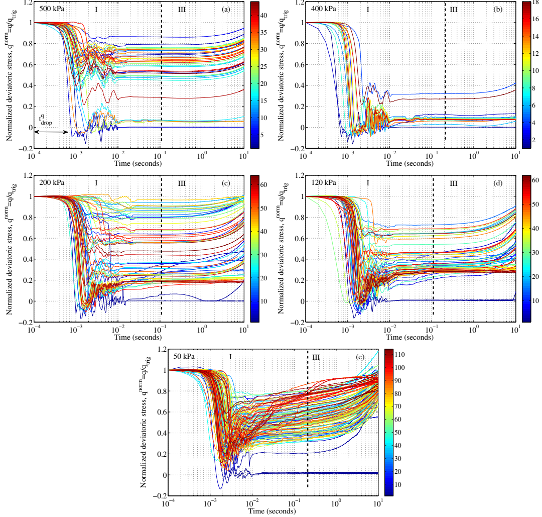
Figure 4.6: Time evolution of normalised deviatoric stress q^{norm} during stick-slip events at (a) 500 kPa of confining pressure, (b) 400 kPa, (c) 200 kPa, (d) 120 kPa and (e) 50 kPa.
