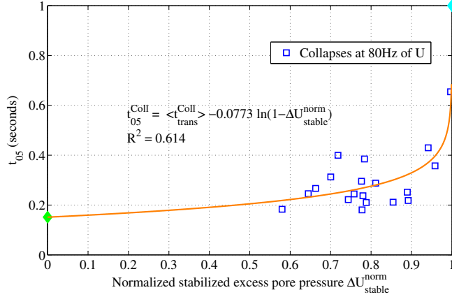
Figure 5.32: Time characteristics of phase II during collapse events.
