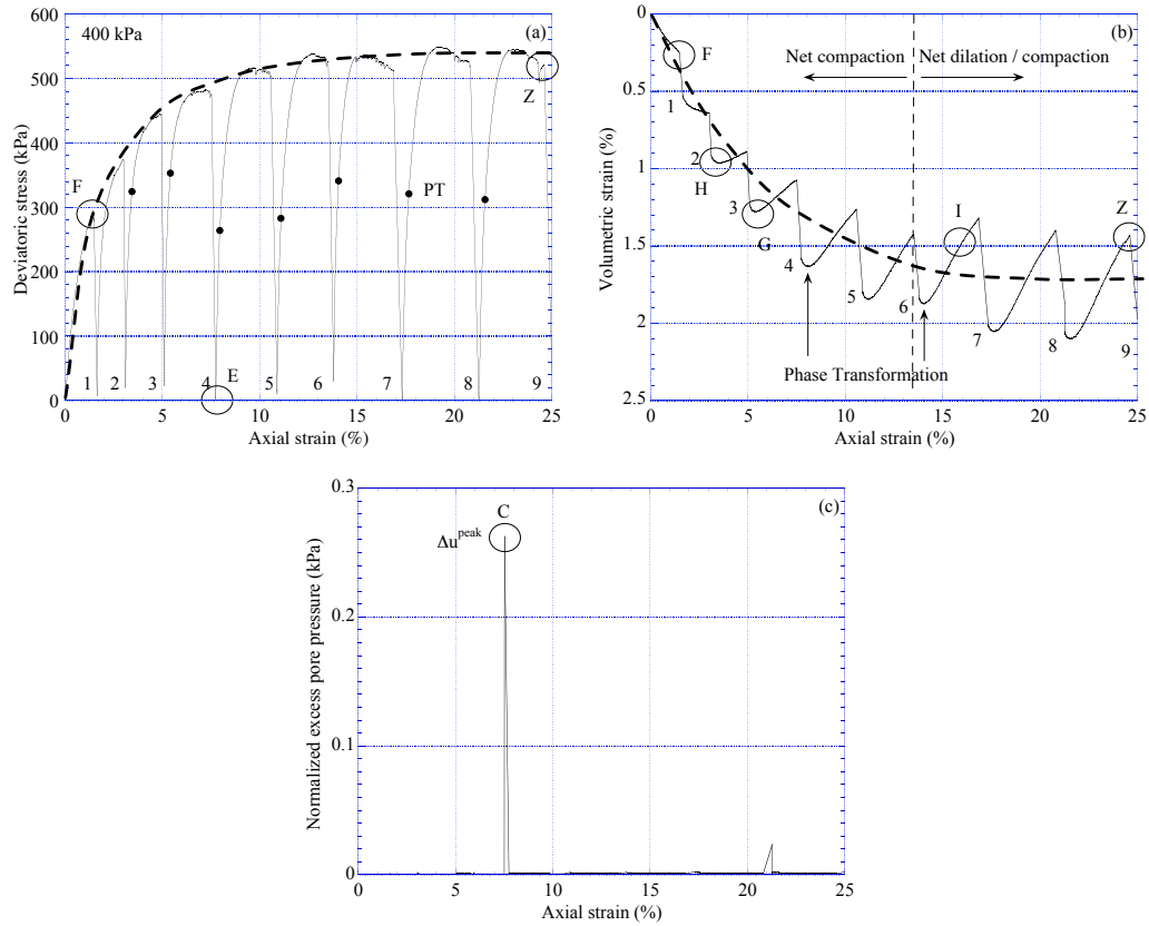
Figure 2.5: Stick-slip behaviour (stress-strain and volumetric) for 0.7 mm beads under 400 kPa of confining pressure (32).
