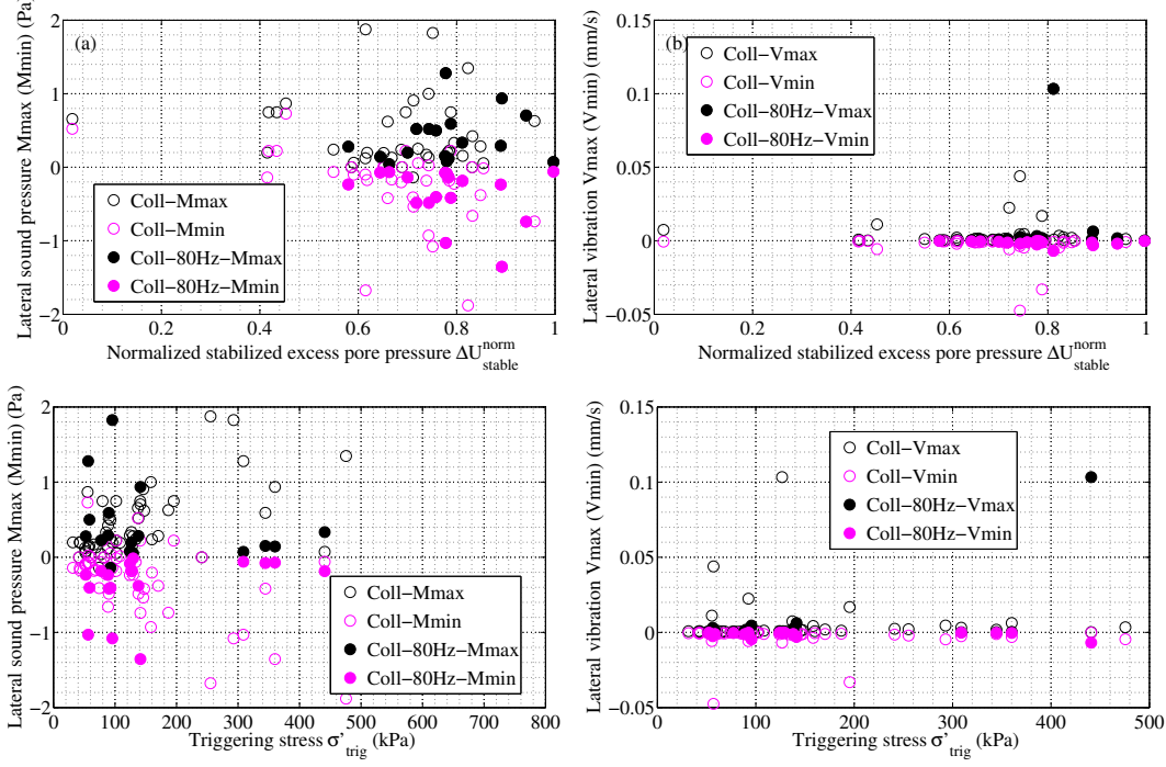
Figure 6.21: Relation of amplitude between lateral sound pressure M , lateral vibration V and normalised stabilised excess pore pressure \Delta U_{stable}^{norm} during collapse events (respectively in accordance with triggering stress \sigma'_{trig} ).
