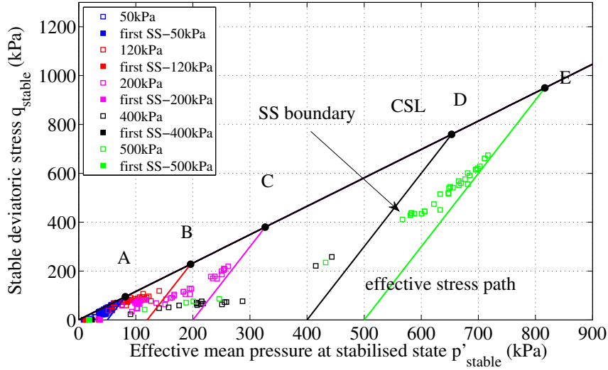
Figure 4.33: Behavior at stabilised stress state in (p' - q) plane.
