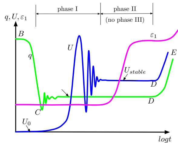
Figure 5.6: Scheme of the time evolution of deviatoric stress q , pore pressure U and axial \epsilon_1 during undrained stick-slip.
