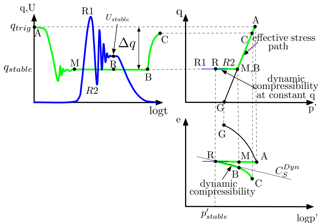
Figure 4.31: Description of stress path and dynamic consolidation of a stick-slip event on q - p' plane.
