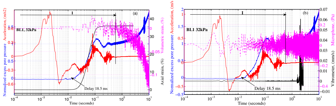
Figure 5.15: Detailed behaviour in liquefaction event BL 01 at effective confining pressure of 32 kPa during application of back pressure.
