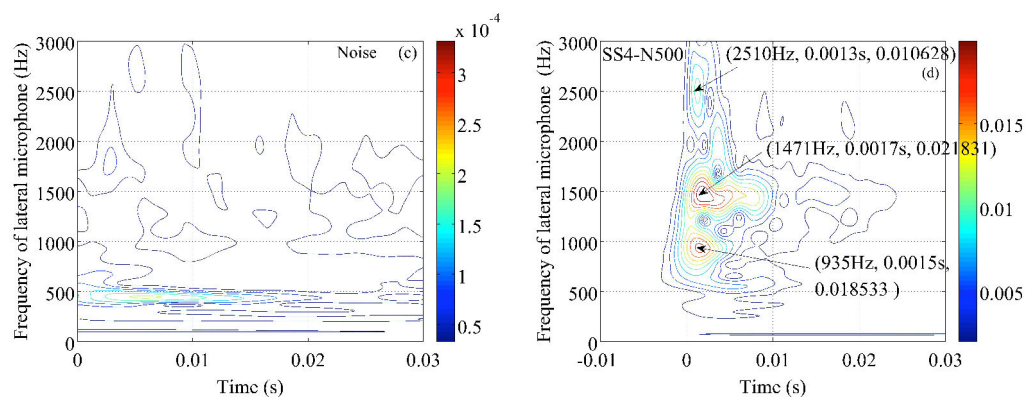
Figure D.5: CCWT spectrum of lateral sound pressure M for noise signal (left) and stick-slip SS_{04} of test N500 (right).
