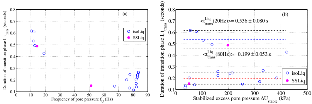
Figure 5.27: Evolution of duration of transient phase according to \Delta U_{stable} during isotropic liquefaction events.
