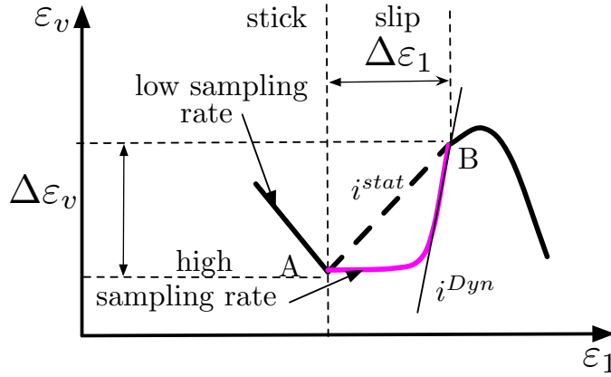
Figure 4.28: Static and dynamic anisotropy coefficients for instability.
