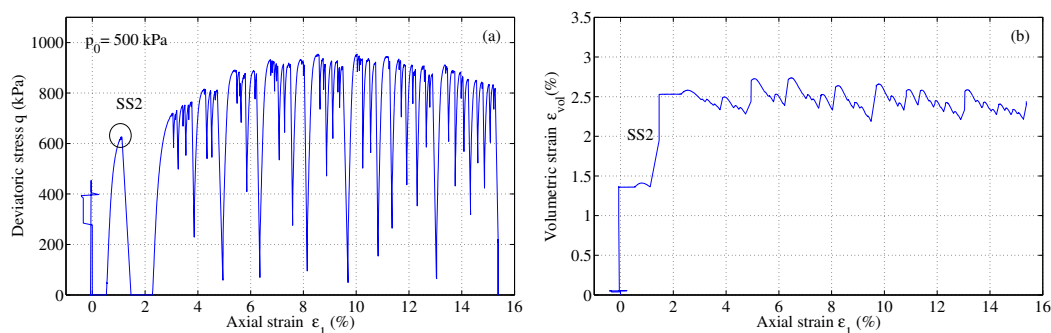
Figure 5.24: Global behaviour of stick-slip during triaxial compression of slender sample H/D = 2 .
