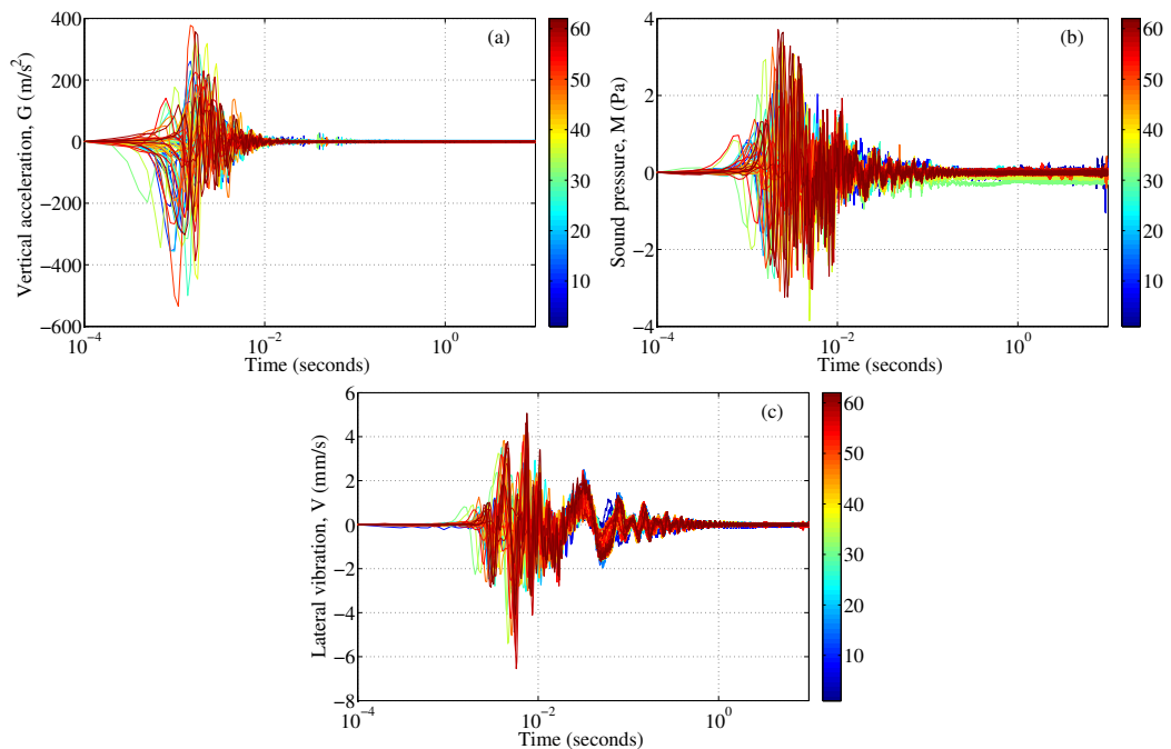
Figure 6.10: Detailed temporal evolution of G, M, V measurements of stick-slips at confining pressure of 120 kPa.
