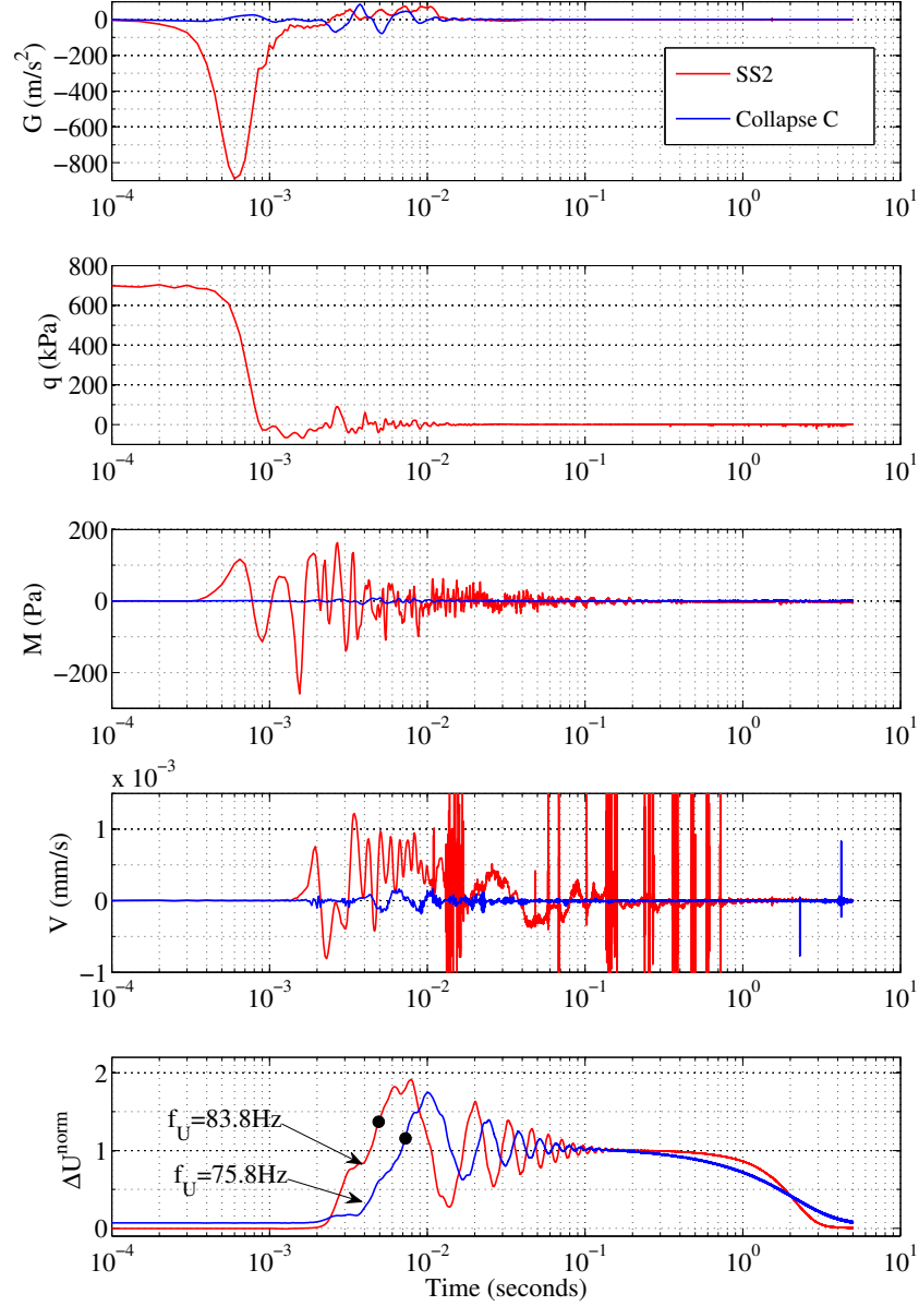
Figure 5.25: Detailed temporal evolution of measurements vertical acceleration, deviatoric stress, lateral sound pressure, lateral vibration, normalised excess pore pressure \Delta U^{norm} during stick-slip SS_{02} and collapse C.
