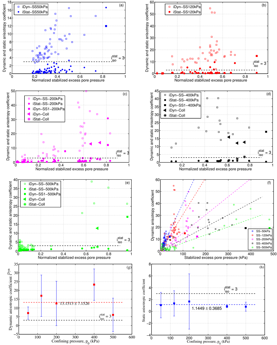
Figure 4.30: Static and dynamic anisotropy coefficients at different confining pressures.
