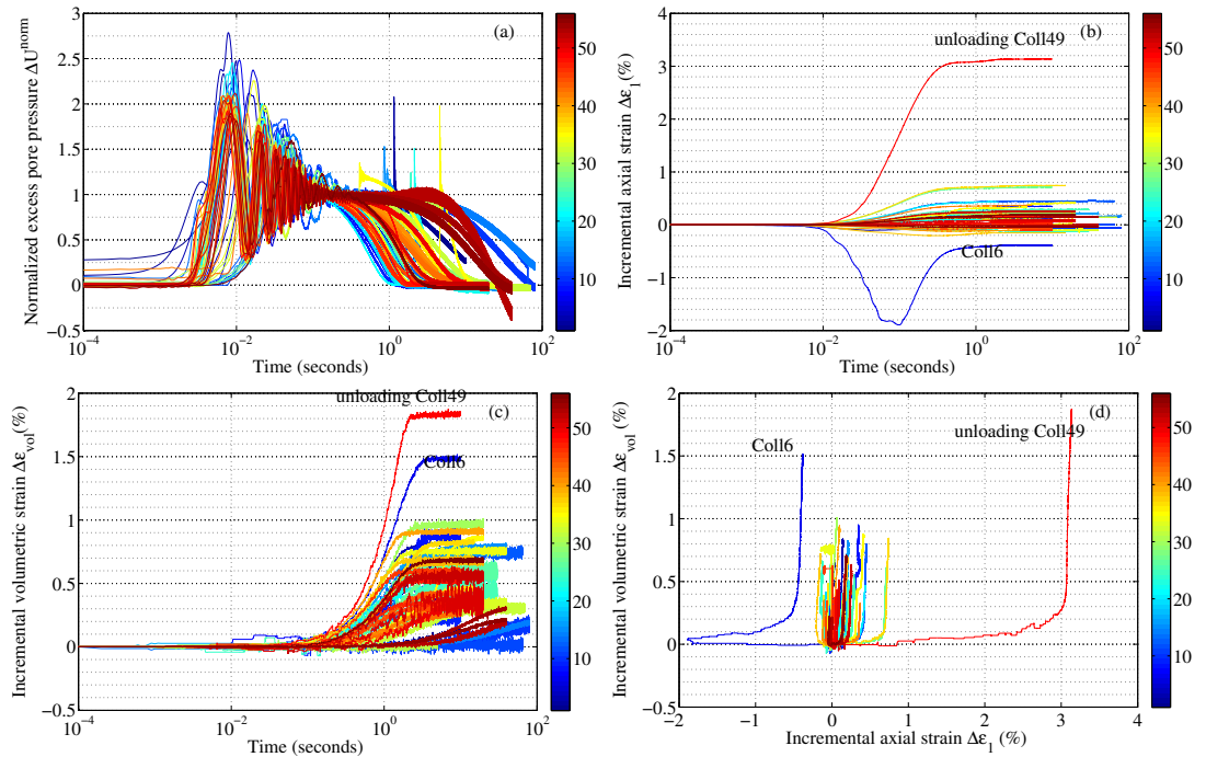
Figure 5.17: Detailed behaviour in isotropic collapse events.
