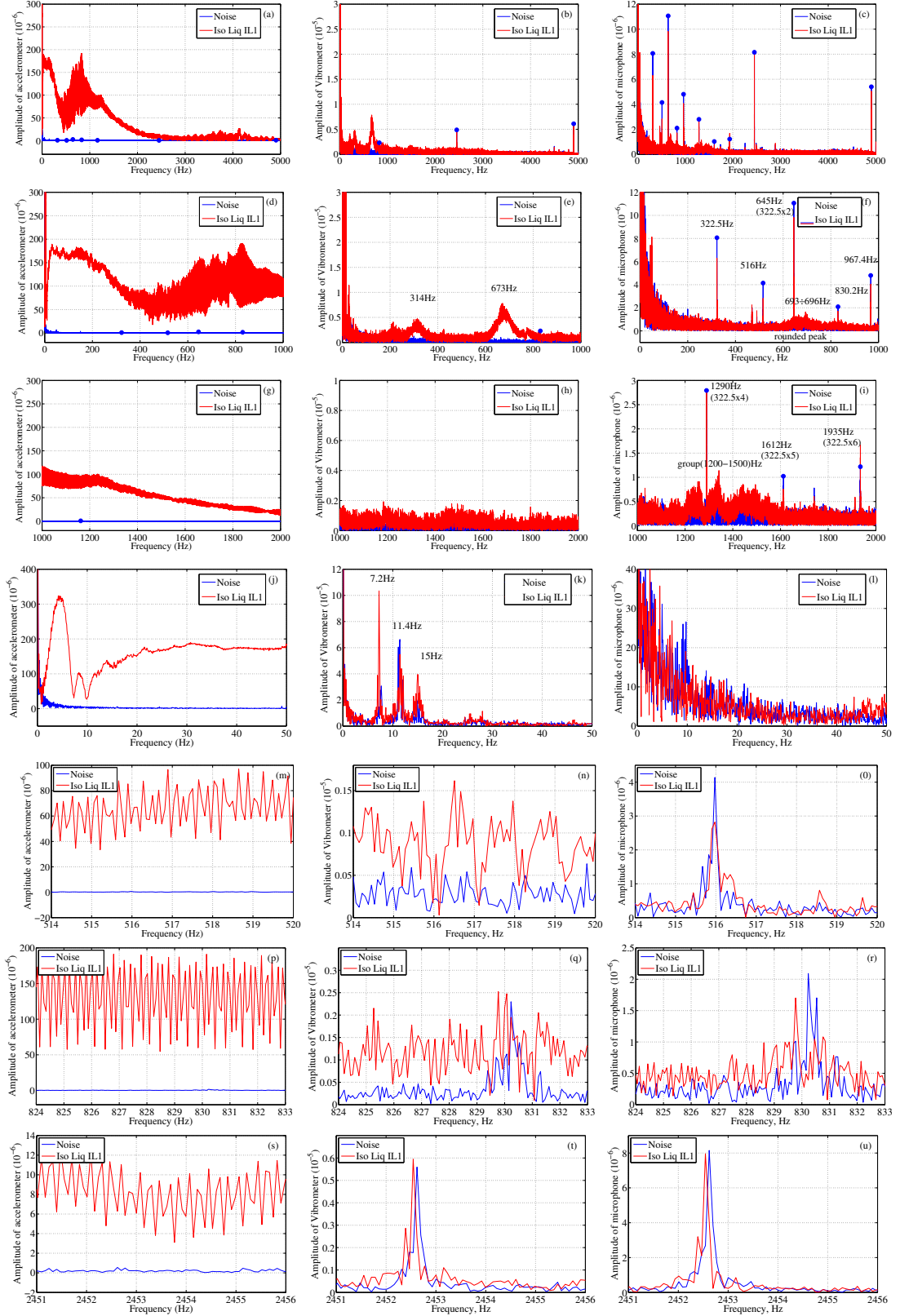
Figure 6.13: Frequency analysis by FFT of acceleration G (left), lateral vibration V (middle), lateral sound pressure M (right) of isotropic liquefaction event IL 01 .
