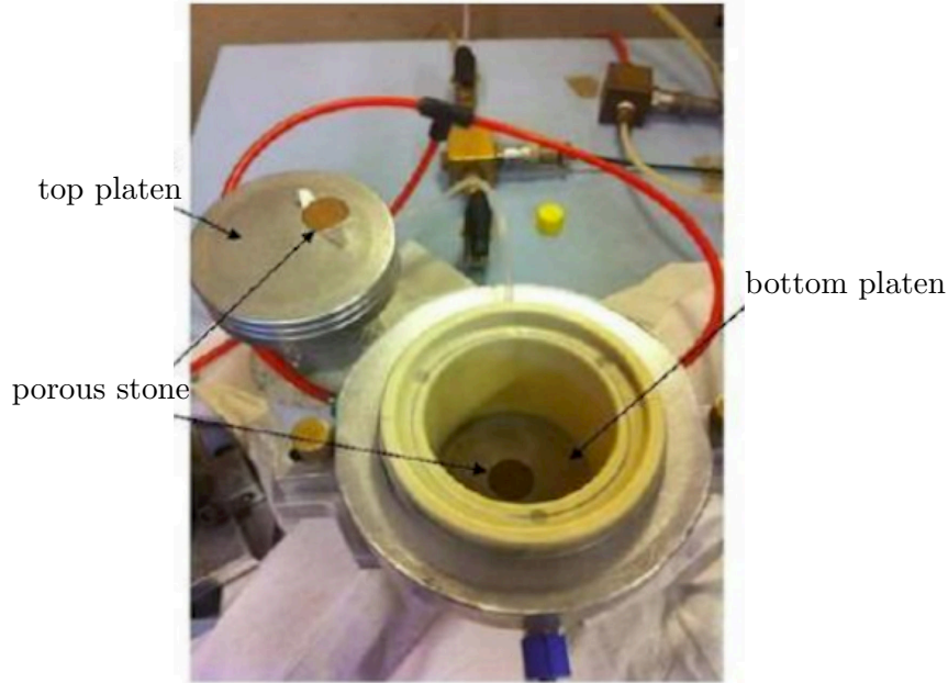
Figure 3.5: Scheme and picture of available mould for deposition of material
