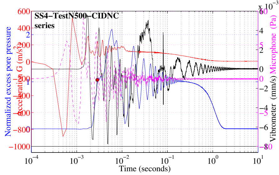
Figure D.3: Temporal evolution of acoustic measurements (G,M,V) and normalised excess pore pressure \Delta U^{norm} during SS 04 of test N500-CIDNC series.
