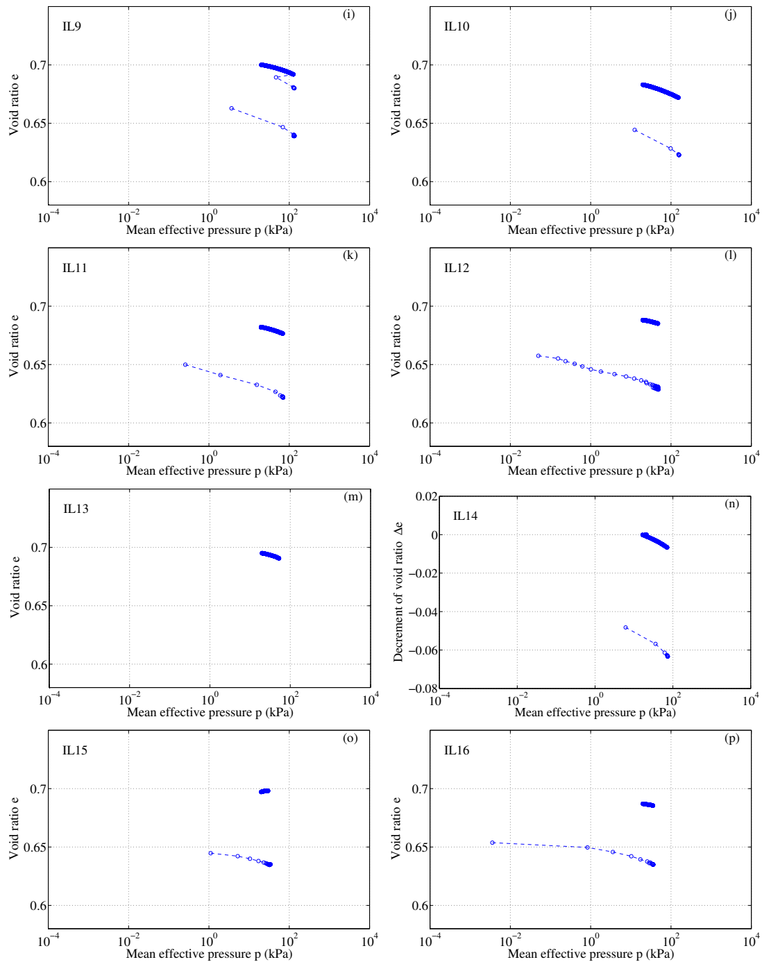
Figure 5.2: Compressibility behaviour in isotropic liquefaction (cont, from test IL 09 to IL 16 ).
