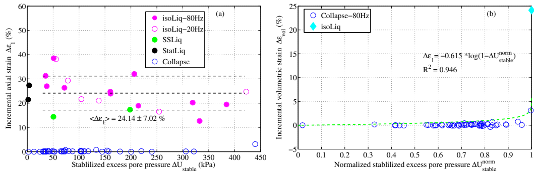
Figure 5.35: Incremental axial strain and stabilised excess pore pressure of liquefaction and collapse.
