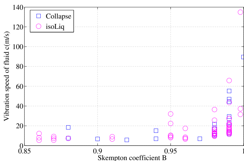
Figure 5.22: Variation of velocity of vibration of pore fluid in the relation to Skempton's coefficient B.
