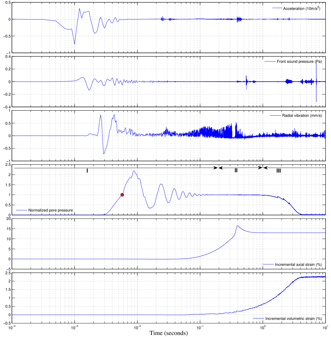
Figure 5.7: Detailed behaviour in typical isotropic liquefaction event IL_{05} at 252 kPa.
