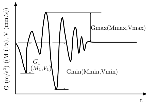
Figure 6.2: Notations of acoustic measurements.
