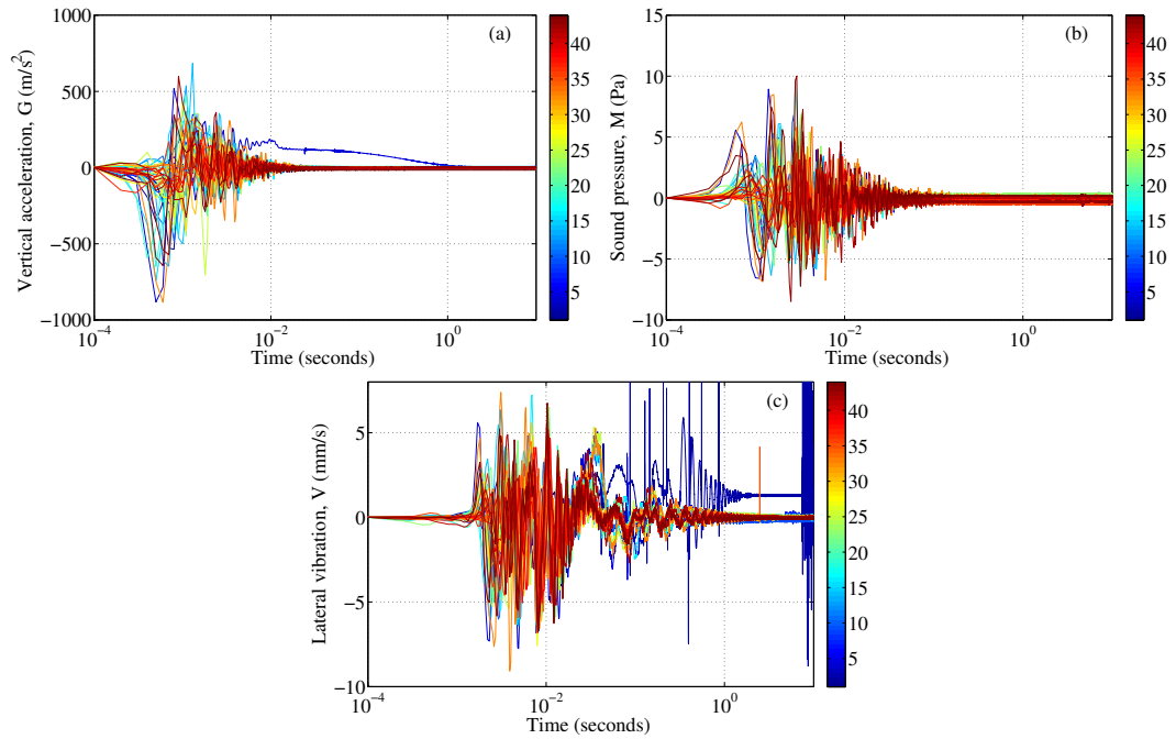
Figure 6.7: Detailed temporal evolution of G , M , V measurements of stick-slips at confining pressure of 500 kPa.
