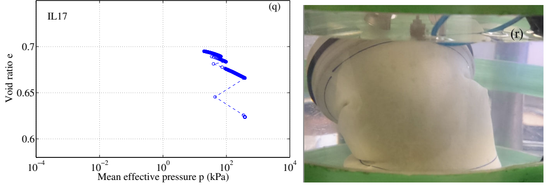
Figure 5.2: Compressibility behaviour in isotropic liquefaction (cont, test IL 17 ).
