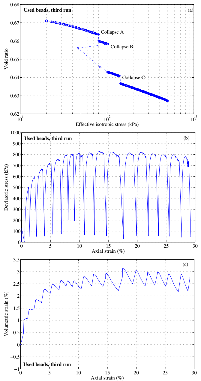
Fig. 14 (a) Isotropic consolidation with collapses at 80, 102 and 140 kPa, (b) drained compression stick-slip with (c) coupled volumetric behaviour at 500 kPa of confining pressure on the third run on saturated used glass beads.
