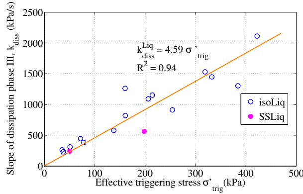
Figure 5.30: Slope of the dissipation phase III, k_{diss} as function of triggering stress \sigma'_{trig} .
