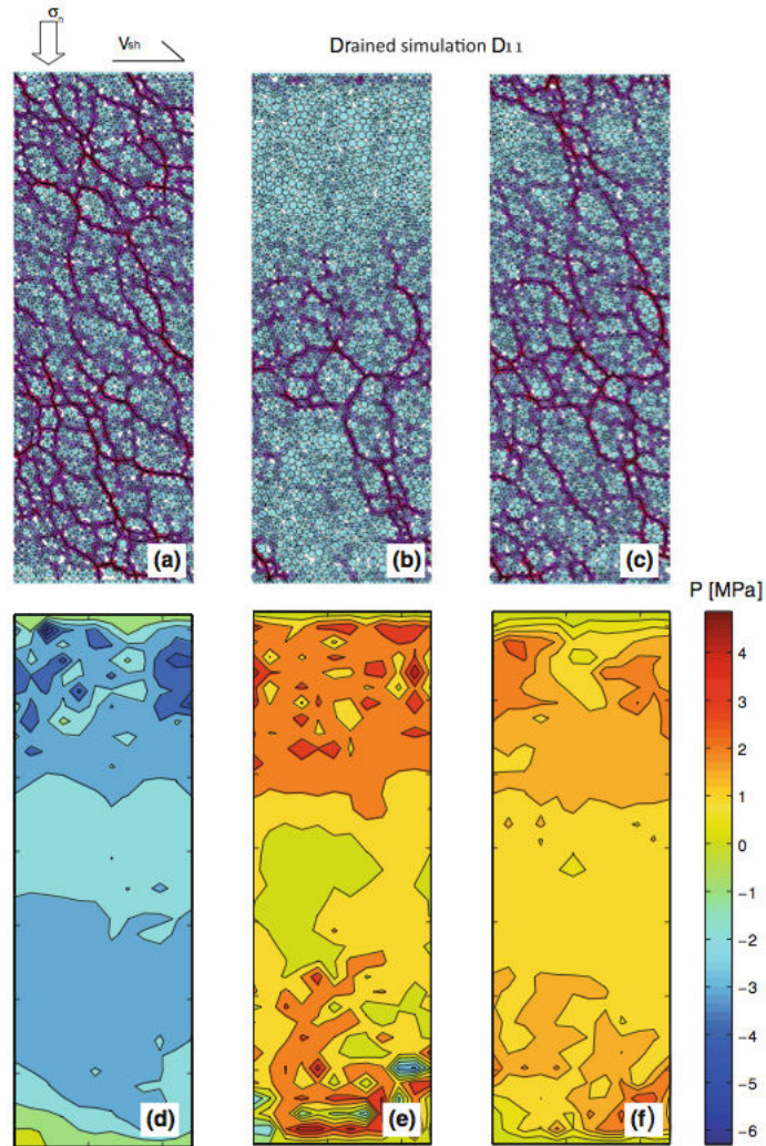
Figure 2.10: Liquefaction potential in drained numerical experiment with granular configuration (top) and pore pressure map (bottom) under 2.4 MPa of confining pressure (46).
