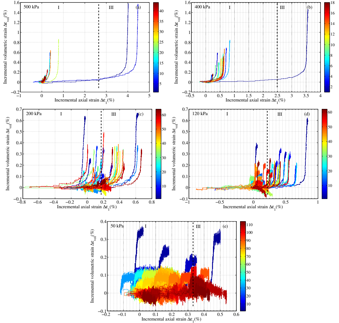
Figure 4.29: Evolution of incremental volumetric strain \Delta\varepsilon_{vol} in accordance with incremental axial strain \Delta\varepsilon_1 at different confining pressures.
