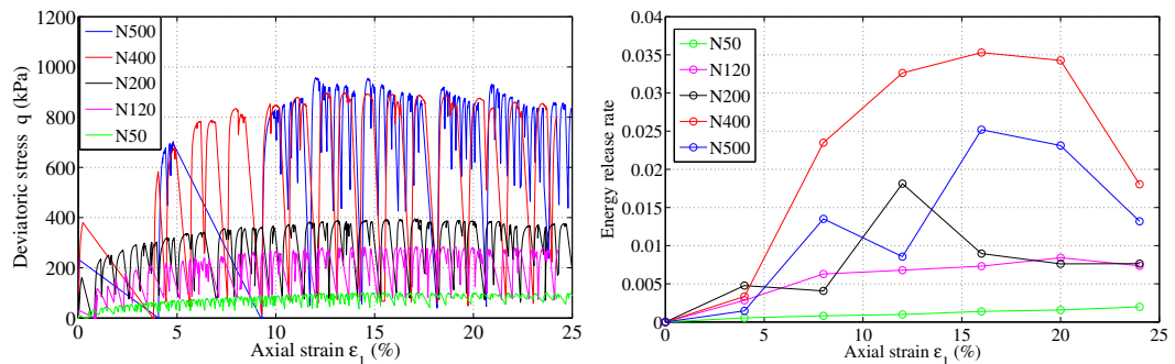
Figure 6.33: Energy release rate during shearing stage at different confining pressure (CIDNC series).
