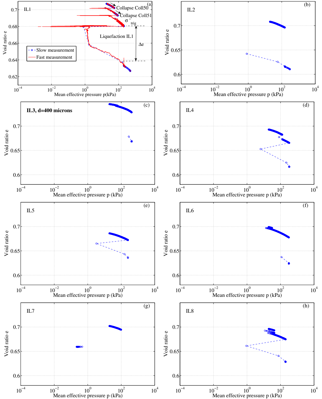
Figure 5.2: Compressibility behaviour in isotropic liquefaction from Test IL 01 to IL 08 .
