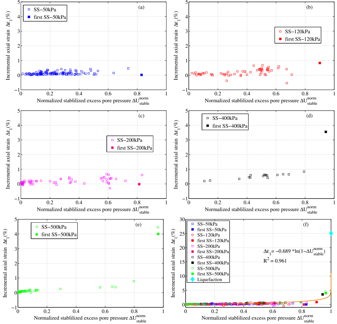
Figure 4.26: Relation of normalised stabilised excess pore pressure \Delta U_{stable}^{norm} and incremental axial strain \Delta \varepsilon_1 .
