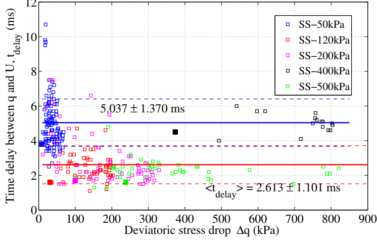
Figure 4.21: Time delay between deviatoric stress q and the buildup of pore pressure \Delta U in relevance with deviatoric stress drop \Delta q .
