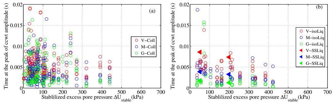
Figure 6.31: Time at the peak of CCWT amplitude of collapse (a) and liquefaction (b).
