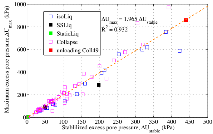
Figure 5.37: Maximum and stabilised excess pore pressure during liquefactions and collapses.
