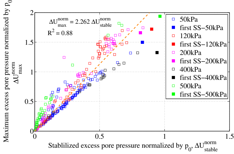
Figure 4.15: Maximum and stabilised excess pore pressure normalised by p'_0 in a linear relation.
