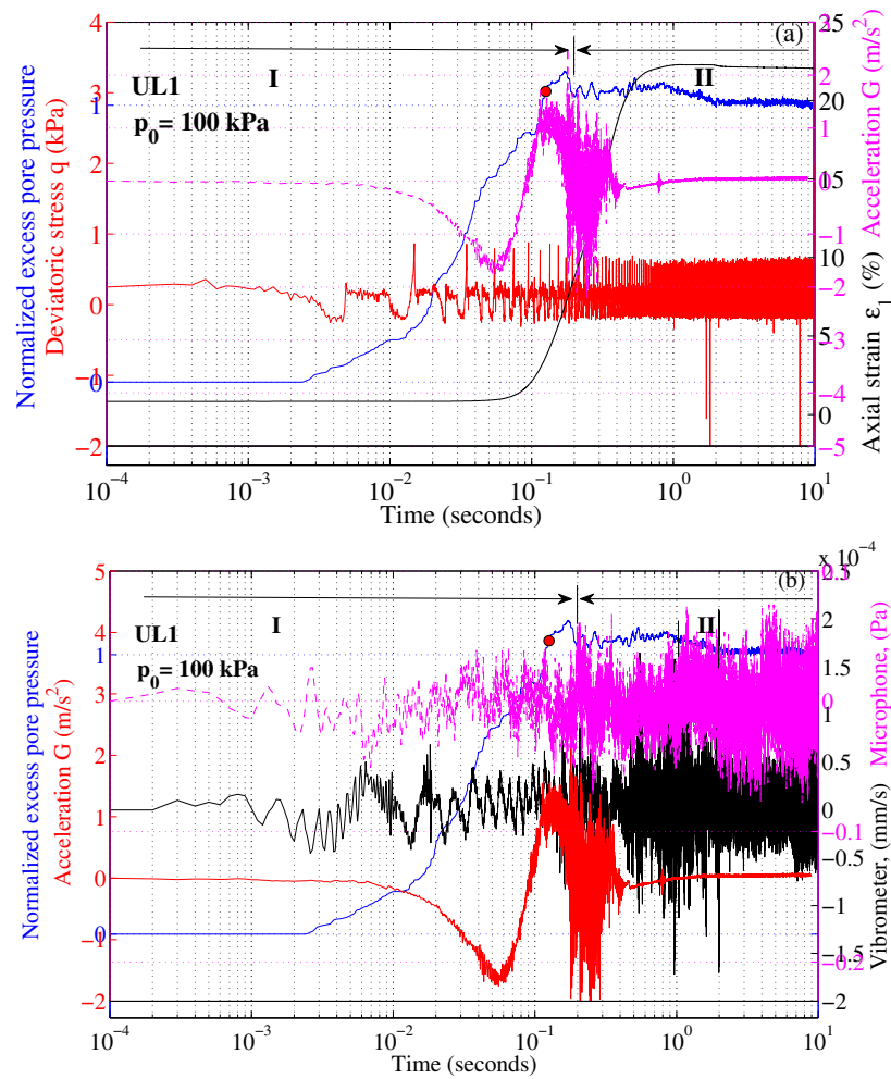
Figure 5.11: Detailed behaviour in static liquefaction event UL_{01} at initial confining pressure of 100 kPa.
