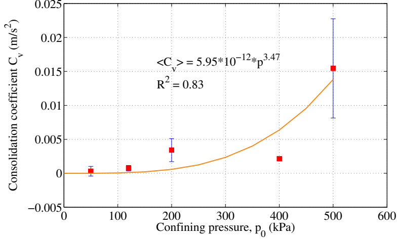
Figure 4.17: Mean of consolidation coefficient \langle C_v \rangle in relation to confining pressure p'_0 .
