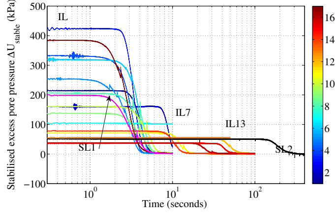
Figure 5.28: Dissipation phase of isotropic liquefaction events.
