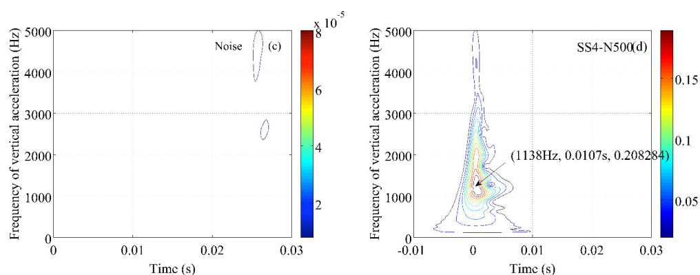
Figure D.6: CCWT spectrum of vertical top cap acceleration G for noise signal (left) and stick-slip SS_{04} of test N500 (right).
