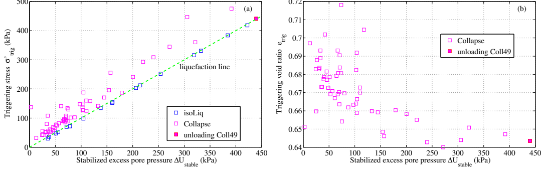
Figure 5.39: Triggering state in relevance with generated \Delta U_{stable} .
