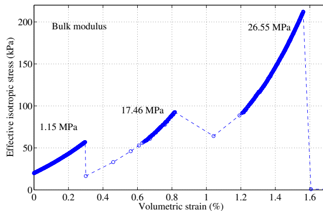
Figure 6.24: Bulk modulus of material during isotropic consolidation phase.
