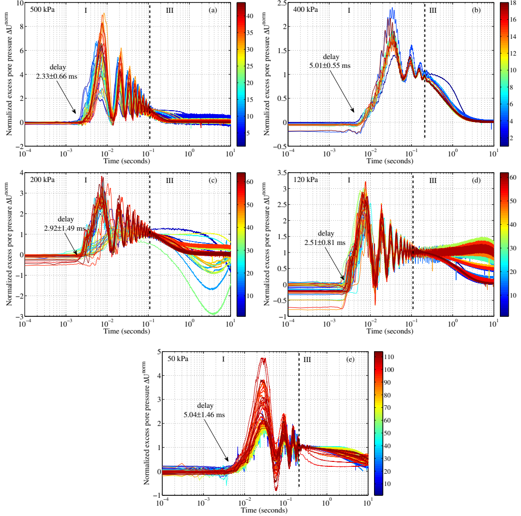
Figure 4.7: Time evolution of normalised excess pore pressure \Delta U^{norm} during stick-slip events at (a) 500 kPa of confining pressure, (b) 400 kPa, (c) 200 kPa, (d) 120 kPa and (e) 50 kPa.
