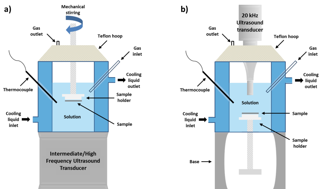
Figure II-4 Schematics of the reactors used for the sonication of the various metallic surfaces at (a) high and (b) low frequency ultrasound. Both set-ups enable the control of temperature, the sampling of solution, and the control of the sample position in the cell.
