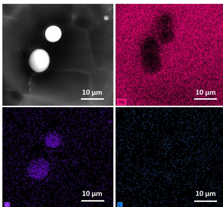
Figure IV-17 SEM-EDX analysis of secondary phases on Mg surface treated at 200 kHz ( P_{ac}= 20 W for 1 hour in 0.01 M oxalic acid solution, Ar, 18 °C). A shadowing effect can be noted on Mg map due to the position of the detector. Mg X-ray counts on the oxides are lower than bulk Mg explaining the color intensity differences for this map.
