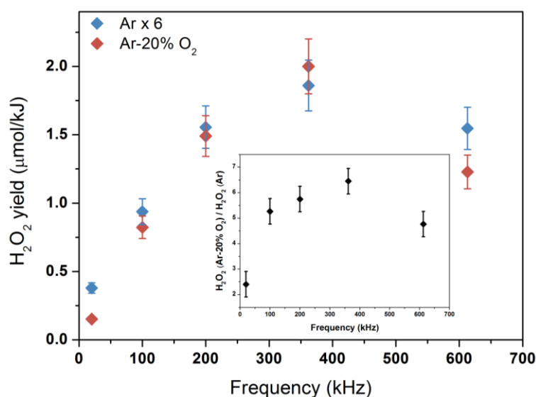
Figure III-1 \text{H}_2\text{O}_2 yields in pure water sonicated at 20 kHz ( P_{ac}= 33 W), 100 kHz ( P_{ac}= 40 W), 200 kHz ( P_{ac}= 45 W), 362 kHz ( P_{ac}= 43 W) and 612 kHz ( P_{ac}= 61 W) under 100 \text{ mL}\cdot\text{min}^{-1} Ar (blue) and Ar/(20 vol.%) \text{O}_2 (red) flow, at 18^\circ\text{C} , 100 rpm mechanical stirring (except at 20 kHz); insert: ratio of \text{H}_2\text{O}_2 yields for Ar/(20 vol.%) \text{O}_2 and Ar.
