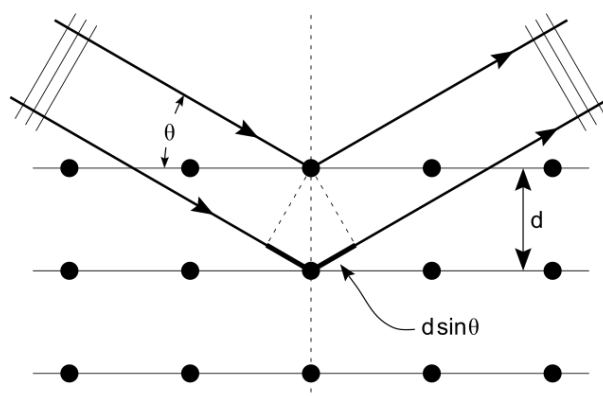
Figure II-9 X-ray diffraction. [183]
