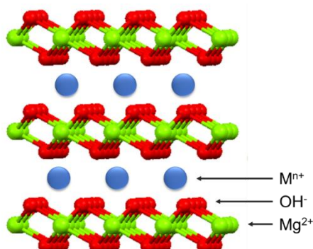
Figure V-21 Schematic representation of metal ions \text{M}^{n+} adsorbed in Brucite structure. [257]
