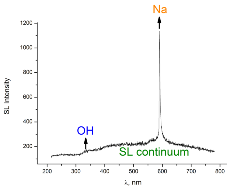
Figure III-8 SL spectra of 1 M NaCl solution sonolysis at 362 kHz ( P_{ac}= 43 W) under 100 \text{ mL}\cdot\text{min}^{-1} Ar flow, 14 \text{ }^{\circ}\text{C} .
