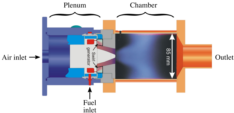
Figure 6.1: Sketch of the PRECCINSTA burner and Mean OH-LIF image. Adapted from (Meier et al. 2007).
