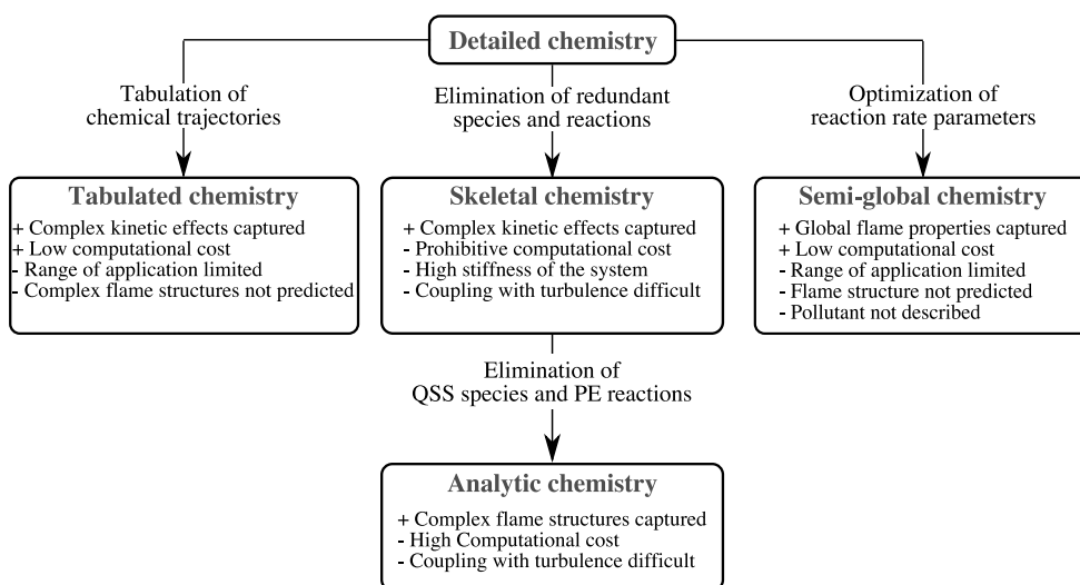
Figure 2.6: Main chemistry description strategies.
