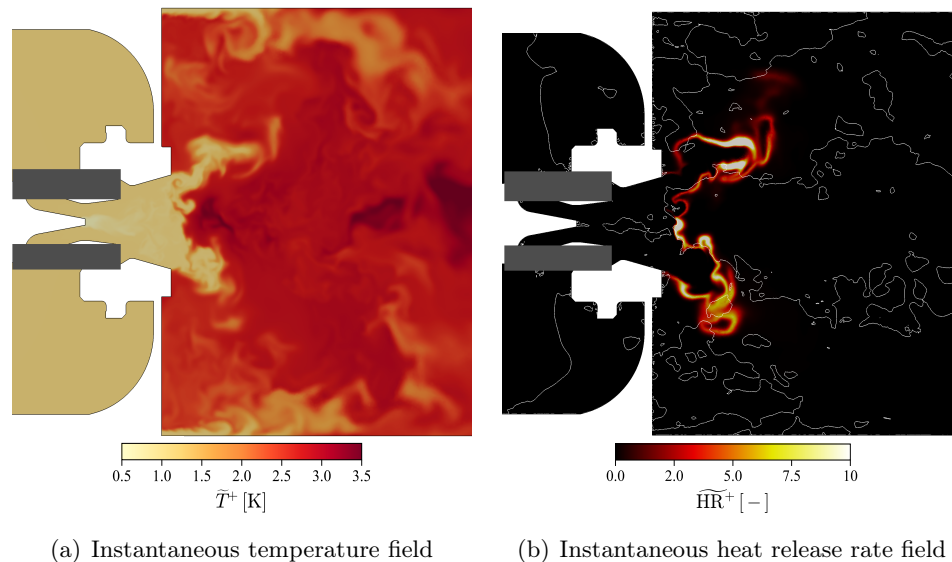
Figure 8.14: Instantaneous fields of resolved temperature and heat release rate. The white line in Fig. 8.14.b identifies the zero axial velocity.
