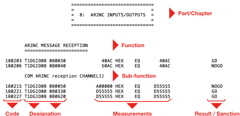
Figure 1.3: Extract of an .AR file. The figure shows the first lines of chapter "8: ARINC INPUT/OUTPUTS", with the function and sub-functions being tested, where two tests present the sanction: "NOGO".
