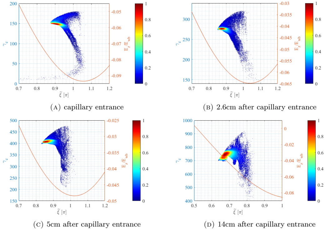
FIGURE 5.33: The longitudinal phase space of the electron bunch when propagates in the capillary
