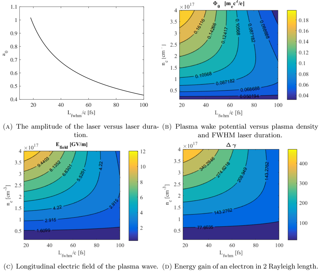
FIGURE 4.7: With the LASERIX laser E_L = 2\text{ J} , by setting the laser waist to r_s = 50.46\mu\text{m} , the amplitude of the laser versus laser length at focal plane is shown in A). The achievable maximum wake potential and longitudinal electric field with various plasma density and laser length are shown in B and C, the longitudinal electric field multiplied by two Rayleigh length is shown in D.
