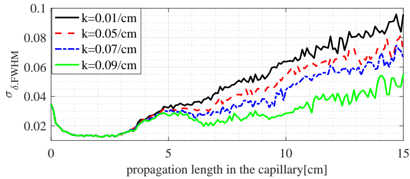
FIGURE 5.39: The evolution of the energy spread in the capillary tube, with different plasma density gradient
