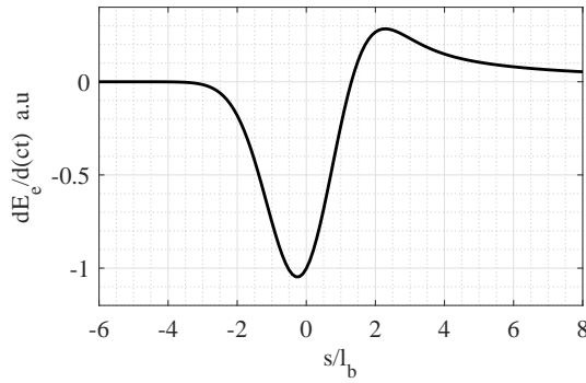
FIGURE 2.4: The CSR induced energy change of a line charge with Gaussian density distribution, the bunch head is on the right side
