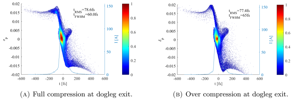
FIGURE 3.24: Longitudinal phase space of the electron bunch at 5.46 m, the dogleg exit is located at 5.03 m.
