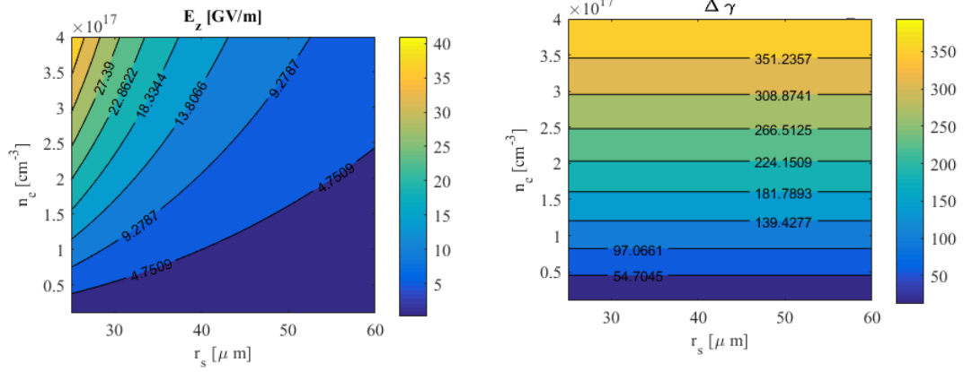
(C) Longitudinal electric field of the plasma wave.
