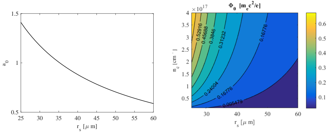
(B) Plasma wake potential versus plasma density and FWHM laser waist.
