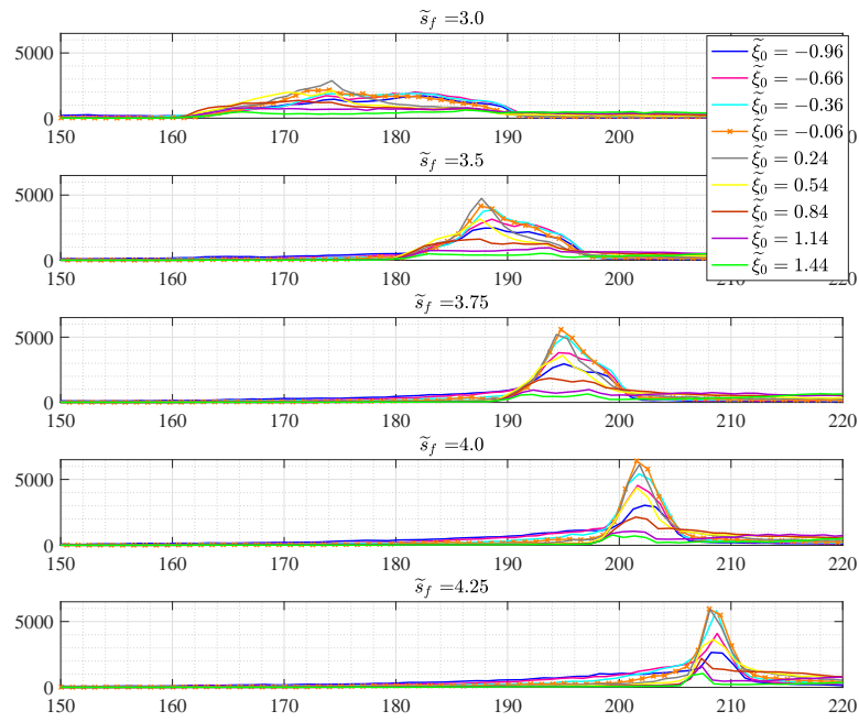
FIGURE 4.29: The energy distribution of the electrons at the exit of the plasma cell, with different starting position and injection phase, bin size is 1, the plasma density is 1.5 \times 10^{17}/\text{cm}^3 .
