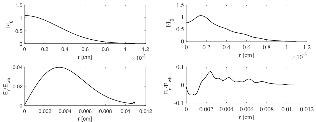
(A) The radial laser profile and the excited transverse electric field at s=0 (B) The radial laser profile and the excited transverse electric field at s=0.2\text{cm}
