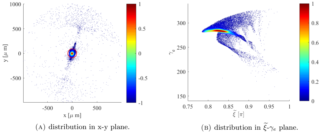
FIGURE 4.21: (A) The distribution of the electrons in the transverse plane, the red line shows a circle with a radius of 90 \mu\text{m} , (B) the longitudinal phase space of the electrons in the circle.
