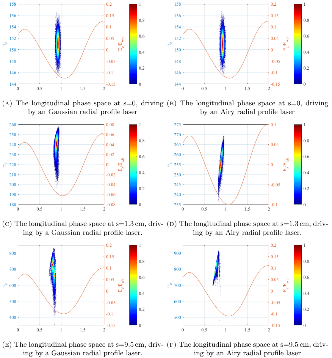
FIGURE 5.12: The longitudinal phase space of the electron bunch and the longitudinal electric field of the plasma wave at different position, the injection phase is 0.92\pi for all case.
