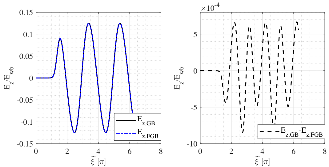
FIGURE 5.23: The excited longitudinal electric field with a GB and a FGB of order 4, with the same laser amplitude.
