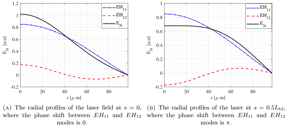
FIGURE 5.16: The radial profile of the laser field at s = 0 and s = 0.5L_{b2} , started with a focused FGB with order of N=4 .
