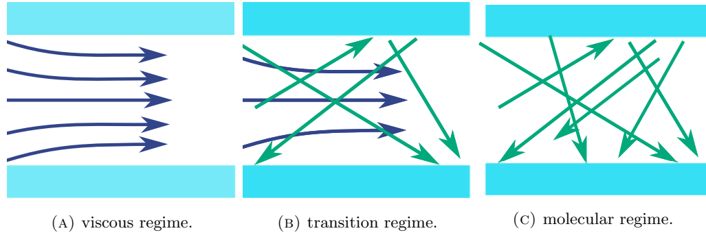
FIGURE 4.4: The motion of molecules in different regimes.
