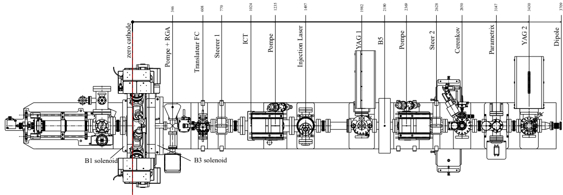
FIGURE 3.1: The layout of the original PHIL beamline.
