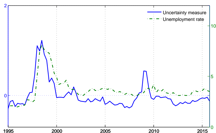
Figure 1.1: Uncertainty measure
