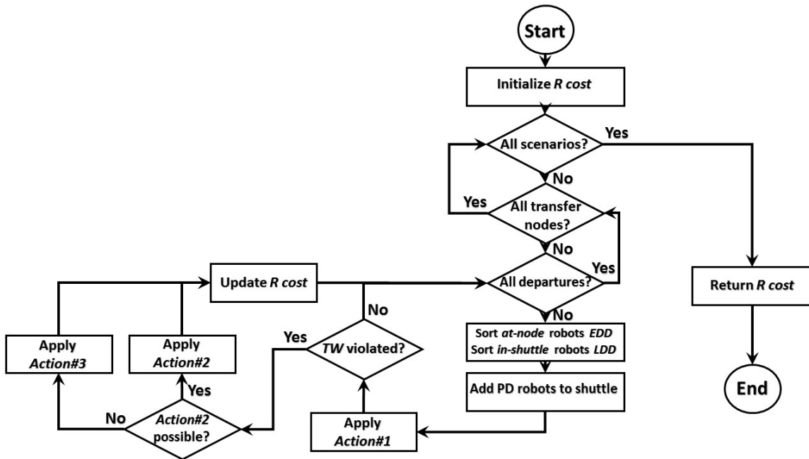
FIGURE 4.4: Calculate-Recourse-Cost Algorithm
