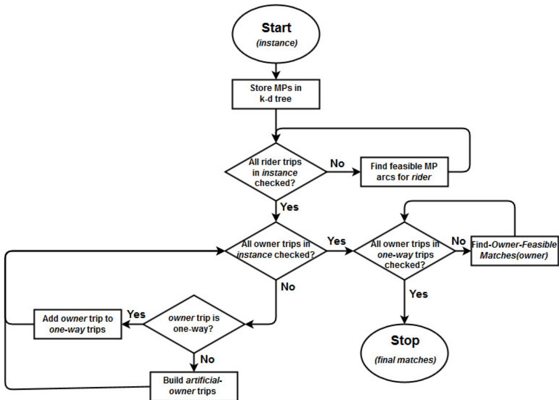
FIGURE 3.6: Algorithm 2 - Match-Generation
