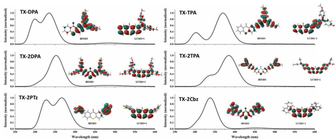
Figure 27: Simulated absorption spectra of studied Thioxanthone derivatives calculated by TD-B3LYP/6-31G(d,p) in gas phase.
