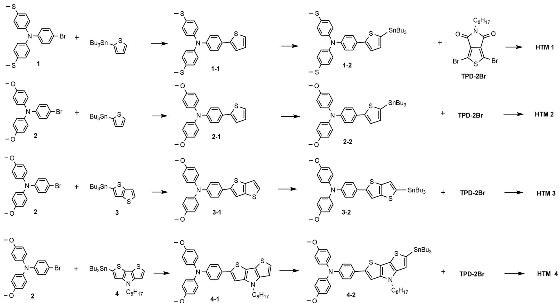
Scheme 3: Synthetic route of TPD-based planar structure molecules. Conditions and reagents: Stille coupling reaction: \text{Pd}(\text{PPh}_3)_4 , Toluene, 110^\circ\text{C} , 24h and Lithium-bromine exchange reaction: n -BuLi, THF, -78^\circ\text{C} , \text{Cl-SnBu}_3 , 8h.
