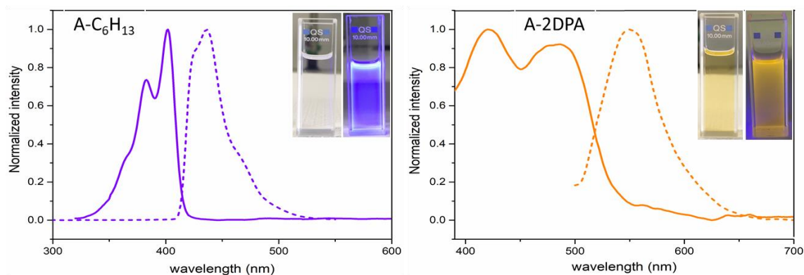
Figure 9 : Absorption (solid line) and emission (dashed line) spectra of A-C 6 H 13 and A-2DPA measured in diluted DCM. Inset: photographs of these solutions under daylight and UV 365 nm.
