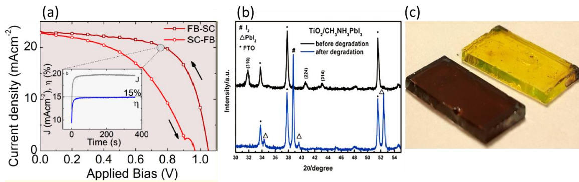
Figure 11: (a) Hysteresis of PSCs. Figure adapted from ref 87 . (b) XRD of perovskite-sensitized TiO 2 before and after degradation. Figure adapted from ref 89 . (c) Appearance of perovskite film before and after degradation.
