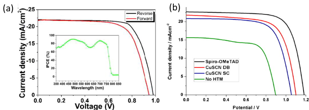
Figure 10: (a) Forward-reverse bias current density–voltage characteristics of the HTM-free PSCs and IPCE spectrum (inset). Figure adapter from ref 83 . (b) J–V curves of mixed perovskite solar cells based on CuSCN, spiro-OMeTAD, and no hole-transporting materials. Figure adapted from ref 84 .
