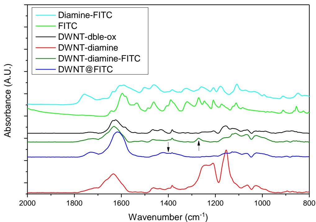
FIGURE A.4: Infra-Red spectra of the Diamine-FITC, FITC, DWNT-dble-ox, DWNT-diamine, DWNT-diamine-FITC and DWNT@FITC samples in the low frequency range between 2000 and 800 \text{cm}^{-1} .
