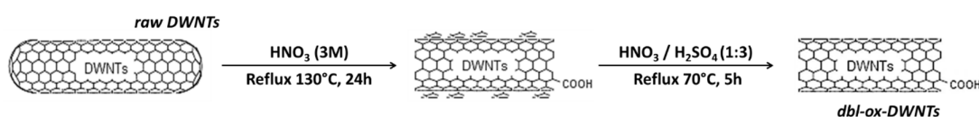
FIGURE 2.1: Illustration of the two steps of the double oxidation treatment.
