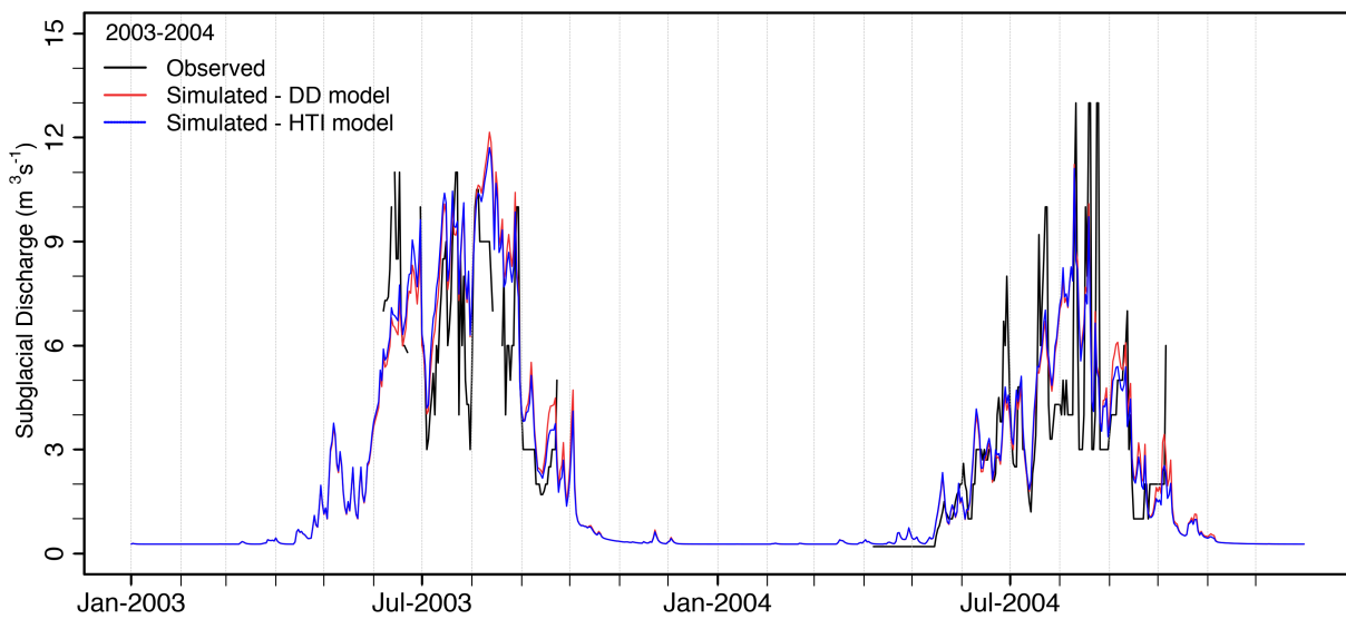
Figure IV.5: Observed and simulated subglacial discharge with DD and HTI models produced by the Argentière glacier, over the years 2003 and 2004.
