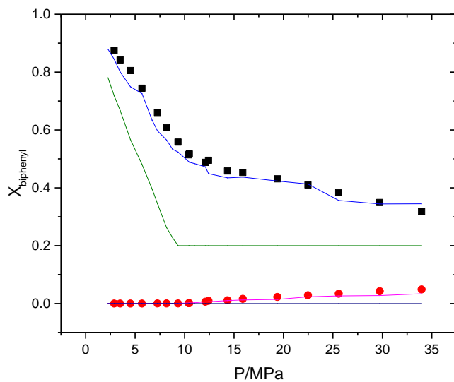
Figure 5.8. solubility curve of biphenyl in liquid and vapor phases. \blacksquare experiment-liquid phase, \bullet experiment-vapor phase, — simulation for the liquid phase CIRCE, — simulation for the vapor phase CIRCE, — simulation for the liquid phase ASPEN, — simulation for the vapor phase ASPEN/RGIBBS.
