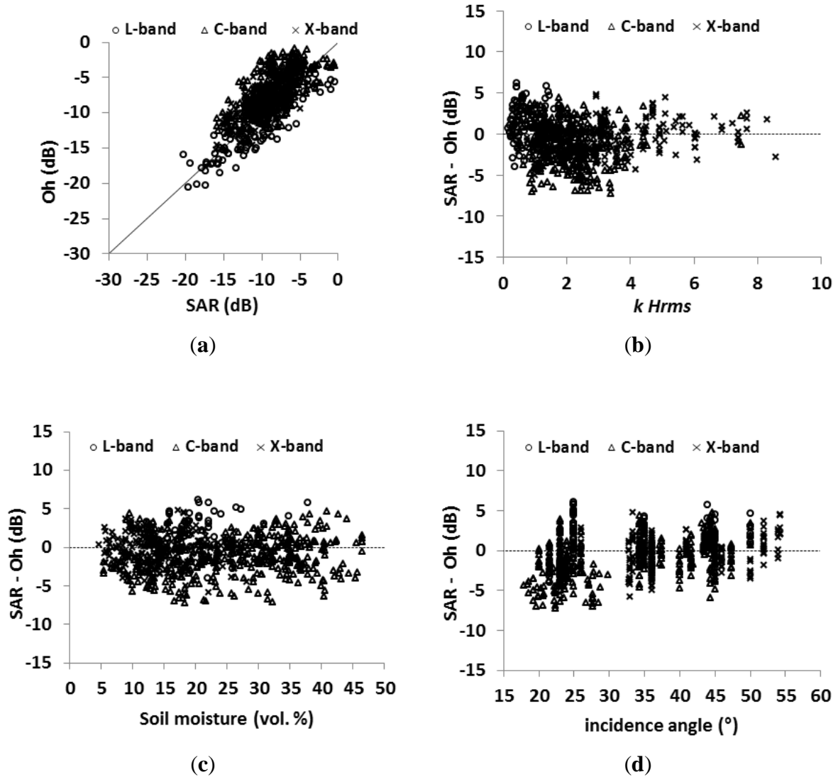
Figure III.9. Comparison between backscattering coefficients derived from SAR images and those estimated from the Oh 2002 model at VV polarization, (a) Oh simulations vs. SAR data; (b) difference between SAR signal and the Oh model vs. soil roughness ( kHrms ); (c) difference between SAR signal and Oh model results vs. soil moisture ( mv ); (d) difference between SAR signal and Oh model results vs. incidence angle.
