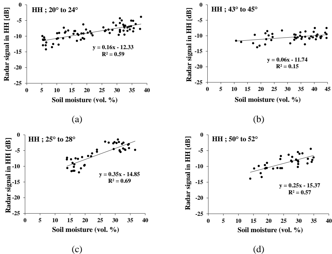
Figure II.6. Sensitivity of the radar signal in C and X bands to soil moisture. The H_{rms} values vary between 0.5 and 1.5 cm. (a): C-HH( 20^{\circ} - 24^{\circ} ), (b): C-HH( 43^{\circ} - 45^{\circ} ) (c): X-HH( 25^{\circ} - 28^{\circ} ), (d): X-HH( 50^{\circ} - 52^{\circ} ) (Baghdadi and Zribi, 2016).
