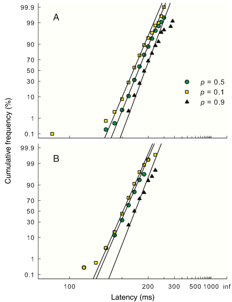
Figure 10: From Anderson & Carpenter (2006). Reciprobity plots of latency for three target appearance probabilities. Straits lines are maximum likelihood fits (Kolmogorov-Smirnov, p = 0.85 and 0.93 for Observers A and B, respectively) constrained to have a common intercept when latency is infinite, which is the characteristic pattern that occurs when an observer's prior probability shifts.
