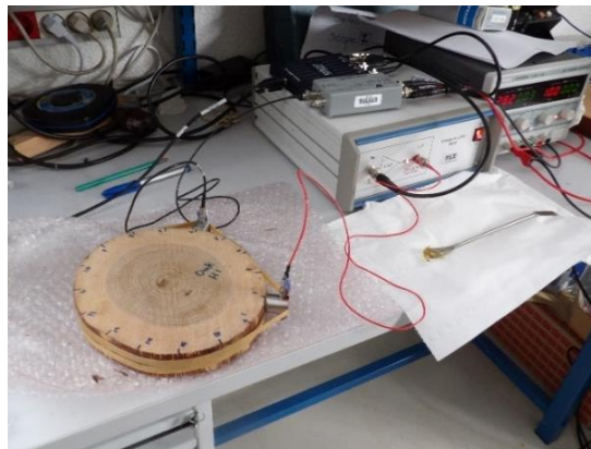
Figure 80: Experimental setting for the validation of the proposed inversion method for the case of a healthy oak disk.
