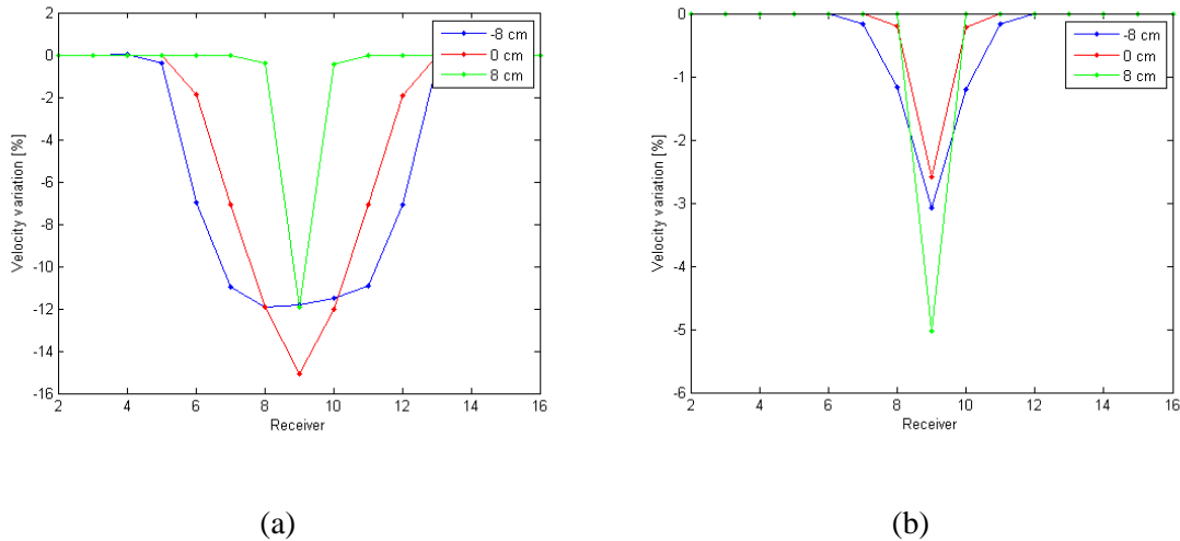
Figure 49: Velocity variation using straight-line distances (a-b) and velocity relative decrease (c-d), for orthotropic (left) and isotropic (right).
