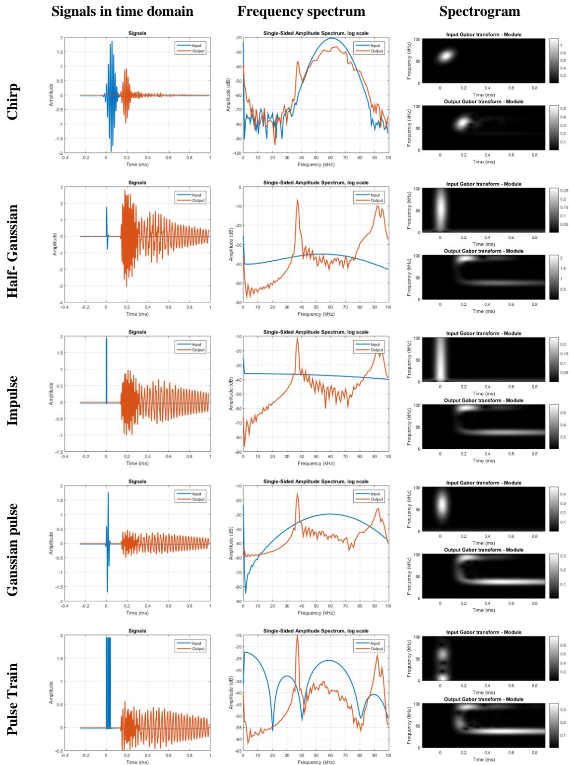
Figure 24: Time-frequency analysis for sensor R6 \alpha : input and output signals in the time domain (left), their frequency spectrum (center) and spectrogram (right) (Espinosa et al. 2018).
