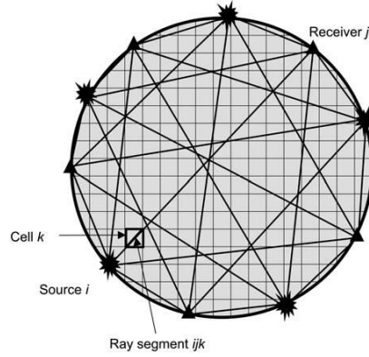
Figure 67: Pixel grid distribution for the algebraic reconstruction (Maurer et al. 2006).
