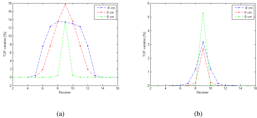
Figure 48: TOF variation in all receivers changing the defect position for (a) Orthotropic and (b) isotropic
