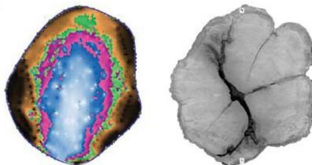
Figure 3: Comparison of acoustic tomogram (left) and photograph from cross-section for Red Oak tree (Wang 2007).
