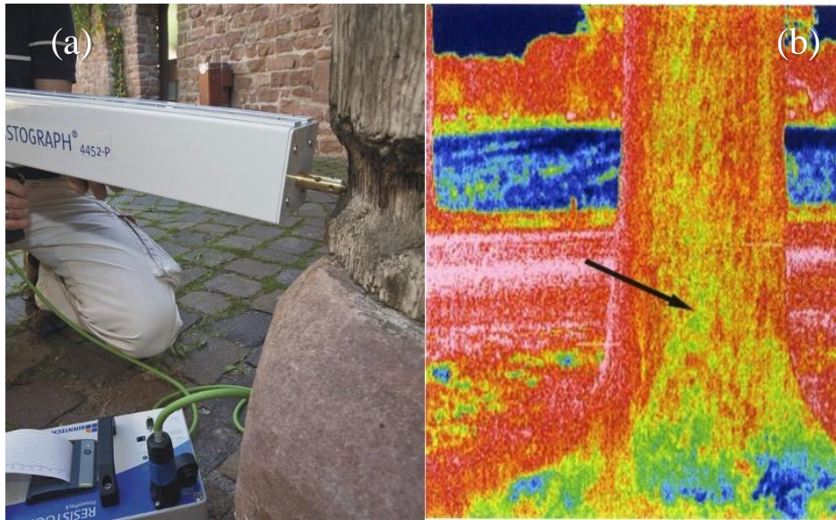
Figure 2: Some methods for nondestructive evaluation of wood: (a) Drilling measure (Source: http://www.resistograph.com/ ), (b) Thermography imaging (Catena and Catena 2008).
