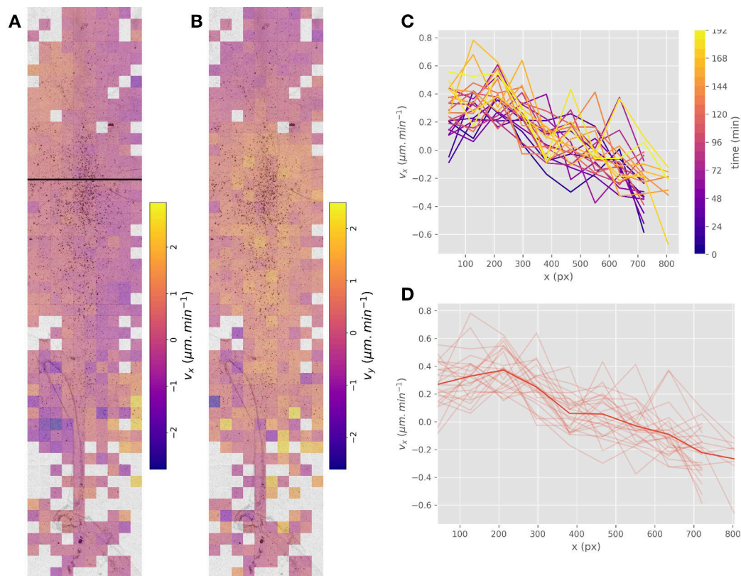
FIGURE C.2 – Map analysis. Maps of velocity components v_x ( A , along the ML axis ) and v_y ( B , along the AP axis ). Anterior is up, posterior is down. Postive values defines left to right displacements and anterior to posterior displacement. Average v_x profile along solid line panel A . Temporal evolution ( C ) and time average ( D ). Individual profiles are shown in transparency and time average as a solid line. Note the positive values (left to right movements) on the left part of the profile and the negative values (right to left movements) on the right part of the profile, indicating convergent movements towards the midline.
