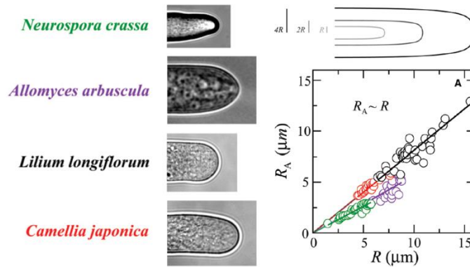
Figure 2.17. Tip scaling in various tip growing organisms. (Left) Typical images of fungal hyphae from Neurospora crassa and Allomyces arbuscula , and pollen tubes from Lilium longiflorum and Camellia japonica . (Right) A schematic of shape scaling and plot of the measured parameters for the species on the left. Adapted from (Campas et al., 2012).
