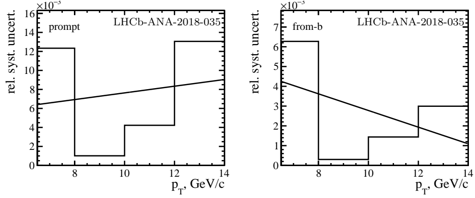
Figure 5.28: Relative systematic uncertainty due to mismodeling of p_T -dependence of t_z resolution in bins of p_T . The solid black line shows a smoothing curve.
