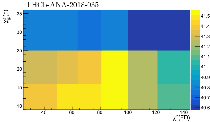
Figure 8.3: Optimisation map as a function of applied requirements on proton transverse momentum p_T(p) and charmonium transverse momentum p_T(p\bar{p}) (a), \chi^2 of flight distance of charmonium candidates \chi^2(FD) and \chi^2 of track impact parameter (b) with respect to the best primary vertex \chi^2_{IP}(p) . The FoM = N_{sig} / \sqrt{N_{sig} + N_{bkg}} is shown with the color code. The plots are 2D projections of the 4D optimisation.
