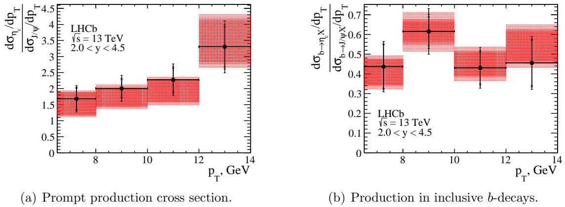
Figure 5.39: The ratios of \eta_c and J/\psi differential production cross-sections (points) compared to result obtained with separation technique (red boxes). The uncertainties shown are statistical, systematic, and the uncertainty due to the J/\psi \rightarrow p\bar{p} and \eta_c \rightarrow p\bar{p} branching fractions.
