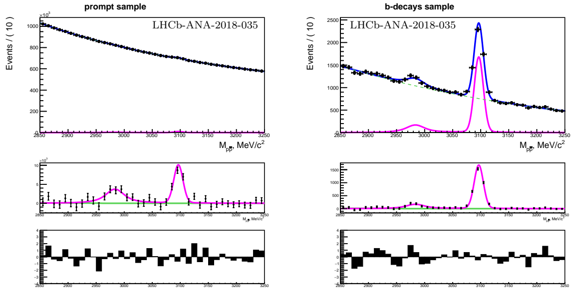
Figure 5.31: The M_{p\bar{p}} distribution for prompt (left) and b -decays (right) for 6.5 \text{ GeV} < p_T < 8.0 \text{ GeV} . The solid blue lines represent the fit result. Magenta and green lines show the signal and background components, respectively. The corresponding residual and pull distributions are shown below.
