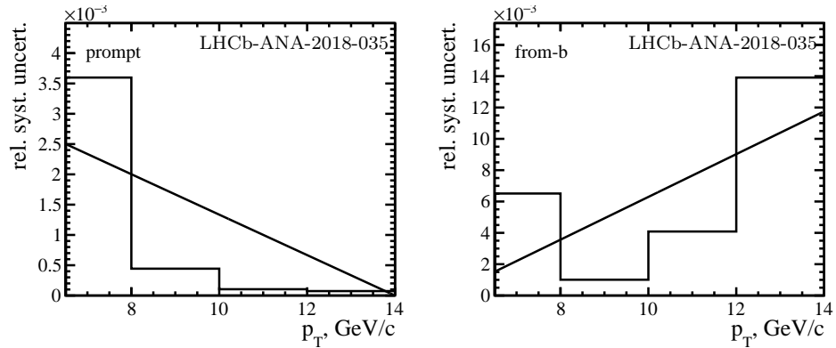
Figure 5.29: Relative systematic uncertainty due to mismodeling of p_T -dependence of \tau_b distribution in bins of p_T . The solid black line shows a smoothing curve.
