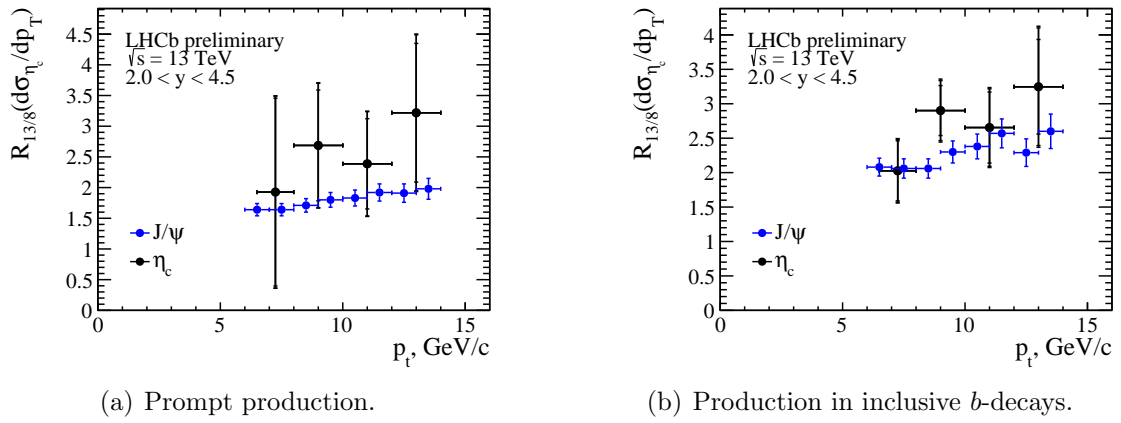
Figure 5.42: Ratios of the \eta_c (black points) and J/\psi (blue points) differential production cross-sections at \sqrt{s} = 13 and 8 TeV. The uncertainties shown are statistical, systematic and due to J/\psi production cross-section ratio.
