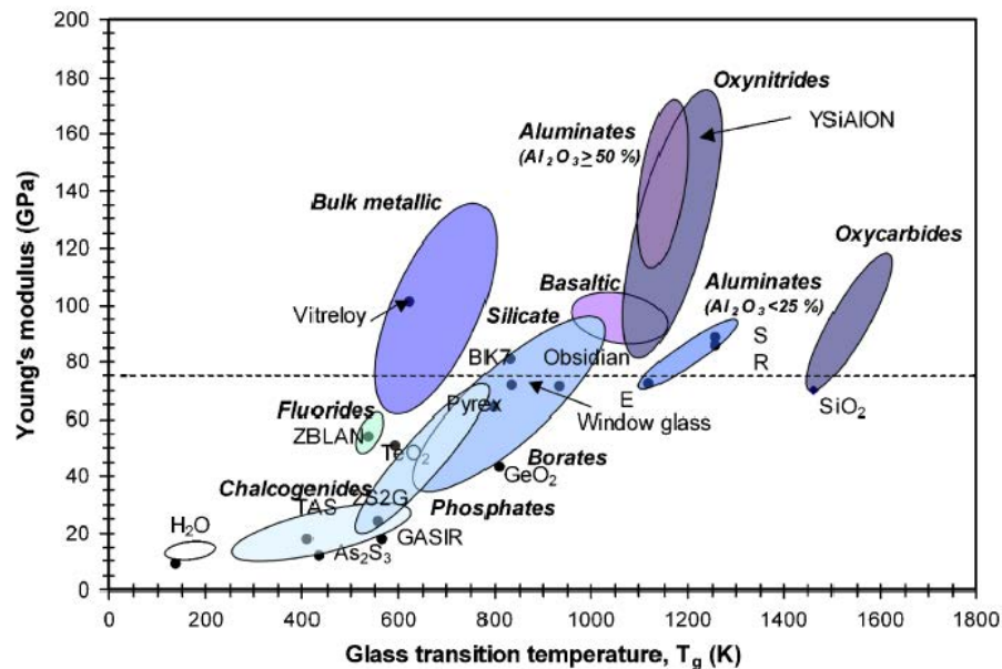
Figure 3.14 Relation between Young's modulus and the glass transition temperature of several glass systems. Values at room temperature, except for glassy H 2 O (taken at -196 °C). Some commercial glasses are also indicated [70].
