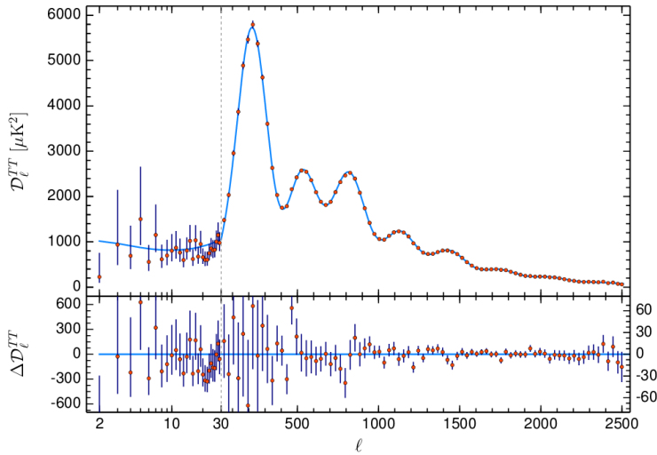
Figure 6.3: Planck 2018 CMB angular power spectra as function of the multipole moment, fitted with the \Lambda CDM prediction. Figure extracted from Ref. [143].
