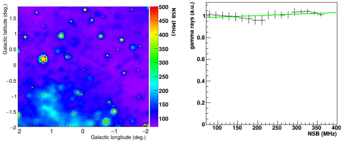
Figure 8.14: Left: Night Sky Background intensity map (MHz) in Galactic coordinates in the GC region. Right: Distribution of the gamma-like rate (residual background) as function of the NSB (MHz), normalized to 1. The standard deviation in the Y-axis is 0.036.
