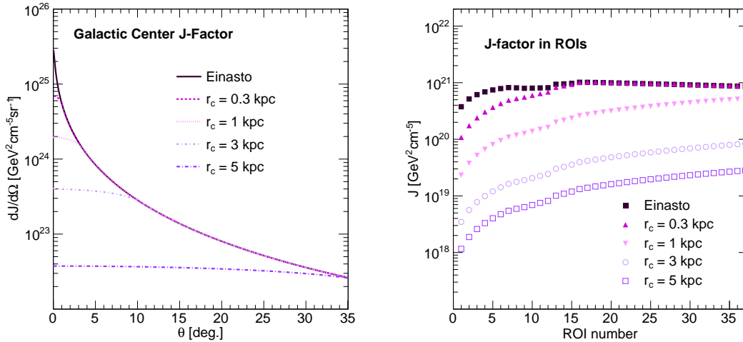
Figure 11.3: Dark matter core profiles considered here for forecast H.E.S.S.-I-like limits on the Wino annihilation cross section. Left panel: differential J-factor curves for several DM core sizes as function of the distance from the GC from Eq. (6.9). Right panel: integrated J-factor in ROIs from Eq. (6.12) up to 4.0^\circ for several DM core sizes.
