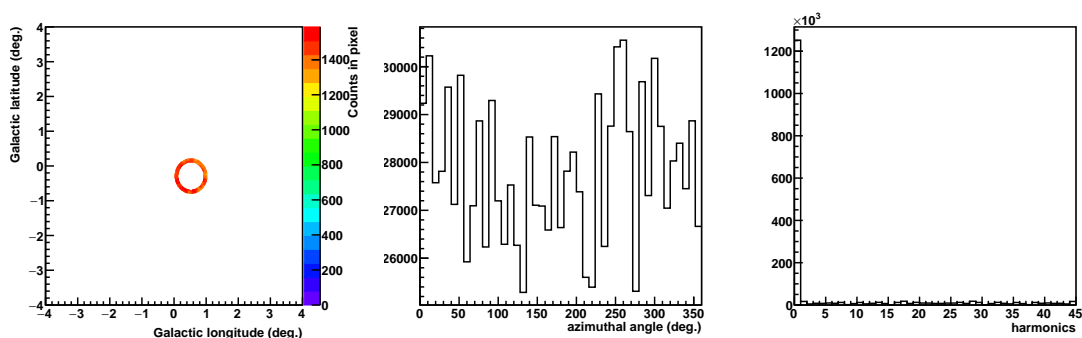
Figure 8.13: Test of azimuthal symmetry. Left panel: Region of the sky, in Galactic coordinates, chosen for the test. The Z-axis represents the number of hadron-like events per pixel of dimension 0.02^\circ \times 0.02^\circ . Central panel: distribution of the number of counts at different azimuthal angles around the pointing position. Right panel: harmonic of the fast Fourier transform of the distribution of counts with respect to the azimuth. No significant harmonic beyond the 0-th. No periodicity is observed in the variation of the number of events.
