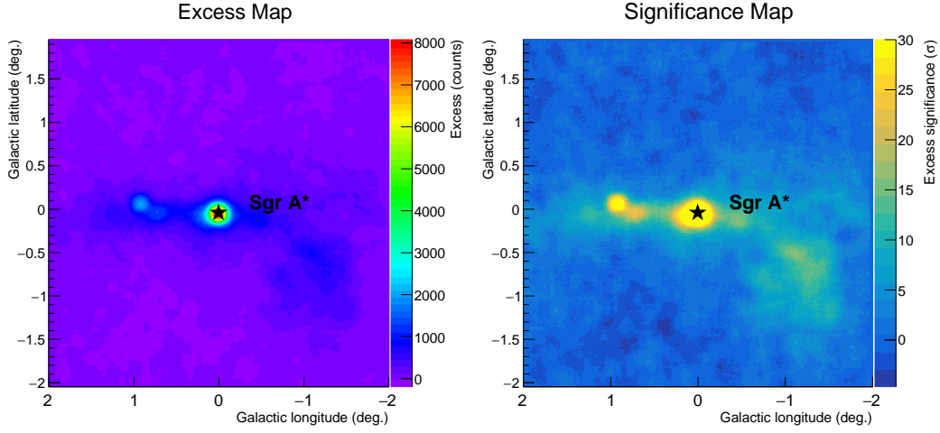
Figure 8.2: Excess and significance sky maps obtained from a Ring Background analysis of 10 years of H.E.S.S. I observations towards the GC. The maps are computed in bins of 0.02^\circ \times 0.02^\circ and they are convoluted for a Gaussian with width chosen according to the H.E.S.S. PSF. The maps are plotted in Galactic longitude and latitude. Left panel : Excess map. Right panel : Significance map.
