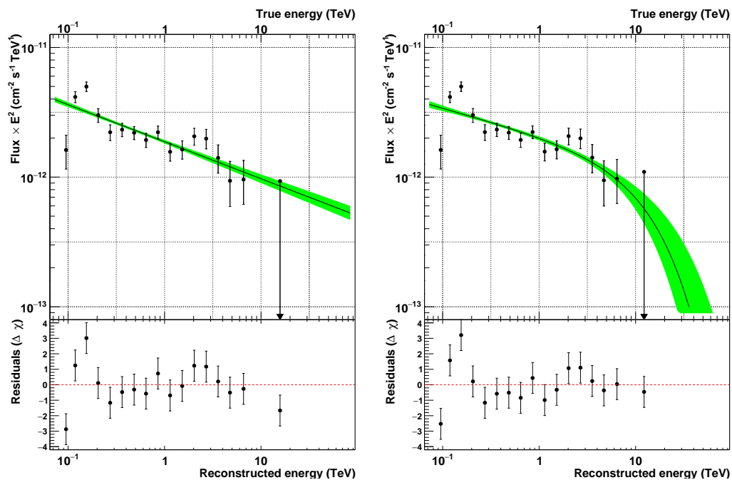
Figure 5.15: Spectrum of Sgr A* with H.E.S.S.-II CT5 Mono analysis. The value of the parameters is given in the text.
