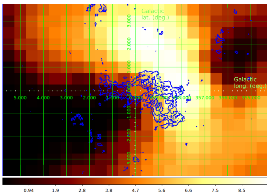
Figure 5.14: Map of low-latitude Fermi Bubble emission detected by Fermi-LAT [89] with overlapped H.E.S.S.-II significance contours at 3\sigma , 5\sigma and 7\sigma . The presence of a VHE asymmetric emission shifted towards the North-West of the GC could be correlated with the Fermi Bubbles. A dedicated analysis is currently carried out in order to search for VHE emission from the Fermi Bubbles with H.E.S.S..
