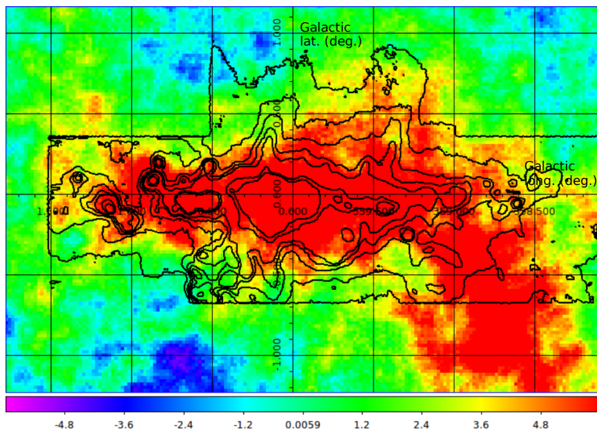
Figure 5.13: H.E.S.S. significance map with overlaid the 5 GHz radio contours by the Green Bank Telescope [101]. The map is saturated at 6\sigma in order to emphasize the diffuse emissions. There may be hints of correlation between H.E.S.S.-II diffuse emission and radio outflows.
