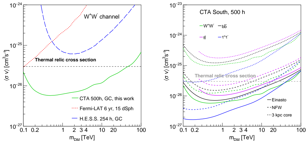
Figure 12.6: Left panel: CTA constraints on \langle\sigma v\rangle (green solid line) in the inner 5^\circ of the GC for the W^+W^- channel, compared to those by H.E.S.S. [236] (blue dashed line) and Fermi-LAT [256] (red dotted line) in the GC region. Right panel: CTA constraints on \langle\sigma v\rangle derived assuming an Einasto profile (solid lines) for the Galactic Center halo, compared to those obtained for a NFW profile (dashed lines) or a cored profile of size 3 kpc (dotted lines). The W^+W^- (green lines), b\bar{b} (black lines), t\bar{t} (violet lines) and \tau^+\tau^- (blue lines) channels are tested. The thermal relic cross section (gray dashed line) is shown.
