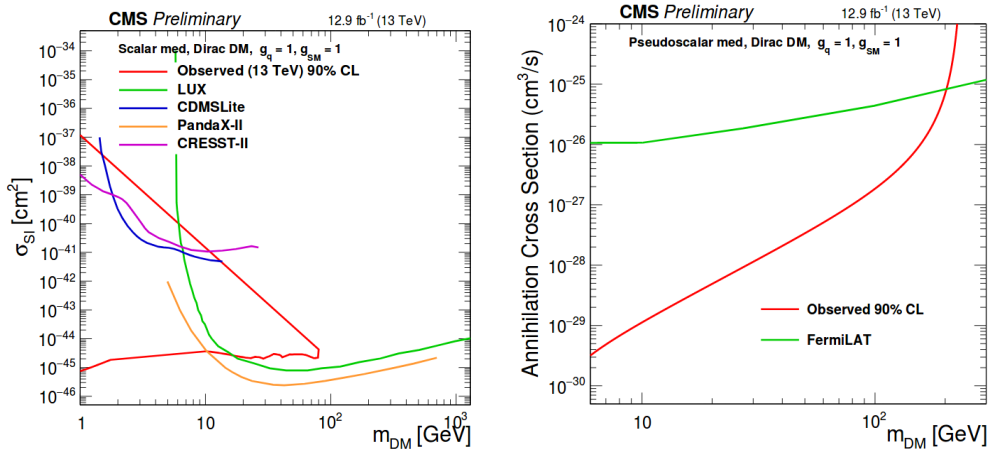
Figure 6.8: Comparison of DM techniques through simplified models. Left panel: comparison of direct detection and collider searches assuming scalar mediator. Constraints on the spin-independent DM-nucleon scattering cross section versus DM mass. Right panel: comparison of indirect detection and collider searches assuming pseudoscalar mediator. Constraints on the DM annihilation cross section versus DM mass. Figure extracted from [198].
