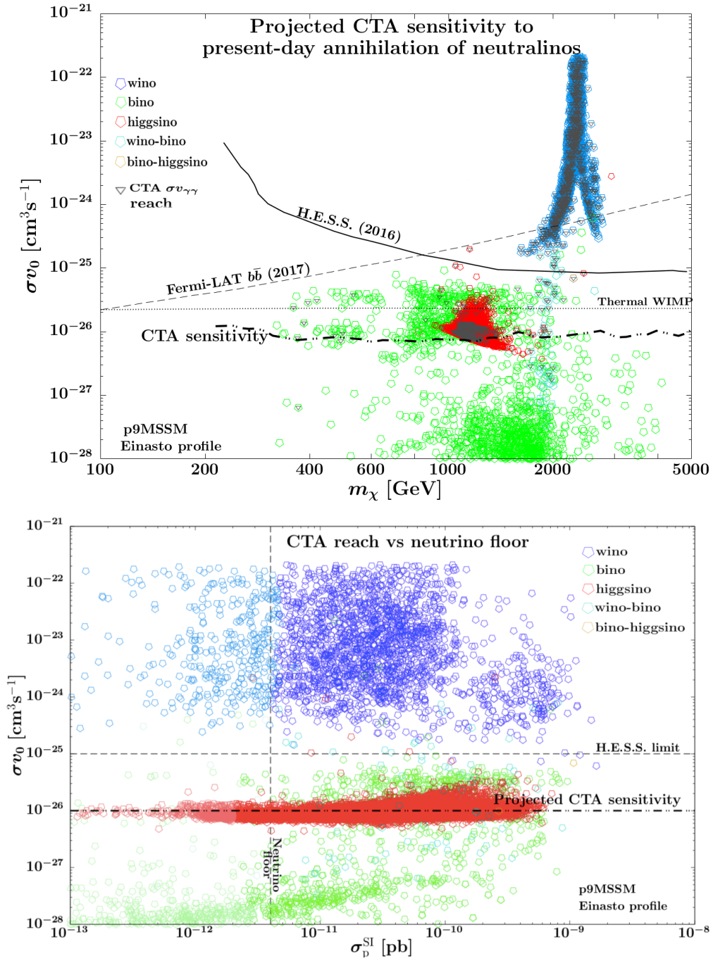
Figure 12.7: Distribution of p9MSSM points with \Delta\chi^2 \leq 5.99 for Wino (blue open dots), Bino (green open dots) and Higgsino (red open dots) and mixed Wino-Bino (cyan open dots) and Bino-Higgsino (orange open dots) models. Top panel: Distribution of p9MSSM points in the (m_\chi, \sigma v_0) space. Constraints set by Fermi-LAT [237] in the b\bar{b} annihilation channel (black dashed line) and by the measured H.E.S.S. constraints [236] (black solid line) and forecast CTA constraints on several continuum annihilation channels (black dash-dotted line) are shown. The thermal relic cross section (black dotted line) is marked on the plot. Bottom panel: Distribution of p9MSSM points in the (\sigma_p^{\text{SI}}, \sigma v_0) . The observed H.E.S.S. limits for m_\chi = 2.5 TeV and CTA projected sensitivity for m_\chi = 1 TeV are shown.
