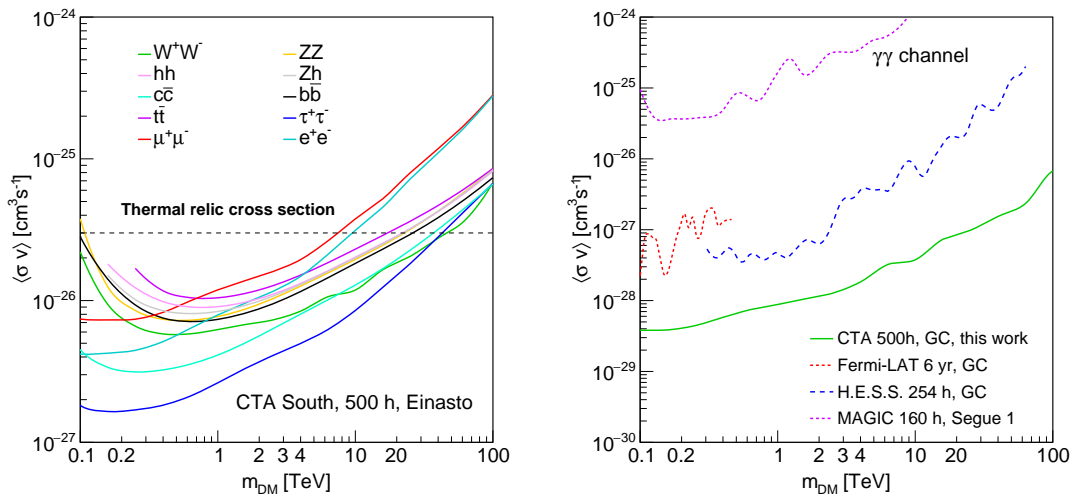
Figure 12.5: 95% C.L. forecast upper limits for CTA on \langle\sigma v\rangle as function of m_{\text{DM}} for 500 h of observations of the inner 5^\circ of the Galactic halo, assuming an Einasto profile. Left panel: The W^+W^- (green solid line), ZZ (orange solid line), Zh (gray solid line), hh (pink solid line), c\bar{c} (teal solid line), b\bar{b} (black solid line), t\bar{t} (violet solid line), e^+e^- (cyan solid line), \mu^+\mu^- (red solid line) and \tau^+\tau^- (blue solid line) annihilation channels are tested. The thermal relic cross section is marked as a black dashed line. Right panel: CTA constraints on gamma lines (green solid line), compared to those from H.E.S.S. [228] observations towards the GC (254 h, blue dashed line), Fermi-LAT [95] data in the GC region (6 years, red dotted line) and MAGIC observations of Segue 1 [232] (160 h, violet dotted line).
