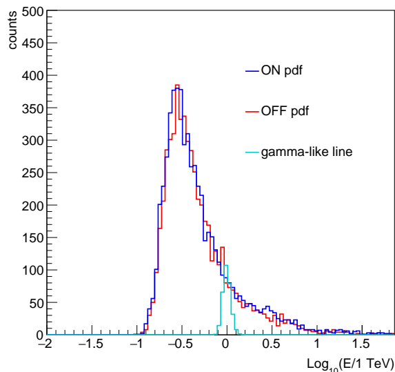
Figure 8.10: Expected DM line events distribution (cyan) for m_{\text{DM}} = 1 \text{ TeV} and \langle\sigma v\rangle = 10^{-26} \text{ cm}^3 \text{ s}^{-1} . Overlaid are the ON (blue) and OFF PDFs (red) for ROI 1.
