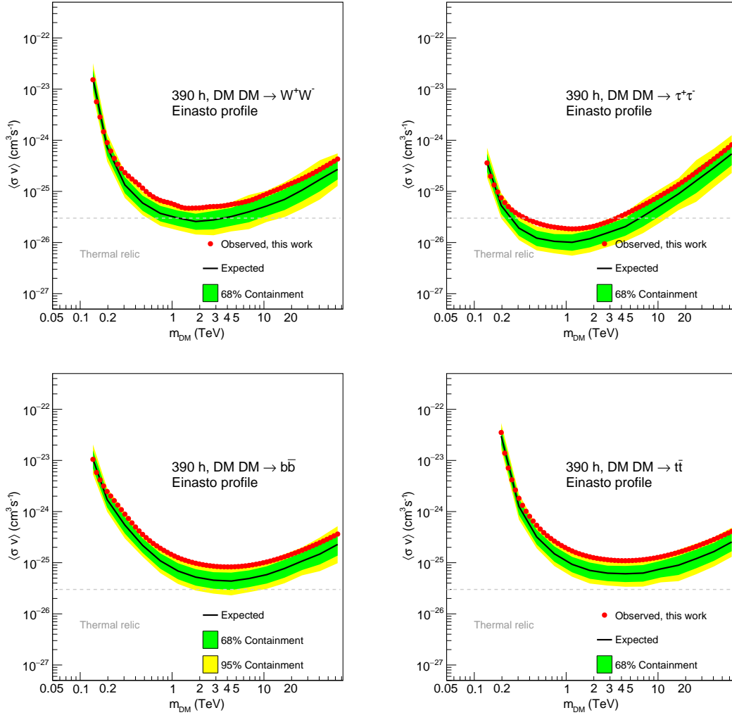
Figure 9.7: 95% C.L. H.E.S.S.-II Mono upper limits on the DM annihilation cross section in continuum channels as function of the DM mass for about 390 h of observations and assuming an Einasto DM density profile. The observed (red dots) and mean expected (solid black line) limits are given with the 1\sigma (green area) and 2\sigma (yellow area) containment bands. The bands include a 15% systematic error due to the uncertainty on the reconstructed energy. Top left panel: for the W^+W^- channel. Top right panel: for the \tau^+\tau^- channel. Bottom left panel: for the b\bar{b} channel. Bottom right panel: for the t\bar{t} channel.
