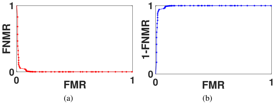
Figure 2.8: An example of a DET curve and a ROC curve. (a) represents the DET curve. (b) represents the ROC curve.
