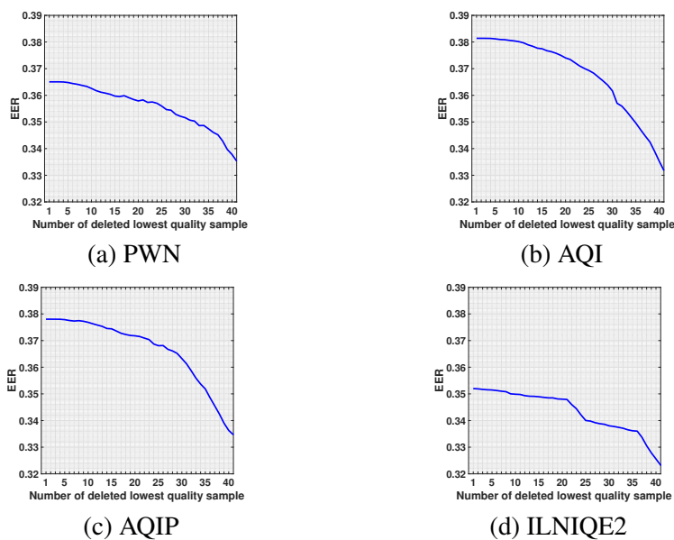
Figure 8.16: Examples of EER values with omitting low quality iris samples one by one until the best quality sample left for LFC.
