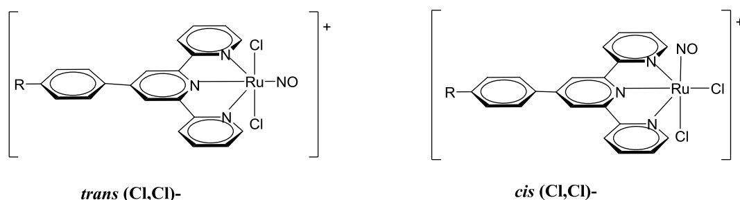
Figure I-32 : Structures des complexes [Ru(R-Phterpy)Cl 2 NO] +
