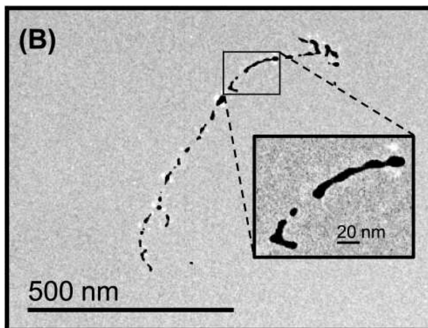
Figure 1.5: Electron-microscope image of an elongated track-shaped Ag-cluster after it is surface-deposited.
