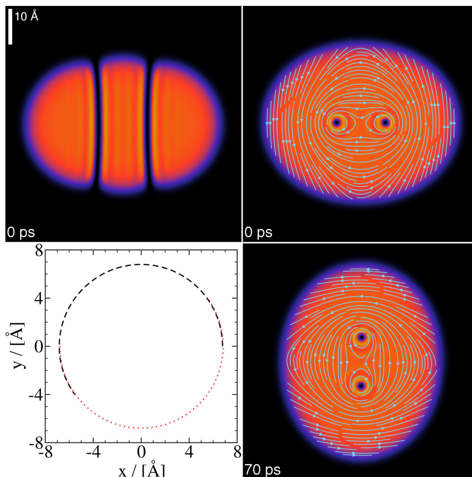
Figure 9.7: ^4\text{He}_{1000} droplet at \omega = 0.0229 \text{ ps}^{-1} : Top panels, stationary two-vortex configuration on the x - z plane (left) and x - y plane (right) in the corotating frame. Bottom left panel, trajectory of the vortex cores in the x - y plane of the laboratory frame. The dashed line is the trajectory of one of the vortex cores, and the dotted line that of the other. Both trajectories overlap and show that the vortex cores rotate rigidly and this is also visualised by the velocity field lines shown in the right two panels. Bottom right panel, helium density in the x - y plane at t = 70 ps obtained in the laboratory frame starting from the above configuration [139] .
