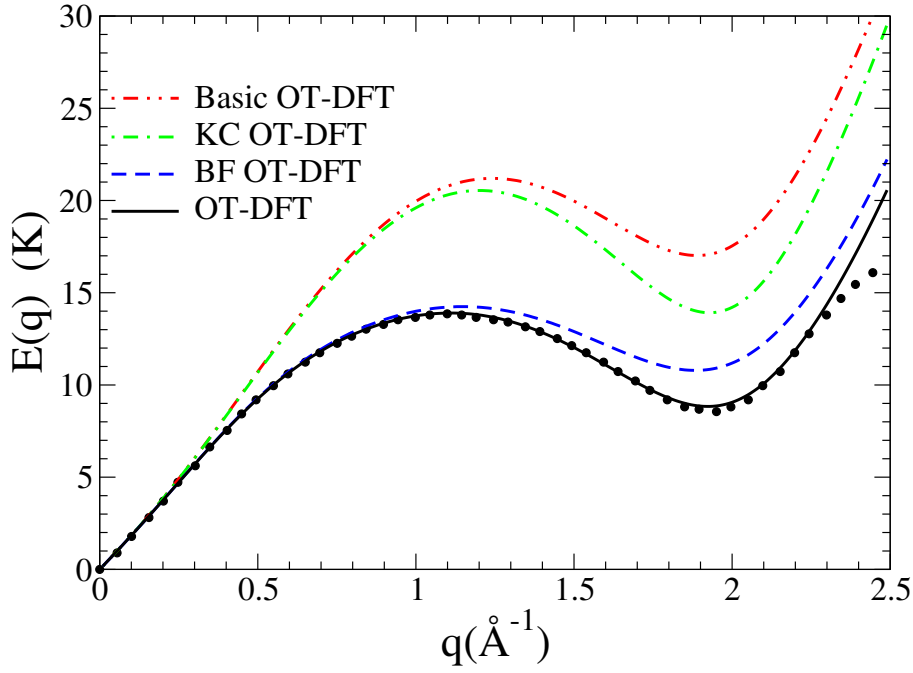
Figure 1.3: Dispersion relation for elementary excitations in liquid {}^4\text{He} calculated as in [28]. ‘Basic’ indicates the Orsay-Trento (OT) functional [29] without the non-local kinetic energy correction (KC) nor the back-flow (BF) terms; KC OT-DFT adds to the basic OT-DFT the KC term; BF OT-DFT adds to the basic OT-DFT the BF term. The dots are the experimental data from [30]. The Landau velocity v_L = E(q)/(\hbar q)|_{min} obtained for each functional is 60.3 m/s (OT-DFT); 75.1 m/s (BF OT-DFT); 94.4 m/s (KC OT-DFT); 118 m/s (basic OT-DFT); and 57.5 m/s (experiment). See also Section 2.3.
