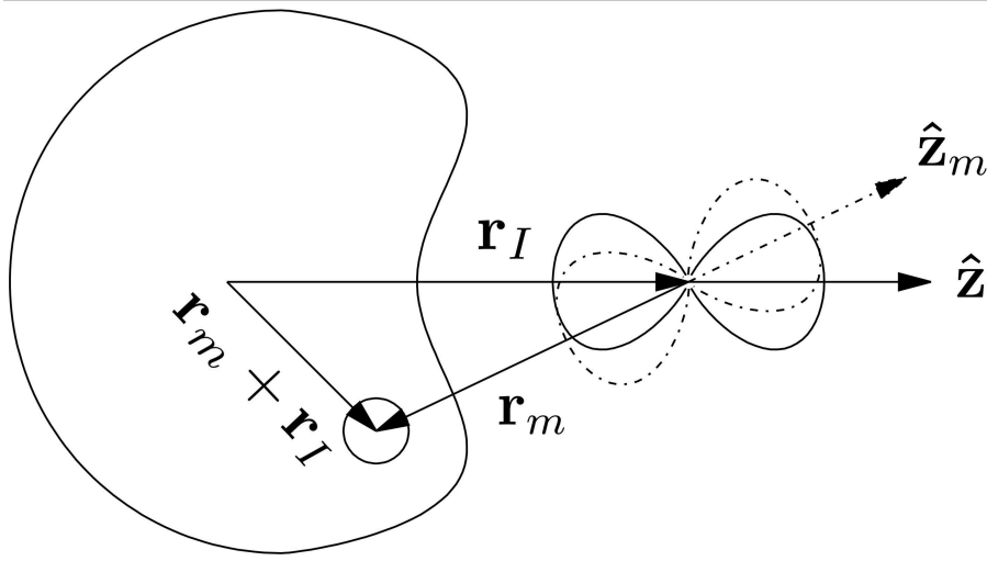
Figure 2.3: The set of axis defined in the DIM description. (Illustration courtesy of M. Martinez [61] .)
