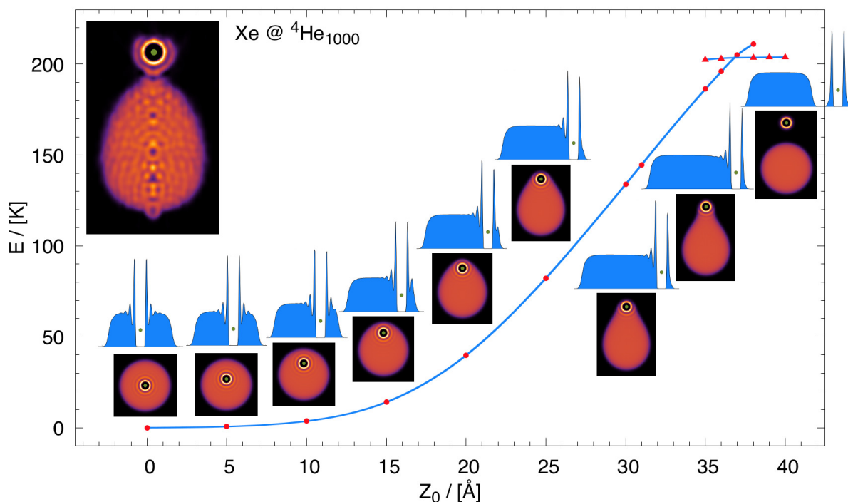
Figure 8.1: Energy of the \text{Xe}@^4\text{He}_{1000} complex as a function of the distance between the Xe atom and the COM of the droplet. Several two-dimensional helium densities and density profiles are shown for distances between 0 and 40 Å in 5 Å steps. Connected (dots) and disconnected (triangles) helium configurations are shown ( see text ). Top left inset: Snapshot of the helium density at the first turning point during the dynamic evolution of a Xe atom (green dot) at v_0 = 600 m/s attained 78 ps after it has started. (Color figure online.)
