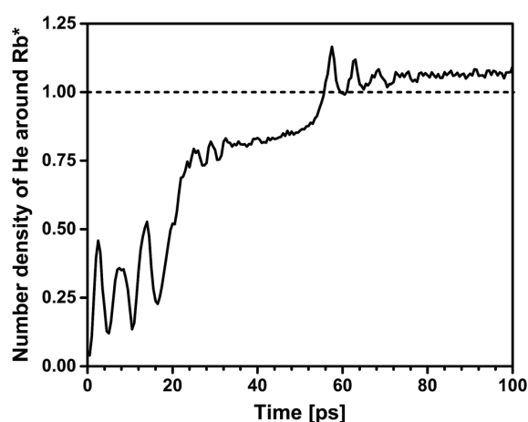
Fig. 7 Simulated time evolution of the integrated He density within an inclusion volume of radius r_{\text{incl}} = 5.7\text{ \AA} around the Rb atom excited to the 5p^2\Pi_{3/2} -state.
