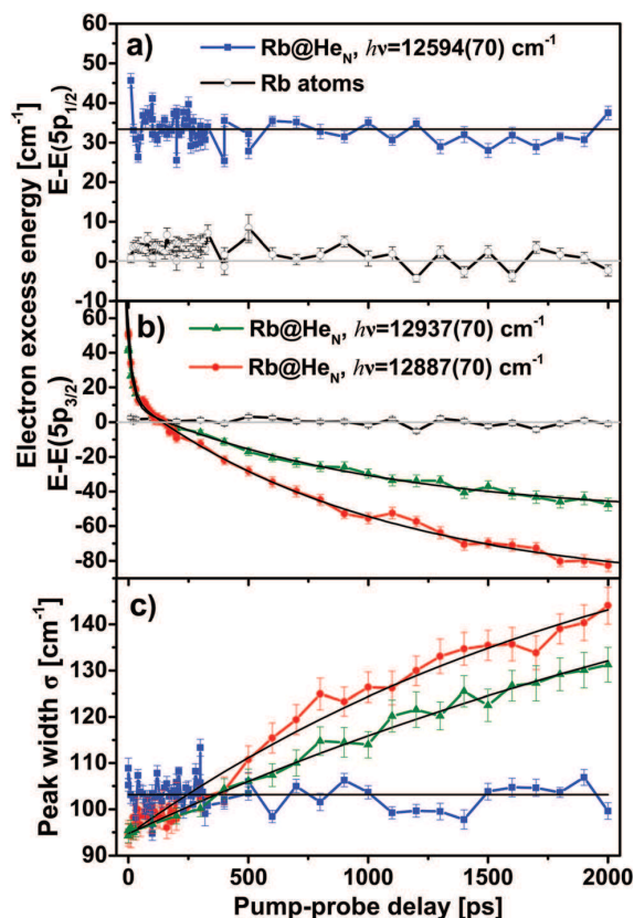
Fig. 4 Photoelectron energies as a function of pump-probe delay (filled circles) recorded at laser wavelengths \lambda = 794 nm ( 12\,594 cm ^{-1} , 5p^2\Pi_{1/2} ) (a), \lambda = 773 nm ( 12\,937 cm ^{-1} , 5p^2\Sigma_{1/2} ), and \lambda = 776 nm ( 12\,887 cm ^{-1} , 5p^2\Pi_{3/2} ) (b). Open circles indicate the electron energies measured for atomic Rb background signal. The widths of electron distributions are depicted in (c).
