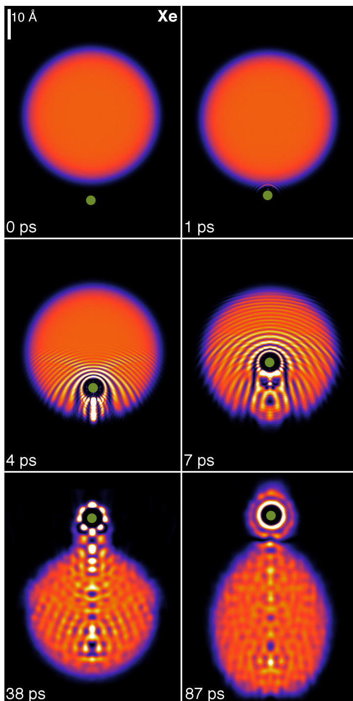
Figure 9.1: Dynamic evolution of a Xe atom (green dot) approaching the {}^4\text{He}_{1000} droplet from below at v_0 = 600 m/s. The corresponding time is indicated in each frame. Bright spots correspond to high density regions. (Reproduced from Ref. [139].)
