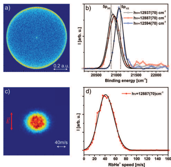
Fig. 2 Raw velocity-map images of photoelectrons (a) and of [\text{RbHe}]^+ photoions (c) recorded at \lambda = 776\text{ nm} ( 12887\text{ cm}^{-1} ) for a long pump-probe delay time of 2 ns. The red vertical arrow indicates the laser polarization. (b) Electron binding energy spectra inferred from the image shown in (a), from an image recorded at \lambda = 773\text{ nm} ( 12937\text{ cm}^{-1} ), and from an image at \lambda = 794\text{ nm} ( 12594\text{ cm}^{-1} ). (d) [\text{RbHe}]^+ photoion speed distribution inferred from (c).
