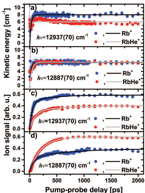
Fig. 3 \text{Rb}^+ and [\text{RbHe}]^+ ion kinetic energies [(a) and (b)] and signal yields [(c) and (d)] recorded at laser wavelengths \lambda = 773 nm [ 12\,937\text{ cm}^{-1} , (a) and (c)] and \lambda = 776 nm [ 12\,887\text{ cm}^{-1} , (b) and (d)]. The smooth gray and black lines are fit curves (see text for details).
