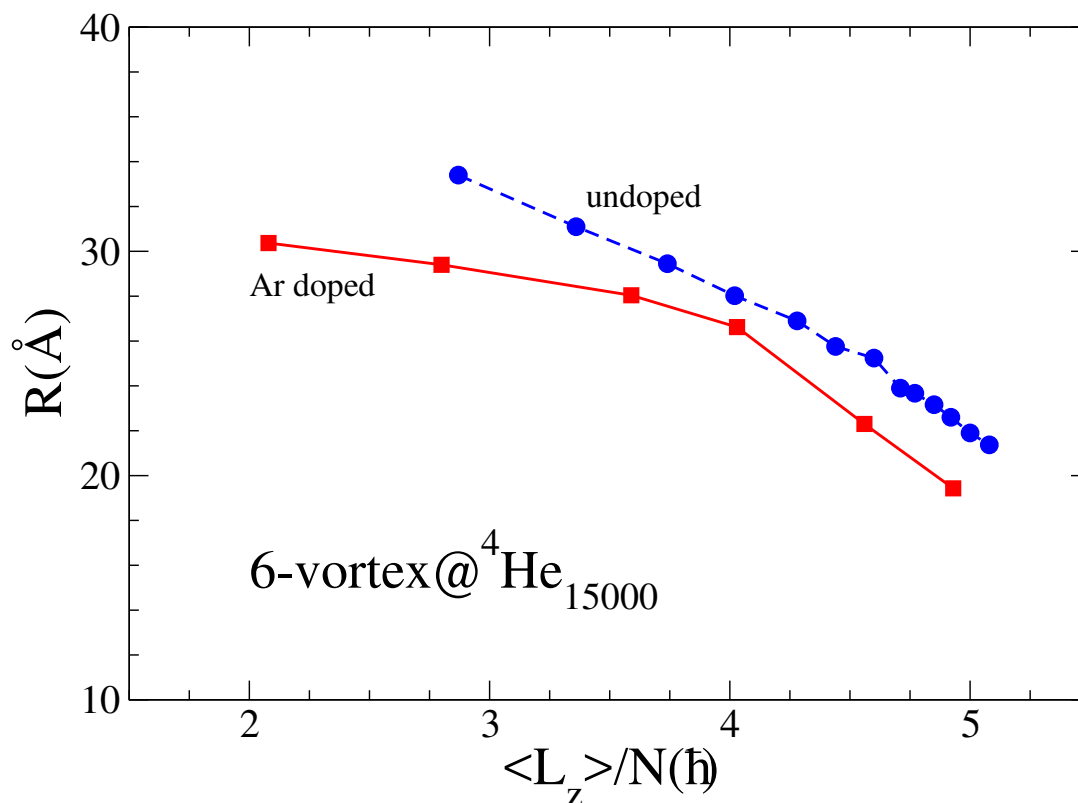
Figure 7.4: Calculated equilibrium distance of the 6-vortex ring from the droplet center as a function of the angular momentum per He atom in units of \hbar . The dots represent the results for undoped vortices, while the squares are the results for Ar-doped vortices. The lines are drawn as a guide to the eye.
