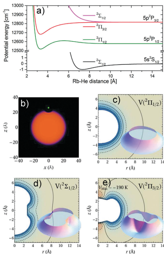
Fig. 1 (a) Rb-He pair potentials used in this work. 51 The potentials correlating to the Rb excited 5p^2P -state are split due to spin-orbit coupling. (b) Equilibrium dimple configuration of Rb in the ground state in the x - z -plane (represented by a green dot). Panels (c)–(e) display the two-dimensional Rb-He potential surfaces in cylindrical coordinates (r, z) corresponding to this configuration, with the Rb atom located at the origin. Regions where the potentials are attractive (repulsive) are represented in pink (blue). The outermost equidensity line corresponds to zero potential. Notice that in panel (e) the 5p^2\Pi_{3/2} potential presents two deep minima of about 190 K on the z -axis. The 5p^2\Pi_{1/2} and 5p^2\Sigma_{1/2} potentials [(c) and (d)] have shallow attractive minima of about 1 K depth at a distance of \sim 10 \text{ \AA} , not represented in the figure. Reprinted from Int. Rev. Phys. Chem. , 2017, 36 , 621–707 with permission from Taylor & Francis Ltd, http://www.tandfonline.com .
