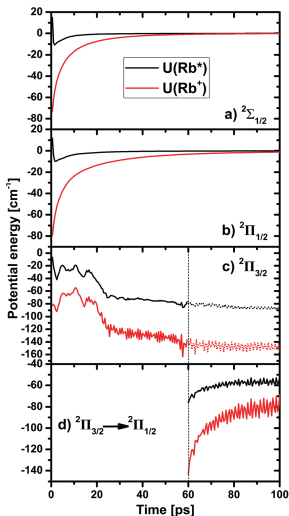
Fig. 9 (a)–(c) Simulated interaction energies of the Rb-atom excited into various states interacting with the surrounding He distribution (black lines), and of the \text{Rb}^+ ion for the same instantaneous geometry (red lines). In (d), the excited state of Rb is suddenly switched from ^2\Pi_{3/2} to ^2\Pi_{1/2} to simulate the dynamics initiated by spin-relaxation.
