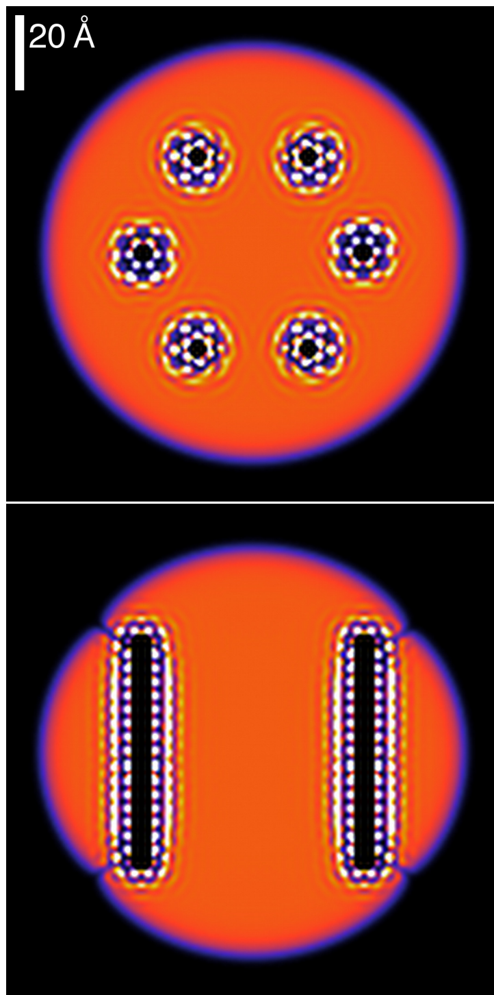
Figure 7.3: Helium droplet configuration hosting six vortices, each doped with a line of regularly spaced Ar atoms (not represented). The top figure shows the density in the x-y symmetry plane (top view), while the bottom figure shows a side view corresponding to the y-z plane. As in some of the previous figures, the bright spots are high density blobs appearing around the impurity atoms.
