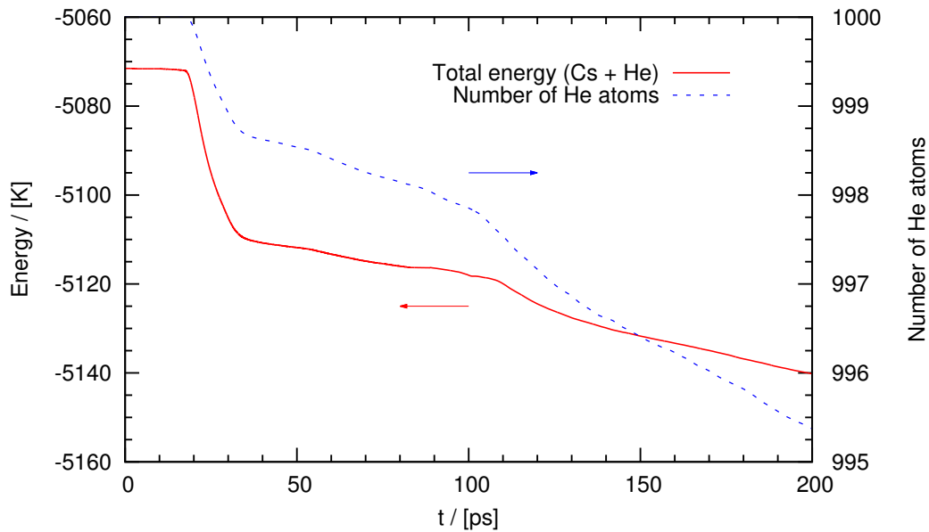
Figure 8.5: Total energy (left scale) and number of atoms in the droplet (right scale) as a function of time for the Cs@ 4 He 1000 system at v_0 = 200 m/s. (Color figure online.)
