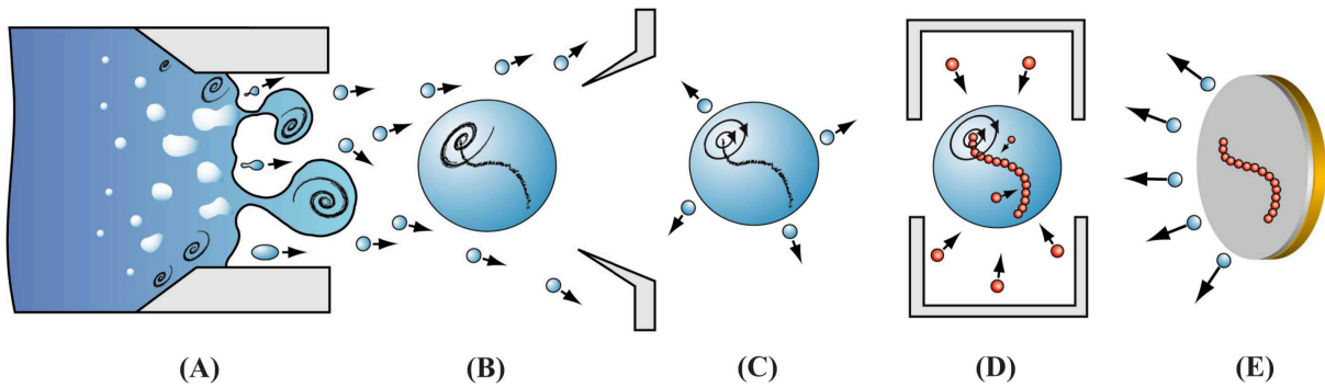
Figure 7.1: Schematic of the experiment. (a) He fluid expands in vacuum and (b) breaks up into rotating droplets. (c) A quantum vortex is formed as a consequence of fast evaporative cooling of the droplet to below T_\lambda . (d) The droplet is doped with Ag atoms, which are attracted to the vortex core. (e) The droplet then collides with the carbon surface leaving behind the Ag trace, whereas the He evaporates. (Illustration courtesy of Gomez et al. 2012, see Ref. [103])
