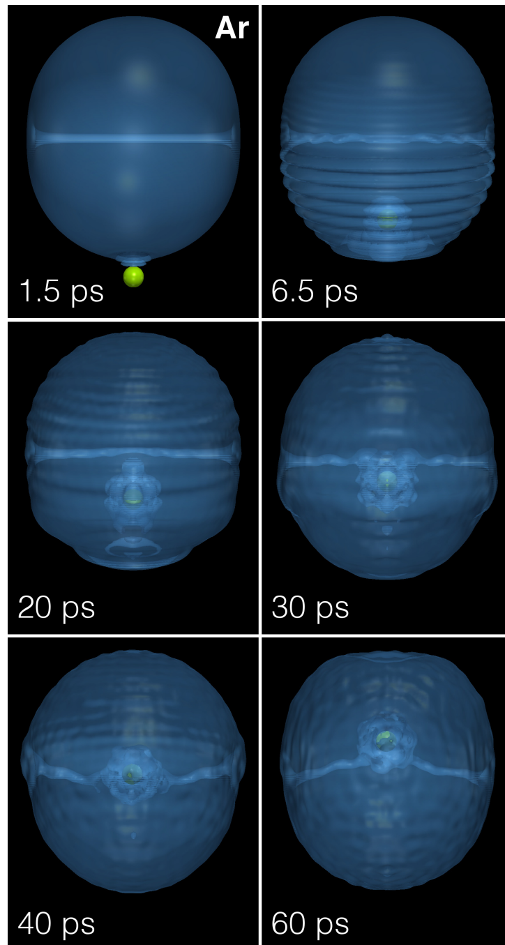
Figure 9.10: Same as Figure 4 for an Ar atom at v_0 = 360 m/s [139] .
