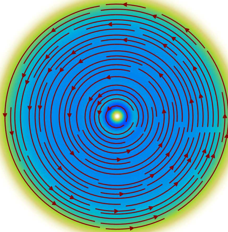
Figure 1.4: Cross section of a ^4\text{He} droplet through a symmetry plane. The droplet is made of 1000 atoms. Superimposed are the streamlines of the velocity field \mathbf{v}_s for s = 1 . They are concentric circles, centred around the vortex core along the z -axis. The colour scale represents the number density \rho(r) where bluer means a higher value. The radius of the droplet is about 22 \text{ \AA} .
