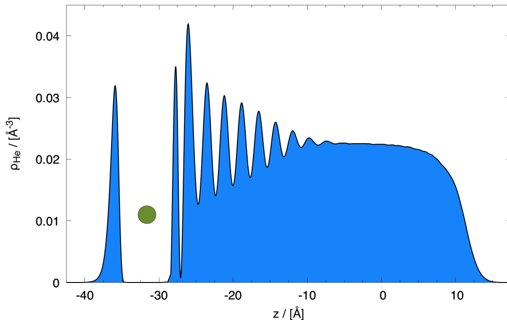
Figure 8.4: Density profile of the \text{He}_{1000} droplet along the incident direction corresponding to the Xe collision at v_0 = 200 m/s after 6 ps. (Color figure online.)
