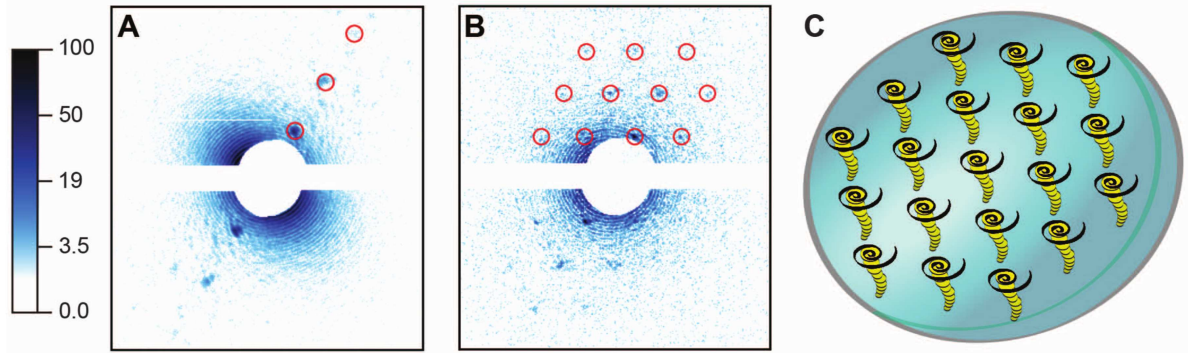
Figure 7.2: He droplets doped with Xe atoms. (A and B) X-ray diffraction images of doped droplets, displayed in a logarithmic intensity scale. (C) Droplet and embedded Xe clusters. Images in (A) and (B) correspond to tilted and parallel alignments of the vortex axes with respect to the incident x-ray beam, respectively. (Illustration courtesy of Gomez et al. 2014, see Ref. [104])
