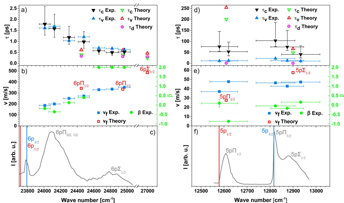
Figure 3. Experimental and theoretical fall-back time constants \tau_c (a,d), velocity rise times \tau_v (a,d), theoretical Rb* desorption times \tau_d (a,d), Rb + final most probable speeds \hat{v}_f (b,e), and anisotropy parameters \beta (b,e) for different excitation wavenumbers corresponding to droplet perturbed Rb states 6p (left column) and 5p (right column). Panels c and f show fluorescence emission spectra as reference. 25,38 Vertical lines indicate free atomic transitions.
