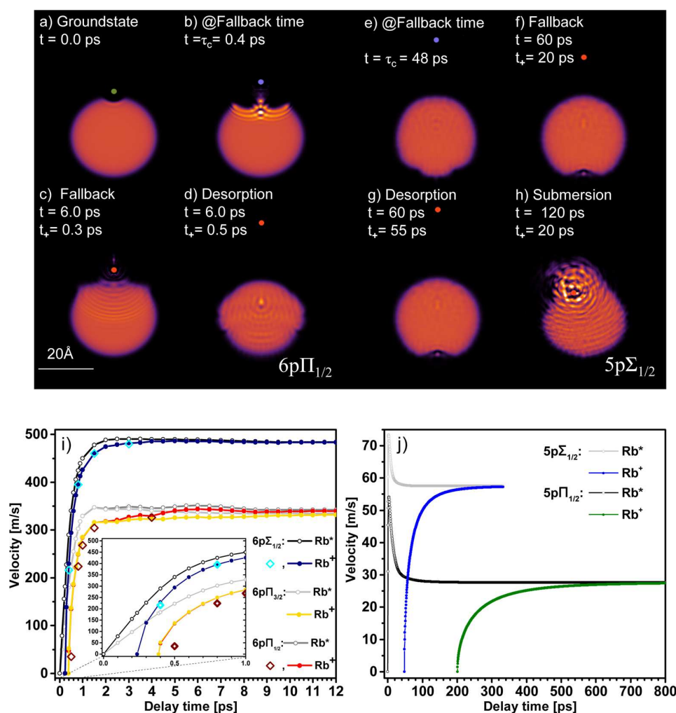
Figure 2. TDDFT-based 2D densities (a–d,e–h) and velocities (i,j) of Rb atoms attached to He_{1000} excited from equilibrium (a) to droplet perturbed 6p (left column) and 5p (right column) states. Configurations are shown for different propagation times t and ionization times t_+ : (b,e) neutral Rb at fall-back time t = \tau_c ; (c,f) t_+ < \tau_c fall-back of Rb^+ ion; (d,g) t_+ > \tau_c desorption of Rb^+ ; (h) solvation of Rb^+ ; (i,j) evolution of Rb^* velocities with time t (gray open dots), and final velocities of Rb^+ (colored filled dots) as a function of t_+ .
