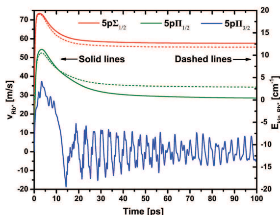
Fig. 6 Velocity (solid lines, left scale) and kinetic energy (dashed lines, right scale) of the Rb atom excited to the 5p-state as a function of time. The kinetic energy of the 5p^2\Pi_{3/2} -state is not given as this state remains bound to the droplet.
