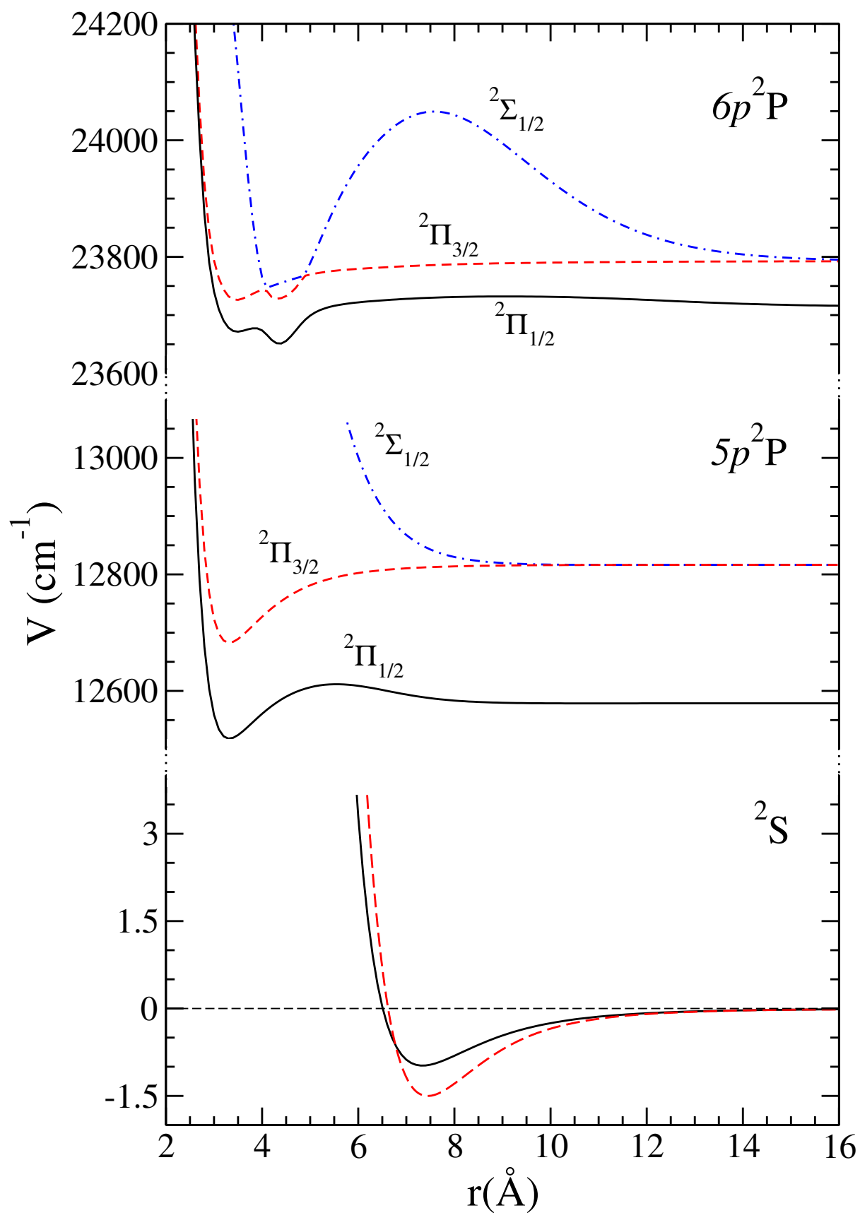
Figure 5.1: ^2S , 5p^2P , and 6p^2P Rb-He pair potentials used in this work. The splitting introduced by the spin-orbit interaction has been included. The ^2S He-Rb pair potential of Ref. [99] is also displayed (bottom dashed line).
