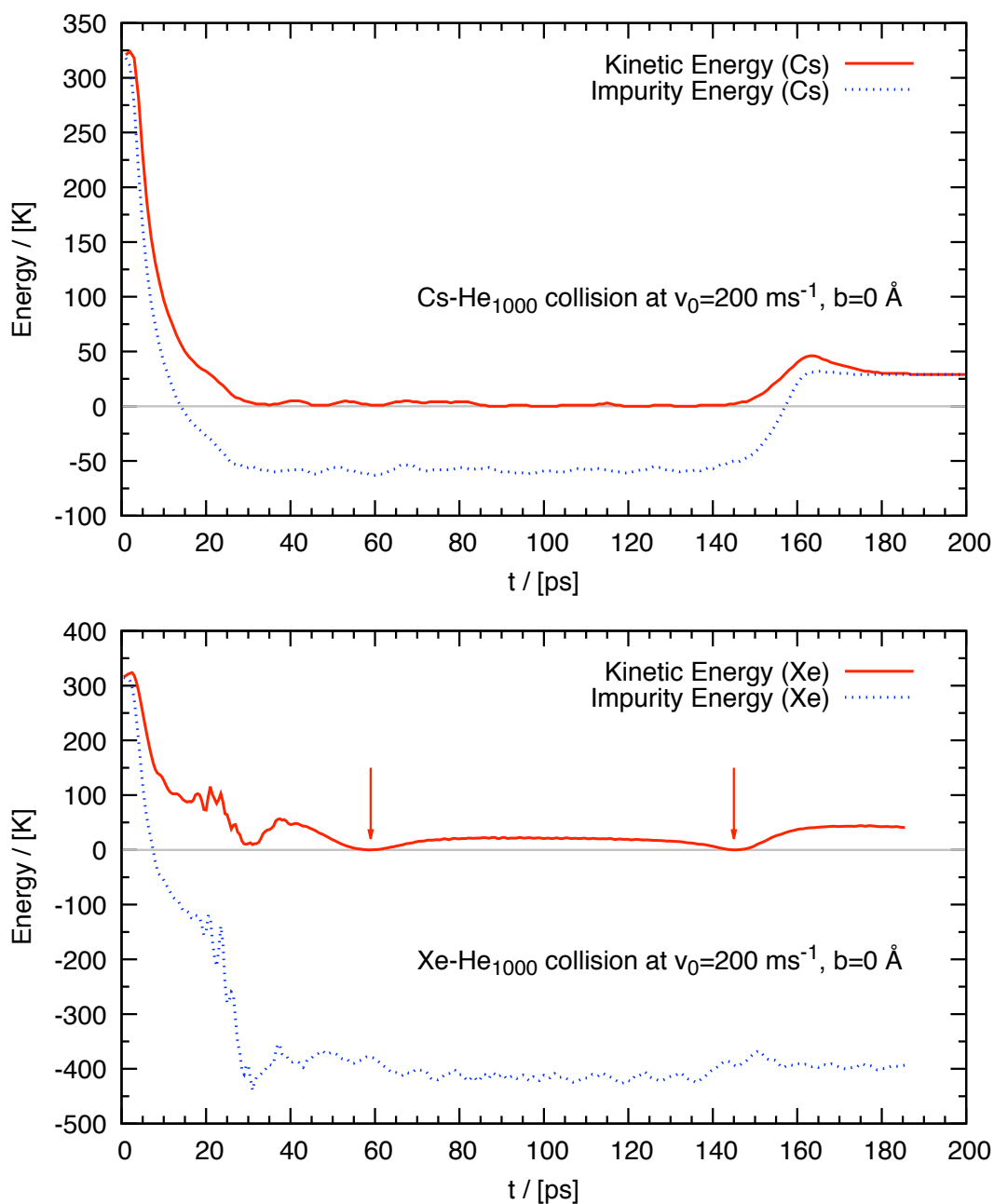
Figure 8.3: Top figure: Kinetic and total (kinetic plus potential) energy as a function of time of a Cs atom head-on colliding against a ^4\text{He}_{1000} droplet at v_0 = 200 \text{ m/s} . Bottom figure: same as top figure for a Xe atom. The vertical arrows indicate the first two turning points at 59 and 145 ps, whose corresponding helium densities are shown in the right Figure 8.2. (Color figure online.)
