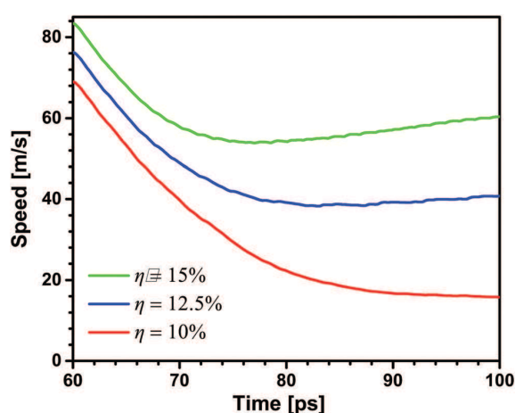
Fig. 8 Velocity of the excited Rb atom with attached He density as a function of time after 5p^2\Pi_{3/2} \rightarrow 5p^2\Pi_{1/2} relaxation at \Delta t = 60\text{ ps} for various values of the energy conversion factor \eta .
