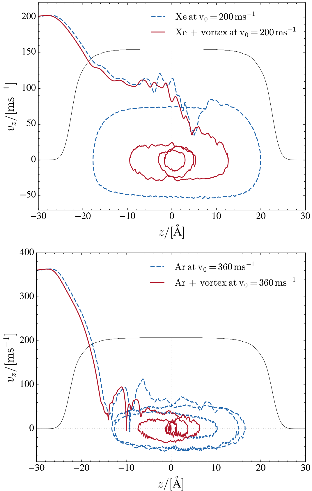
Figure 9.3: Top: Phase-space trajectory of Xe for a head-on collision at v_0 = 200 \text{ m/s} against a {}^4\text{He}_{1000} droplet with and without a vortex line. The Xe atom is referred to the COM frame of the droplet. Bottom: Same as top panel for Ar at v_0 = 360 \text{ m/s} . The droplet density at t = 0 is also represented in arbitrary scale (black profile)
