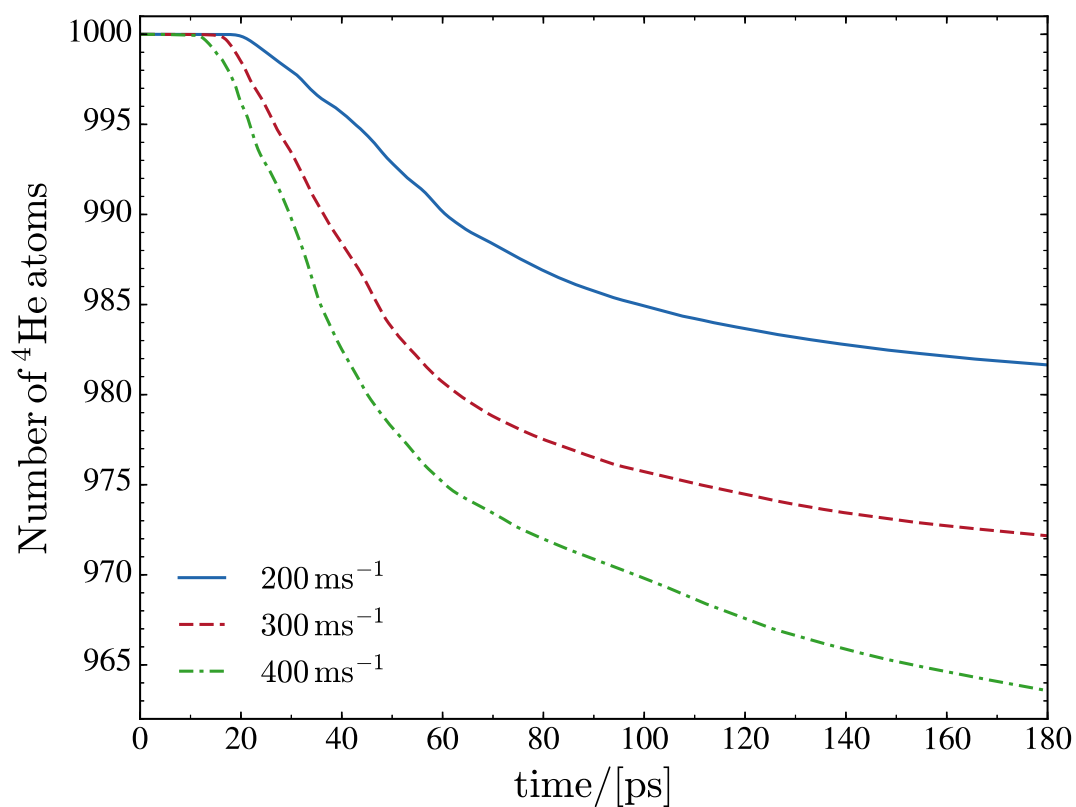
Figure 9.4: Number of He atoms remaining in the droplet as a function of time for the Xe against {}^4\text{He}_{1000} collision at v_0 = 200, 300 and 400\text{ m/s} .
