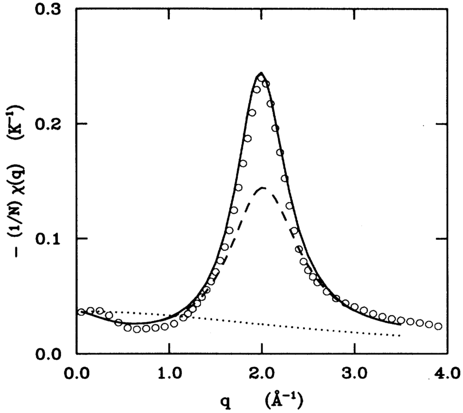
Figure 2.1: Static response -\chi (see Ref. [29], Eqn. (11)) per atom of liquid {}^4\text{He} at zero pressure. Points: experimental data; dotted line: from the functional of Refs. [51, 52]; dashed line: Orsay-Paris (OP) functional [57] ; solid line: OT functional.
