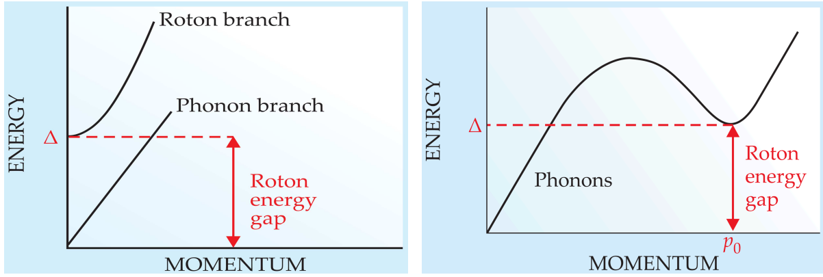
Figure 1.2: Left: Lev Landau’s 1941 energy dispersion curve [22] for the excitations in liquid helium below T_\lambda . It exhibits a phonon- and a roton branch. The slope of the linear phonon branch corresponds to the velocity of sound. Right: Lev Landau’s 1947 modified dispersion curve. The roton-branch is no longer a separate excitation branch but rather an extension of the phonon-branch. (Illustration courtesy of R.J. Donnelly [10] )
