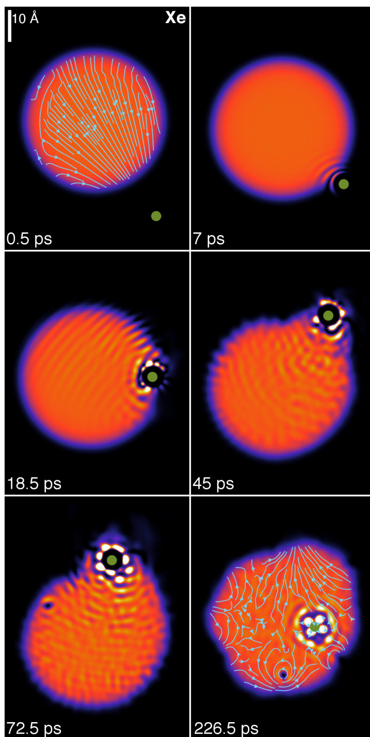
Figure 9.5: Dynamic evolution of a Xe atom (green dot) approaching the ^4\text{He}_{1000} droplet from below at v_0 = 200 m/s with impact parameter b = 20.3 Å. The corresponding time is indicated in each frame. The velocity fields are represented in cyan in the panels at 0.5 ps and 226.5 ps. The bright spots are high He density blobs appearing around the Xe atom because of the attractive He-Xe interaction. See the ESI [139] for the movie of the complete evolution.
