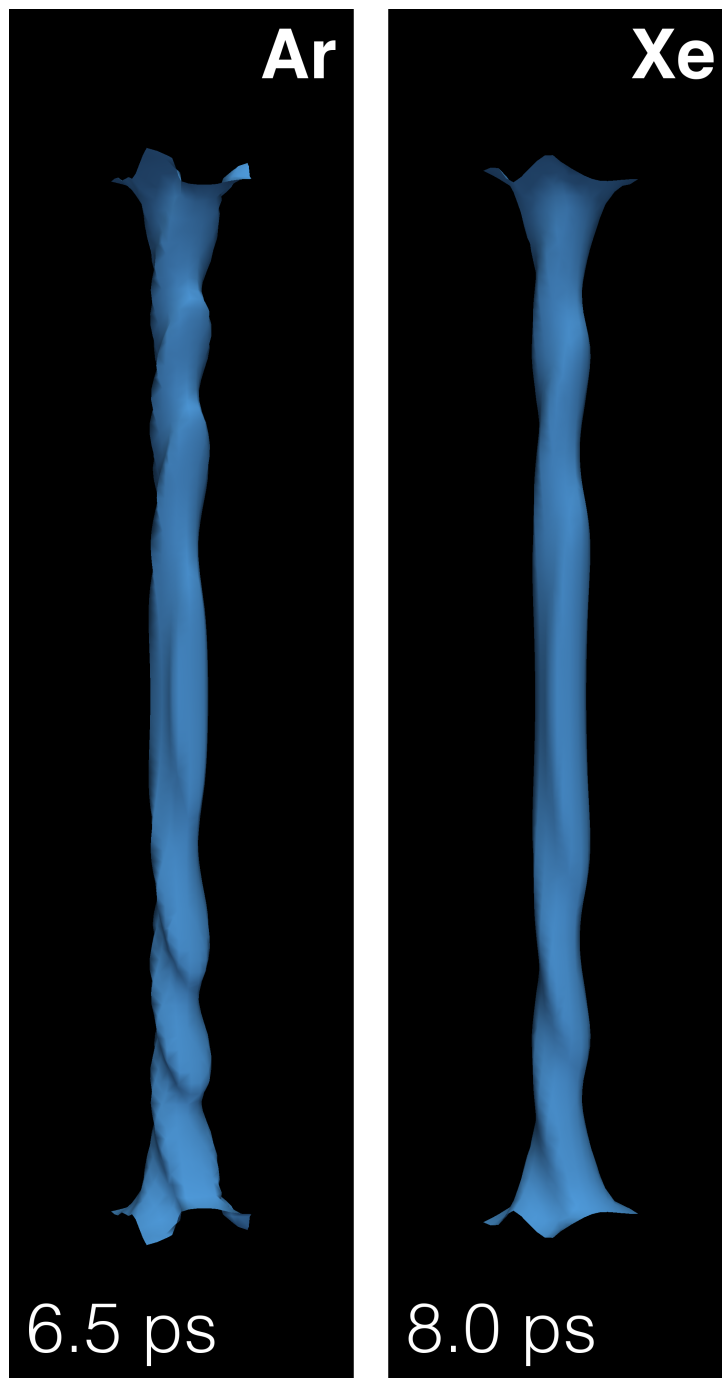
Figure 9.11: Core structure of the vortex line in a {}^4\text{He}_{1000} droplet after colliding with Xe at v_0=200 m/s (right panel, t = 8 ps) and Ar at 360 m/s (left panel, t=6.5 ps). The full structure of the droplet is shown in Figure 4 and Figure 9.10.
