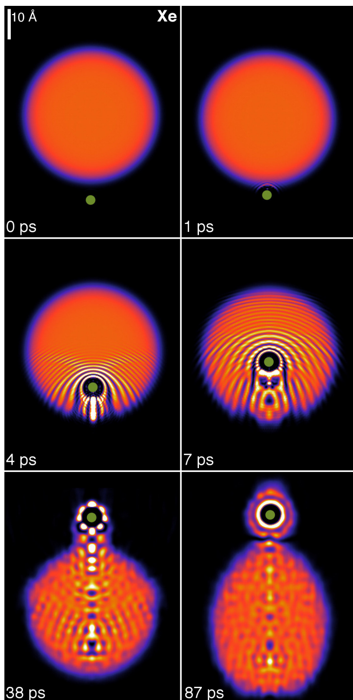
Figure 9.1: Dynamic evolution of a Xe atom (green dot) approaching the ^4\text{He}_{1000} droplet from below at v_0 = 600 m/s. The corresponding time is indicated in each frame. Bright spots correspond to high density regions. (Reproduced from Ref. [139].)
