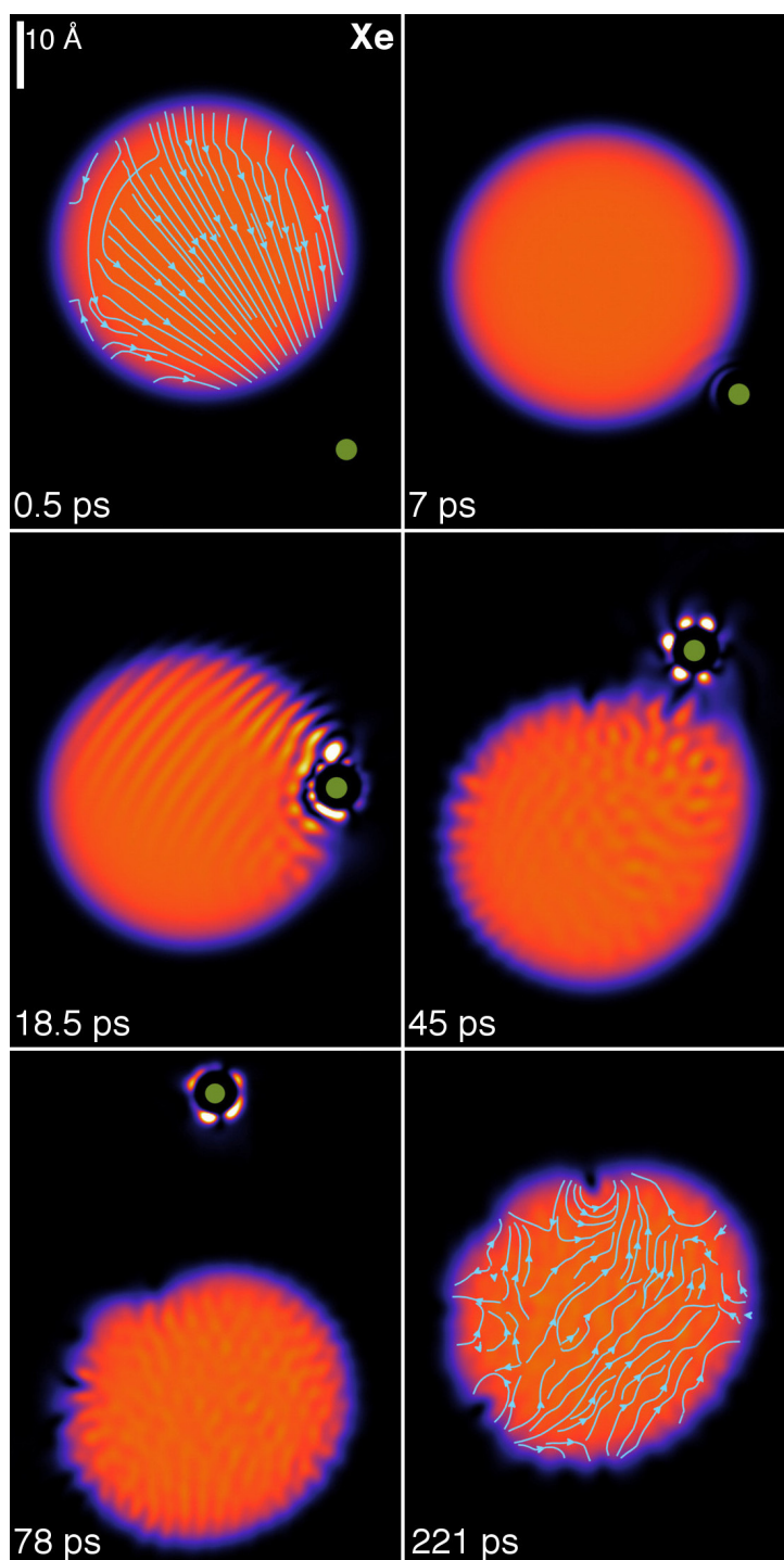
Figure 9.6: The same process as in Figure 9.5 but with an impact parameter b = 22.2 \text{ \AA} instead of b = 20.3 \text{ \AA} . Note that in this case, after about 78 ps (bottom left panel), the Xe atom is ejected with some helium density attached to it. See the ESI [139] for the movie of the complete evolution.
