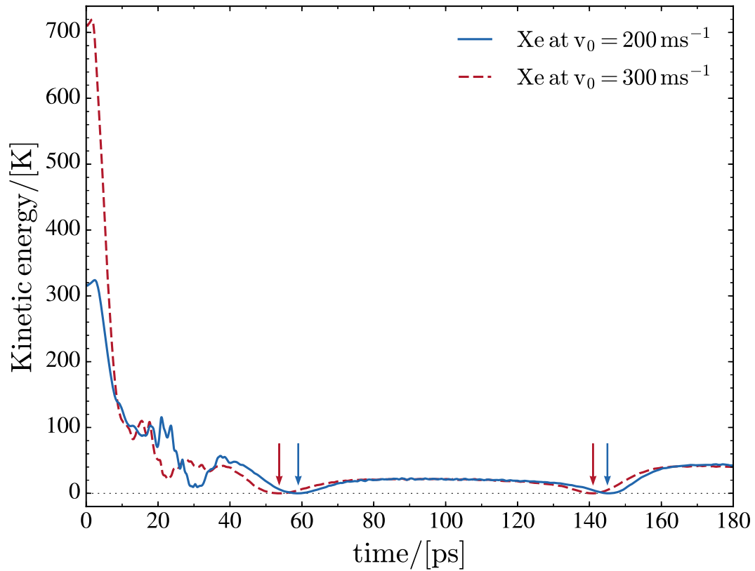
Figure 9.2: Kinetic energy of the Xe atom in the center of mass (COM) frame of the {}^4\text{He}_{1000} droplet as a function of time for a head-on collision at v_0 = 200 and 300 \text{ m/s} . The kinetic energy increase during the first few picoseconds is due to the acceleration produced by the attractive part of the Xe-He potential. The vertical arrows indicate the first two turning points inside the droplet.
