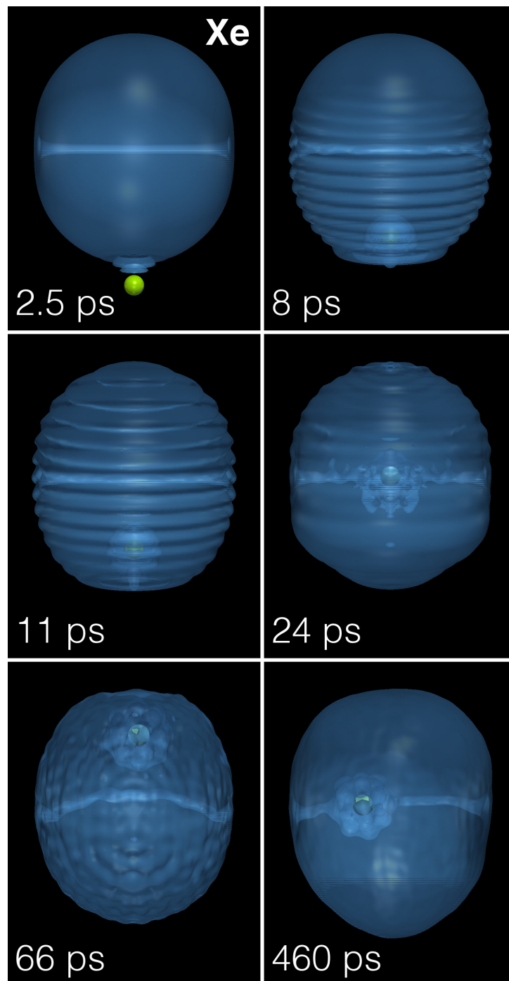
Figure 9.9: Dynamic evolution of a Xe atom (green dot) approaching a {}^4\text{He}_{1000} droplet hosting a vortex line from below at v_0 = 200 m/s. The corresponding time is indicated in each frame [139] .
