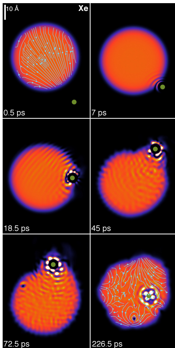
Figure 9.5: Dynamic evolution of a Xe atom (green dot) approaching the {}^4\text{He}_{1000} droplet from below at v_0 = 200 m/s with impact parameter b = 20.3 Å. The corresponding time is indicated in each frame. The velocity fields are represented in cyan in the panels at 0.5 ps and 226.5 ps. The bright spots are high He density blobs appearing around the Xe atom because of the attractive He-Xe interaction. See the ESI [139] for the movie of the complete evolution.
