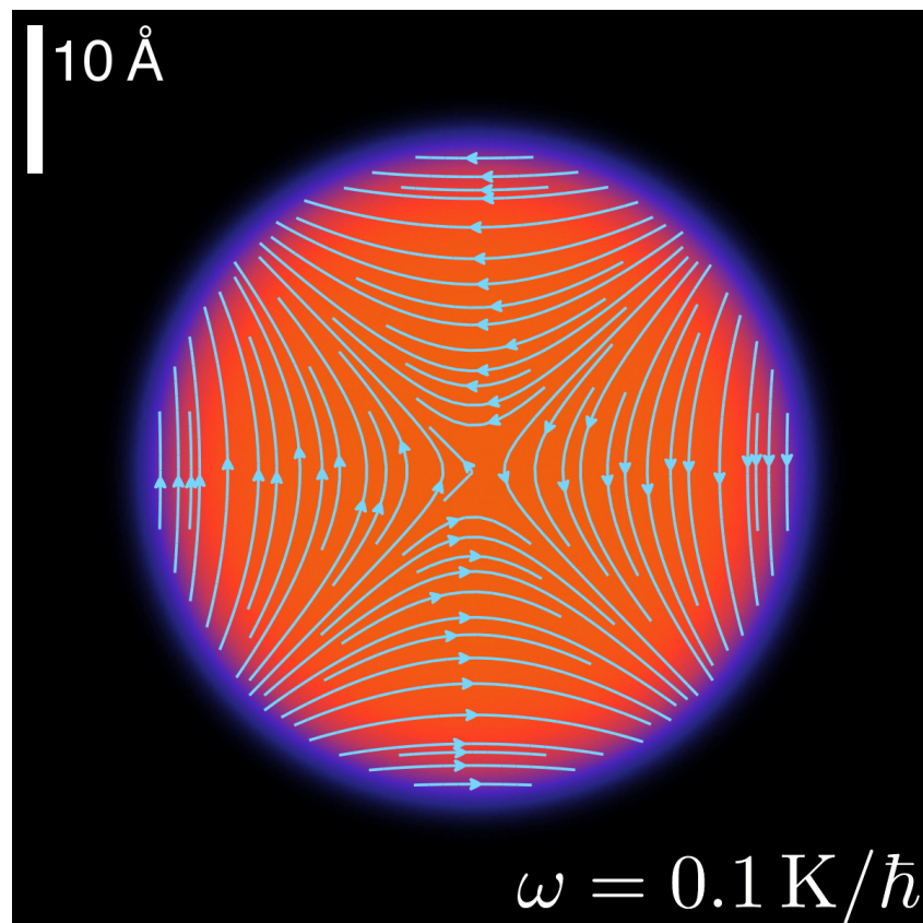
Figure 9.8: Stationary configuration of the {}^4\text{He}_{1000} droplet at \omega_c \gtrsim \omega = 0.10 \text{ K}/\hbar = 0.0131 \text{ ps}^{-1} in the corotating frame ( x-y plane). Superimposed is the irrotational velocity field arising from a velocity potential of the form S(\mathbf{r}) = \alpha xy .
