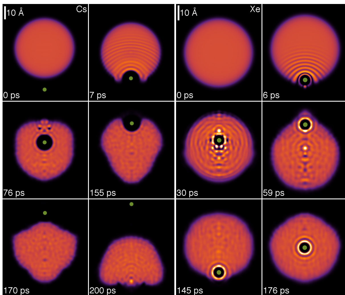
Figure 8.2: Right panel: Dynamic evolution of a Xe atom (big dot) approaching the {}^4\text{He}_{1000} droplet from below at v_0 = 200 m/s. The corresponding time is indicated in each frame. Left panel: Same as the right panel, but for a Cs atom. (Color figure online.)
