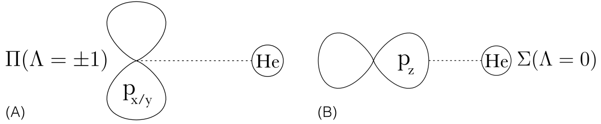
Figure 2.2: Level splitting of the p-orbitals in the presence of helium, that breaks the spherical symmetry. (A) A double degenerate n'p_{x/y} -orbital and (B) a single n'p_z -orbital. (Illustration courtesy of M. Martinez [61] .)
