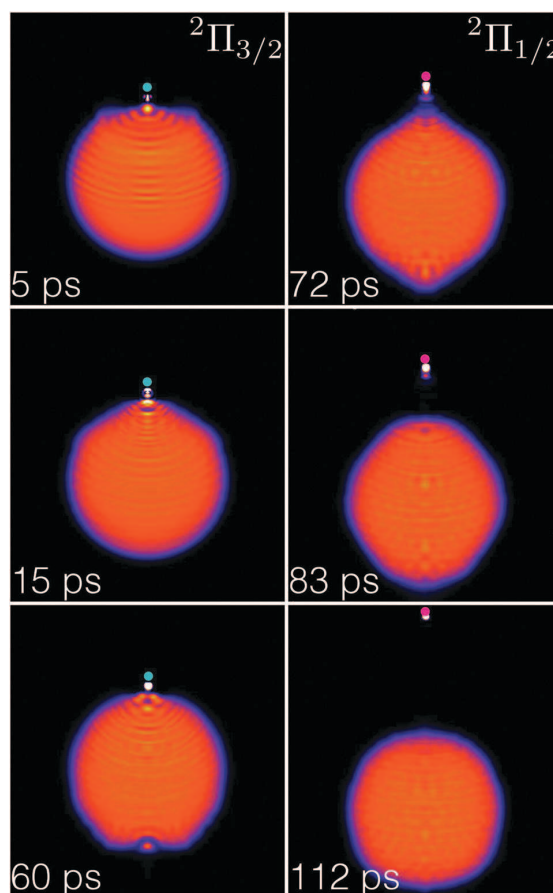
Fig. 5 Snapshots of the He density during the evolution of the excited RbHe 1000 complex for \eta = 15\% , \Delta t = 60 \text{ ps} . The green dot represents the Rb atom excited into the 5p^2\Pi_{3/2} -state; the magenta dot is the Rb atom after suddenly relaxing to the 5p^2\Pi_{1/2} -state. The white spot accompanying the green or magenta dot representing the Rb atom depicts the He density carried away with it.
