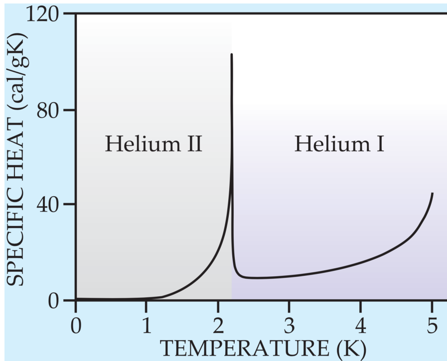
Figure 1.1: The specific heat of ^4\text{He} as a function of the temperature. There is a clearly visible singularity around 2.2 K and the graph itself has the distinct \lambda -like shape that inspired [9] Willem and Anna Keesom to call the temperature at which the singularity occurs the “ \lambda -point”. (Illustration courtesy of R.J. Donnelly [10] )
