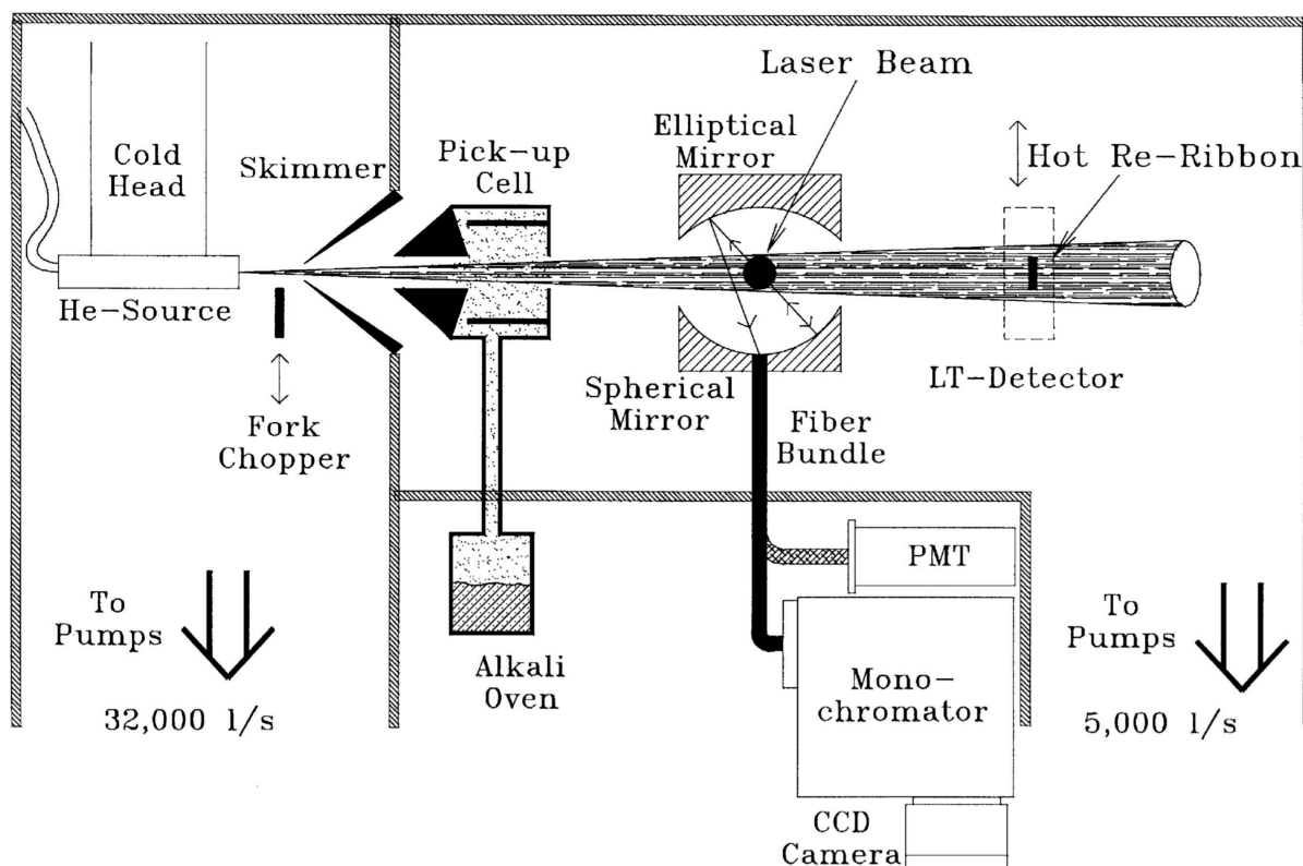
Figure 3.1: Principle of an alkali-doped helium nanodroplet experiment from Ref. [96]
