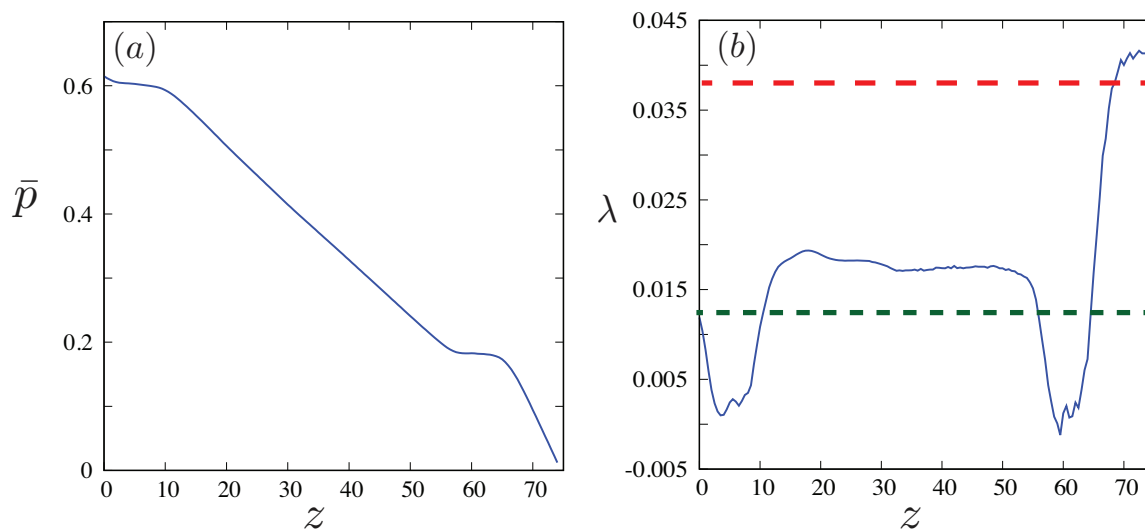
Figure 6.4: (a) Mean value of pressure \bar{p} along the axial direction. (b) Skin friction factor \lambda along the streamwise direction (dark line). Small and large dotted line correspond to friction factor for laminar flow and fully-developed turbulent flow (Blasius). 80 000 data samples from four probes around the near wall region were used to obtain the time average.
