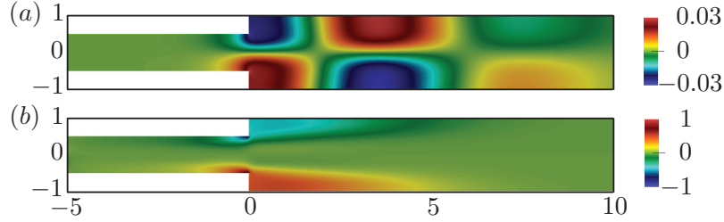
Figure 2.7: Contour plot of pressure at Re_c = 143 . (a) Direct mode, (b) adjoint mode. Only 10d out of 35d is shown.
