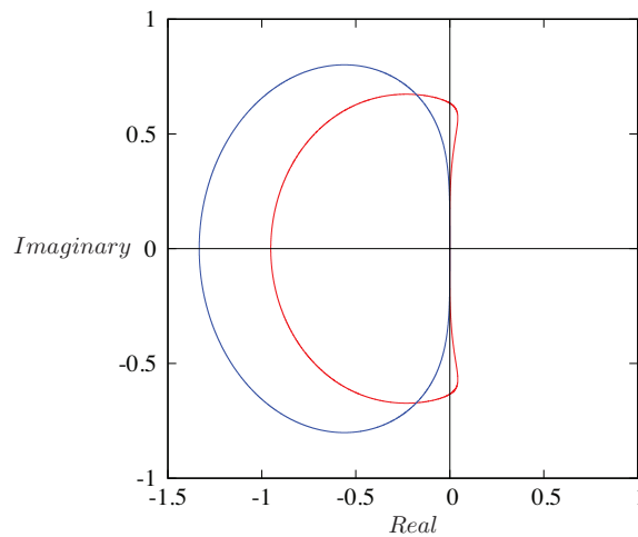
Figure 3.3: Stability regions of BDF k /EXT k methods. Red line and blue line corresponds to BDF3/EXT3 and BDF2/EXT2 respectively.
