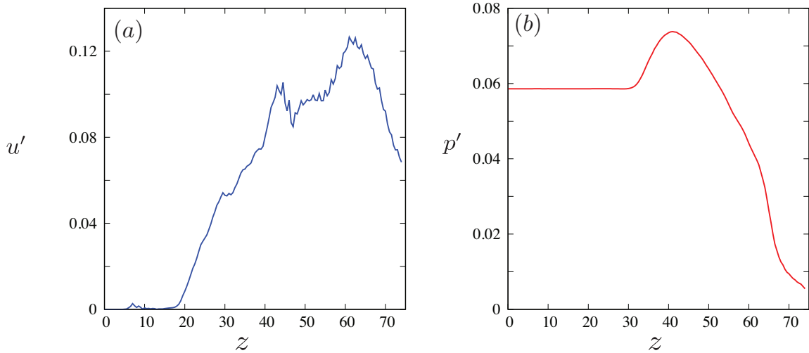
Figure 6.6: Standard deviation of fluctuations obtained using 80 000 samples of (a) velocity (b) pressure respectively.
