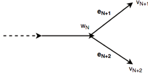
Figure 16: the internal vertex w_N is connected with the two external vertices v_{N+1} and v_{N+2} .
