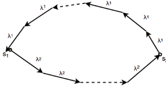
Figure 20: The graph \Gamma'_b .
