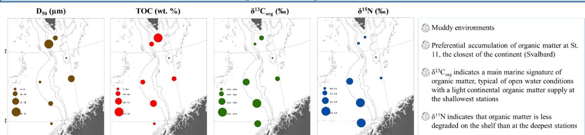
Figure 3: Bubble points representing the surface values of major environmental parameters (grain size D 50 , total organic carbon TOC, δ 13 C org and δ 15 N).
