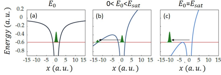
Figure 2.1: Potential felt by an electron in argon, I_p = 15.76 \text{ eV} = 0.58 \text{ a.u.} , in the absence of an electric field (a), in the presence of a field E_0 = 0.04 \text{ a.u.} ( I = 5.5 \times 10^{13} \text{ W/cm}^2 ) (b) and in the presence of a field at the saturation illumination of argon E_0 = E_{sat} = 0.084 \text{ a.u.} ( I = 2.4 \times 10^{14} \text{ W/cm}^2 ) (c). Adapted from Ref. [Barreau, 2017].
