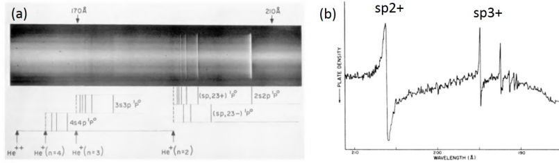
Figure 6.7: Absorption spectra of helium where the asymmetric line shapes of autoionization resonances are visible: (a) taken from Ref. [Madden and Codling, 1965] and (b) from Ref. [Madden and Codling, 1963].
