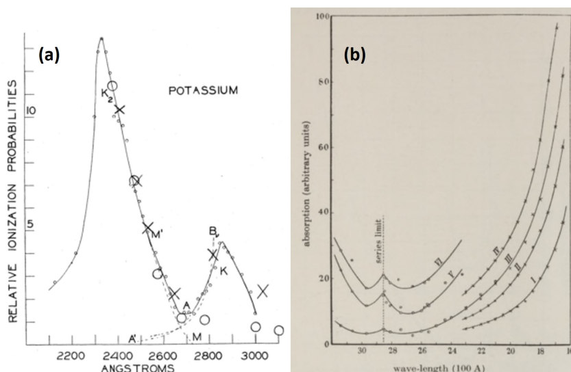
Figure 7.1: (a) [Lawrence and Edlefsen, 1929]: The ionization per unit light intensity B_v as a function of the wavelength. The small circles represent the data of the reported experiments. The large circles represent earlier observations by Lawrence, and the crosses Williamson's data [Williamson, 1923]. (b) [Ditchburn, 1943]: Absorption curves in the vapor-pressure range 1.6-8.5 mm.
