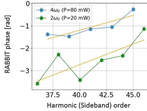
Figure 6.31: Classic RABBIT phases measured for high ( 4\omega_0 ) and low ( 2\omega_0 ) dressing power .
