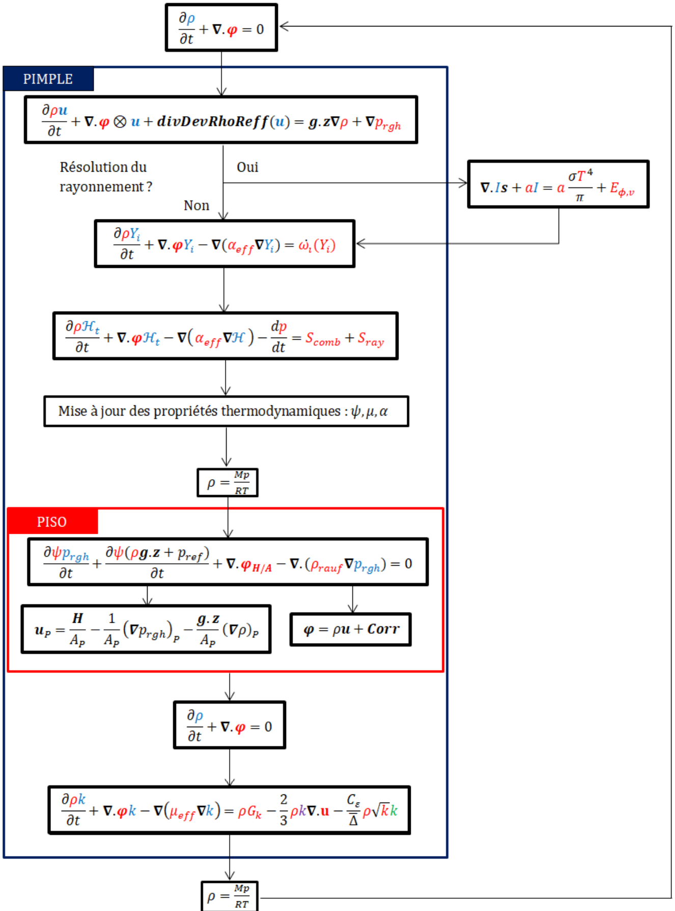
Figure 1.32 – Organigramme de FireFOAM-4.0.
