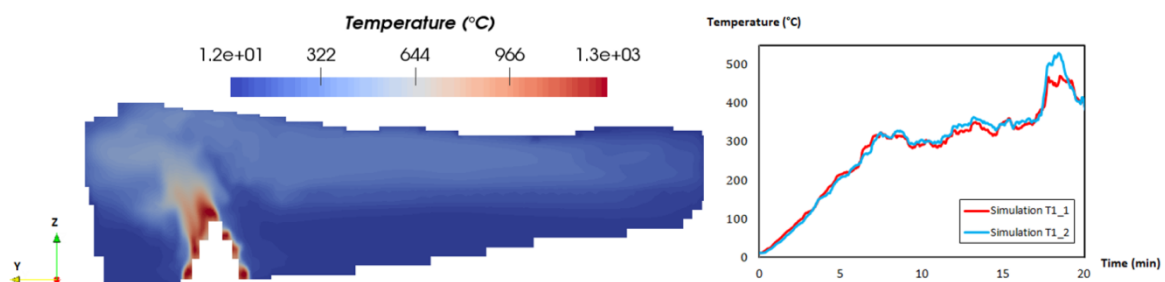
Fig. 10. On the left: numerical temperature field in the median section of the second gallery 20 minutes after the ignition of the combustion. On the right: simulated temperature at the tree T1 at the points T1_1 and T1_2. Both are performed without z-velocity outside the turning region.
