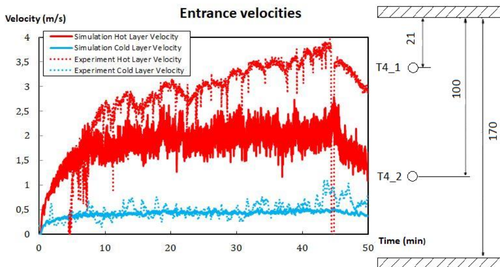
Fig. 22. On the left: comparison between the numerical and experimental velocities at the tree T4. On the right: cross section of the gallery near the tree T4, showing the vertical locations (in cm) of the velocity sensors.
