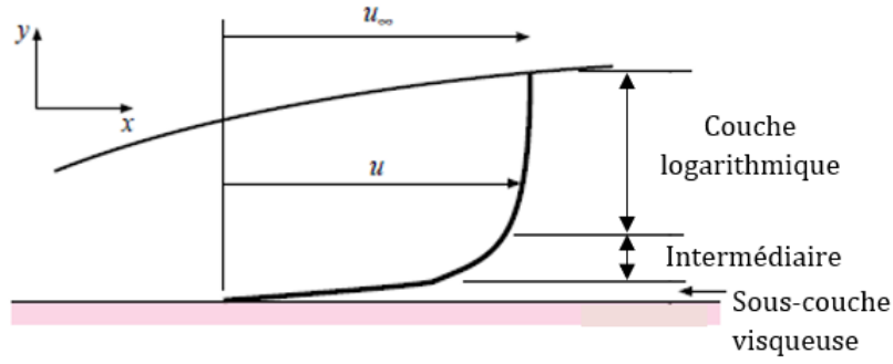
Figure 1.17 – Divisions de la couche limite.
