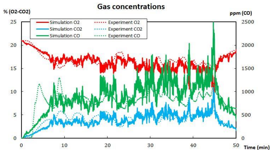
Fig. 19. Comparison between the numerical and experimental gases concentration at the point T2_1.
