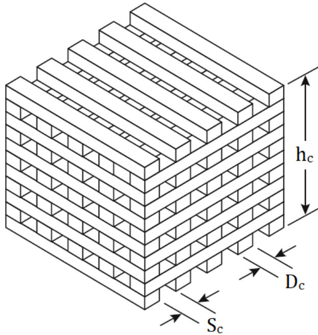
Figure 4.8 – Structure du wood crib [11].
