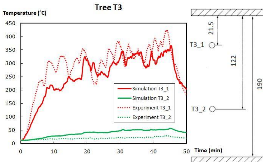
Fig. 18. On the left: comparison between the numerical and experimental temperatures at the tree T3. On the right: cross section of the gallery near the tree T3, showing the vertical locations (in cm) of the thermocouples.
