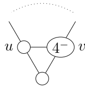
Figure 1.6 – A semi-weak neighbor v of u .
