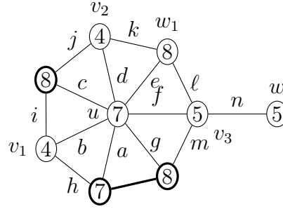
Figure 1.47 – Notation for Lemma 1.44
