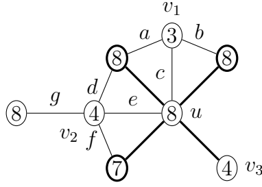
Figure 1.75 – Notation for Lemma 1.71
