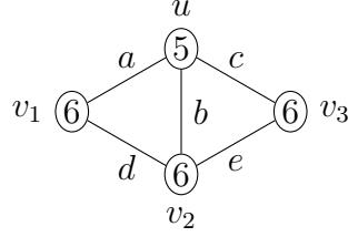
Figure 1.32 – Notation for Lemma 1.30
