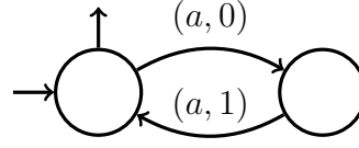
Figure 3.10 – The automaton \hat{\mathcal{A}}
