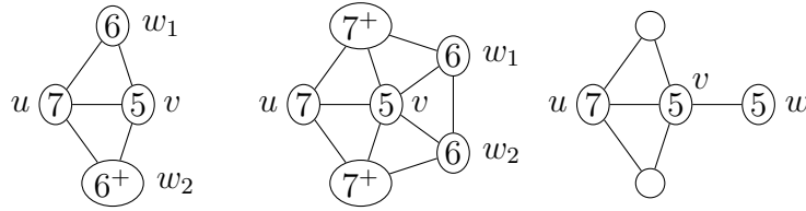
Figure 1.7 – v is an S_3 -neighbor of u
