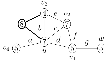
Figure 1.37 – Notation for Lemma 1.35
