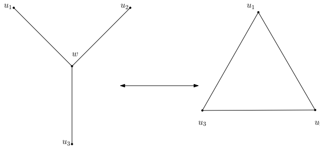
Figure 1.7 – The star-triangle equivalence
