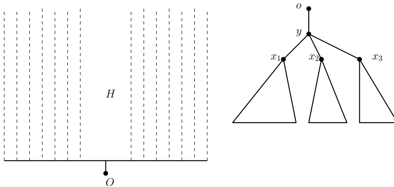
Figure 2.13 – The upper-half plane on the left and the tree \mathcal{T}_{\mathbb{H}} on the right.
