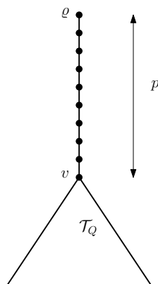
Figure 2.9 – The tree \mathcal{T}
