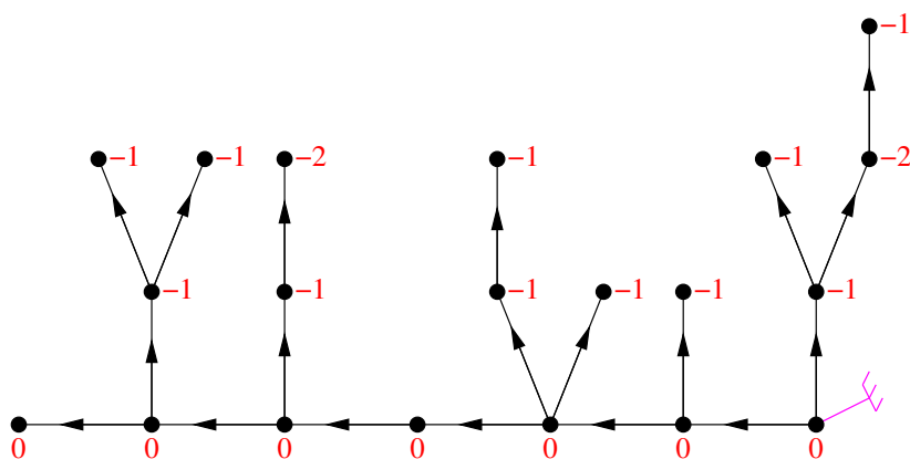
Figure 6.11 – Example of a well-labeled forest of \mathcal{F}_6^{13} .
