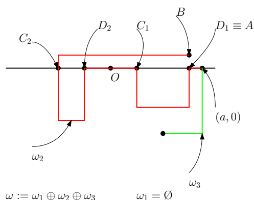
Figure 2.7 – Illustration of the proof of Lemma 6.3, case \mathcal{T}_{\mathbb{Z}^2}
