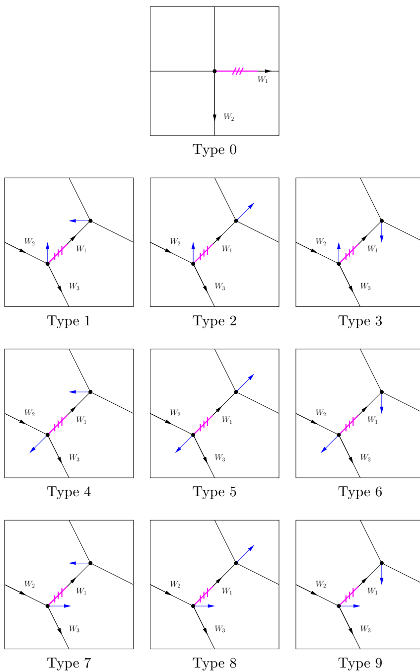
Figure 6.14 – The ten possible types of kernels for an element of \mathcal{U}_r(n) . The red half-edge indicates the root half-edge.
