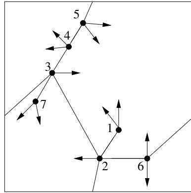
Figure 6.6 – Example of an element of \mathcal{U}_b(7) .
