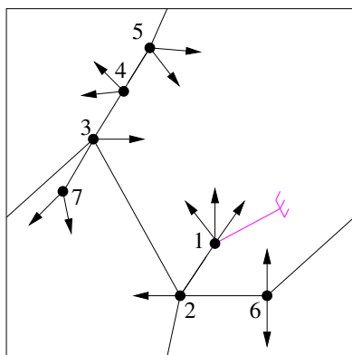
Figure 6.2 – Example of an element of \mathcal{T}_r(7) .
