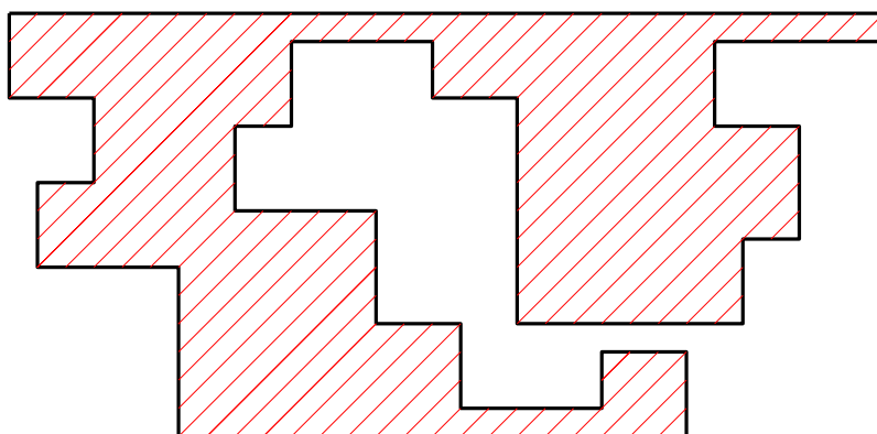
Figure 2.8 – A closed, simple curve C of \mathbb{Z}^2 with its interior in red
