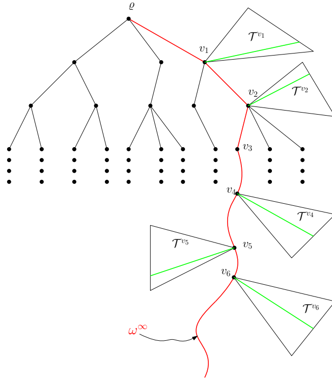
Figure 5.2 – The proof’s idea of Proposition 10.2. The limit walk \omega^\infty is in red. Conditioning on the event \{\omega^\infty(0) = \rho, \omega^\infty(1) = v_1, \dots, \omega^\infty(6) = v_6\} and denote by \ell the last time the critical M -digging random walk \mathbf{X} on \mathcal{T} visits v_6 . For each 1 \leq i \leq 6 , running the walk \mathbf{X}^{v_i, \lambda_c} on \mathcal{T}^{v_i} . The property of uniformly transient implies that there exists a surviving ray (in green) in \mathcal{T}^{v_i} with probability is larger than a constant which do not depend on i .
