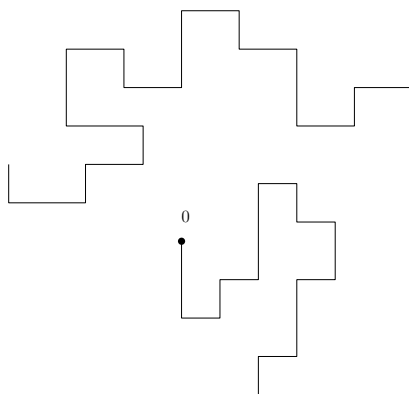
Figure 1.5 – A 111-step self-avoiding walk on \mathbb{Z}^2
