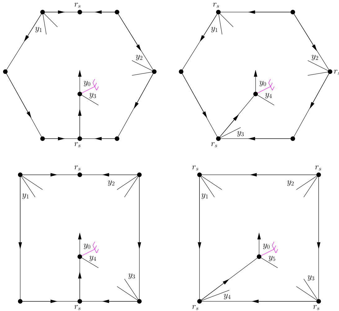
Figure .23 – Definition of the angles y_1, \dots, y_{t-1} .
