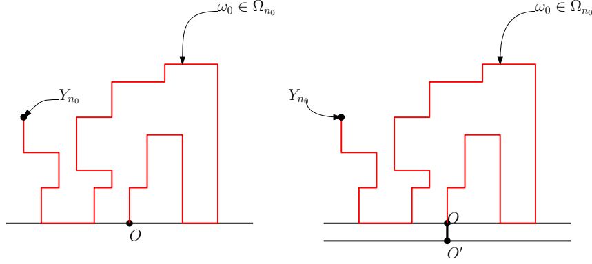
Figure 2.5 – Illustration of the proof of Lemma 6.3, case \mathcal{T}_{\mathbb{H}}
