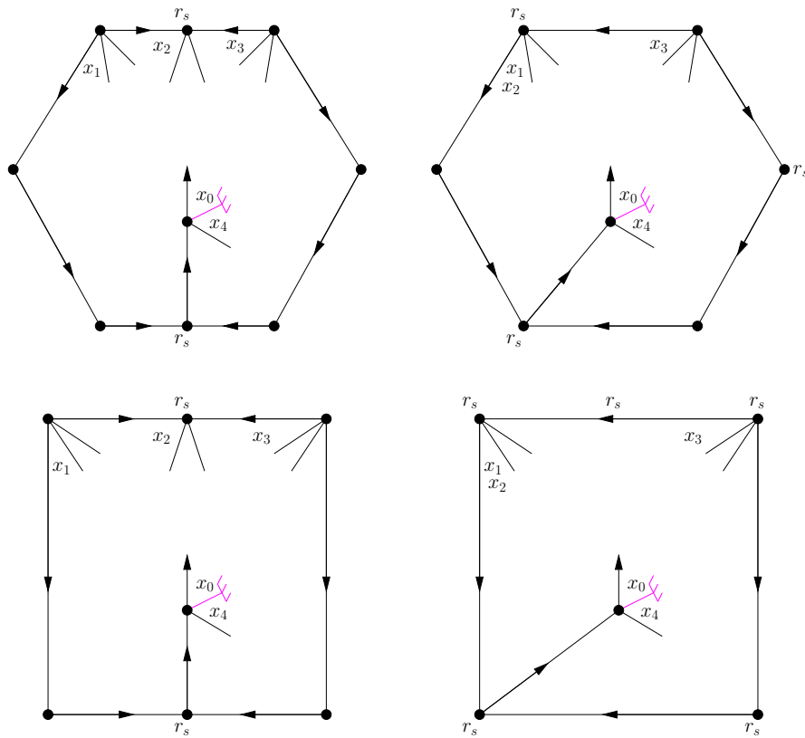
Figure .22 – Definition of the angles x_1, x_2 and x_3 depending on the type of unicellular map.
