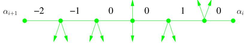
Figure 6.17 – The Motzkin path corresponding to R_i (from right to left).
