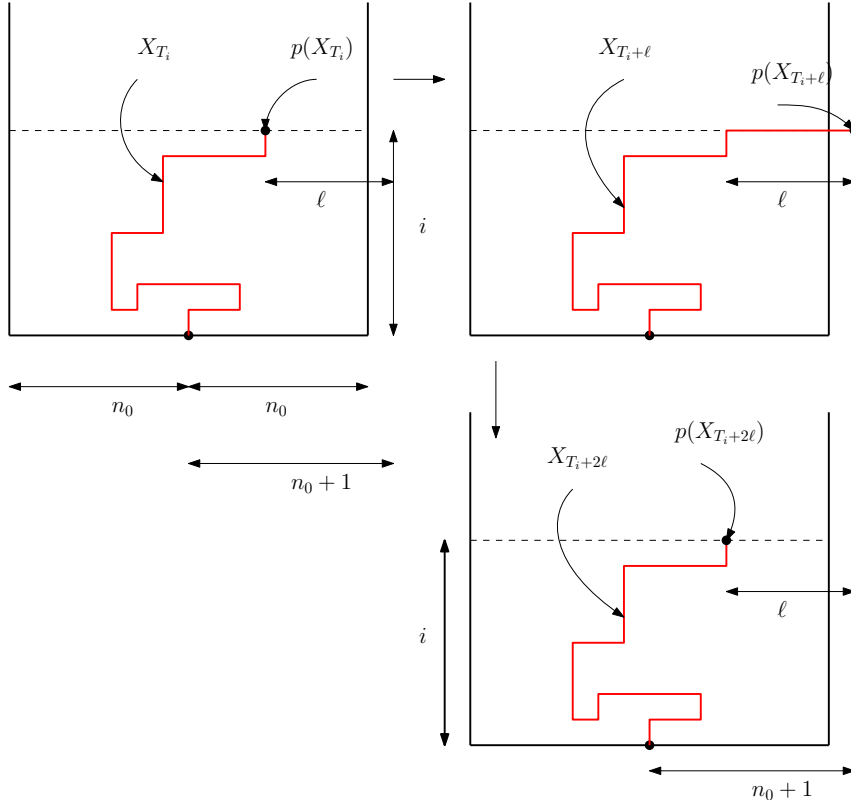
Figure 2.3 – Illustration of the proof of Lemma 6.1
