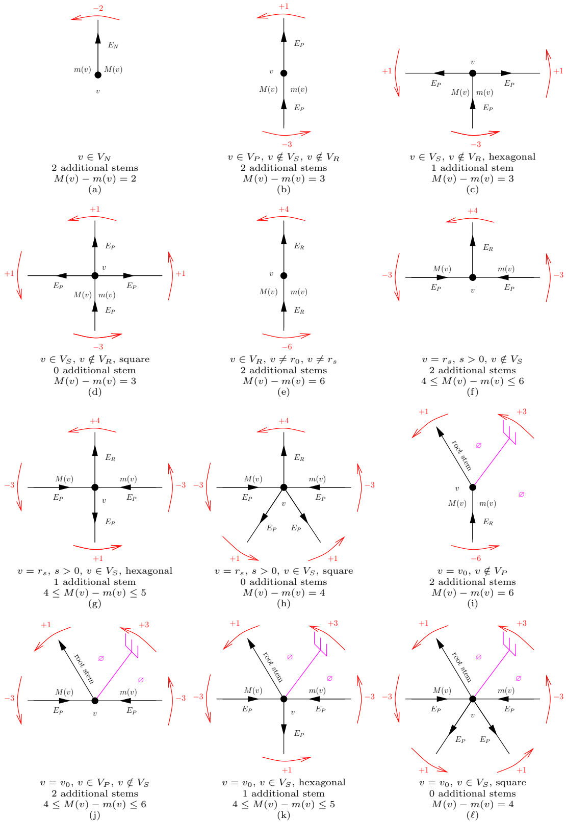
Figure 6.9 – Variations of the labeling around the different kind of possible vertices of \Gamma .
