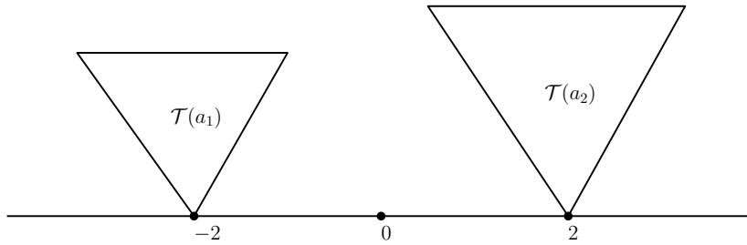
Figure 2.1 – Tree \mathcal{H}^0
