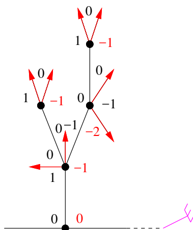
Figure 6.21 – Computation of the label \lambda around a tree of a well-labeled forest.
