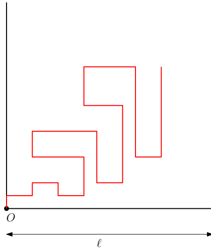
Figure 2.11 – A bridge of a strip B_\ell
