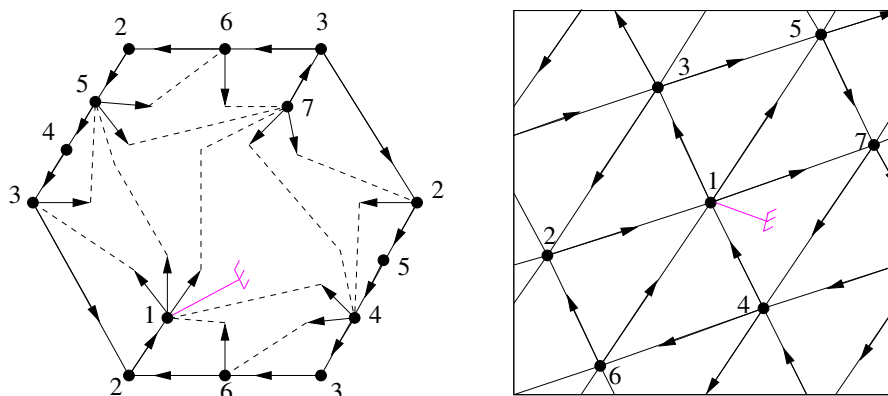
Figure 6.5 – The canonical orientation of K_7 .
