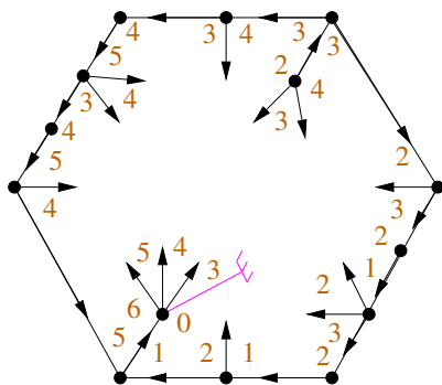
Figure 6.7 – Labeling of the angles of the unicellular map.
