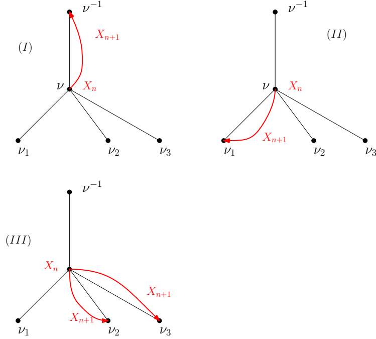
Figure 5.1 – The movement of \mathbf{X} to \nu_1 after visiting \nu .
