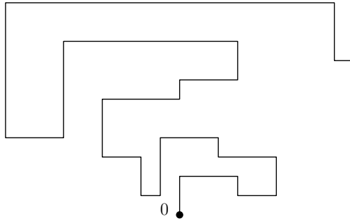
Figure 1.6 – A 86-step bridge on \mathbb{Z}^2
