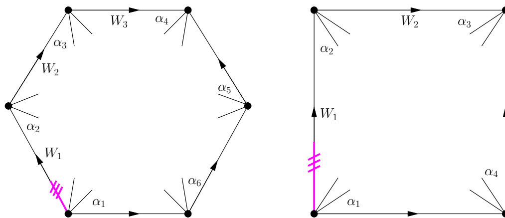
Figure 6.15 – Definition of the angles \alpha_1, \dots, \alpha_{2t} .
