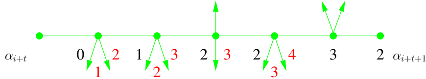
Figure 6.19 – The inverse of the extension of the Motzkin path (from left to right).
