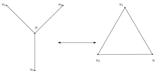
Figure 1.7 – The star-triangle equivalence
