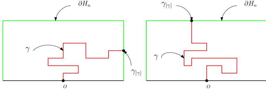
Figure 2.2 – The boundary of \mathbb{H}_n is green and the self-avoiding walk \gamma is red. Recall that \gamma is a vertex of the tree \mathcal{T}_{\mathbb{H}} . On the left (resp. right), we can add a new quadrant \mathbb{Q} (resp. new half-plane \mathbb{H} ) rooted at \gamma|_{\gamma|} . Hence, on the left (resp. on the right) the sub-tree (\mathcal{T}_{\mathbb{H}})^{\gamma} contains the tree \mathcal{T}_{\mathbb{Q}} (resp. \mathcal{T}_{\mathbb{H}} ).
