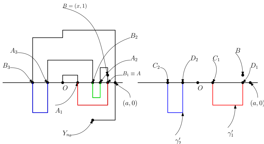
Figure 2.6 – Illustration of the proof of Lemma 6.3, case \mathcal{T}_{\mathbb{Z}^2}
