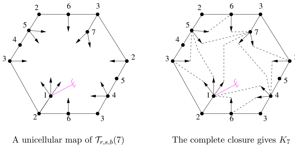
Figure 6.3 – Example of the complete closure procedure.
