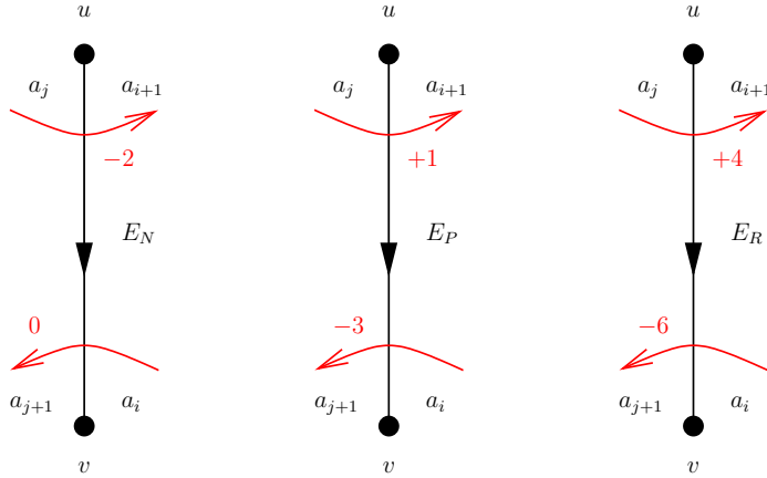
Figure 6.8 – Variations of the labeling around the three different kind of edges of \Gamma .
