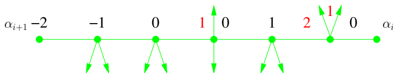
Figure 6.18 – The extension of the Motzkin path (from right to left).
