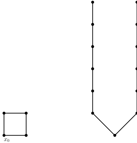
Figure 1.1 – A graph and part of its universal cover
