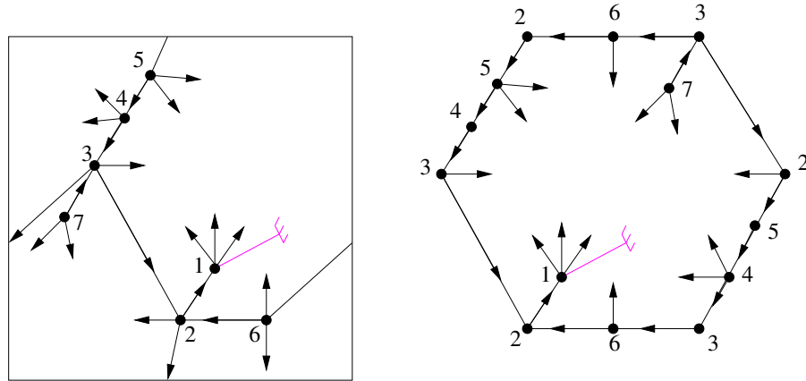
Figure 6.4 – Orientation of the edges and stems of an element of \mathcal{T}_r(7) .
