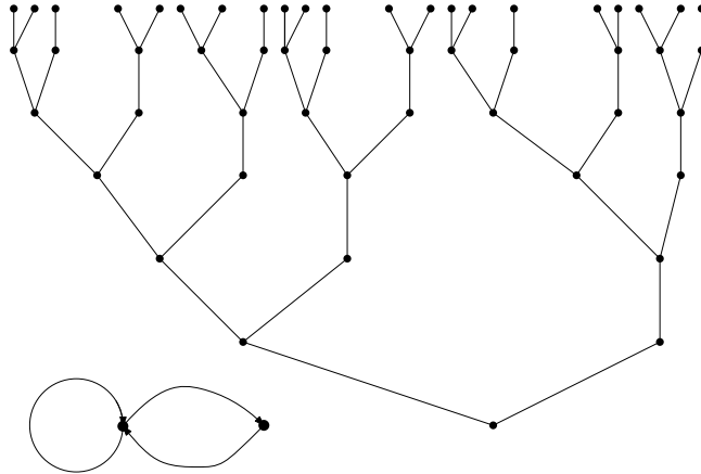
Figure 1.2 – A graph and part of its directed cover
