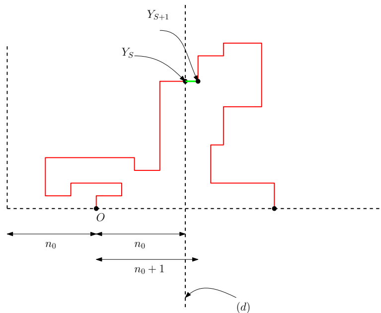
Figure 2.4 – Illustration of the proof of Lemma 6.2
