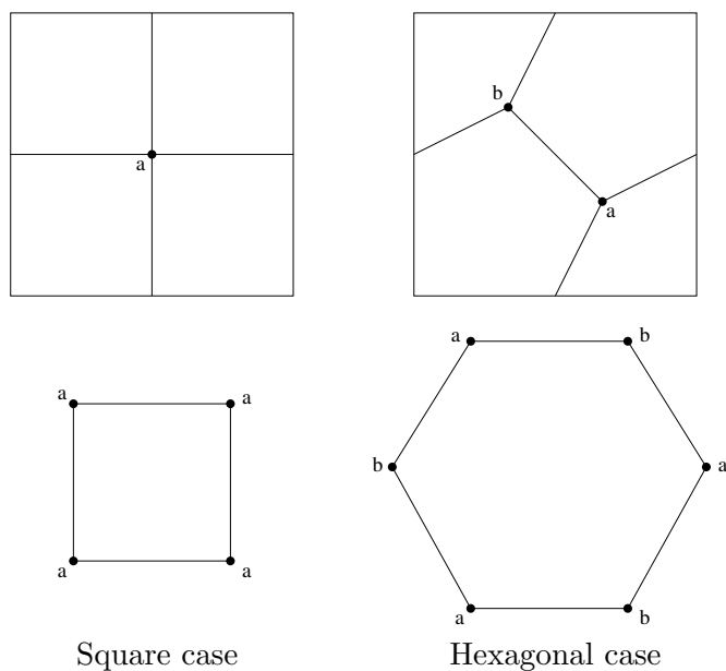
Figure 6.1 – The two types of toroidal unicellular maps with two different representations for each case.
