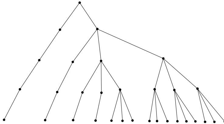
Figure 1.3 – Arbre 1-3
