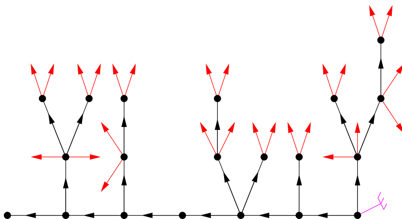
Figure 6.12 – Representation of the well-labeled forest of Figure 6.11 by a plane rooted tree with two additional stems incident to each tree-vertex.
