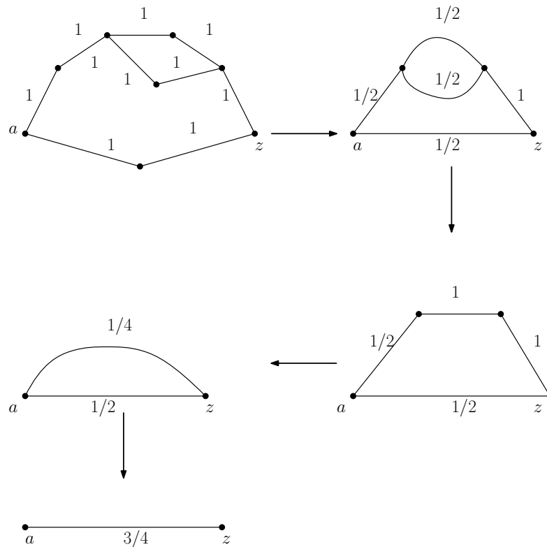
Figure 1.8 – The sequence of transformations
