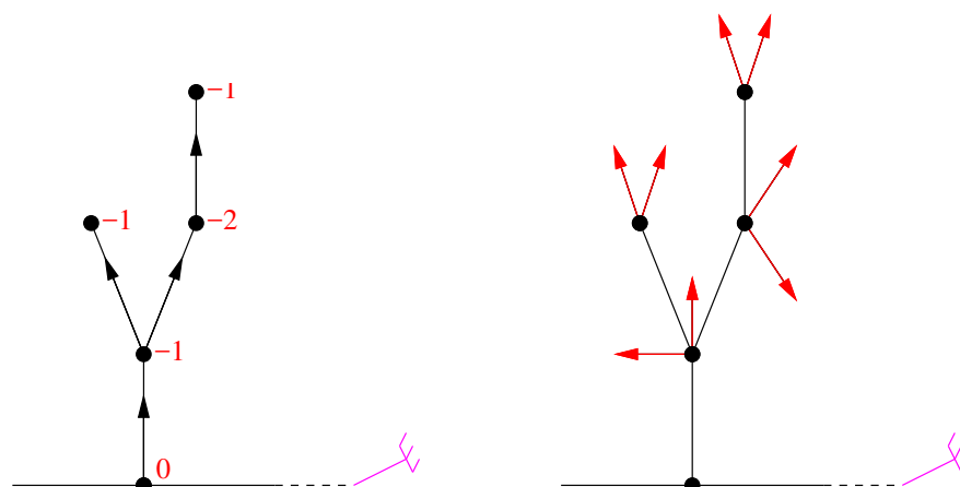
Figure 6.20 – Example of a tree of a well-labeled forest.
