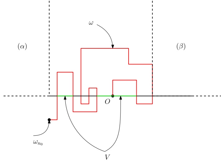
Figure 2.10 – The self-avoiding walk \omega is colored by red; the domain D is the union of two quadrants \alpha and \beta and the set V is colored by green.
