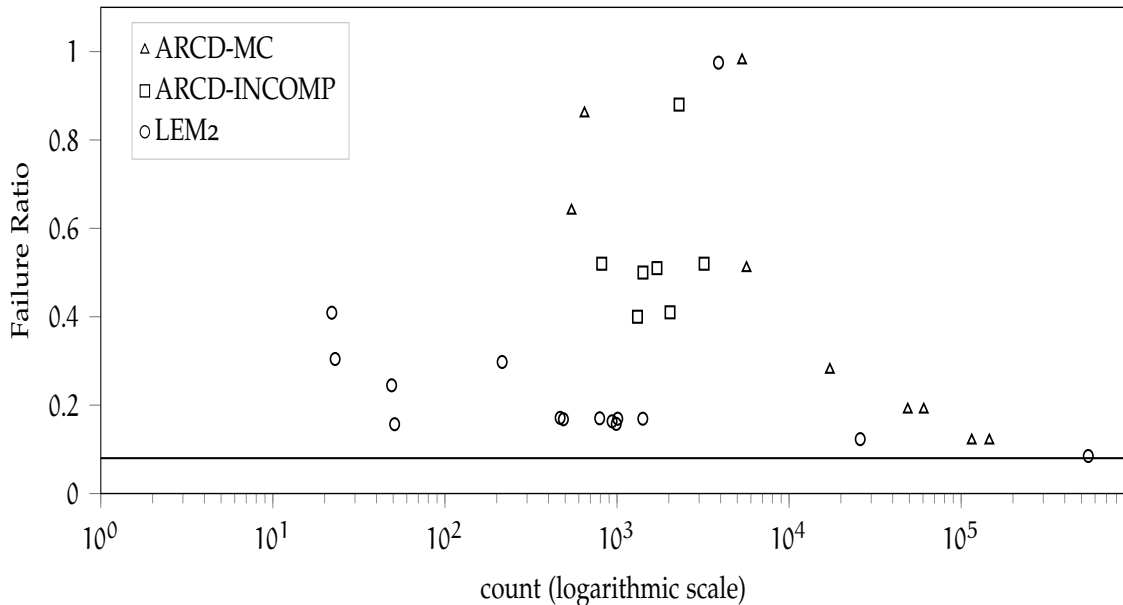
Figure 47: Output from Set 3, signatures identified by ARCD-MC (major contributors), by ARCD-INCOMP (incompatibilities), and LEM 2 . Each point corresponds to one signature, with its failure ratio and the number of related logs.
