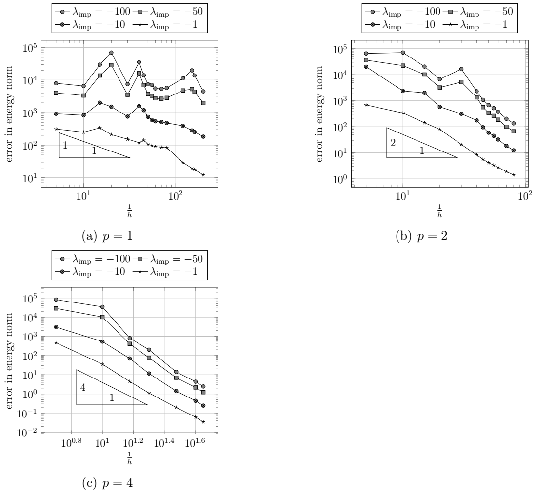
Figure 2.5: Rates of convergence for \lambda_{imp} = -1, -10, -50, -100 with p = 1, 2, 4 .
