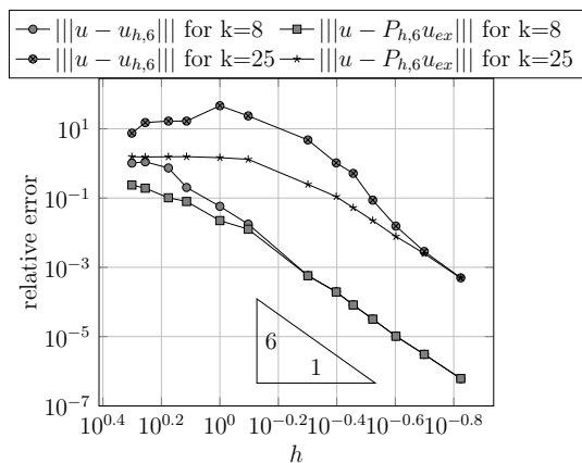
(c) Rates of convergence for k = 8 or 25 with p = 6
