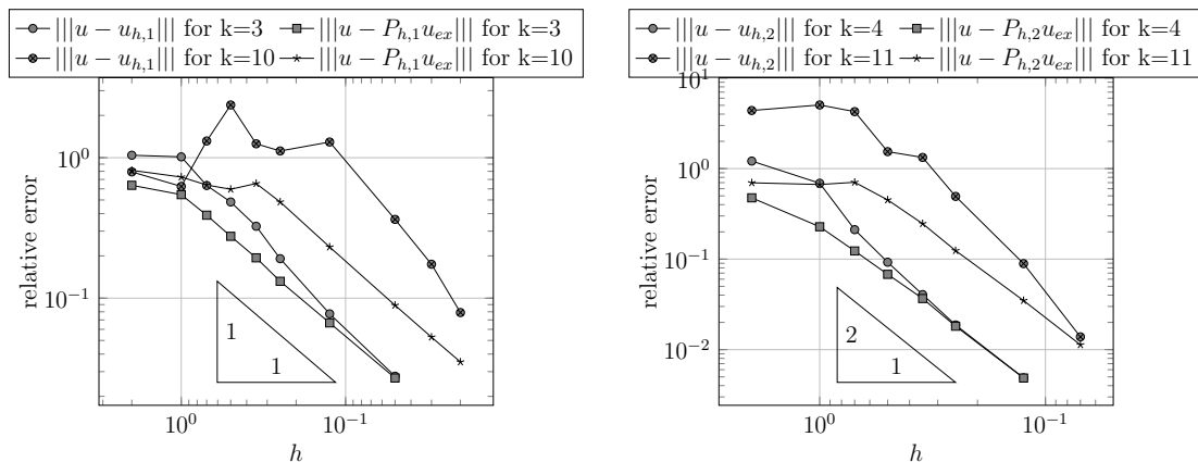
(a) Rates of convergence for k = 3 or 10 with p = 1
