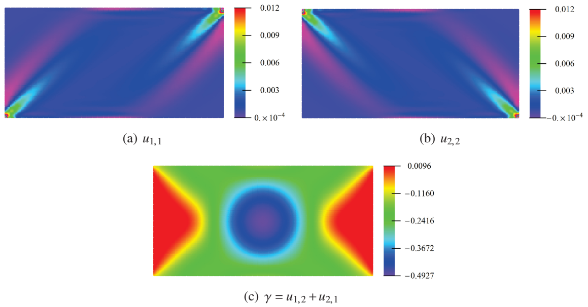
Figure 4.22: Bias test of a second gradient material: components of the first gradient of the displacement \mathbf{u} with respect to the material axes.
