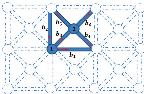
Figure 3.8: Reference cell rectangular braced with pivot
