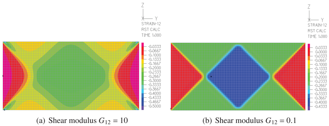
Figure 4.19: Shear strain \gamma_{12} for two values of the equivalent shear modulus G_{12}
