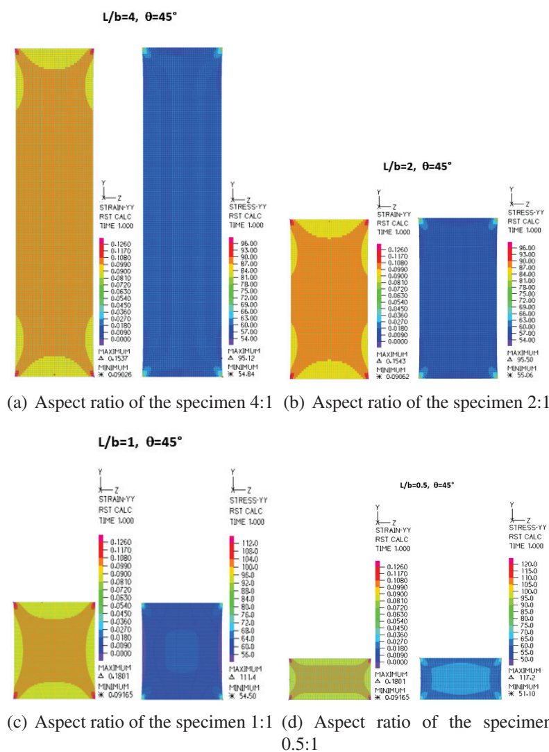
Figure 4.3: Plot of the strain \epsilon_{yy} and the stress \sigma_{yy} for bias test of a network with square braced reference cell with rigid connections varying the aspect ratio of the specimen.
