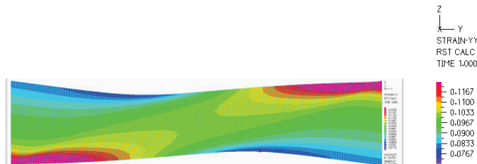
(b) Strain in direction y - \epsilon_{yy}
