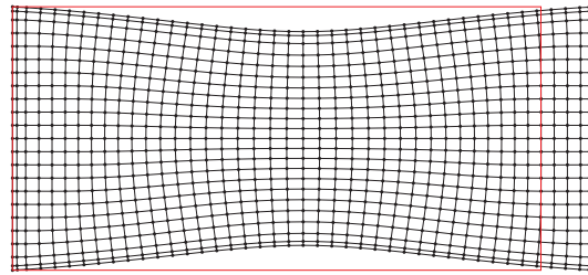
Figure 4.21: Deformed configuration of the bias test on a second gradient material
