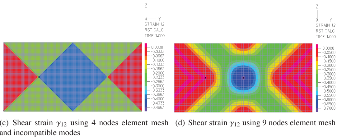
Figure 4.20: Deformed configuration and shear strain \gamma_{12} for the equivalent shear modulus G_{12} = 10^{-7}
