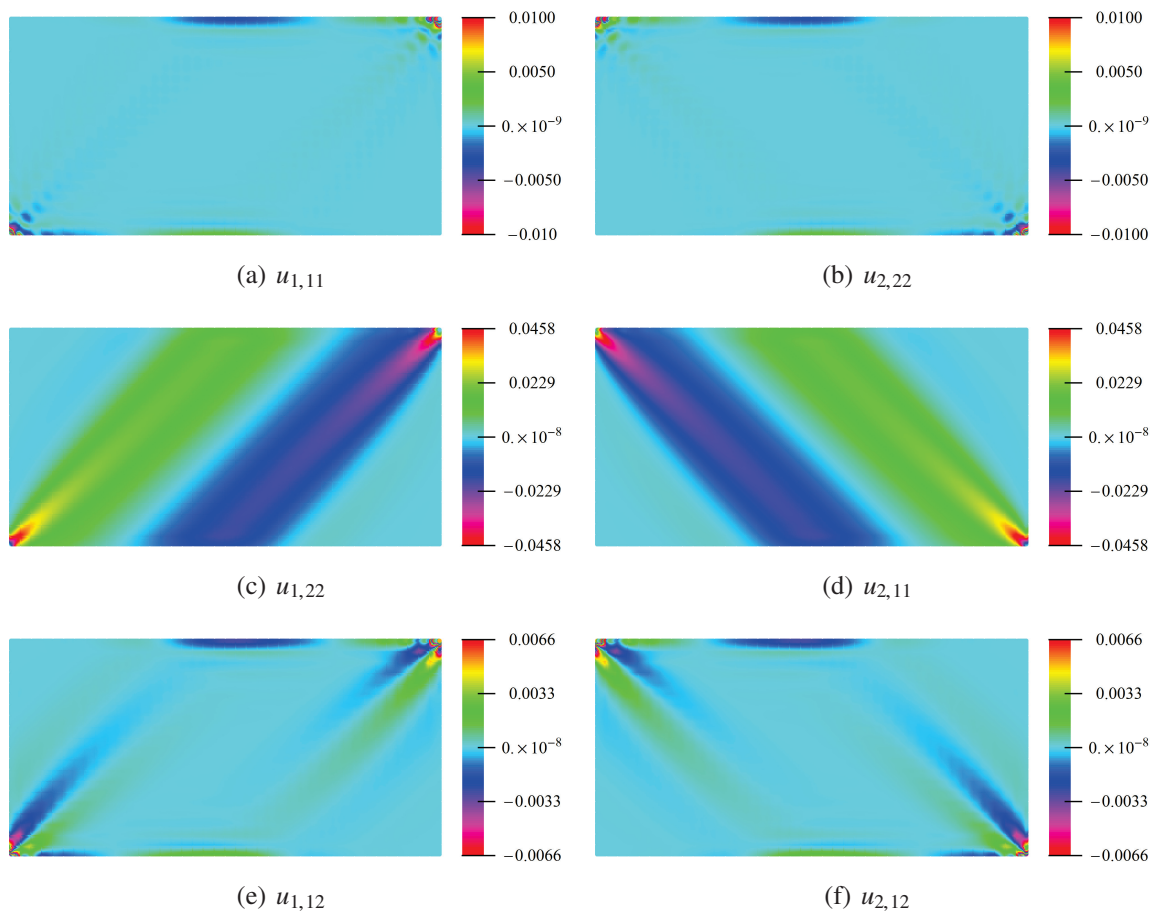
Figure 4.23: Bias test of a second gradient material: components of the second gradient of the displacement \mathbf{u} with respect to the material axes.
