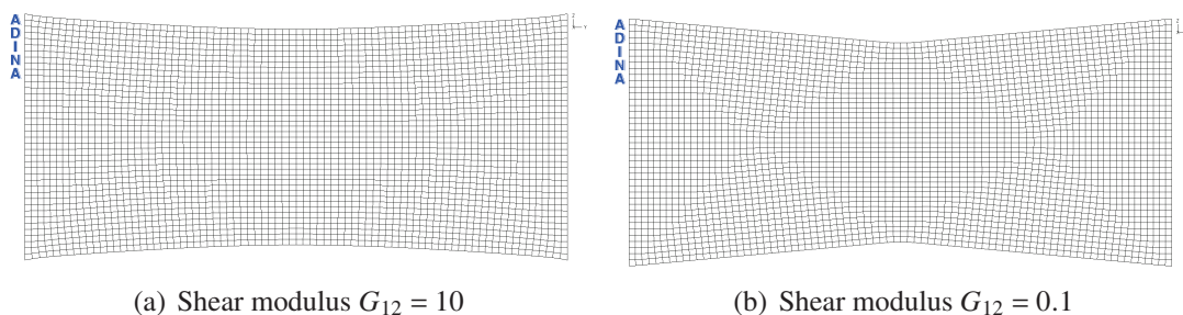
Figure 4.18: Deformed configurations for two values of the equivalent shear modulus G_{12}
