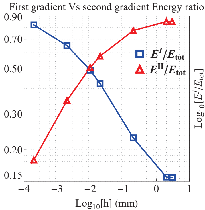
Figure 4.26: Ratio between the first gradient energy and the total energy and ratio between the second gradient energy and the total energy vs. height of the microbeams.
