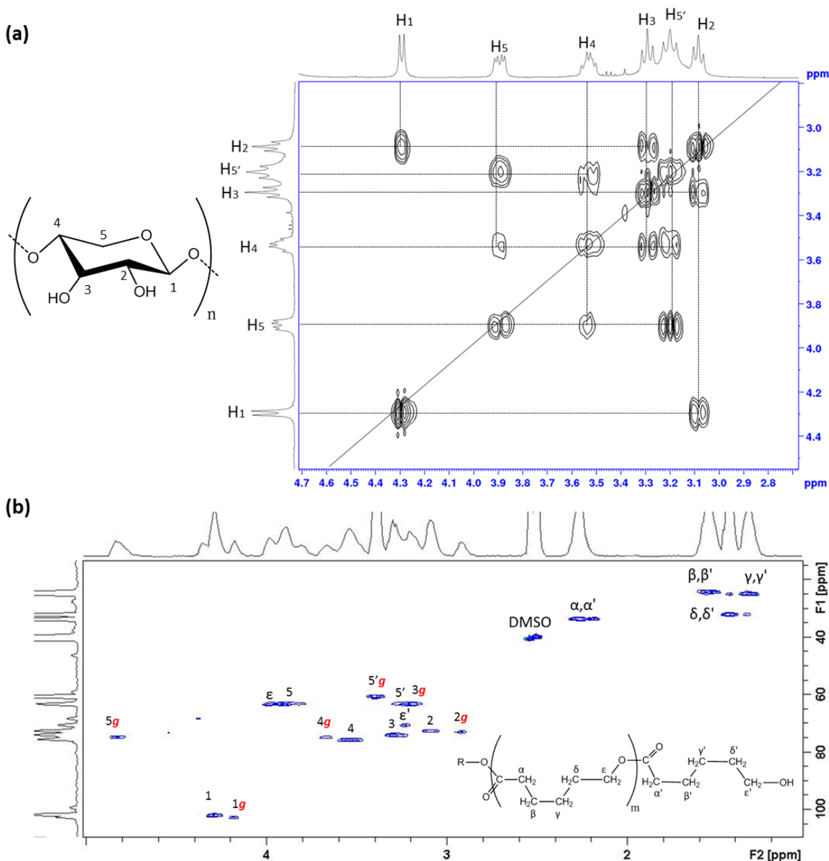
Figure 5. 2D NMR spectra. (a) ^1\text{H} - ^1\text{H} COSY spectrum of pure hemicellulose, (b) ^1\text{H} - ^{13}\text{C} HSQC spectrum of HCgPCL-2 (DP 3.35, SR T 0.62) copolymer
