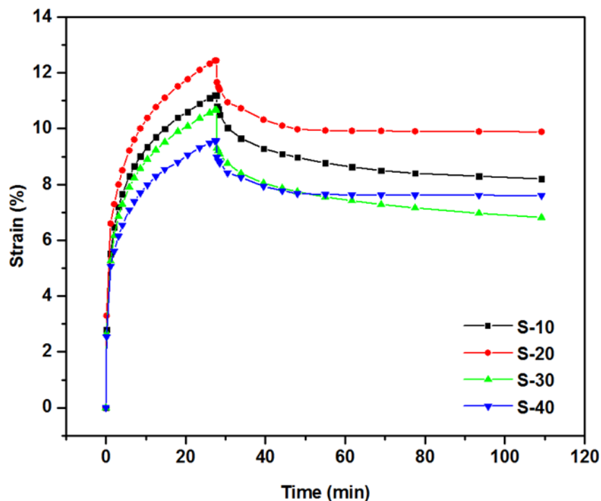
Figure 11. Creep-recovery response of the furan grafted copolymers at 80°C
