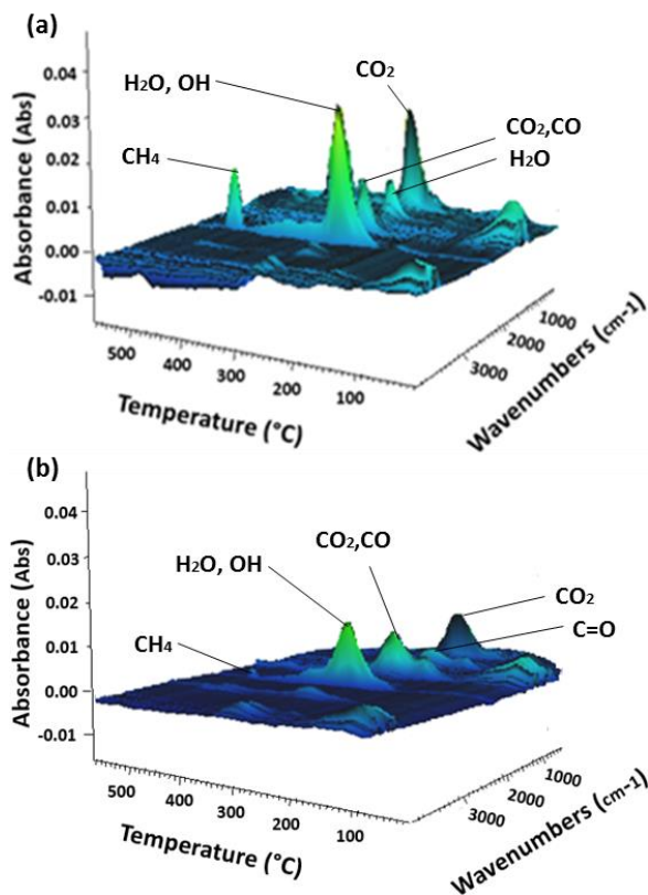
Figure 8. Corresponding gas absorption profile. (a) Native hemicellulose, and (b) \text{HC}_g\text{PCL-3} (DP 4.26, \text{SR}_T 0.69) copolymer.
