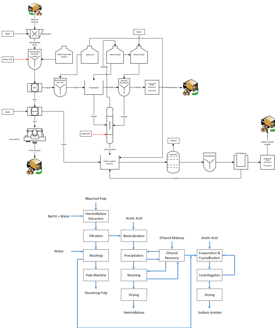
Figure 7. Schematic representation of the bio-refining pathways for the production of dissolving pulp and hemicellulose
