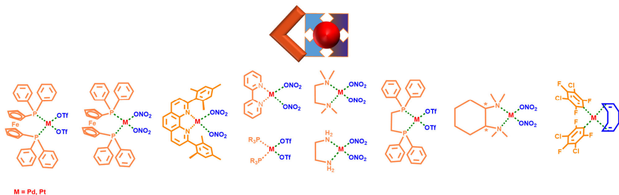
Figure 1.3.1. Structures of common cis -blocked acceptor units.
