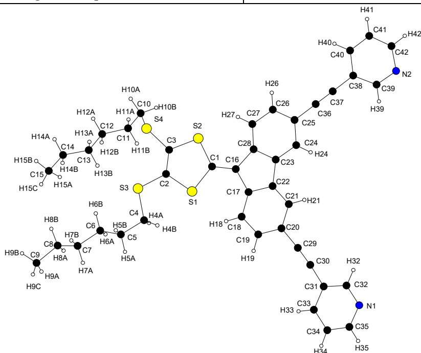
Annex 6.4. X-ray data for ligand 27 (3Py-DTF-SPr)
