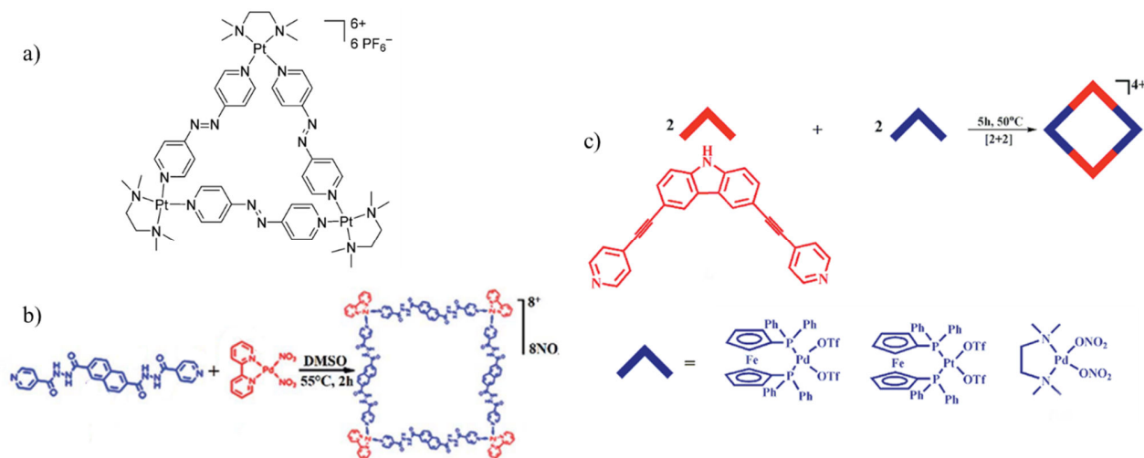
Figure 1.3.2. Self-assembled molecular triangles (a) and squares (b, c). 30-32
