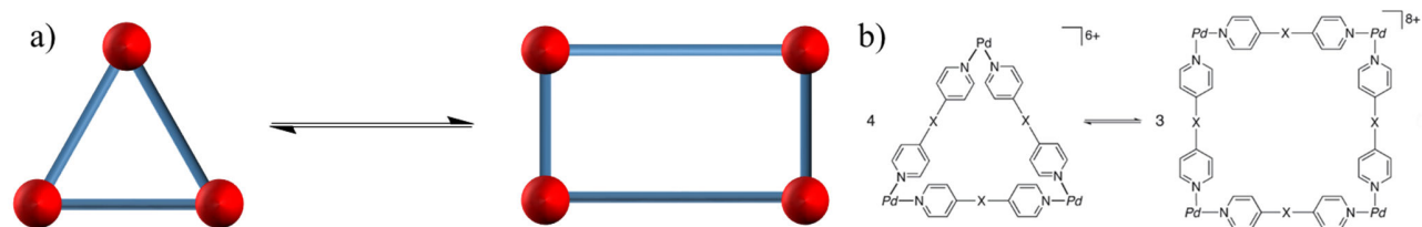
Figure 1.3.3. Triangle-square equilibrium. 35
