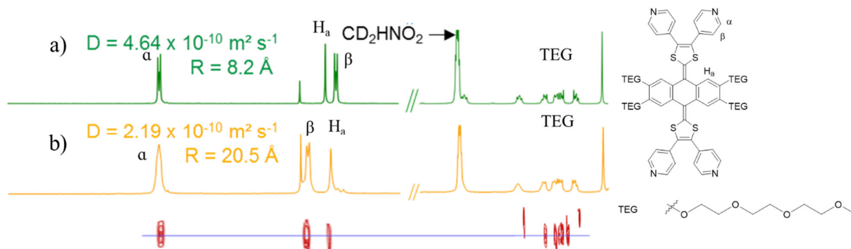
Figure 4.3.3. ^1\text{H} and DOSY NMR for the exTTF-TEG ligand (a) and resulting self-assembly AA15 after reaction with \text{AgOTf} (b) in \text{CDCl}_3/\text{CD}_3\text{NO}_2
