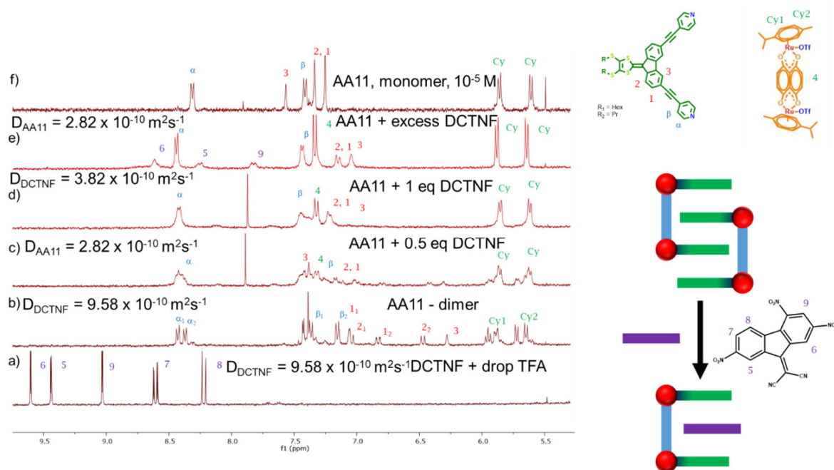
Figure 3.4.11. ^1H and DOSY NMR of guest DCTNF (a), self-assembly AA11 (b – dimer, f – monomer) and their mixture (c, d, e) in methanol- d_4
