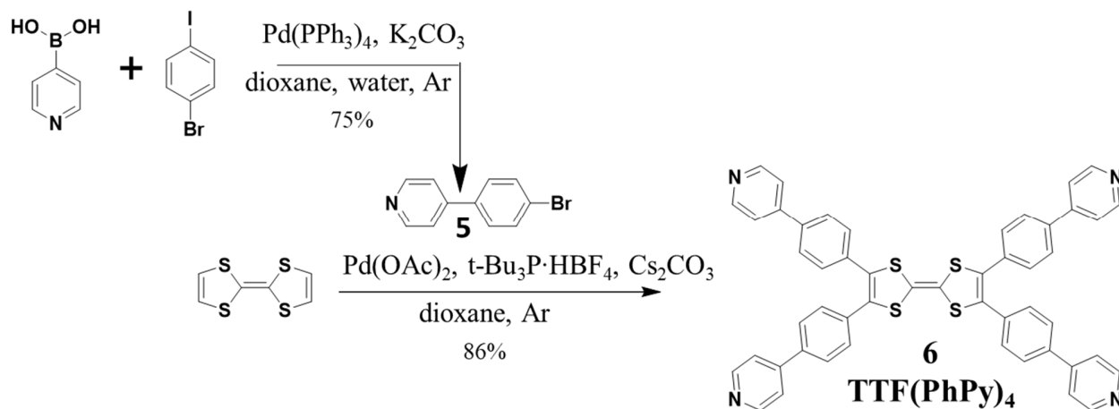
Scheme 2.1.2. Synthesis of the \text{TTF}(\text{PhPy})_4
