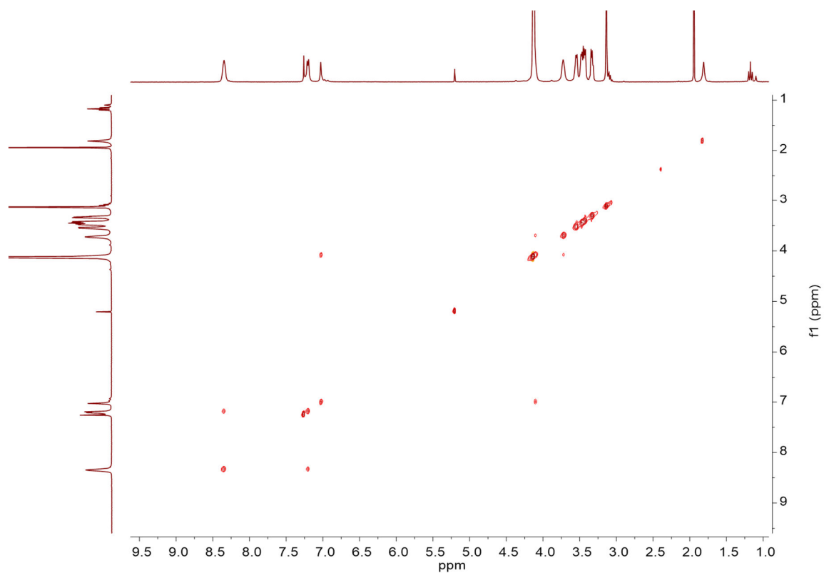
Annex 3.27. ^1\text{H} NMR for ligand exTTF-TEG with 4 eq. of \text{AgBF}_4 in \text{CD}_3\text{CN}
