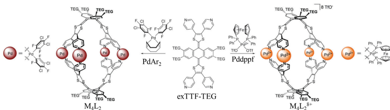
Scheme 1.5.2. Redox-active cages using exTTF-TEG ligand. 150
