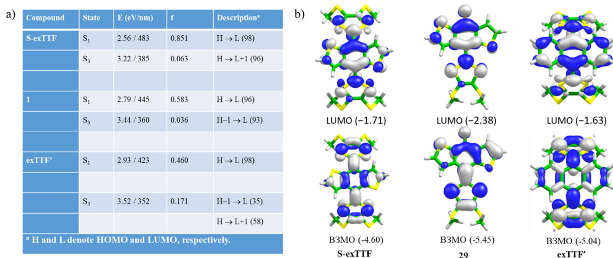
Figure 5.3.9. a) Lowest singlet excited states calculated at the TDDFT B3LYP-D3/6-31G** level for S-exTTF, intermediate 1S-exTTF and exTTF' in CH 2 Cl 2 solution. Vertical excitation energies (E), oscillator strengths (f) and dominant monoexcitations with contributions (within parentheses) greater than 10%. b) frontier molecular orbitals computed for S-exTTF, 29 and exTTF' at the B3LYP-D3/6-31G** level in CH 2 Cl 2 . Isovalue contours (±0.03 a.u.) were used. Molecular orbital energies are given within parentheses in eV.
