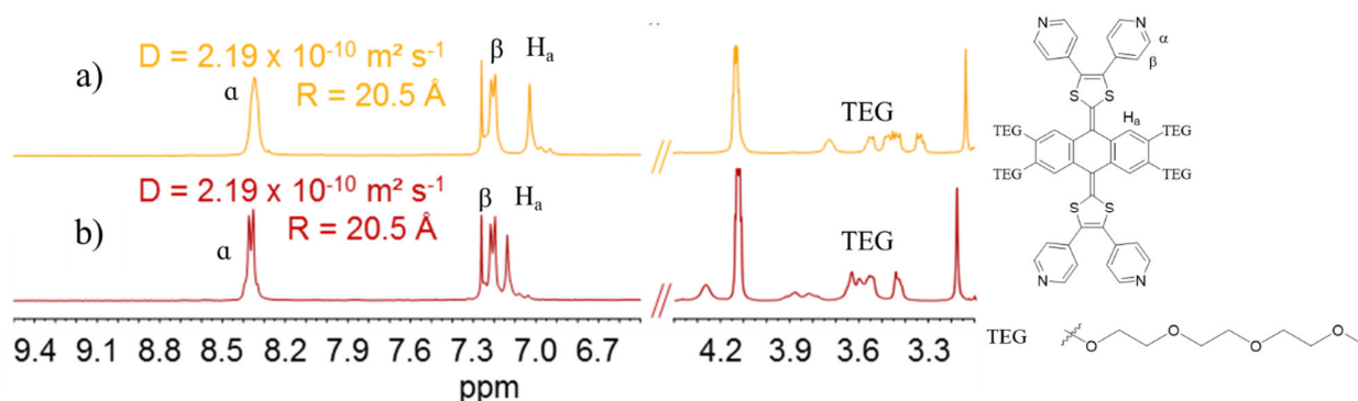
Figure 4.4.1. ^1\text{H} and DOSY NMR for the self-assembly AA15 (a) and resulting complex [\text{Ag}_{12}(\text{Ag}_2(\text{exTTF-TEG})_6)]^{2+} (b) in \text{CDCl}_3/\text{CD}_3\text{NO}_2
