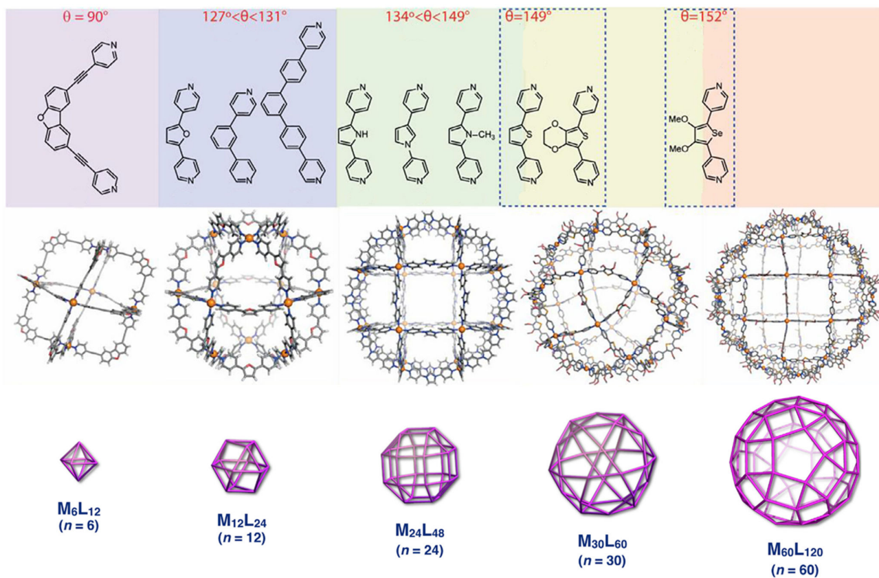
Figure 1.3.9. Large cages of the M_nL_{2n} type. 48
