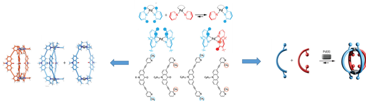
Figure 1.3.15. Rational design of a social cage leads to the formation of either mixture of homoleptic cages (left) or heteroleptic cis-[PdL_1^2L_2^2] cage (right). 60
