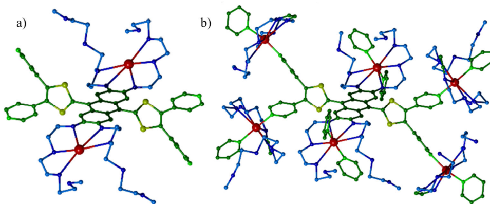
Figure 4.4.3. Partial [(Ag_2(exTTF-TEG^{2+}))^{2+}]_x X-ray structure showing a) the repeating (Ag_2exTTF-TEG^{2+})^{2+} motifs and b) the silver coordination sphere. BF_4^- anions omitted for clarity
