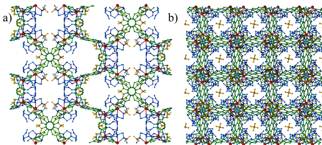
Figure 4.4.2. X-Ray structure of the [(\text{Ag}_2(\text{exTTF-TEG}^{2+}))^{2+}]_x three-dimensional supramolecular polymer, \text{BF}_4^- anions are located in the free space
