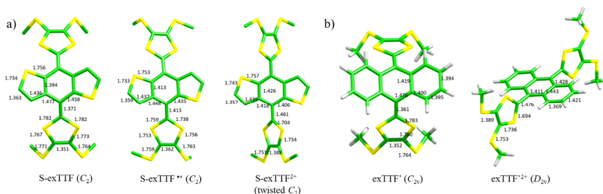
Figure 5.4.7. B3LYP-D3/6-31G**-optimized bond lengths (in Å) calculated for S-exTTF , S-exTTF •+ and S-exTTF 2+ (a) and exTTF' and exTTF 2+ (b) in CH 2 Cl 2
