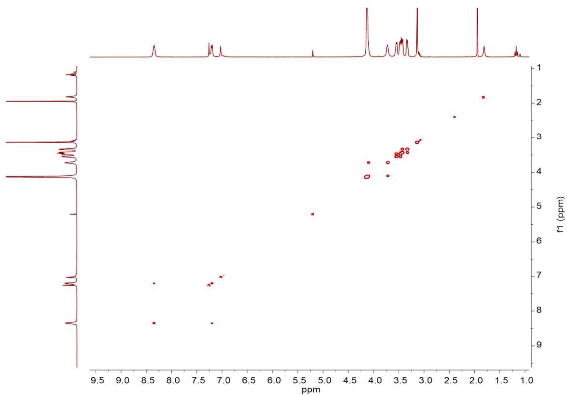
Annex 3.26. NOESY NMR for self-assembly AA15 in \text{CDCl}_3
