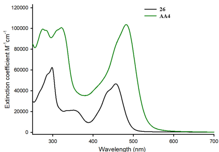
Figure 3.3.5. UV-vis absorption spectra of ligand 26 and metalla-macrocycle AA4 , r.t. ( C = 1.5 \times 10^{-5} \text{ M} in \text{CH}_2\text{Cl}_2 ).
