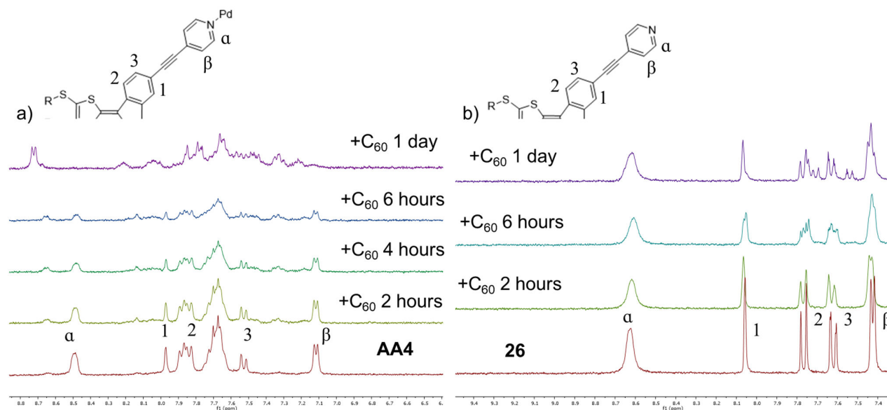
Figure 3.3.6. Progression of ^1\text{H} NMR for the mixture of C 60 with clip AA4 (a) and ligand 26 (b) upon irradiation, ( \text{C}_2\text{H}_2\text{Cl}_4\text{-}d_2 ).
