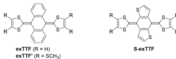
Figure 5.3.2. Molecular structure of exTTF , exTTF' and S-exTTF
