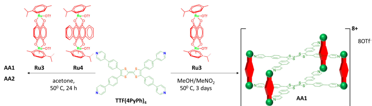
Scheme 2.2.1. Synthesis of the self-assemblies AA1 and AA2 .
