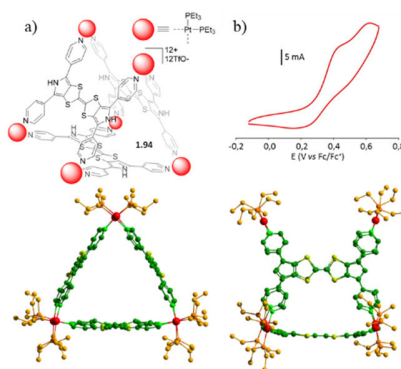
Figure 1.5.12. A BPTTF metallocage and XRD structure (a), cyclic voltammetry (b). 148
