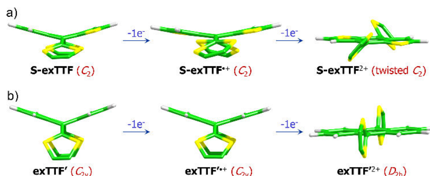
Figure 5.4.6. Summary of the structural evolution of S-exTTF (a) and exTTF' (b) upon oxidation calculated at the B3LYP-D3/6-31G** level in CH 2 Cl 2 . The thiomethyl groups have been omitted for clarity. A scheme of the aromatization achieved by the exTTF 2+ dication species is also given
