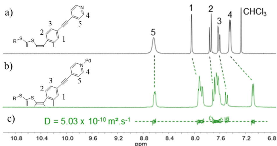
Figure 3.3.1. ^1\text{H} (a, b) and DOSY (c) NMR for the 26 (in \text{CDCl}_3 ) and AA4 (in \text{CD}_2\text{Cl}_2 ).
