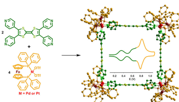
Figure 2.1.2. A TTF-based M 8 L 4 cage and its cyclic voltammetry. 149
