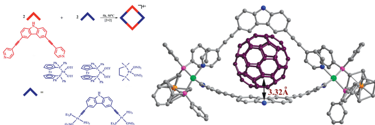
Figure 3.3.4. Example of host-guest complex using C 60 and M 2 L 2 self-assembly clip. 32
