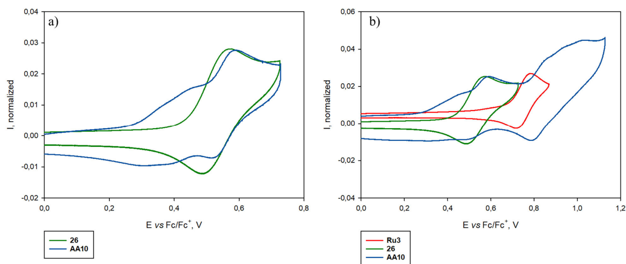
Figure 3.4.7. Normalized cyclic voltammograms of ligand 26 and metalla-ring AA10 ( C = 10^{-3}M , CH_3CN/CH_2Cl_2 , 0.1 M nBu_4NPF_6 , 100 mV \cdot s^{-1} , Pt) V vs. Fc/Fc^+ .
