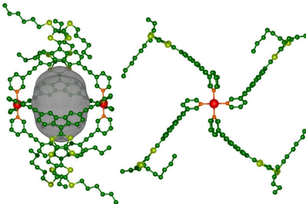
Figure 3.2.3. X-Ray crystal structure of AA3 , lateral view (left) and top view through the Pd-Pd axis (right). Counter anions, solvent molecules and hydrogens were omitted for clarity. The cavity is depicted as a grey volume.
