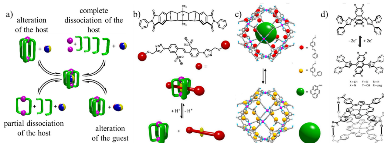
Figure 1.4.1. Different ways to control host-guest chemistry. a) general principle; b) pH c) irradiation d) redox stimuli. 10
