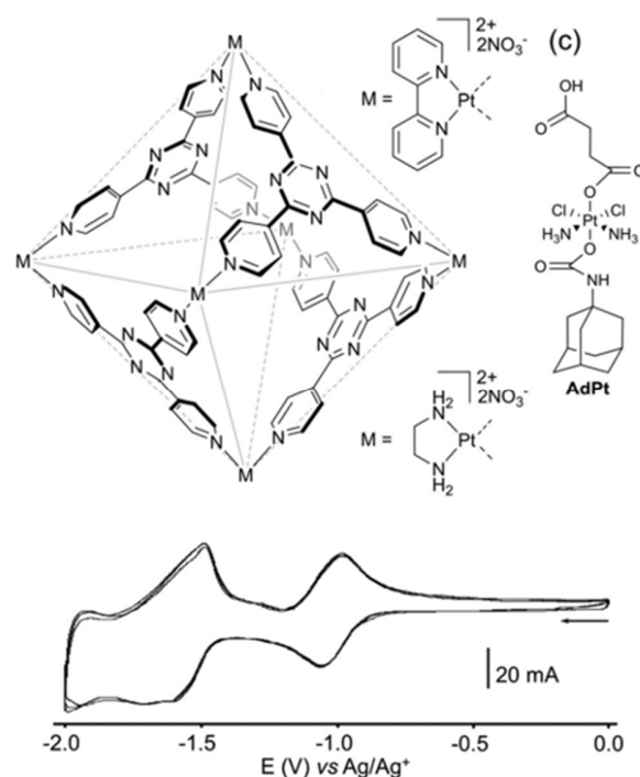
Figure 1.5.1. Triazine-based electron-poor redox-active cages.[126]
