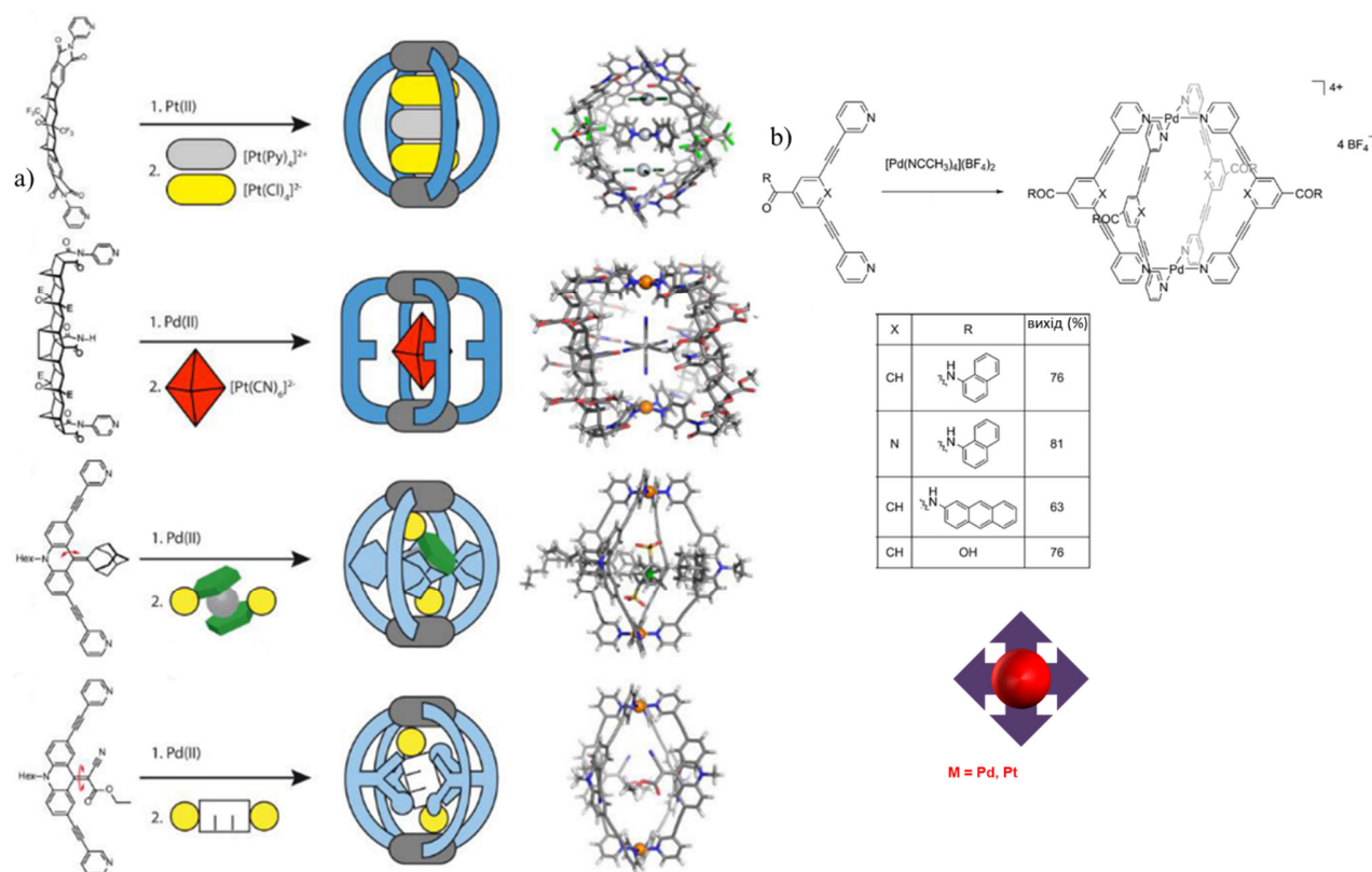
Figure 1.3.7. Examples of inner (a) and outer (b) modification of M_2L_4 cages. 42-43
