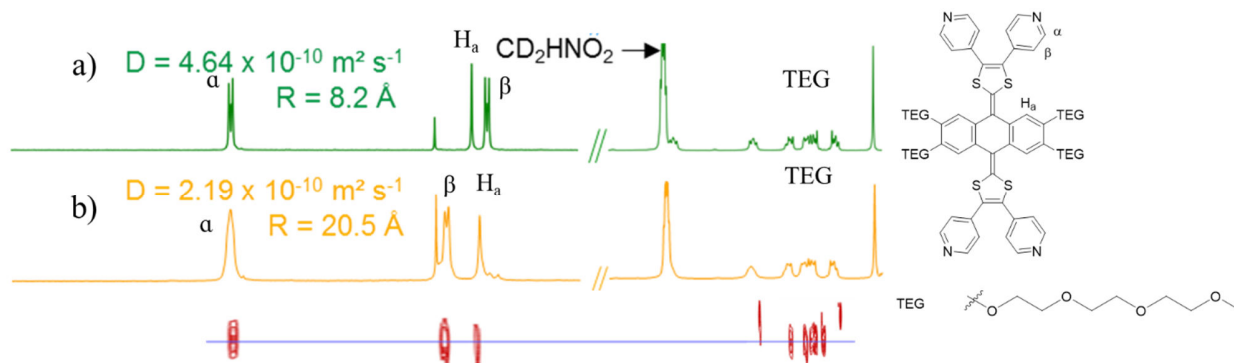
Figure 4.3.3. ^1\text{H} and DOSY NMR for the exTTF-TEG ligand (a) and resulting self-assembly AA15 after reaction with \text{AgOTf} (b) in \text{CDCl}_3/\text{CD}_3\text{NO}_2
