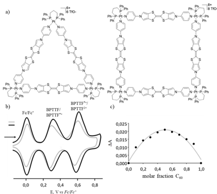
Figure 1.5.11. BPTTF-based metallocycles (a), their deconvoluted cyclic voltammetry (black, square; grey, triangle) (b) and Job's plot for the interaction between the electron-rich triangle cavity and C_{60} . 145
