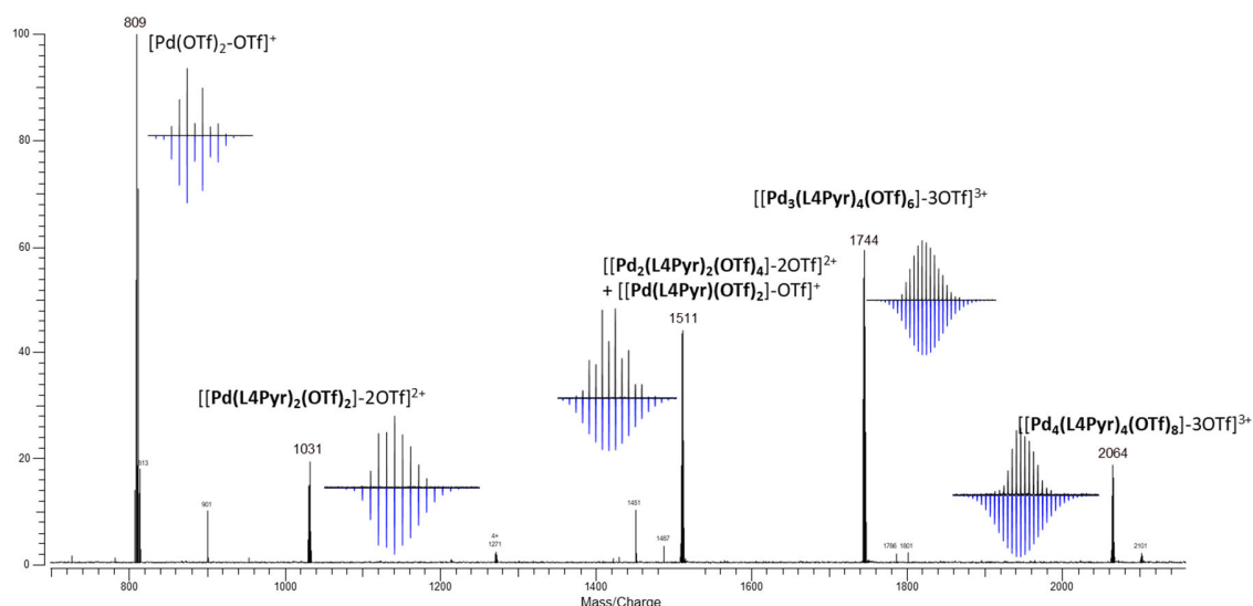
Figure 3.3.2. ESI-FTICR mass spectrum of AA4 in \text{CH}_2\text{Cl}_2 (9/1) ( C = 10^{-3} \text{ M} ), in black experimental isotopic pattern, in blue theoretical isotopic pattern.
