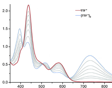
Figure 2.1.4. Temperature dependent UV-vis signature of \text{TTF}^+ and of the corresponding \pi -dimer (\text{TTF}^+)_2 (1,3 mM, acetone) from \text{TTF}^+\text{CB}^- ( \text{CB}^- : dodecamethylcarba-closo-dodecaborate) (in ^{\circ}\text{C} , from bottom to top at 740 nm) : 22, -40, -55, -63, -70, -78, -85, and -90).
