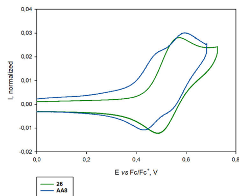
Figure 3.4.6. Normalized cyclic voltammograms of ligand 26 and metalla-ring AA8 ( C = 10^{-3} M , CH 3 CN/CH 2 Cl 2 , 0.1 M nBu 4 NPF 6 , 100 mV·s -1 , Pt) V vs. Fc/Fc + .
