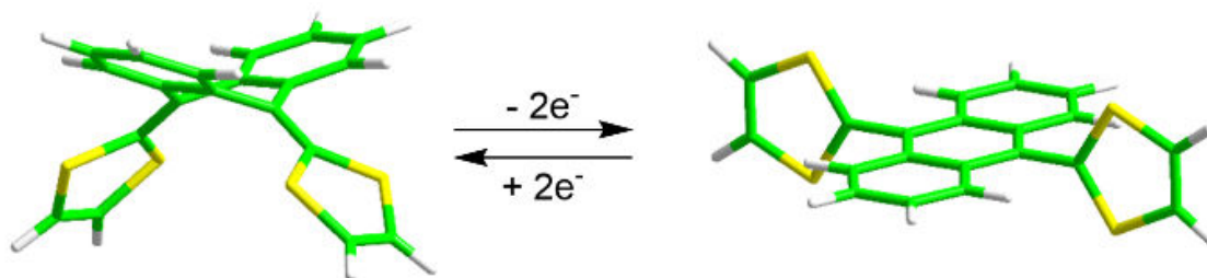
Figure 4.1.2. Conformational change of exTTF molecule upon oxidation/reduction process
