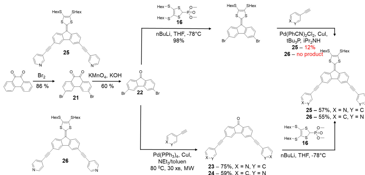
Scheme 3.1.3. Synthesis of the S-Hex DTF based ligands.
