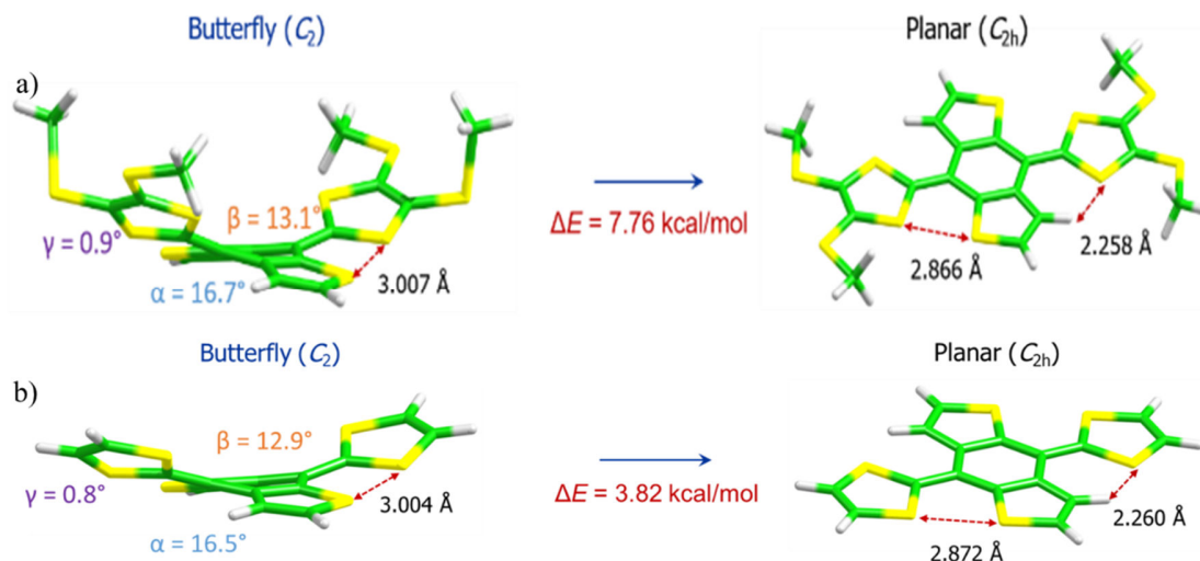
Figure 5.4.3 B3LYP-D3/6-31G** - optimized structure (left) and forced planar structure (right) computed for the radical cation S-exTTF •+ (a) and S-exTTF •+ in which the thiomethyl groups have been removed (b) in CH 2 Cl 2 . The molecular symmetry, the intramolecular contacts and the energy difference between both structures are indicated.
