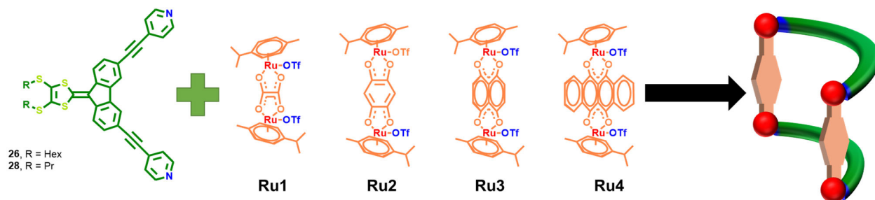
Scheme 3.4.1. Expected of self-assemblies using 4Py-DTF motif in combination with bis -ruthenium acceptors.
