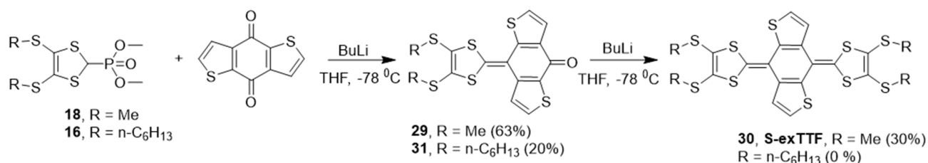
Scheme 5.2.1. Synthesis of the S-exTTF
