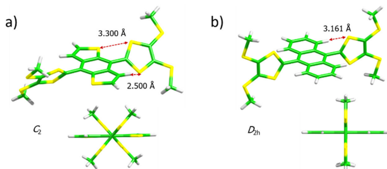
Figure 5.4.4. Minimum-energy B3LYP-D3/6-31G**-optimized geometries computed for S -exTTF 2+ (a) and exTTF 2+ (b) in CH 2 Cl 2 .
