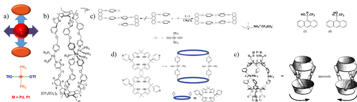
Figure 1.3.5. General structure (a) and examples of application (b, c, d, e) of the trans-blocked acceptor units. 38-41
