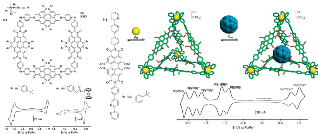
Figure 1.5.3. Redox-active self-assemblies using perylene bisimide (PBI) unit. 113-114
