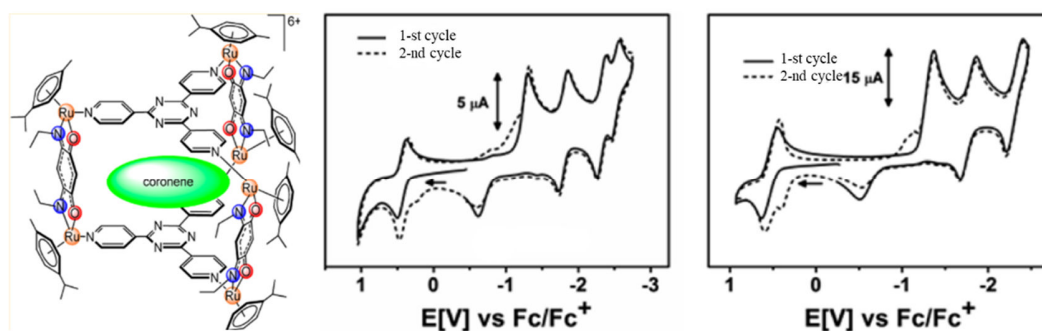
Figure 1.5.2. Ruthenium-based triazine redox-active cage and its cyclic voltammetry. 110
