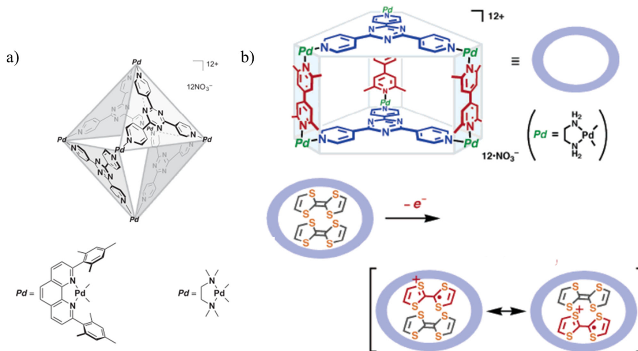
Figure 1.3.4. Examples of self-assembled metallocages using cis -blocked acceptors. 36-37
