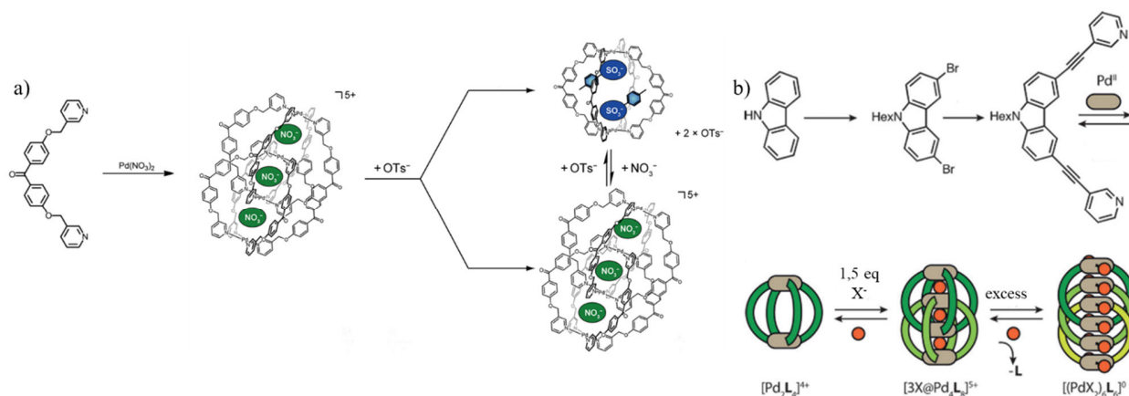
Figure 1.3.16. Interlocked self-assemblies using Palladium complexes. 70-71
