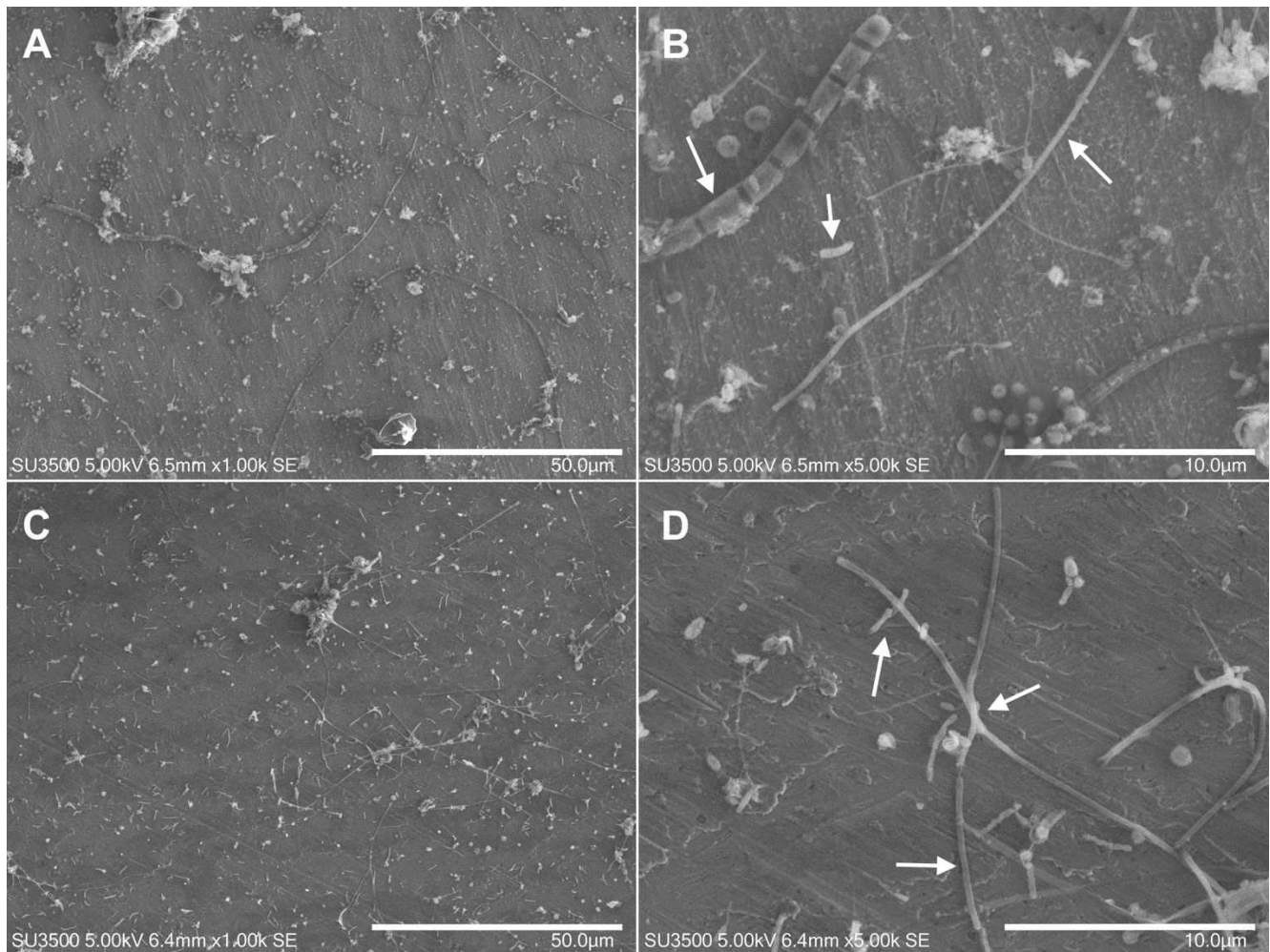
Figure 26. Scanning electron microscopy micrographs at 1K (A, C) and 5K (B, D) magnification. UNS532750 after two weeks of exposure, in aerobic (A, B) and anaerobic (C, D) conditions.
