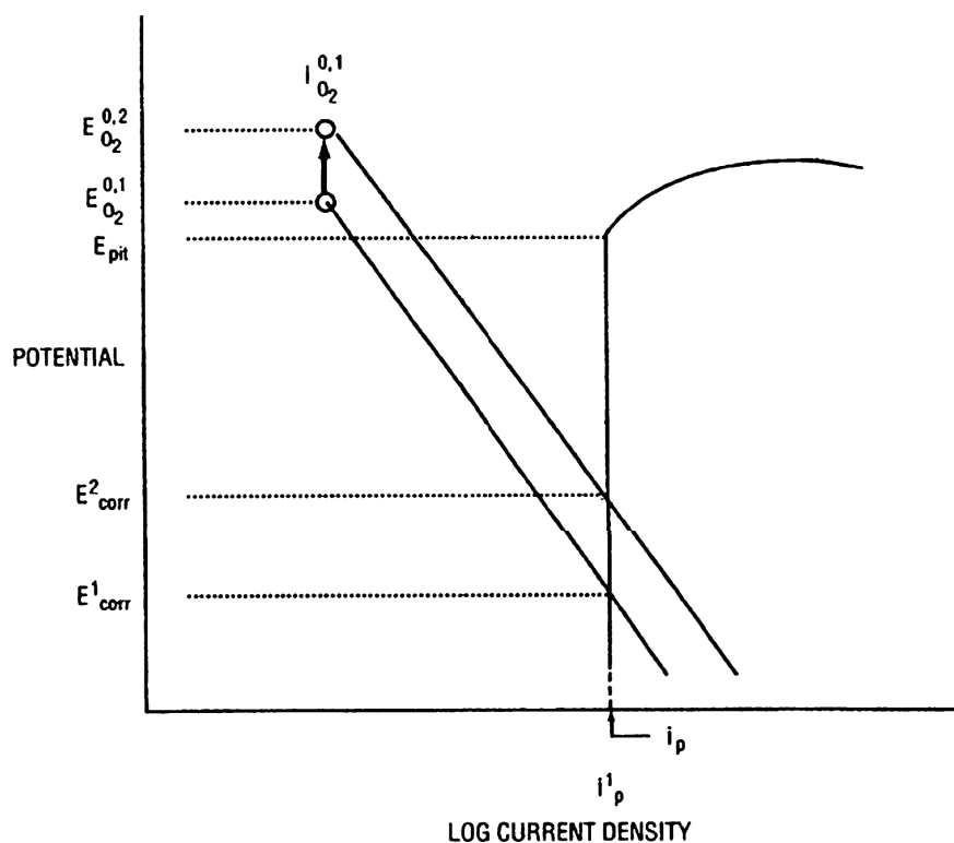
Figure 4. Schematic polarization curve for stainless steel. Change of either pH or O_2 partial pressure would change the reversible potential E_{O_2}^{0.1} to E_{O_2}^{0.2} . As a result, the measured potential (also referred as E_{corr} ) would raise from E_{corr}^1 to E_{corr}^2 . Adapted from (Little et al., 2008).
