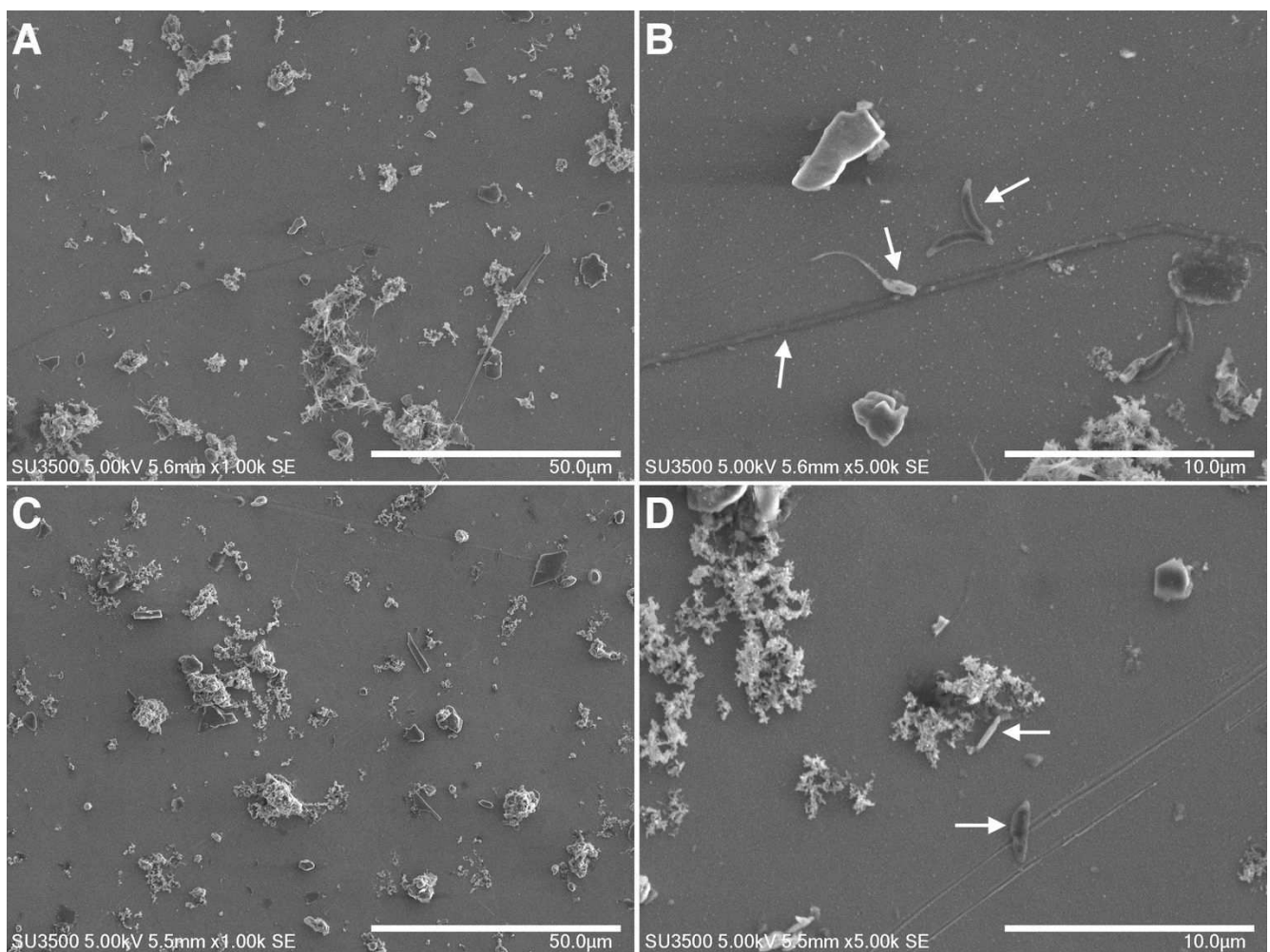
Figure 15. SEM images at 1k (A, C) and 5k (B, D) magnification of stainless steel exposed for one week to seawater and heated to 36°C (A, B) and 40°C (C, D). Some cells are pointed by arrows.
