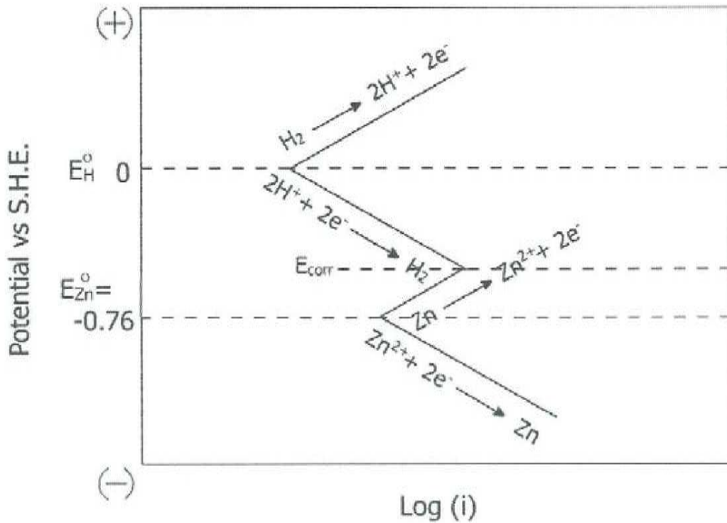
Figure 1. Example of an Evan’s diagram for the oxidation of Zn and the reduction of H + . E_{corr} is the total redox potential. Adapted from (Ahmad, 2006).
