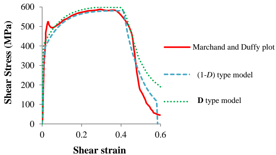
Fig. 3.3 Experimental and simulated shear stress-shear strain curves for Marchand and Duffy torsion test.
