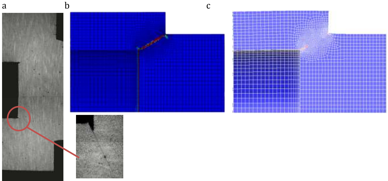
Fig. 3.9 Configuration with L_{striker}=200 mm; V_{striker}=17.8 m/s. (a) Specimen post-mortem; (b) numerical deterioration map of (1-D) type model (Step time = 9 \mu s); (c) numerical deterioration map of D type model (Step time = 100 \mu s). After [1].
