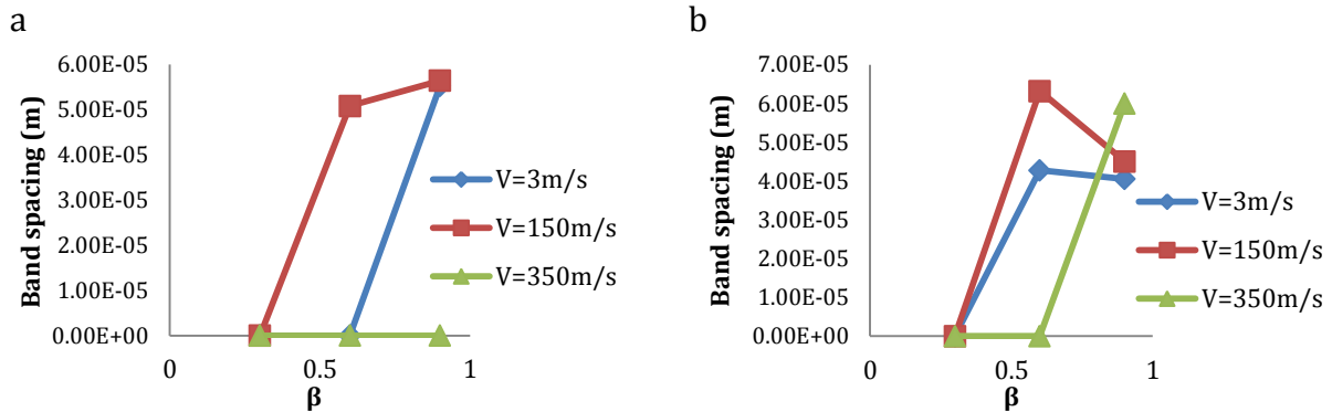
Fig. 3.29 Variation of shear banding spacing with \beta for (a) Full coupling (b) Weak coupling
