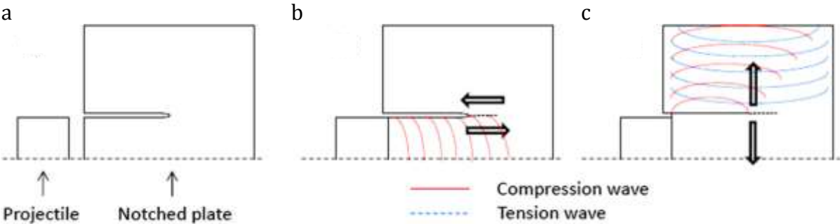
Fig. 2.21 After [23]. Schematic representation of possible wave propagation during KW impact test. (a) Configuration before impact accounting for plane symmetry. (b) Shear wave in the impact direction propagation. (c) Tension wave in the perpendicular direction
