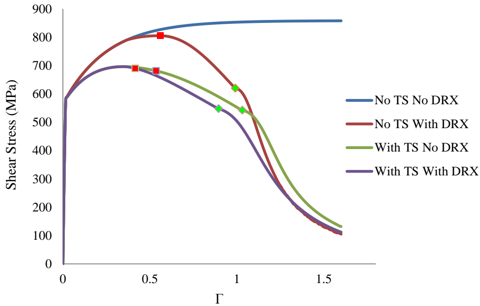
Fig. 2.30 Shear stress vs shear strain for different cases of thermal softening and DRX induced softning.
