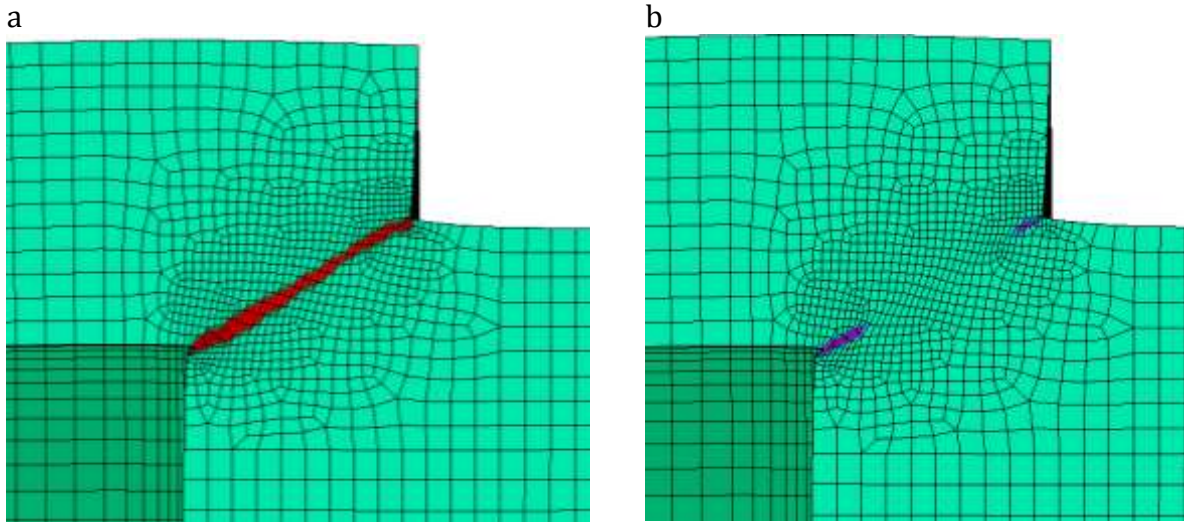
Fig. 3.20 Map of the degradation variable indicator at 40.5 \mu s. Configuration with ASB+MV. Numerical simulation of the dynamic loading of HSS. a) Elements in red are subject to ASB. b) Elements in magenta are subject to MV.
