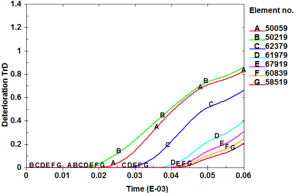
Fig. 3.17 Degradation variable history in finite elements located inside the strip of intense shearing, see Fig. 3.11. Configuration with ASB only. Numerical simulation of the dynamic loading of HSS.
