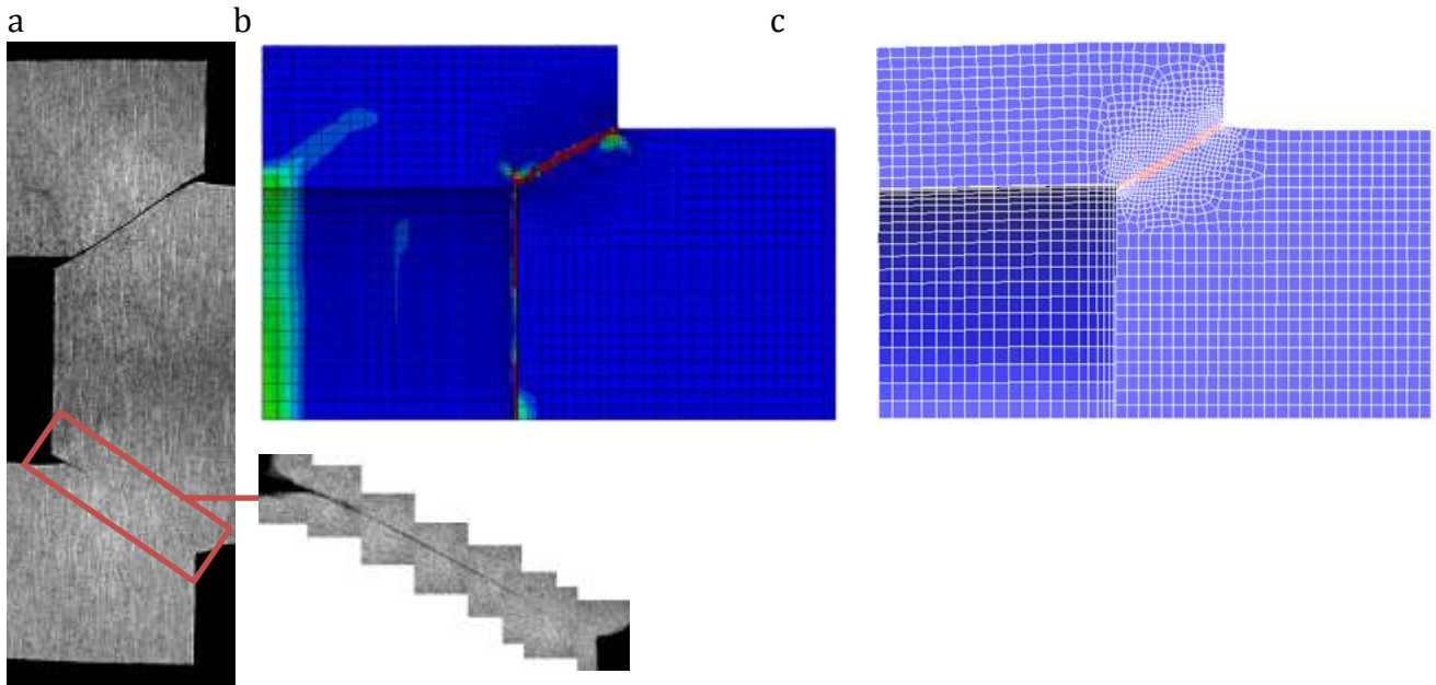
Fig. 3.5 Configuration with L_{striker}=40 mm; V_{striker}=35.6 m/s. (a) Specimen post-mortem; (b) numerical deterioration map of (1-D) type model (Step time = 6 \mu s ); (c) numerical deterioration map of D type model (Step time = 40 \mu s ). After [1].
