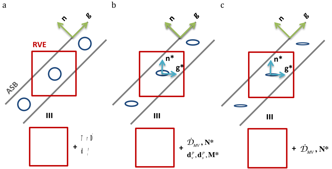
Fig. 2.15 Illustration of micro-void configurations. a) Spherical void configuration b) Ellipsoidal void configuration c) Micro-crack configuration.
