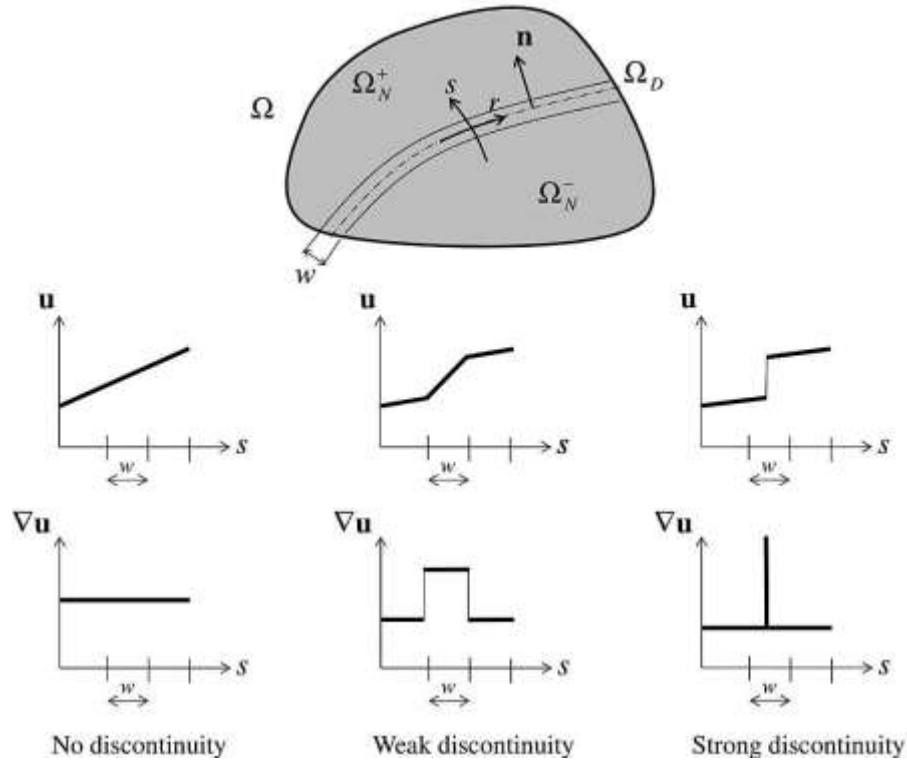
Fig. 2.12 Displacement and strain fields in different cases of discontinuity. After [20]
