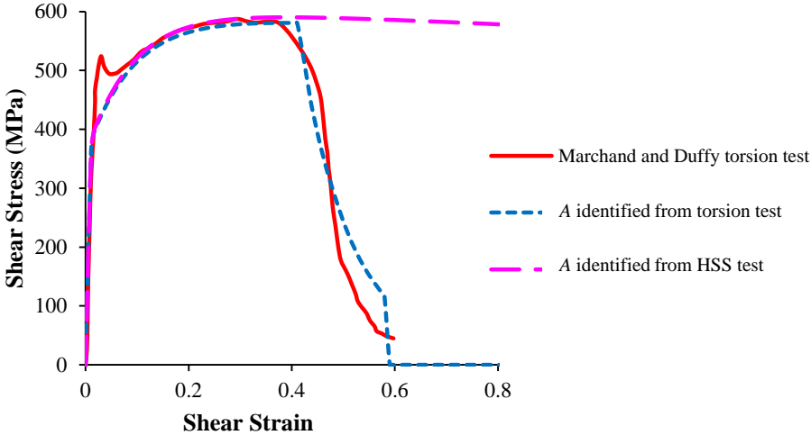
Fig. 3.14 (1-D) type model shear stress-shear strain plot for torsion test. The simulated post critical response is strongly dependent on the experiment (torsion test vs. HSS test) considered for the calibration of the constant A
