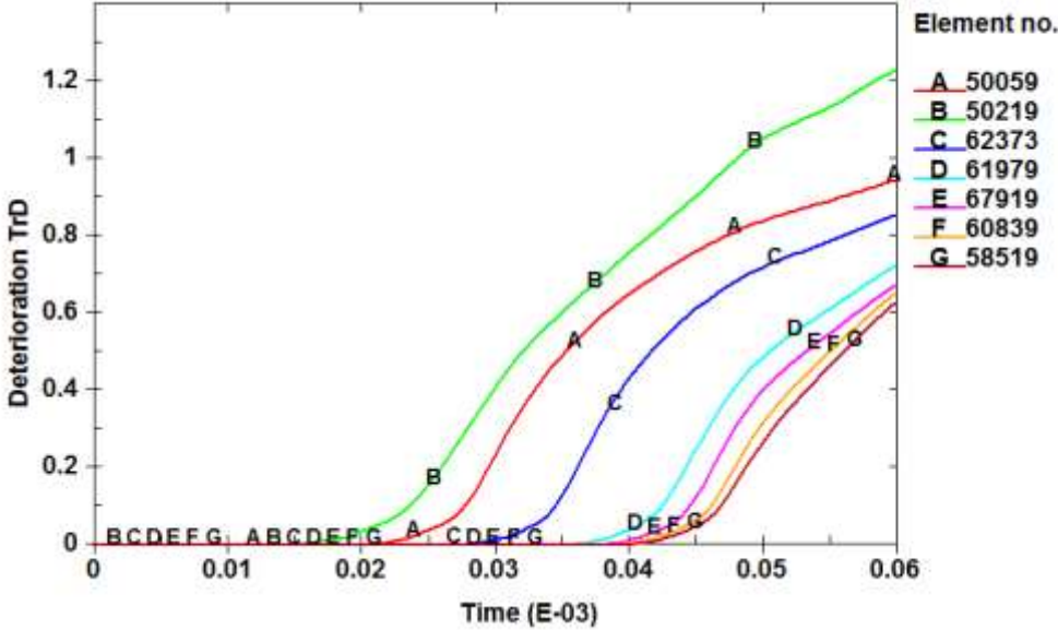
Fig. 3.18 Degradation variable history in finite elements located inside the strip of intense shearing, see Fig. 3.11. Configuration with ASB+MV. Numerical simulation of the dynamic loading of HSS.
