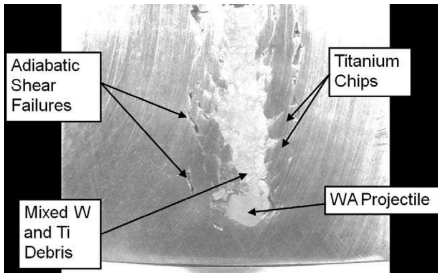
Fig. 1.5 ASB formed in titanium alloy plate allows the deep penetration of tungsten penetrator. After [4].
