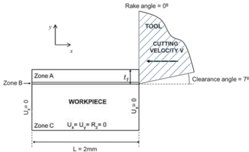
Fig. 3.23 High speed orthogonal machining configuration. After [18].
