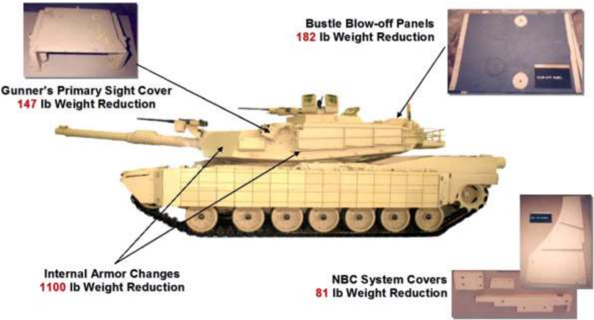
Fig. 1.11 Titanium weight reduction program for US army battle tank. After [4].
