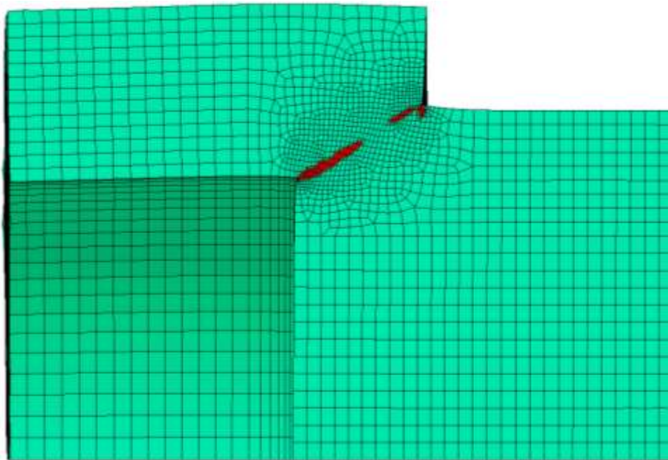
Fig. 3.19 Map of the degradation variable indicator at 40.5\mu\text{s} . Elements in red/dark are subject to ASB. Configuration with ASB only. Numerical simulation of the dynamic loading of HSS.
