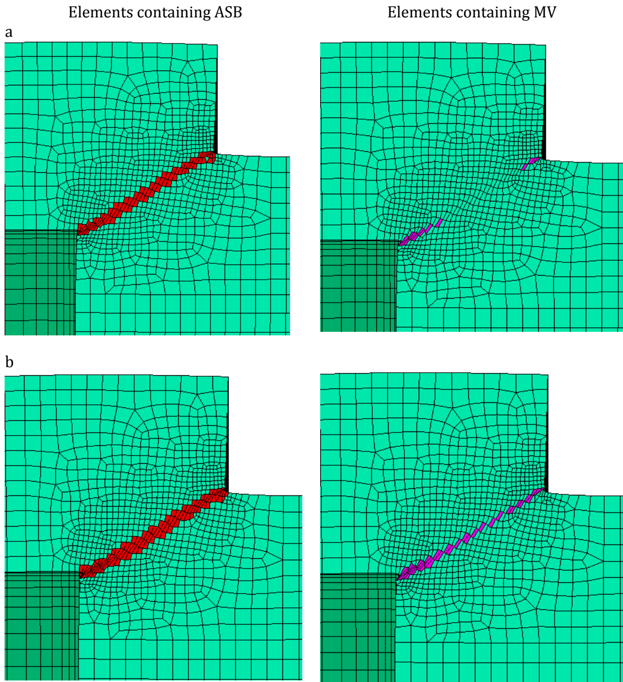
Fig. 3.22 Map of the degradation variable indicator at 40.5\mu\text{s} . Configuration with ASB+MV. Numerical simulation of the dynamic loading of Ti6Al4V hat shaped structure. Elements in red/dark are subject to ASB. Elements in magenta/dark are subject to MV. a) Case of no thermal softening and with DRX b) Case considering thermal softening and DRX.
