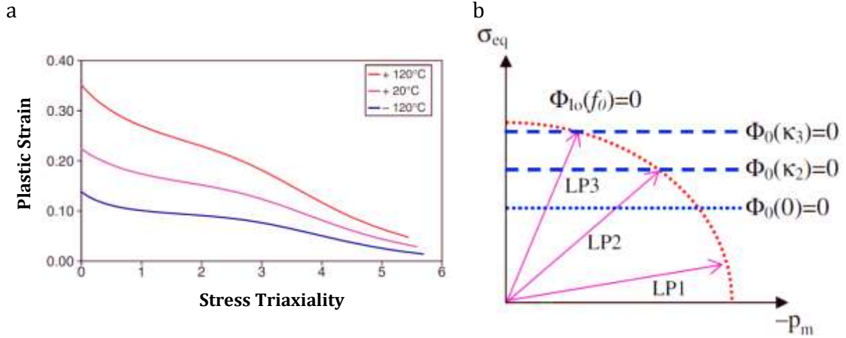
Fig. 2.24 After [61] a) Plastic strain at hole nucleation vs. stress triaxiality b) Illustration of various loading paths on the map of initial and current elastic domains and the void nucleation locus.
