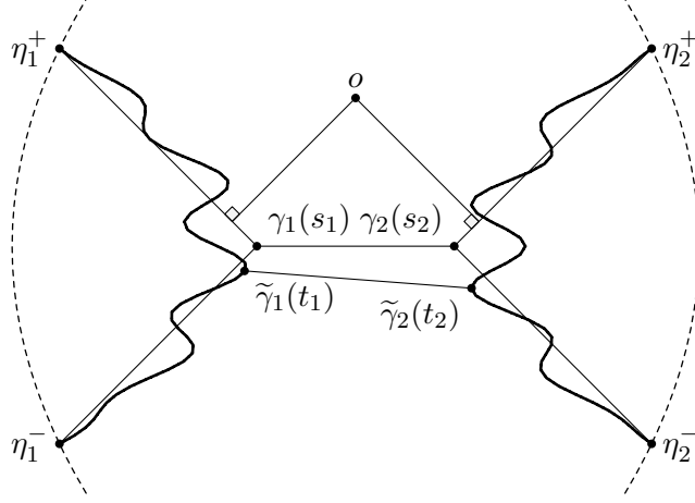
Figure 14: Main points occurring in the proof of Lemma I.37. Straight, resp. wavy lines depict geodesic, resp. O(u) -geodesic lines; the boundary is dashed.
