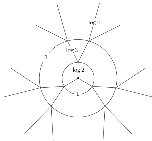
Figure 21: A metric graph (The underlying tree is that of figure 5, but we do not mean to relate them beyond this. The resulting graph is one-ended).
