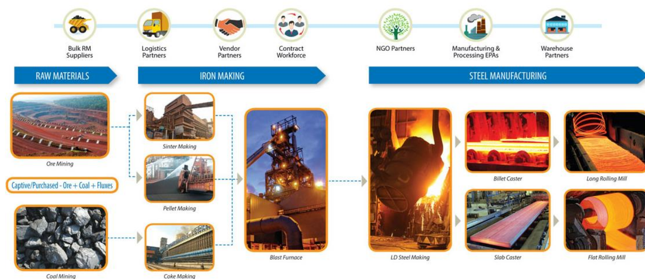
Figure 2.1.4.14 - Crude steel production Value Chain, adapted from (Tata Steel, 2014).
