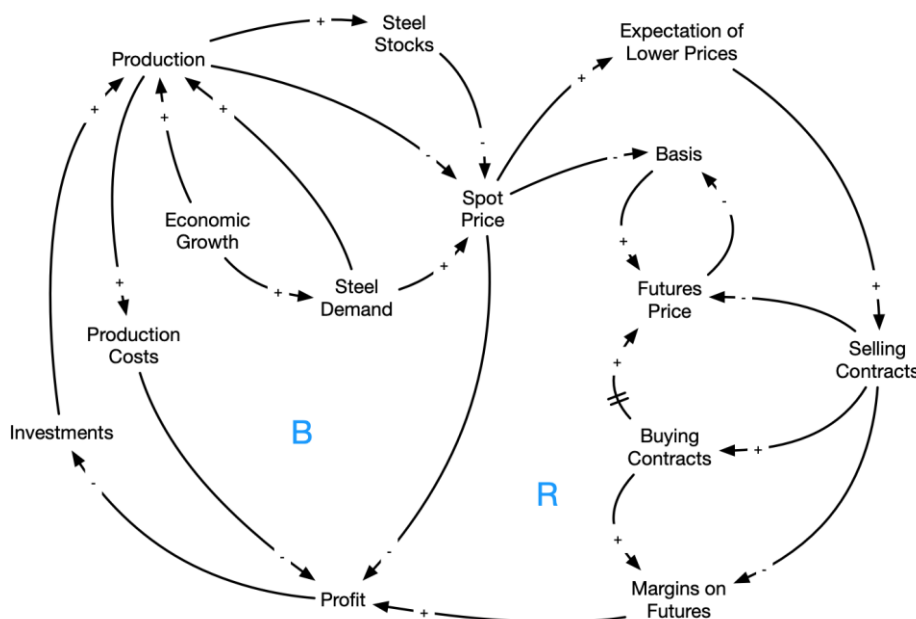
Figure 4 - Hedging dynamics.
