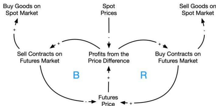
Figure 2.1.3.12 - Arbitrage dynamics (developed by the author).
