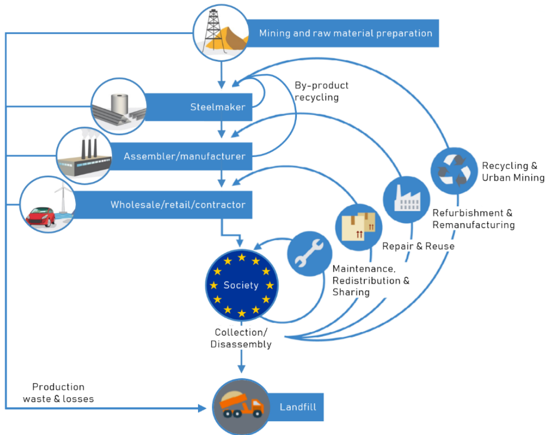
Figure 3.1.25 - Steel's life cycle as per the Circular Economy framework (developed by the author).
