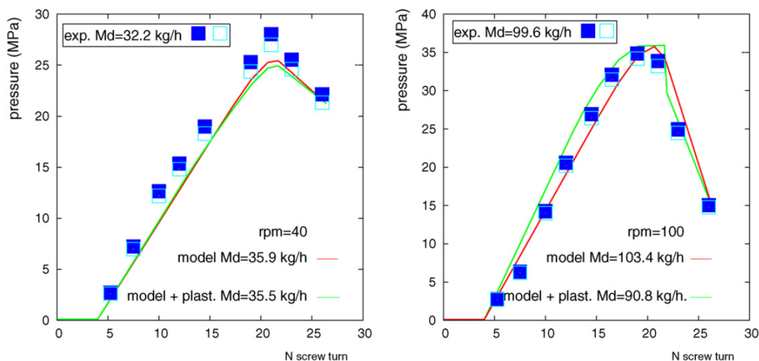
Figure 1.7: Model predictions (with and without plastification included) plotted against experimental data [HAN 90] of pressure along 63.5 mm diameter screw for LDPE at 40 and 100 rpm. [BÉR 09]
