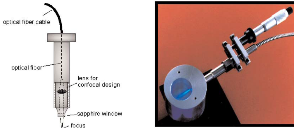
Figure 1.12: Schematic representation of the confocal optical sensor with micrometer movement [BUR 04].
