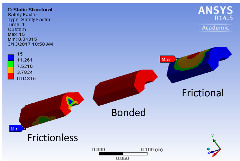
Figure 5.6: The safety factor distribution of the 3 glass blocks with different contact types under a temperature condition of 100°C (Friction coefficient between glass and steel is set as 0.6)
