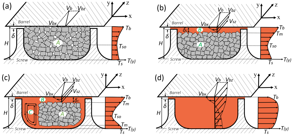
Figure 2.2: Cross-section schematic of plastification process along the screw channel: (a) solid bed conveying zone, (b) delay zone, (c) melting zone, and (d) metering zone. (A) Solid bed, (B) melt film, (C) melt pool.
