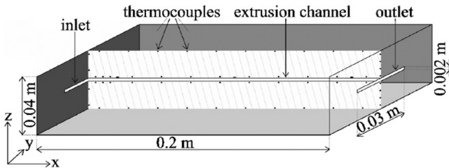
Figure 1.9: Schematic representation of extrusion die [PUJ 08].
