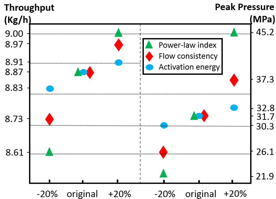
Figure 2.10: The effect of 20% variations of flow consistency, power-law index, and activation energy on the fluctuations of throughput and peak pressure of plastication process
