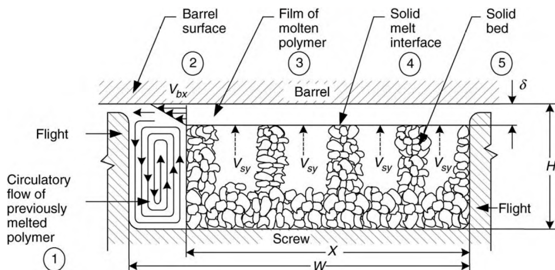
Figure 1.3: Cross-section in the melting zone of a single screw extruder [TAD 70].
