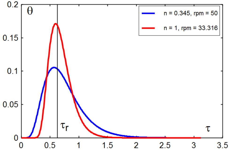
Figure 3.9: Comparison of dispersion behavior of thermal fluctuations with different power-law index of fluid. Two cases with same throughput of 2.0 \text{ cm}^3/\text{s} and same back pressure of 91.2 \text{ MPa} but different power-law index: Red curve case n = 1 with 33.316 \text{ rpm} screw rotation frequency, blue curve case n = 0.345 with 50 \text{ rpm} .
