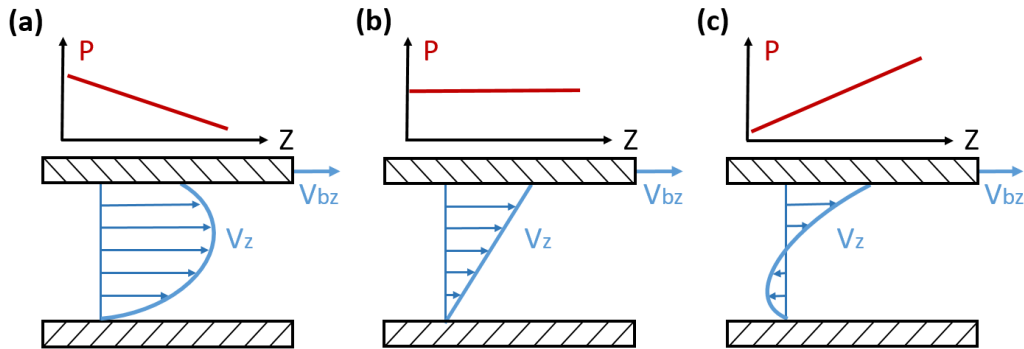
Figure 3.1: Sketch of the three different possible flow configurations: (a) drag and pressure flow, (b) drag flow and (c) drag and backpressure flow.
