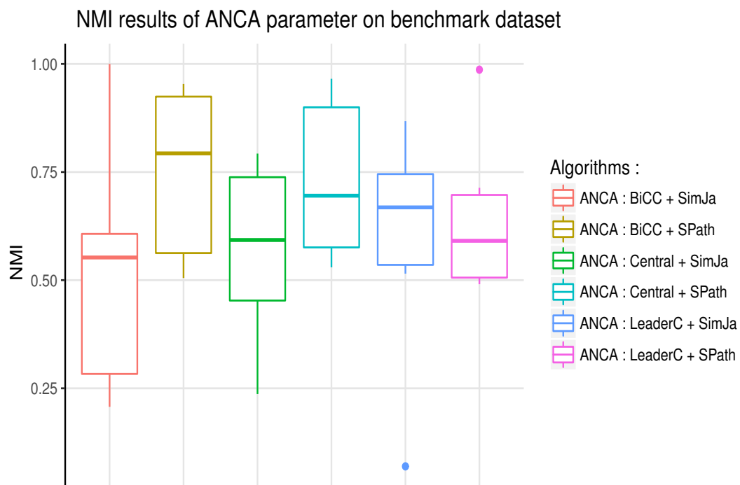
FIGURE 3.5: Evaluation of n-ANCA parameters according to normalize mutual information (NMI).
