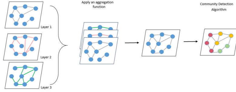
FIGURE 2.2: Layer Aggregation
