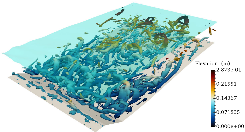
Figure 4.19: Instantaneous isosurfaces of \lambda_2 criterion.
