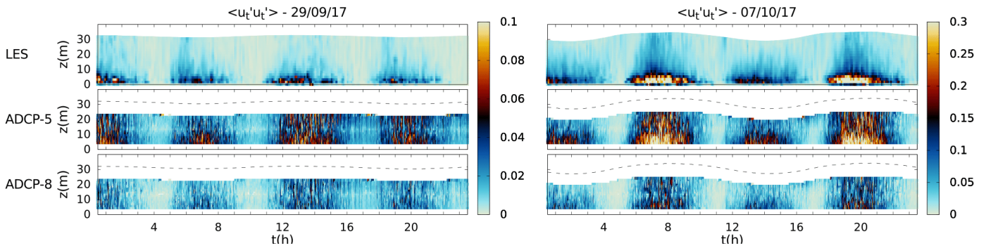
Figure 5.12: Temporal vertical profile of the Reynolds stress \langle u'_t u'_t \rangle ( \text{m}^2\text{s}^{-2} ) on the 29/09/17 and the 07/10/17.
