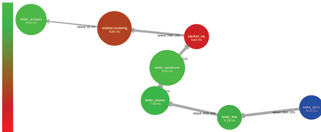
FIGURE 3.24: RePLoD visualization performance at time t1 .
