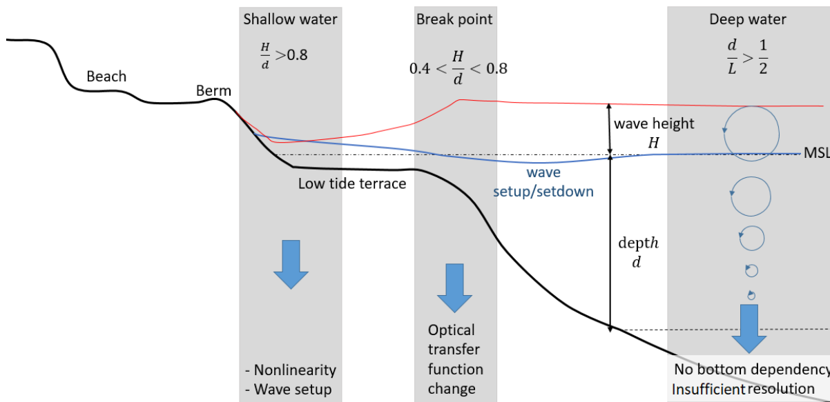
Figure 6.10: Description of the main sources of error for the use of video-based depth inversion methods. Namely, non-linearity and wave-setup in shallow area, optical modulation transfer function change at the breakpoint and relative deep water conditions for shortest waves.
