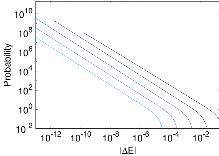
Figure 2.5: b. Plot for a function y(q) that diverges with \mu = \mu_{SK} = \mu_{\text{UNSAT}} = \frac{1}{2} , for several perturbations (from the left to the right, with \gamma = 10^{-5}, 10^{-4}, 10^{-3}, 10^{-2}, 10^{-1} ); here, the exponent of the power law displays minor corrections for larger field.
